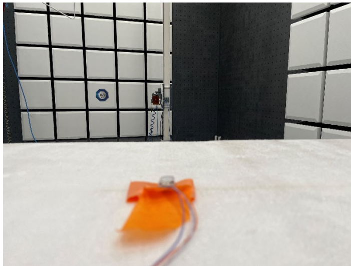
Radiated Emissions Test Setup (18GHz to 26GHz)
