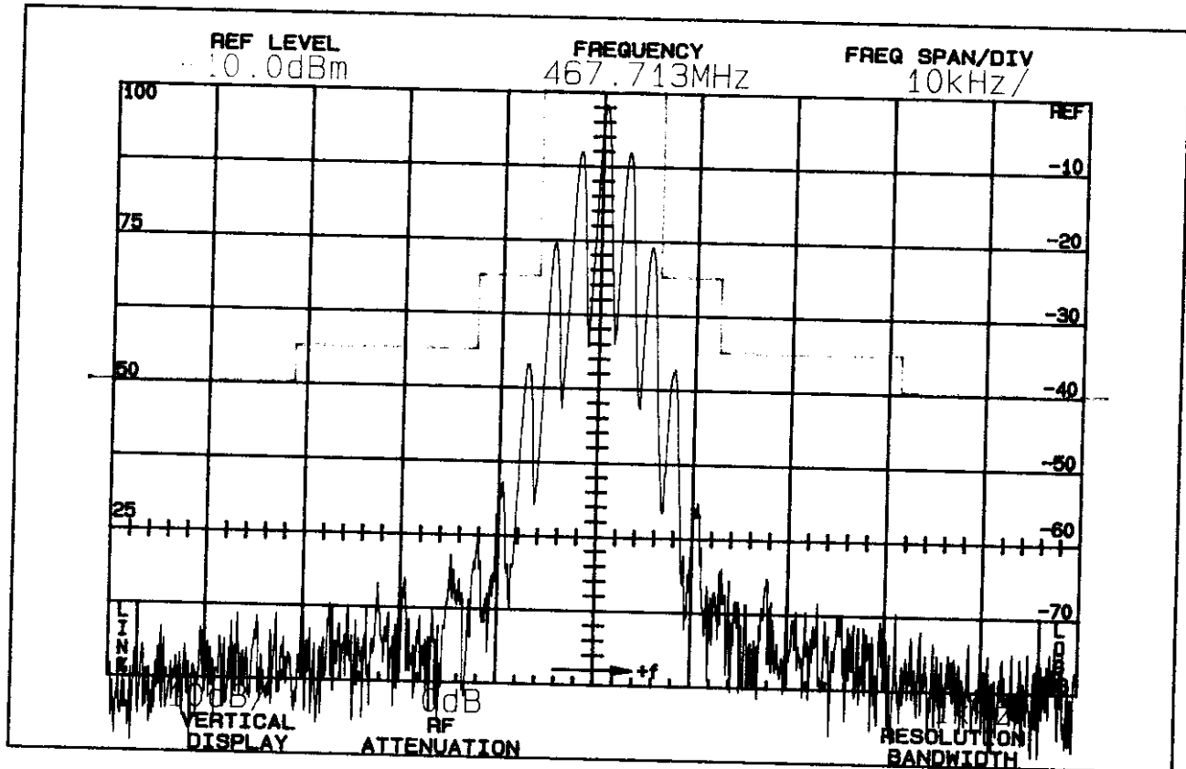
FIGURE 4 OCCUPIED BANDWIDTH
