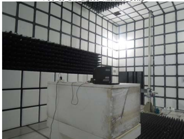
FCC 15 247 Zigbee Radiated Setup
