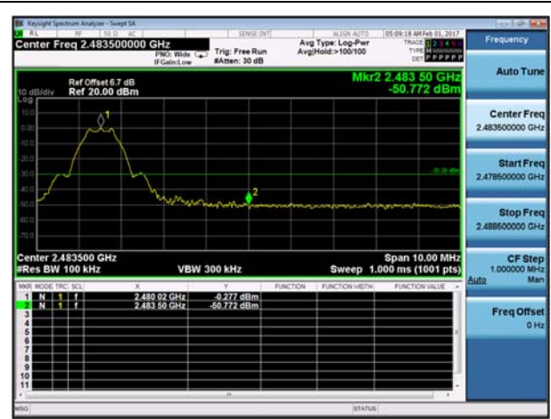
Band Edge-LE High
