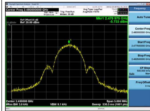
PSD -Bluetooth LE High
