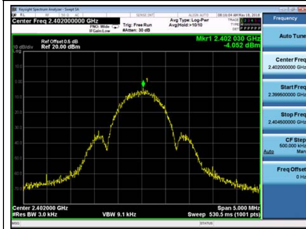
PSD -Bluetooth LE Low
