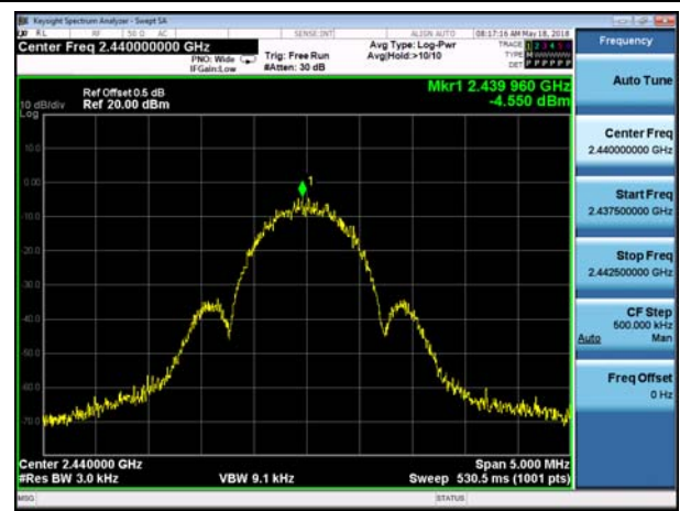
PSD -Bluetooth LE Mid
