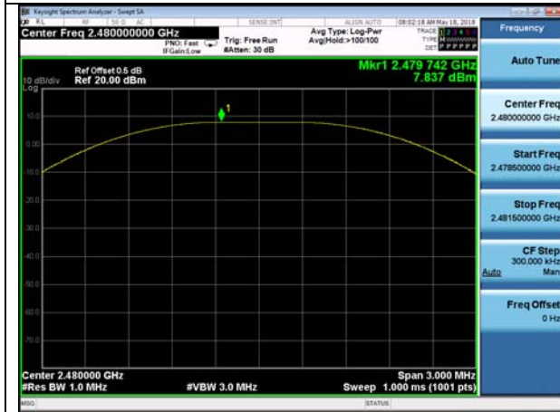
Output Power –Bluetooth LE 2480MHz
