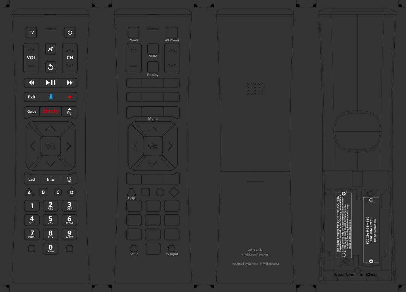
Keypad Artwork Top Case Artwork Bottom Case Artwork PCB Artwork & Country of Origin
