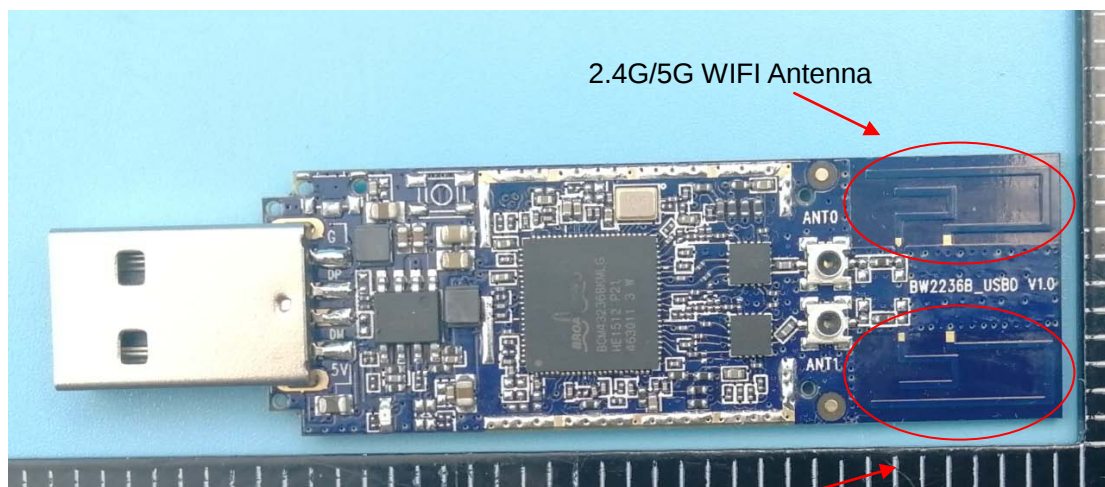
2.4G/5G WIFI Antenna
