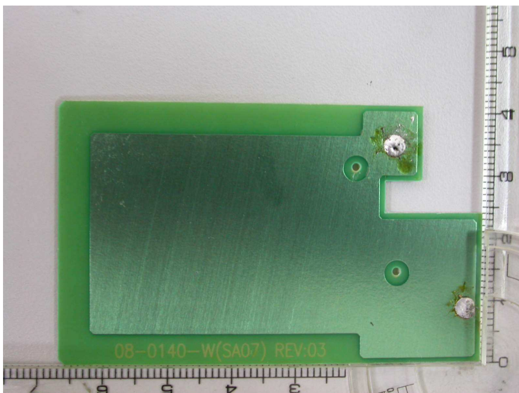
18. Front view of PCB2 (adaptor)
