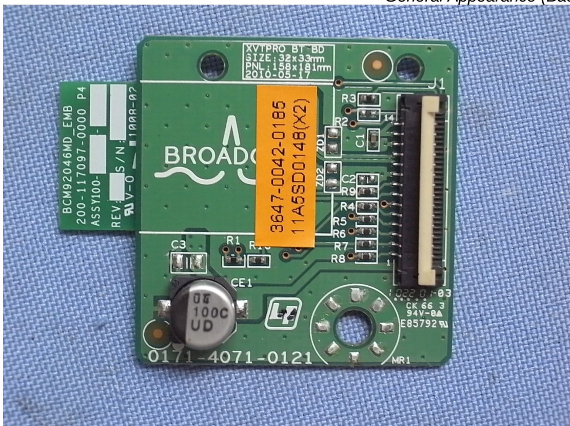
General Appearance (Back View)
