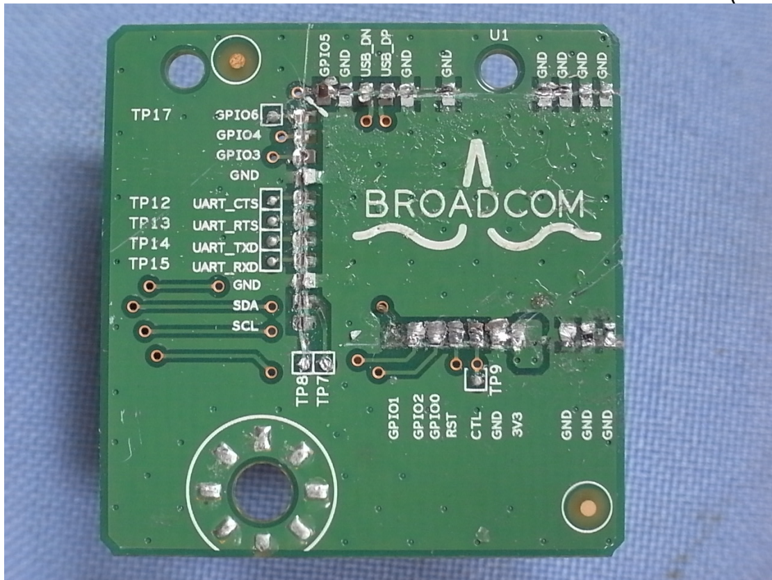
Photo 3 PCB (Front View)
