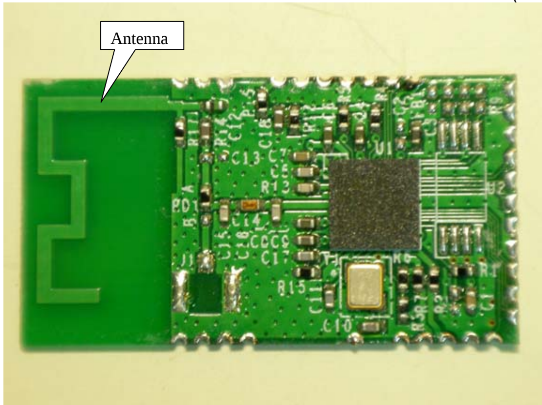
Photo 5 PCB (Front View)
