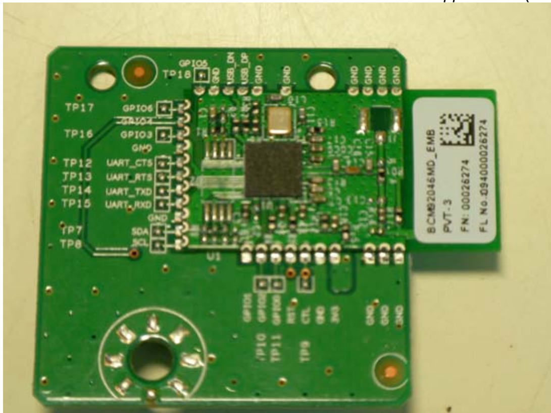
General Appearance (Front View)
