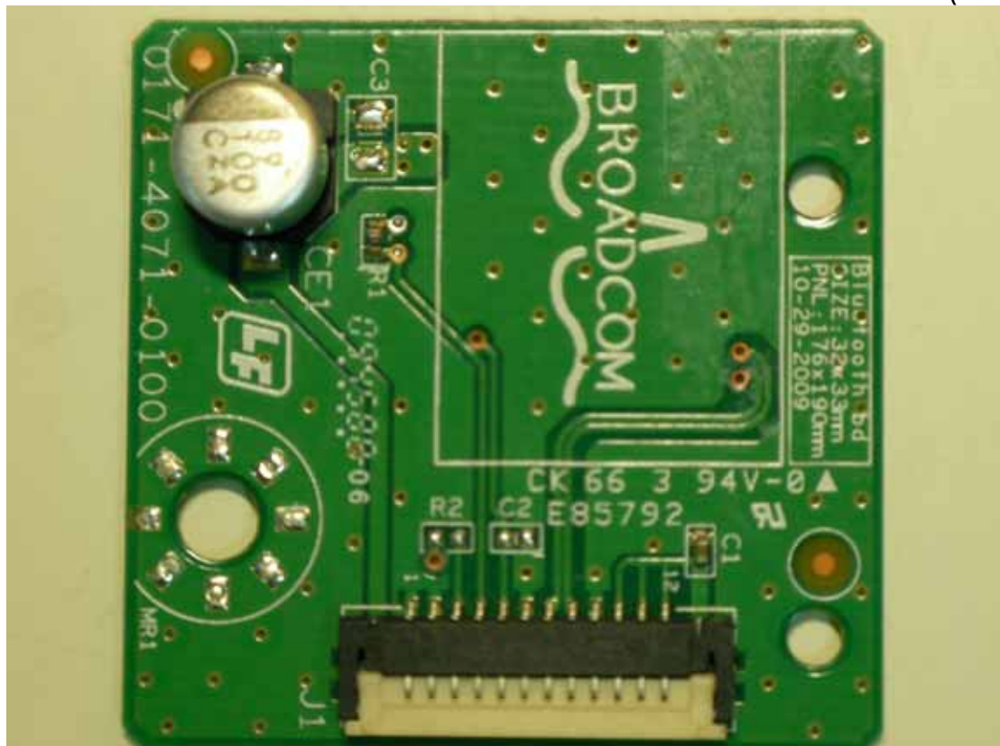
Photo 4 PCB (Back View)
