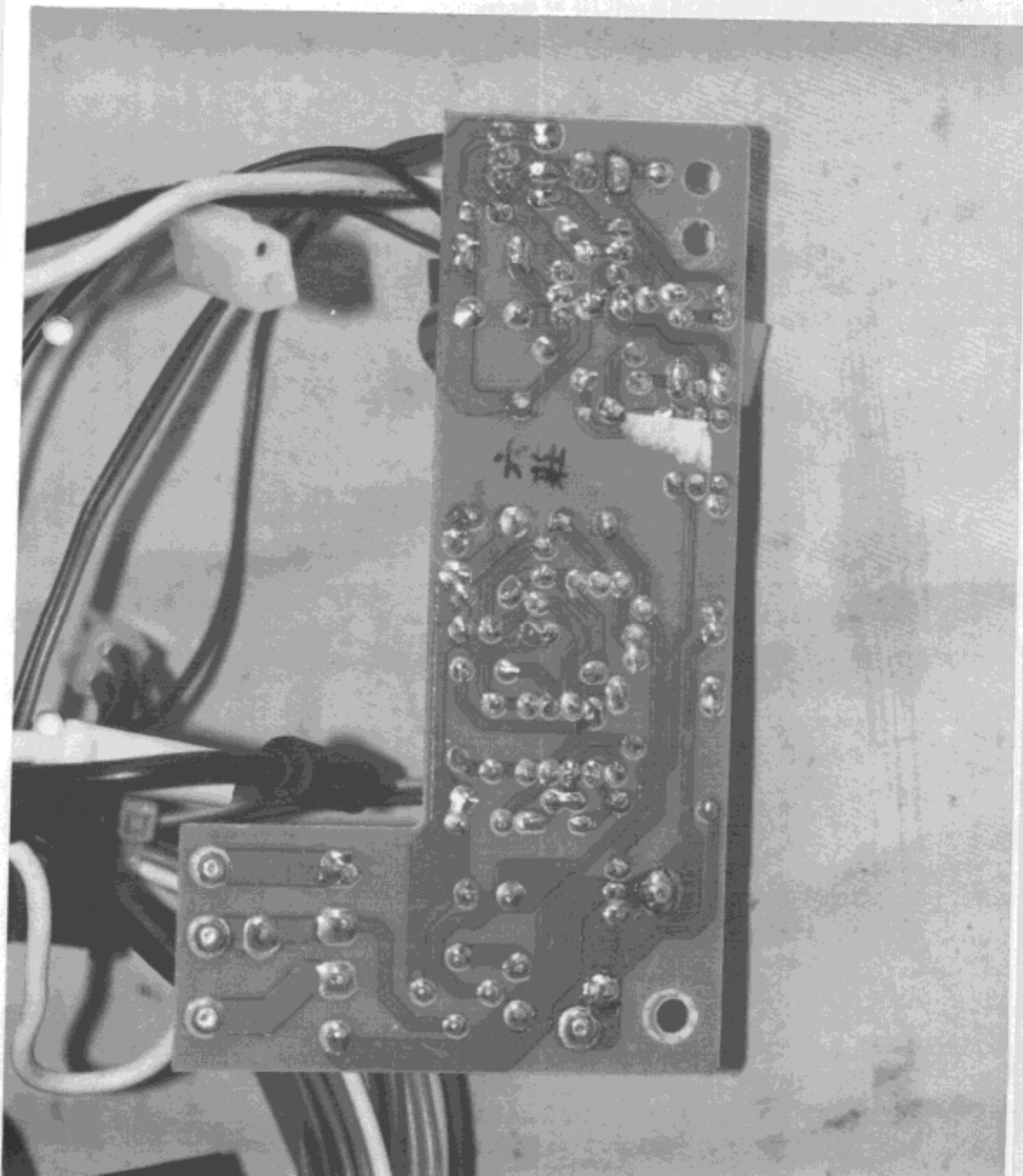
Figure 22 Switching Power Supply (Filter Board, Solder Side)
