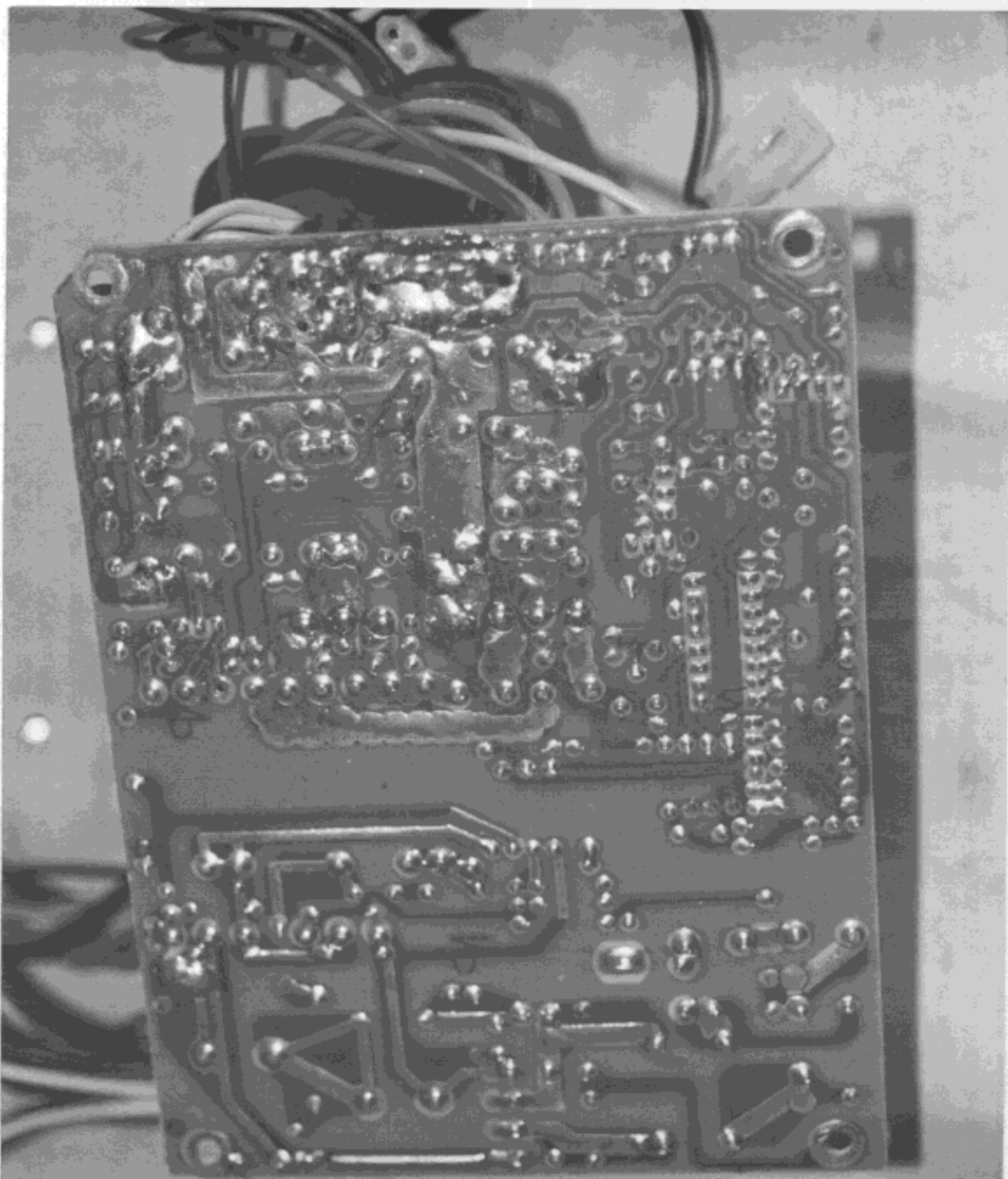
Figure 20 Switching Power Supply (PCB View, Solder Side)
