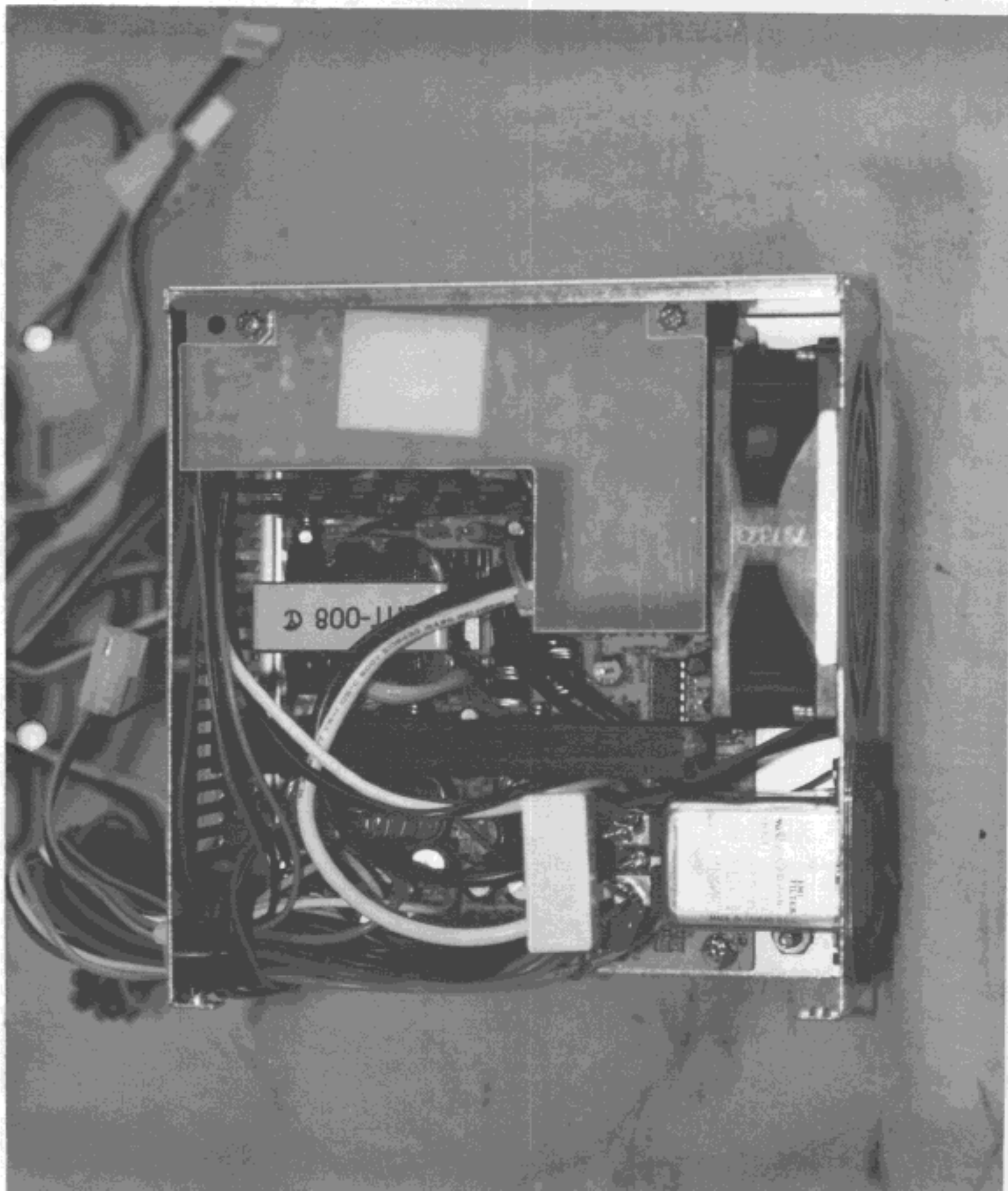
Figure 18 Switching Power Supply (Removed Case Cover, Internal View)
