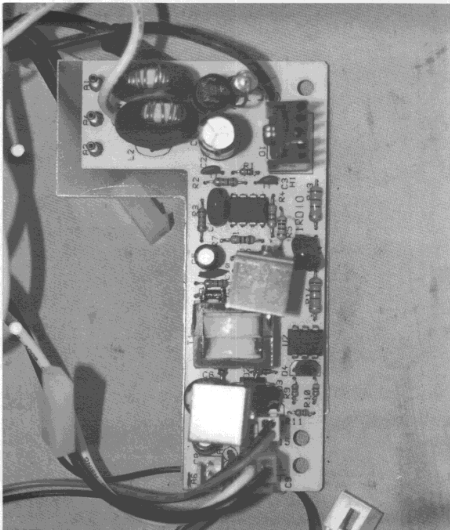
Figure 21 Switching Power Supply (Filter Board, Component Side)
