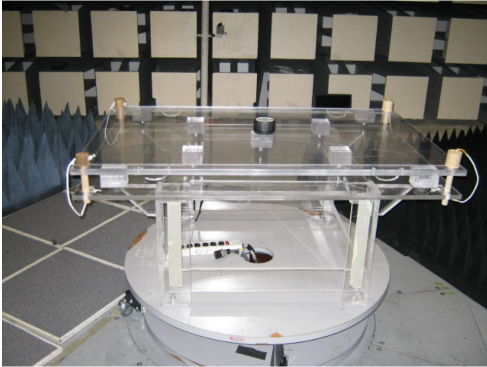
Radiated Spurious, Power, and Band Edge Tests, Front View
