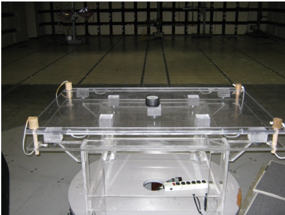
Radiated Spurious, Power, and Band Edge Tests, Back View
