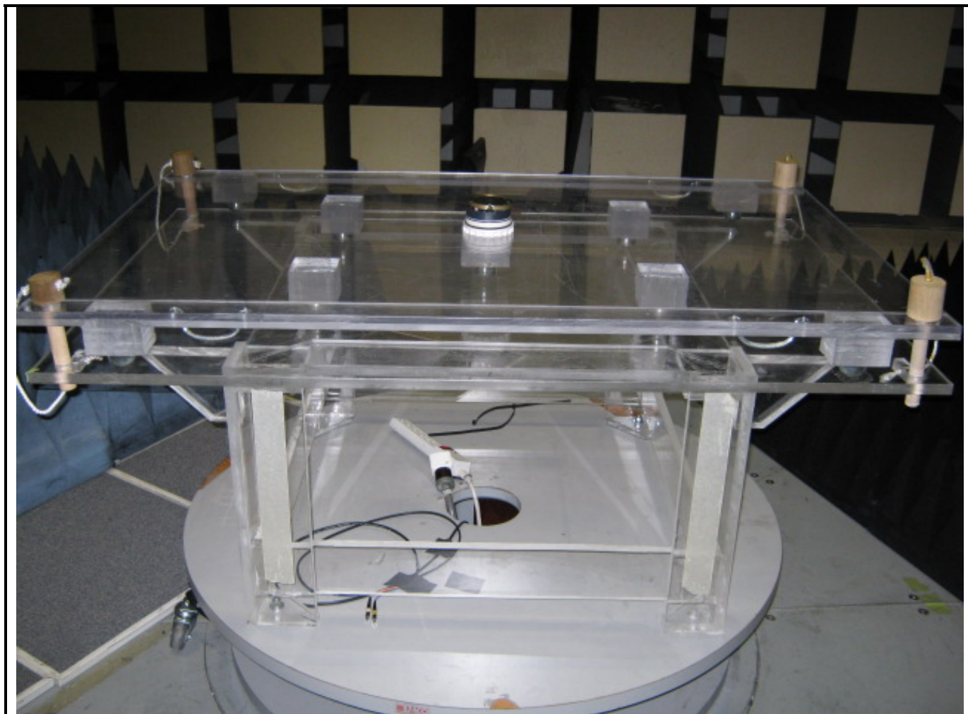
Radiated Tests Below 1 GHz
