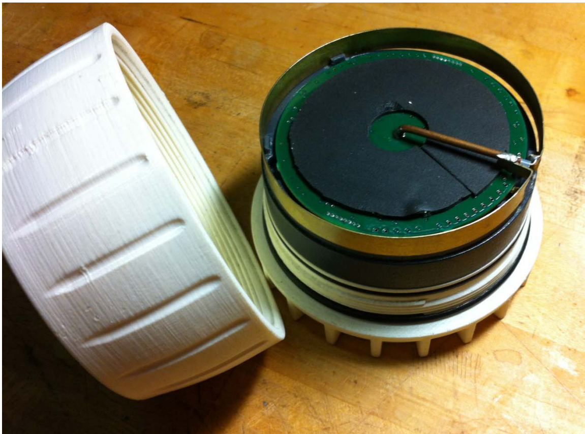
Figure 2 Top Removed, Reveals Loop Antenna and Ferrite for Magnetic Vehicle Sensors
