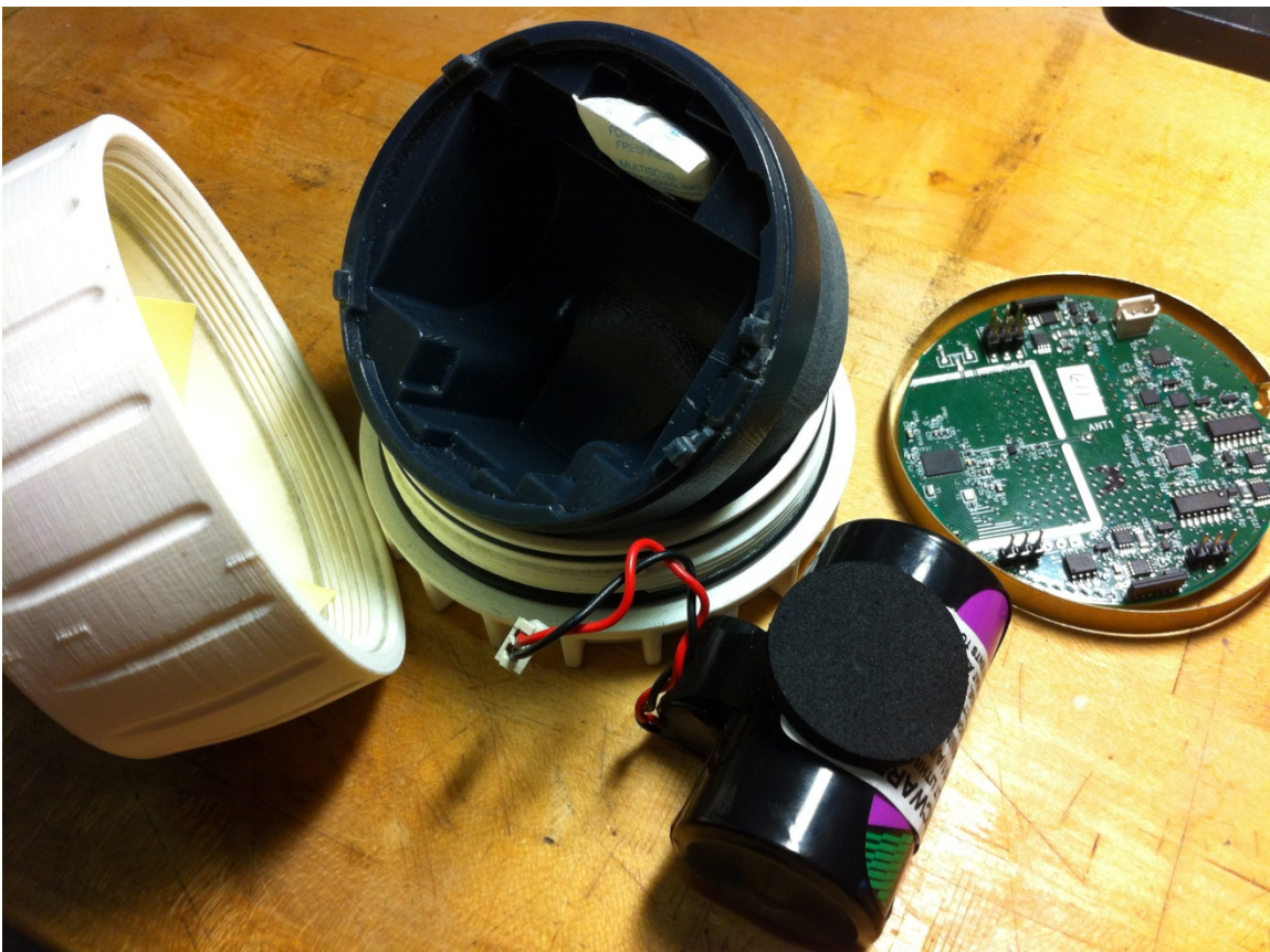
Figure 4 Battery Removed to Reveal Inner Case Construction
