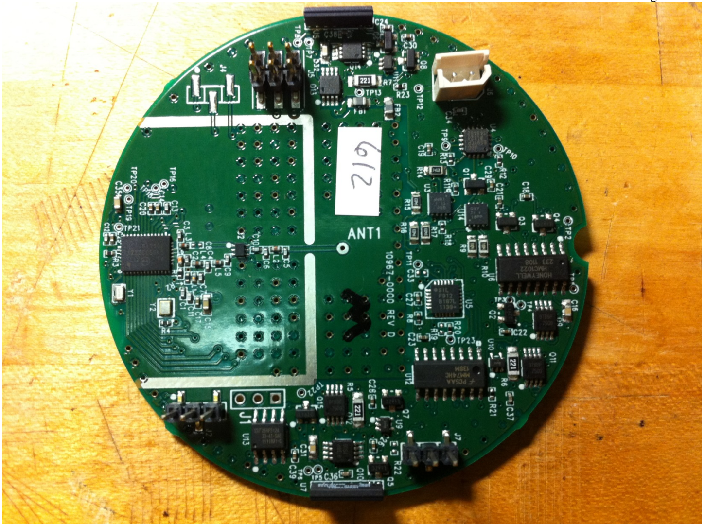
Figure 7 Circuit Card Assembly without Loop Antenna - Component Side
