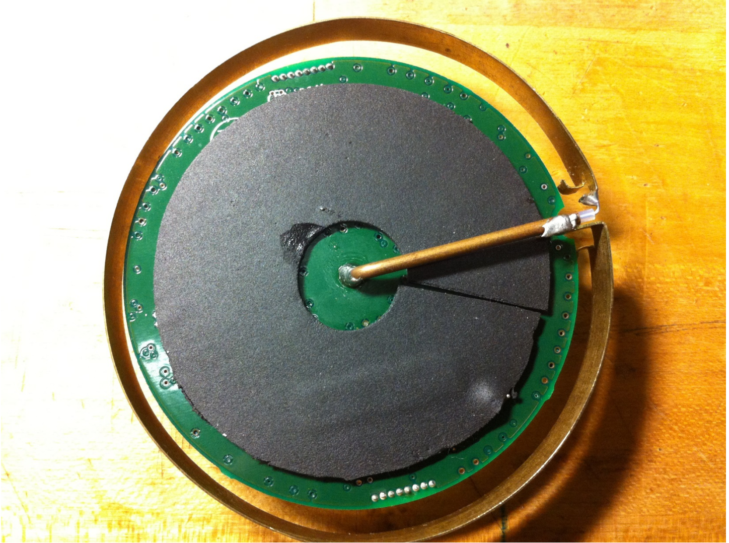
Figure 6 Circuit Card Assembly Non-component Side with Ferrite for Magnetic Vehicle Sensors Visible
