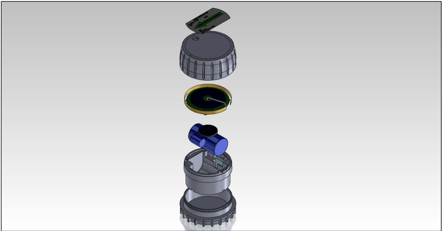
Figure 1 Illustrated Exploded Diagram To Aid in Viewing Photographs
