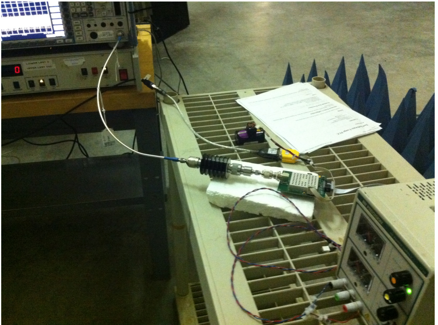
Power, Bandwidth
