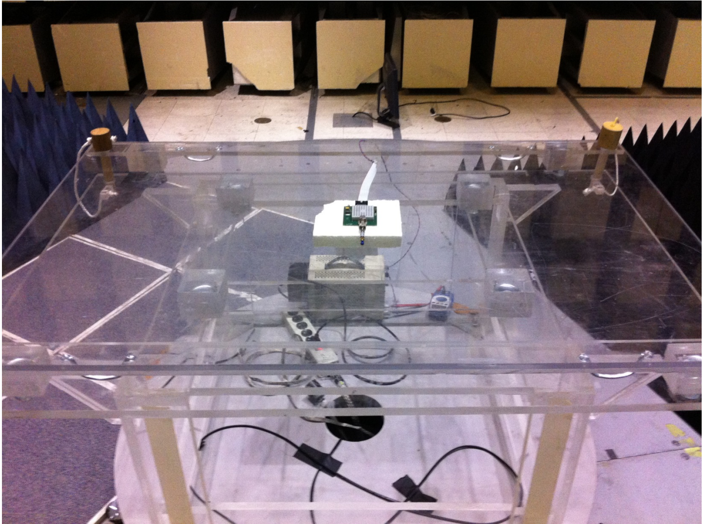
Radiated Emissions Below 1 GHz
