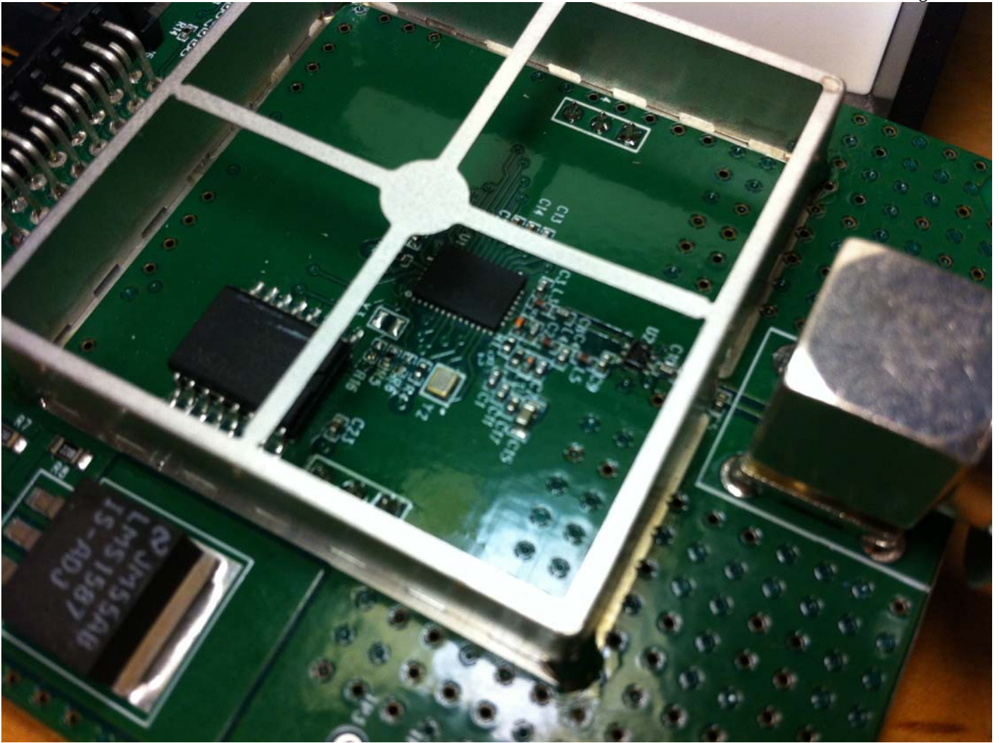
Figure 4 - Shield Removed, Oblique View 1 st Angle, Component Side
