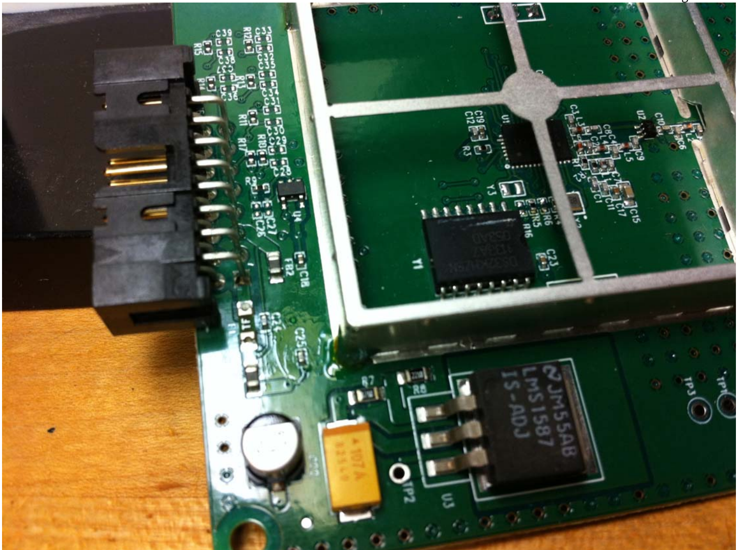
Figure 5 - Shield Removed, Oblique View 2 nd Angle, Component Side
