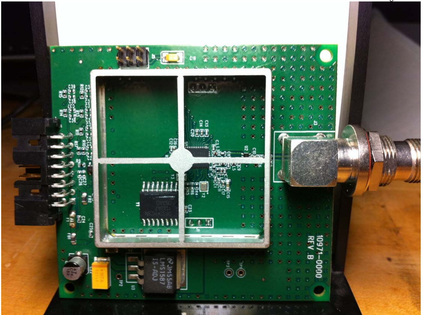
Figure 2 - Shield Removed, Top View, Component Side
