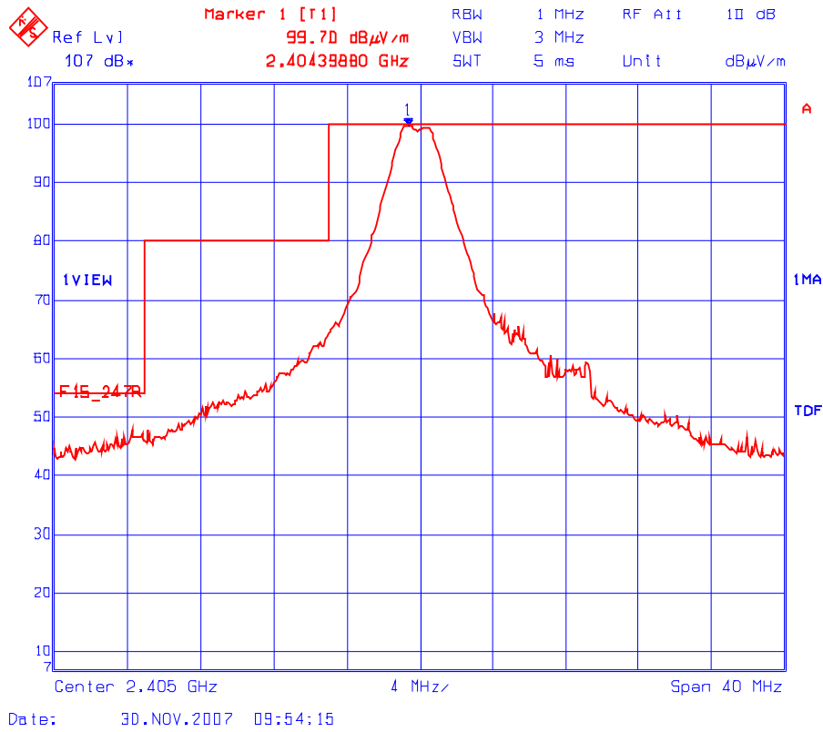
Plot 6.9.5.2 Band-Edge RF Radiated Emissions @ 3 m Low End of Frequency Band Rx Antenna Orientation: Vertical
