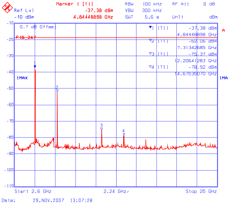
Plot 6.8.5.2.2(ii) Spurious RF Conducted Emissions Transmitter Frequency: 2440 MHz
