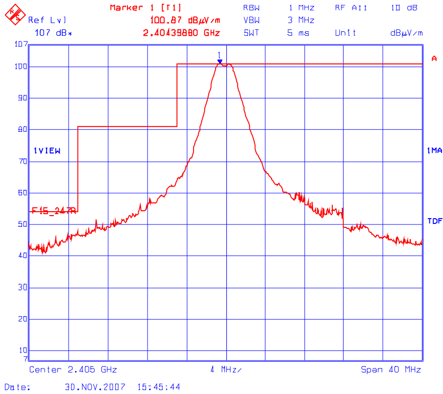
Plot 6.9.5.1 Band-Edge RF Radiated Emissions @ 3 m Low End of Frequency Band Rx Antenna Orientation: Horizontal
