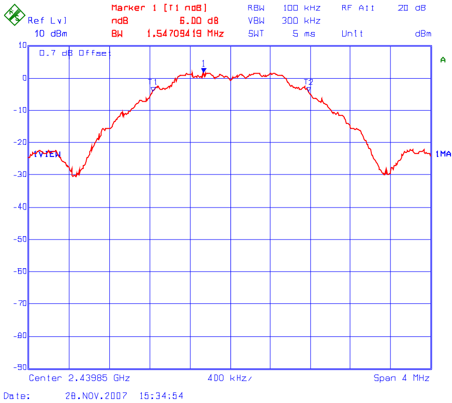
Plot 6.6.5.2 6 dB Bandwidth Frequency: 2440 MHz
