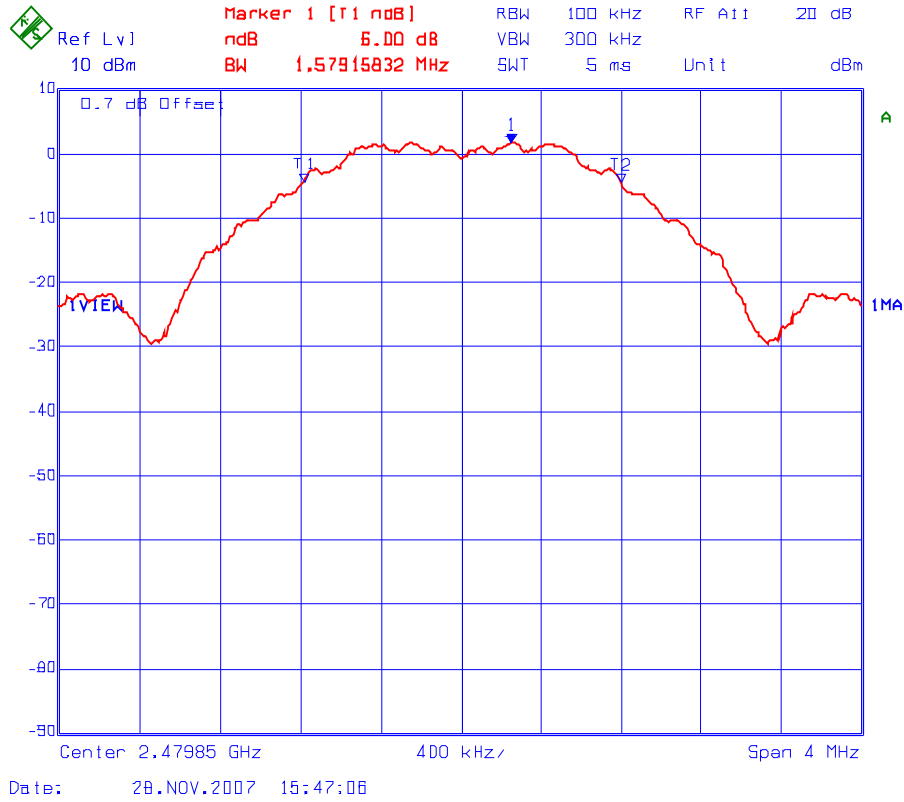
Plot 6.6.5.3 6 dB Bandwidth Frequency: 2480 MHz
