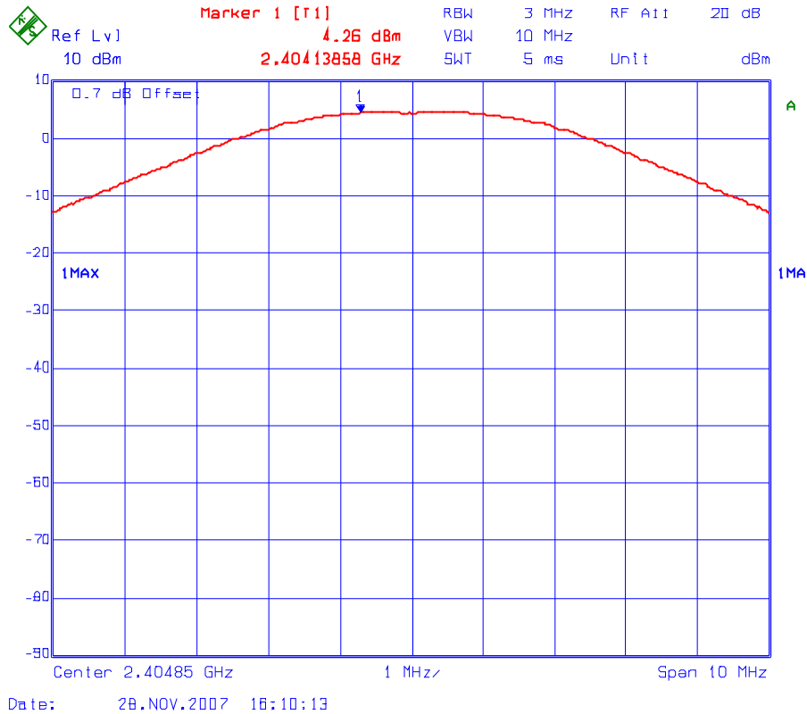
Plot 6.7.5.1 Peak Conducted Output Power Frequency: 2405 MHz
