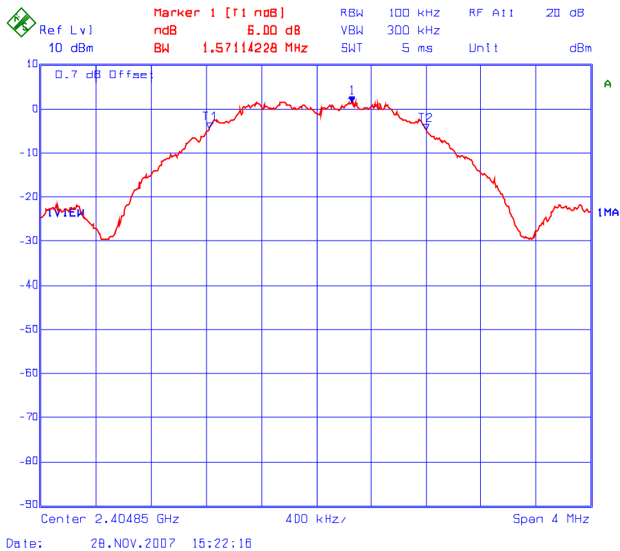
Plot 6.6.5.1 6 dB Bandwidth Frequency: 2405 MHz
