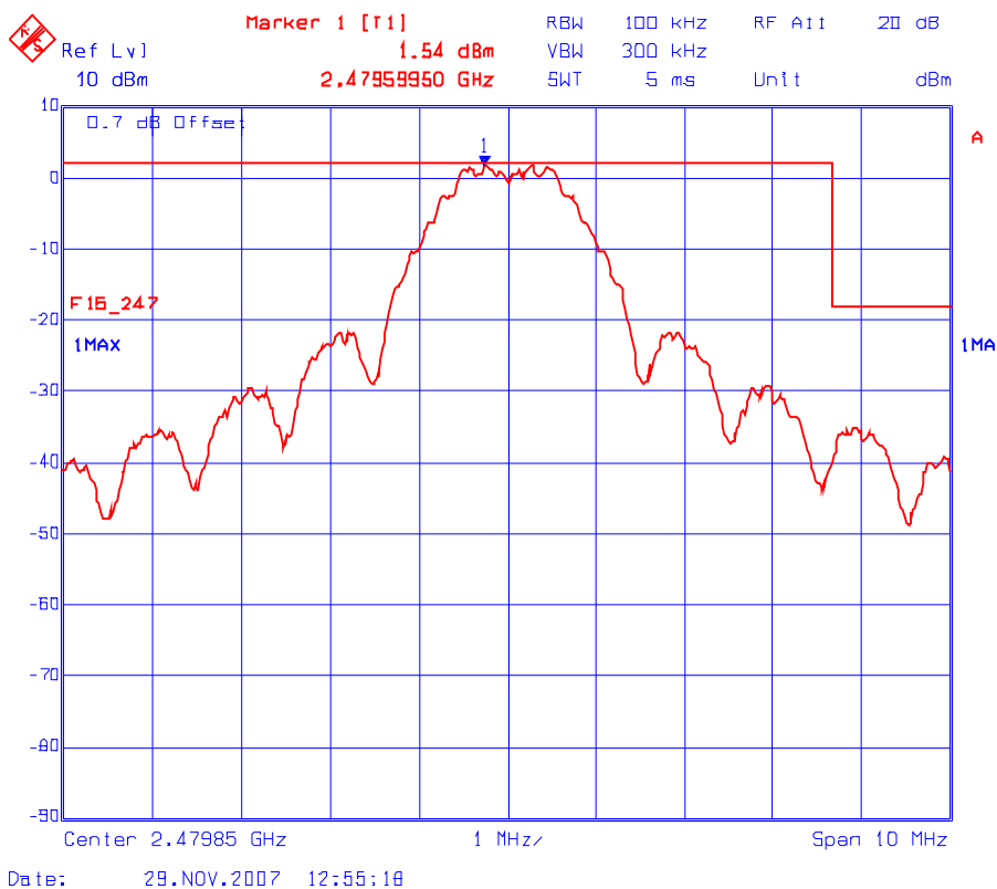
Plot 6.8.5.1.2 Band-Edge RF Conducted Emissions High End of Frequency Band
