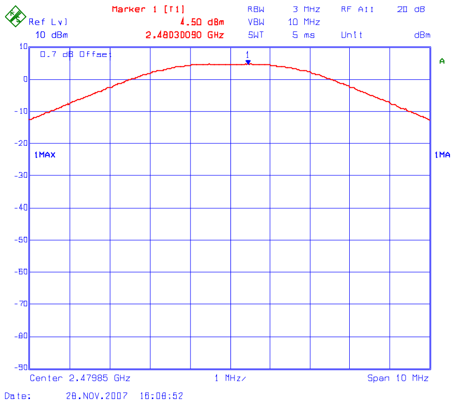
Plot 6.7.5.3 Peak Conducted Output Power Frequency: 2480 MHz
