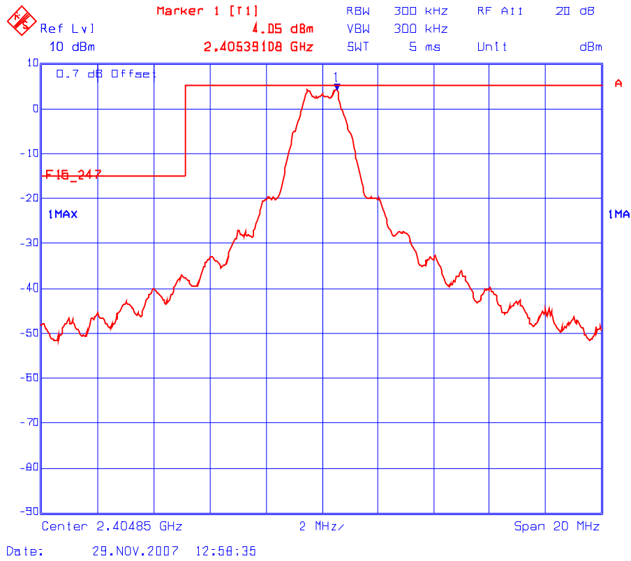
Plot 6.8.5.1.1 Band-Edge RF Conducted Emissions Low End of Frequency Band
