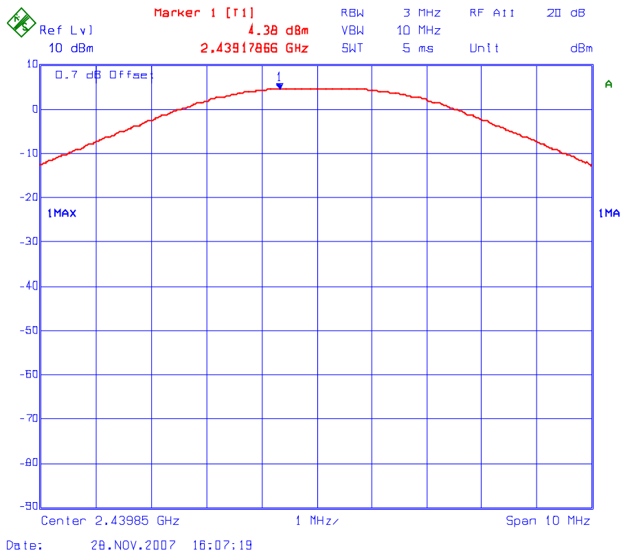
Plot 6.7.5.2 Peak Conducted Output Power Frequency: 2440 MHz
