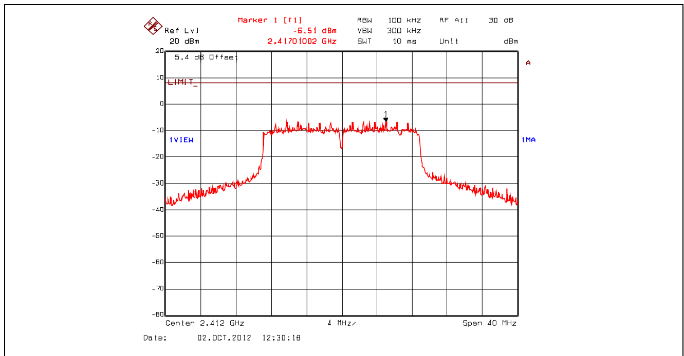
Plot 5.6.4.31. Power Spectral Density, 802.11n 800ns, 65 Mbps 64-QAM 5/6, 2412 MHz, Setting 23 Offset: Insertion Loss + BWCF = 20.63 dB + 10*log(3 kHz/ 100 kHz) = 5.43 dB
