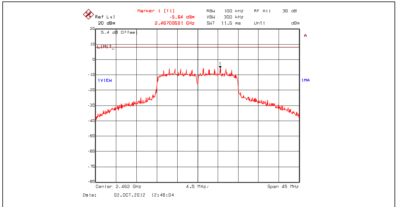
Plot 5.6.4.36. Power Spectral Density, 802.11n 400ns, 7.2 Mbps BPSK1/2, 2462 MHz, Setting 23 Offset: Insertion Loss + BWCF = 20.63 dB + 10 \cdot \log(3 \text{ kHz} / 100 \text{ kHz}) = 5.43 dB
