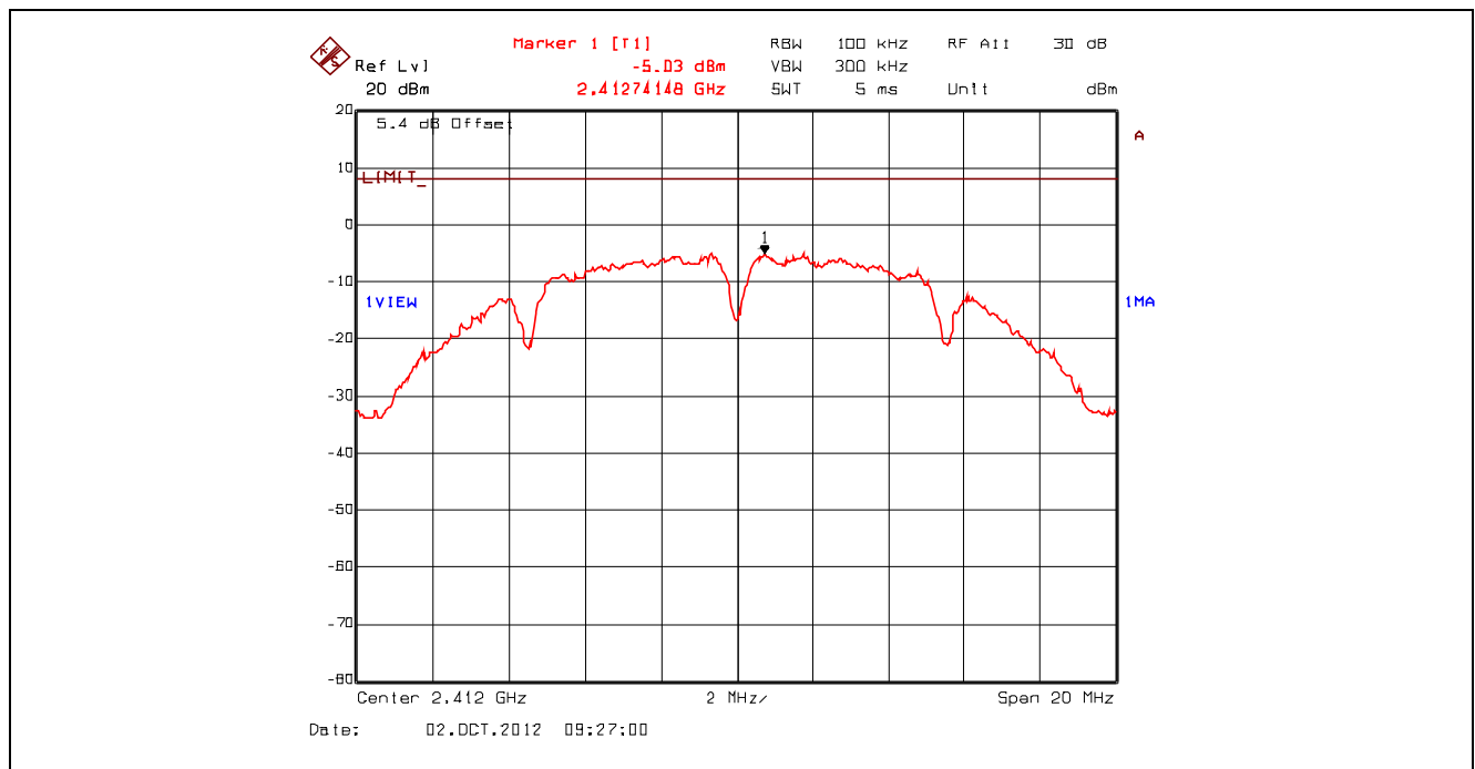
Plot 5.6.4.4. Power Spectral Density, 802.11b, 2 Mbps DQPSK, 2412 MHz, Setting 23 Offset: Insertion Loss + BWCF = 20.63 dB + 10 \cdot \log(3 \text{ kHz} / 100 \text{ kHz}) = 5.43 dB
