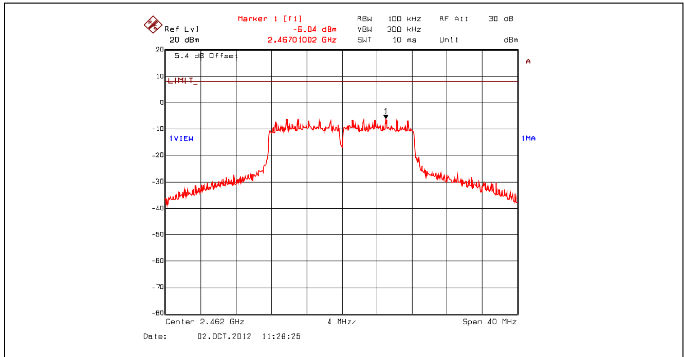
Plot 5.6.4.18. Power Spectral Density, 802.11g, 36 Mbps 16-QAM, 2462 MHz, Setting 23 Offset: Insertion Loss + BWCF = 20.63 dB + 10 \cdot \log(3 \text{ kHz} / 100 \text{ kHz}) = 5.43 dB
