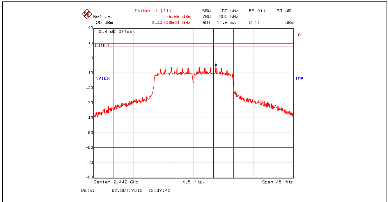
Plot 5.6.4.26. Power Spectral Density, 802.11n 800ns, 19.5 Mbps QPSK 3/4, 2442 MHz, Setting 23 Offset: Insertion Loss + BWCF = 20.63 dB + 10 \cdot \log(3 \text{ kHz} / 100 \text{ kHz}) = 5.43 \text{ dB}
