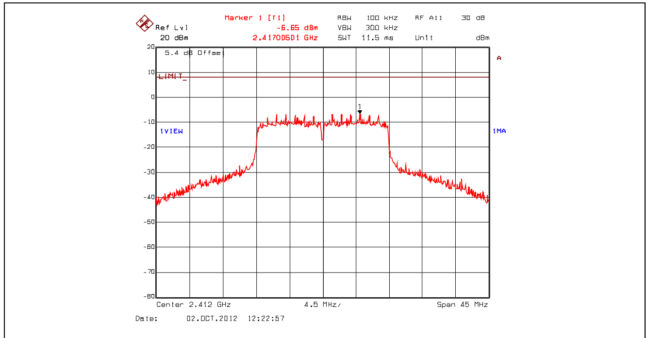
Plot 5.6.4.28. Power Spectral Density, 802.11n 800ns, 39 Mbps 16-QAM 3/4, 2412 MHz, Setting 23 Offset: Insertion Loss + BWCF = 20.63 dB + 10*log(3 kHz/ 100 kHz) = 5.43 dB
