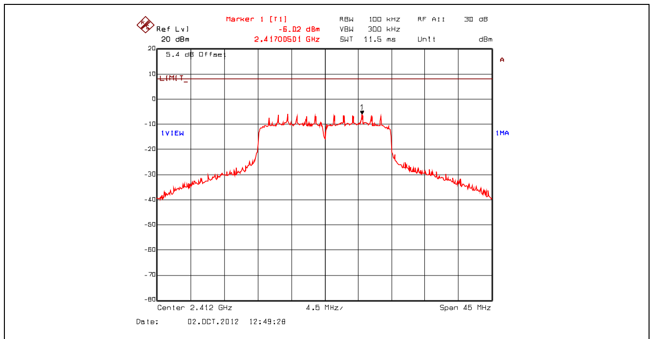
Plot 5.6.4.37. Power Spectral Density, 802.11n 400ns, 21.7 Mbps QPSK 3/4, 2412 MHz, Setting 23 Offset: Insertion Loss + BWCF = 20.63 dB + 10 \cdot \log(3 \text{ kHz} / 100 \text{ kHz}) = 5.43 dB
