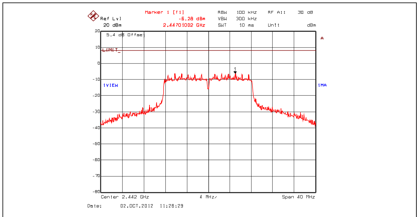
Plot 5.6.4.17. Power Spectral Density, 802.11g, 36 Mbps 16-QAM, 2442 MHz, Setting 23 Offset: Insertion Loss + BWCF = 20.63 dB + 10 \cdot \log(3 \text{ kHz} / 100 \text{ kHz}) = 5.43 \text{ dB}
