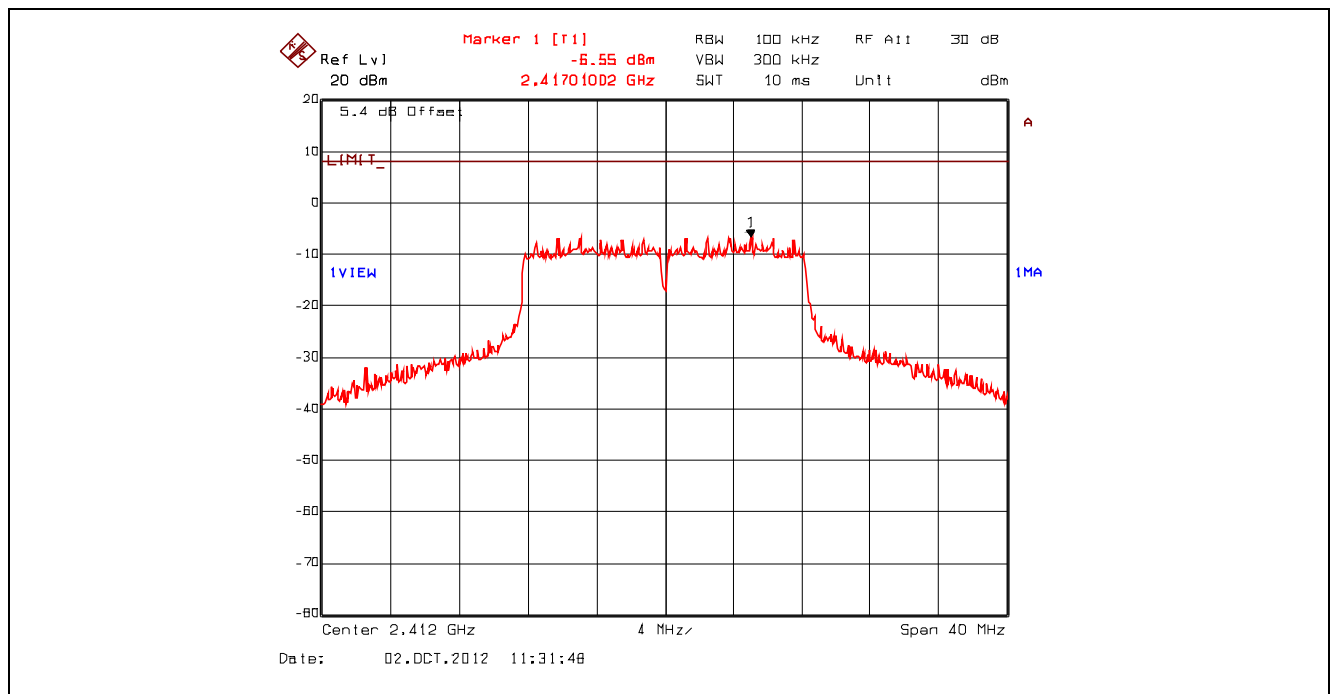
Plot 5.6.4.19. Power Spectral Density, 802.11g, 54 Mbps 64-QAM, 2412 MHz, Setting 23 Offset: Insertion Loss + BWCF = 20.63 dB + 10 \cdot \log(3 \text{ kHz} / 100 \text{ kHz}) = 5.43 dB
