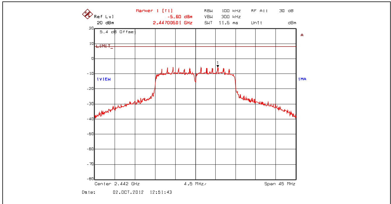
Plot 5.6.4.38. Power Spectral Density, 802.11n 400ns, 21.7 Mbps QPSK 3/4, 2442 MHz, Setting 23 Offset: Insertion Loss + BWCF = 20.63 dB + 10*log(3 kHz/ 100 kHz) = 5.43 dB
