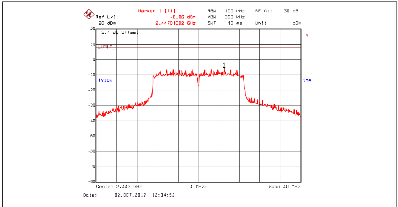
Plot 5.6.4.32. Power Spectral Density, 802.11n 800ns, 65 Mbps 64-QAM 5/6, 2442 MHz, Setting 23 Offset: Insertion Loss + BWCF = 20.63 dB + 10 \cdot \log(3 \text{ kHz} / 100 \text{ kHz}) = 5.43 \text{ dB}
