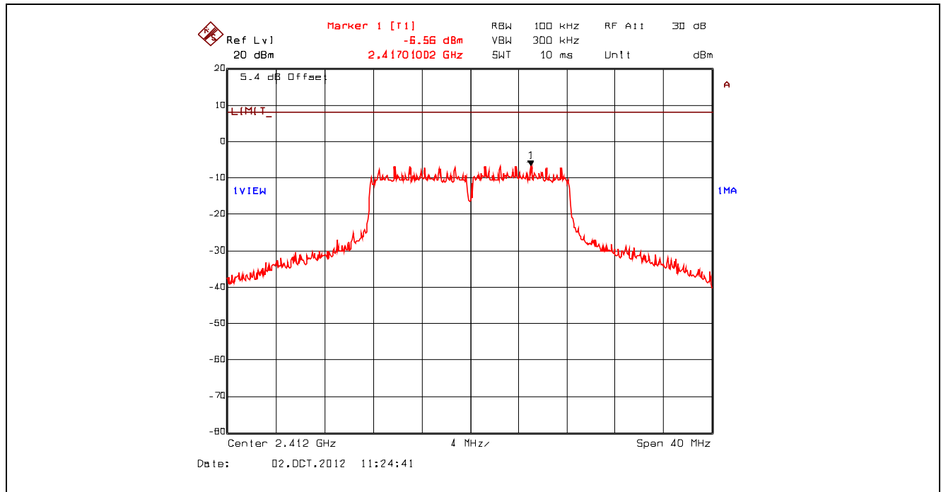
Plot 5.6.4.16. Power Spectral Density, 802.11g, 36 Mbps 16-QAM, 2412 MHz, Setting 23 Offset: Insertion Loss + BWCF = 20.63 dB + 10 \cdot \log(3 \text{ kHz} / 100 \text{ kHz}) = 5.43 \text{ dB}
