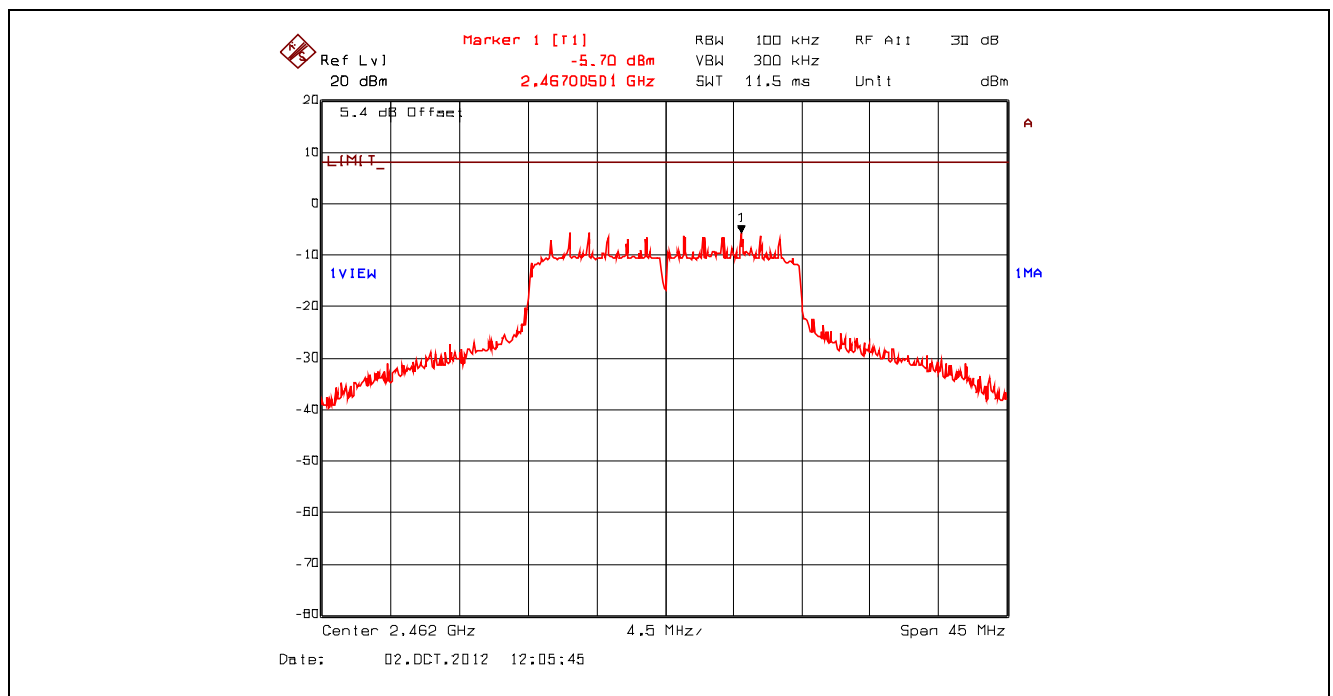
Plot 5.6.4.27. Power Spectral Density, 802.11n 800ns, 19.5 Mbps QPSK 3/4, 2462 MHz, Setting 23 Offset: Insertion Loss + BWCF = 20.63 dB + 10 \cdot \log(3 \text{ kHz} / 100 \text{ kHz}) = 5.43 \text{ dB}
