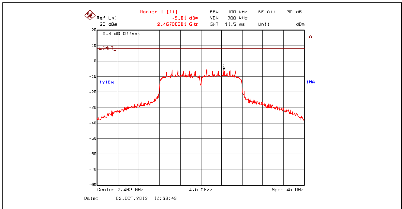
Plot 5.6.4.39. Power Spectral Density, 802.11n 400ns, 21.7 Mbps QPSK 3/4, 2462 MHz, Setting 23 Offset: Insertion Loss + BWCF = 20.63 dB + 10*log(3 kHz/ 100 kHz) = 5.43 dB
