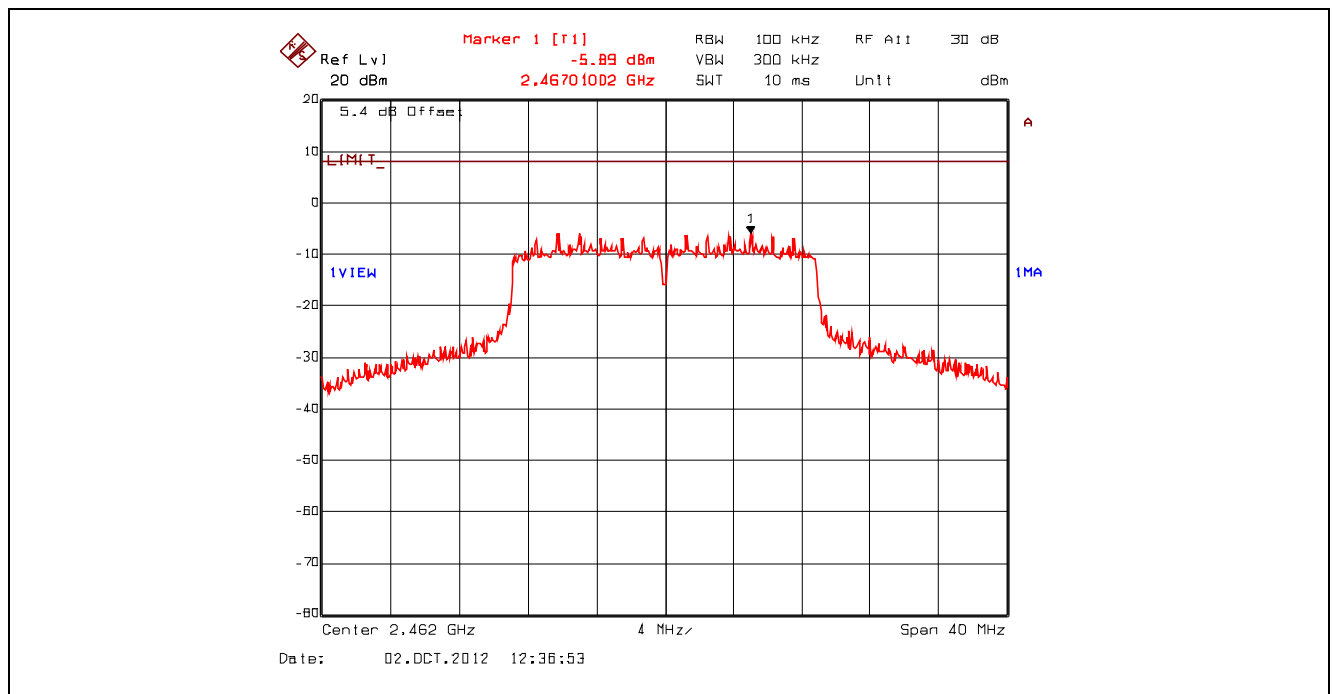
Plot 5.6.4.33. Power Spectral Density, 802.11n 800ns, 65 Mbps 64-QAM 5/6, 2462 MHz, Setting 23 Offset: Insertion Loss + BWCF = 20.63 dB + 10 \cdot \log(3 \text{ kHz} / 100 \text{ kHz}) = 5.43 \text{ dB}
