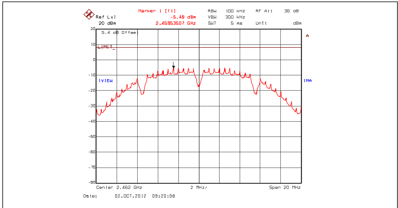
Plot 5.6.4.3. Power Spectral Density, 802.11b, 1 Mbps DBPSK, 2462 MHz, Setting 23 Offset: Insertion Loss + BWCF = 20.63 dB + 10 \cdot \log(3 \text{ kHz} / 100 \text{ kHz}) = 5.43 dB
