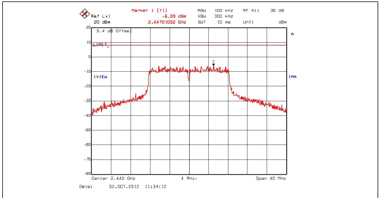
Plot 5.6.4.20. Power Spectral Density, 802.11g, 54 Mbps 64-QAM, 2442 MHz, Setting 23 Offset: Insertion Loss + BWCF = 20.63 dB + 10 \cdot \log(3 \text{ kHz} / 100 \text{ kHz}) = 5.43 \text{ dB}
