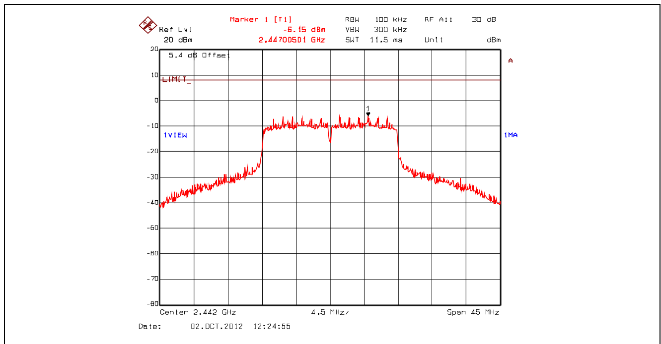
Plot 5.6.4.29. Power Spectral Density, 802.11n 800ns, 39 Mbps 16-QAM 3/4, 2442 MHz, Setting 23 Offset: Insertion Loss + BWCF = 20.63 dB + 10*log(3 kHz/ 100 kHz) = 5.43 dB
