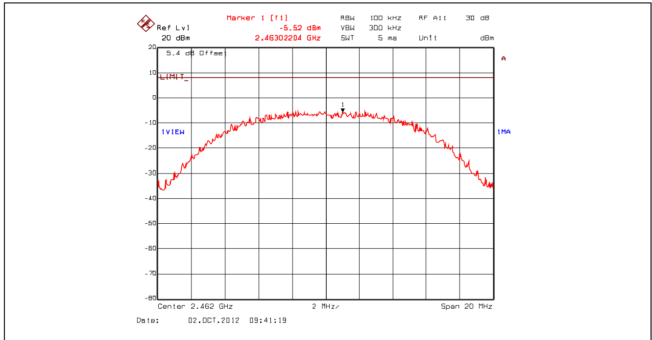
Plot 5.6.4.9. Power Spectral Density, 802.11b, 11 Mbps CCK, 2462 MHz, Setting 23 Offset: Insertion Loss + BWCF = 20.63 dB + 10 \cdot \log(3 \text{ kHz} / 100 \text{ kHz}) = 5.43 dB
