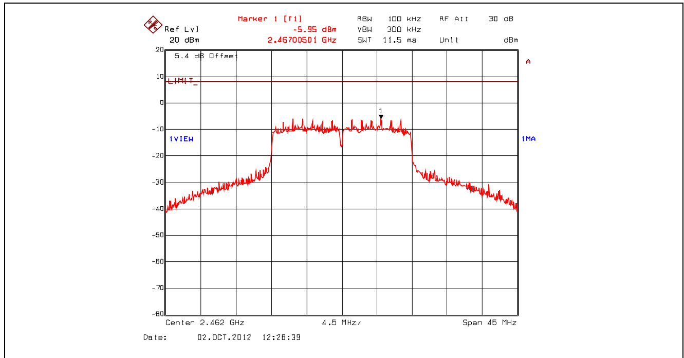
Plot 5.6.4.30. Power Spectral Density, 802.11n 800ns, 39 Mbps 16-QAM 3/4, 2462 MHz, Setting 23 Offset: Insertion Loss + BWCF = 20.63 dB + 10*log(3 kHz/ 100 kHz) = 5.43 dB
