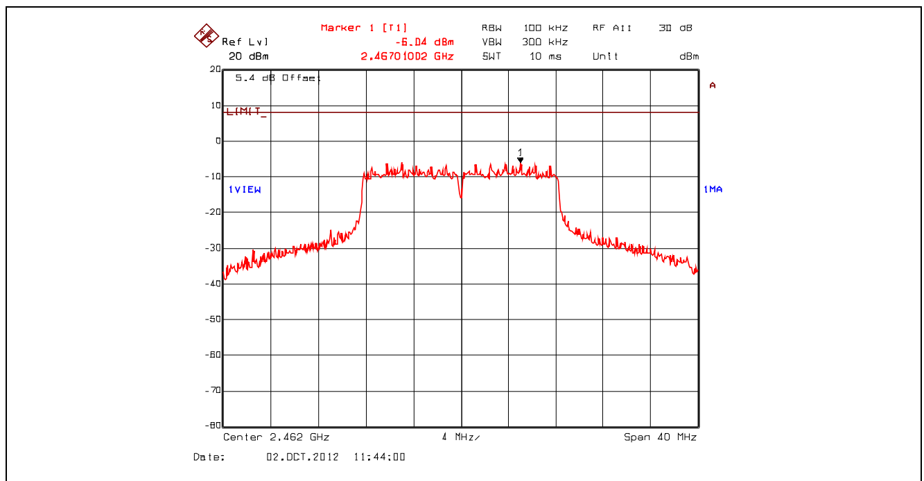
Plot 5.6.4.21. Power Spectral Density, 802.11g, 54 Mbps 64-QAM, 2462 MHz, Setting 23 Offset: Insertion Loss + BWCF = 20.63 dB + 10 \cdot \log(3 \text{ kHz} / 100 \text{ kHz}) = 5.43 \text{ dB}
