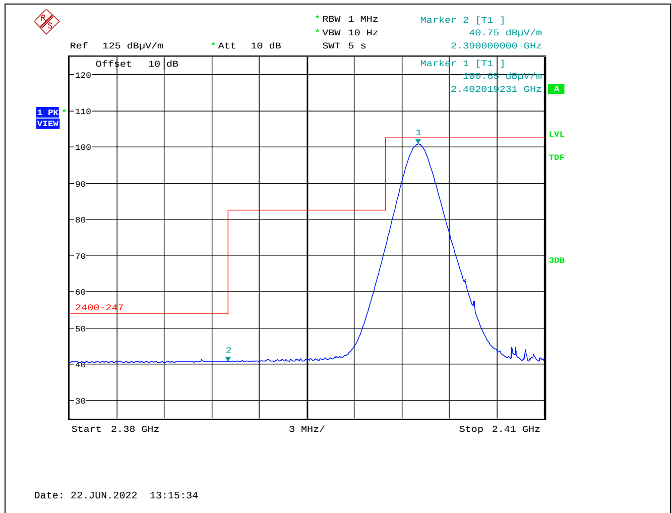
Plot 5.2.3.1.2.2. Band-Edge RF Radiated Emissions at 3 m, Vertical Polarization, Average Low End of Frequency Band, 2402 MHz, 8 dBm Power Setting, 1 Mbps
