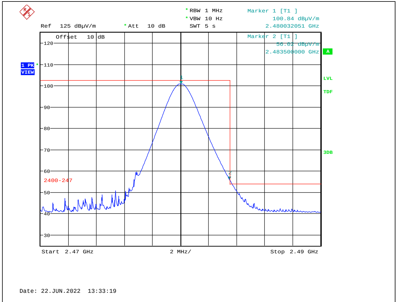
Plot 5.2.3.1.2.6. Band-Edge RF Radiated Emissions at 3 m, Vertical Polarization, Average High End of Frequency Band, 2480 MHz, 8 dBm Power Setting, 1 Mbps Marker 2: 56.02 dBμV/m – 35.94 dB Duty Cycle Factor = 20.08 dBμV/m (Limit 54 dBμV/m)
