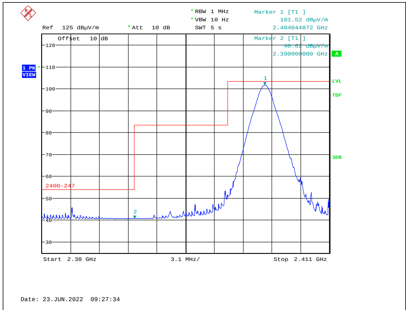
Plot 5.2.3.2.2.4. Band-Edge RF Radiated Emissions at 3 m, Horizontal Polarization, Average Low End of Frequency Band, 2404 MHz, 8 dBm Power Setting, 2 Mbps
