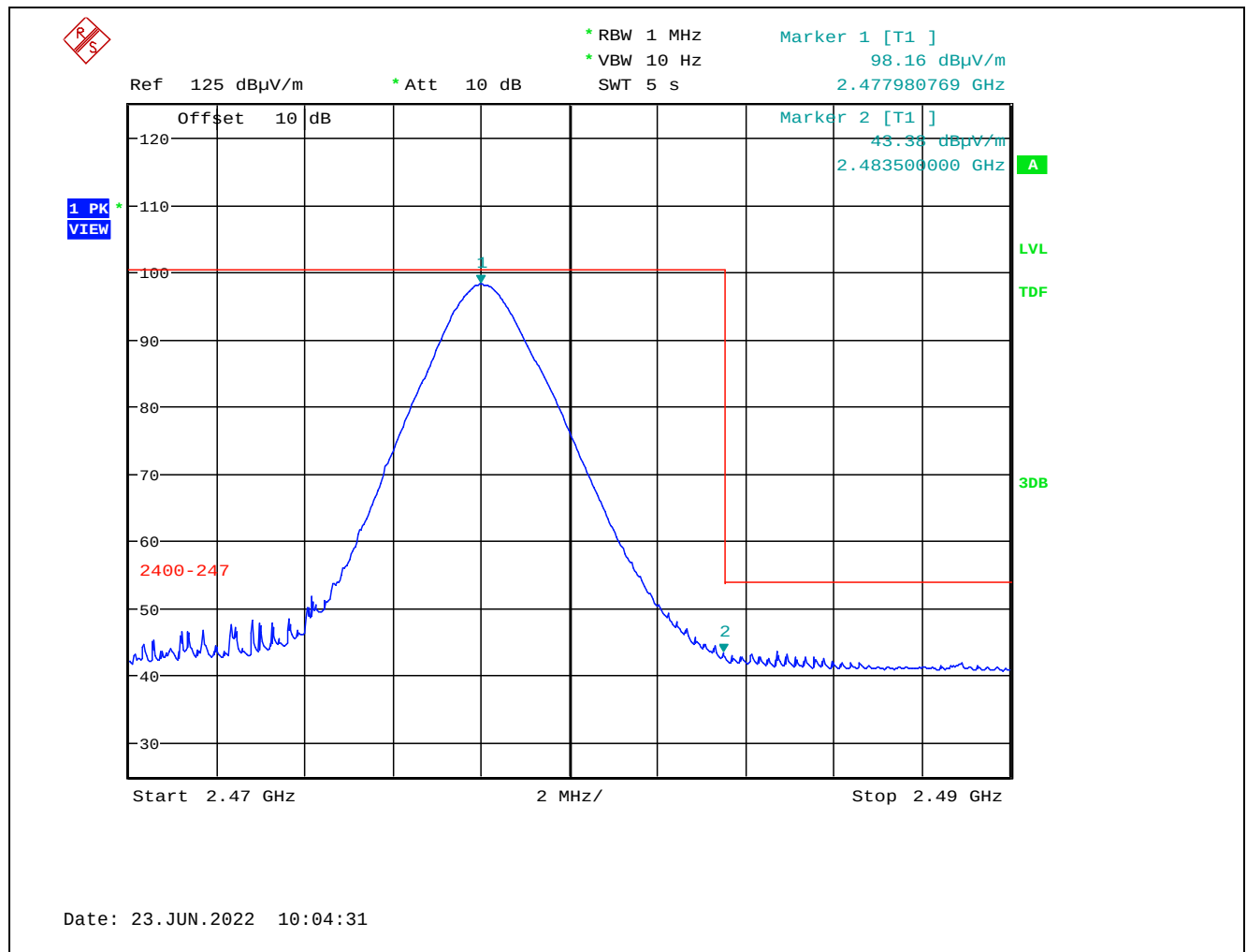
Plot 5.2.3.2.2.6. Band-Edge RF Radiated Emissions at 3 m, Vertical Polarization, Average High End of Frequency Band, 2478 MHz, 8 dBm Power Setting, 2 Mbps
