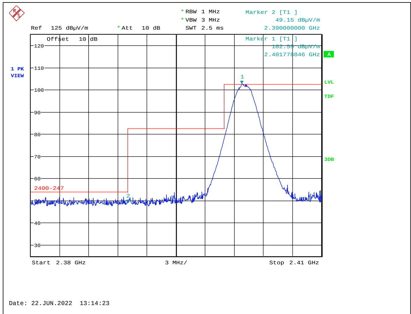
Plot 5.2.3.1.2.1. Band-Edge RF Radiated Emissions at 3 m, Vertical Polarization, Peak Low End of Frequency Band, 2402 MHz, 8 dBm Power Setting, 1 Mbps
