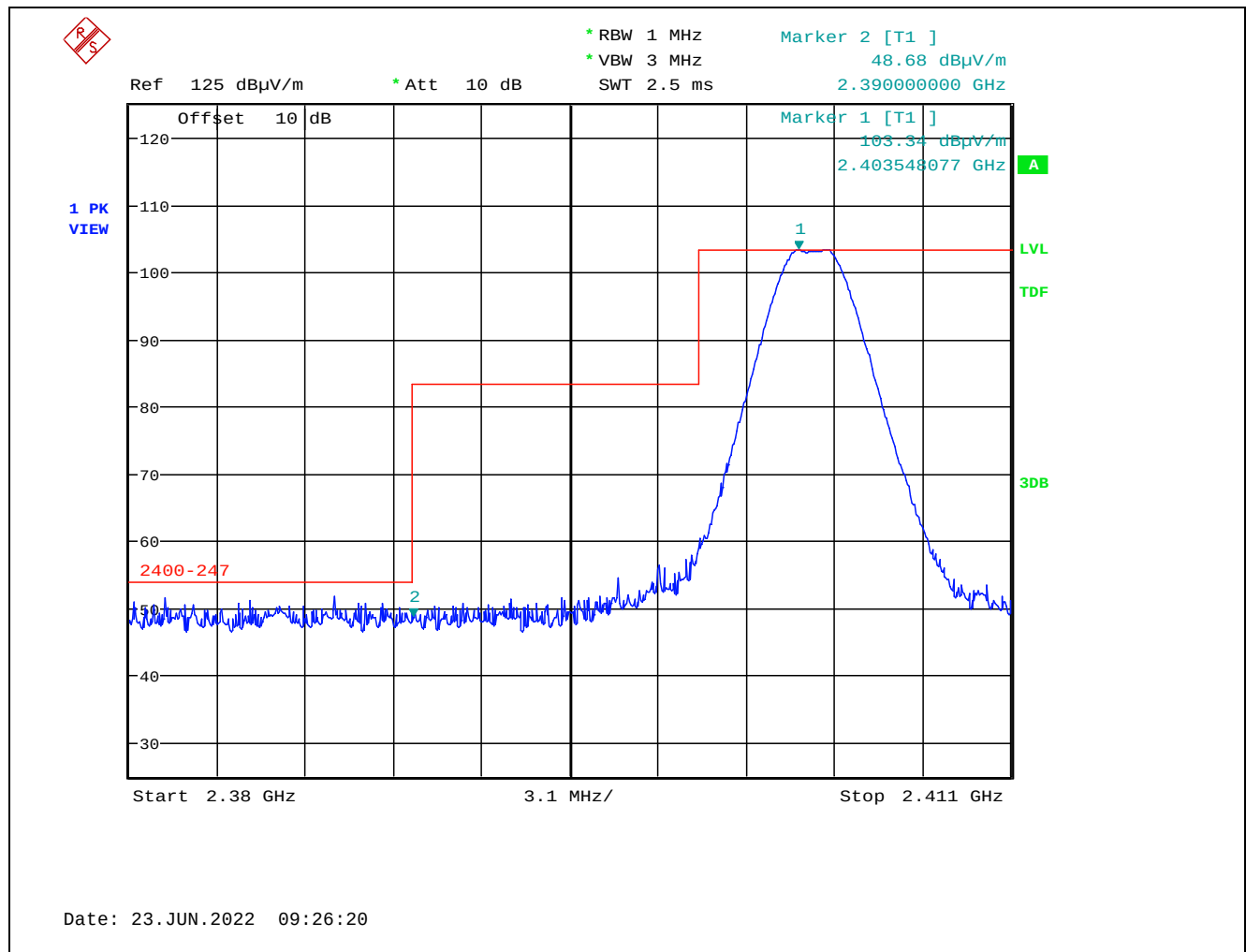
Plot 5.2.3.2.3. Band-Edge RF Radiated Emissions at 3 m, Horizontal Polarization, Peak Low End of Frequency Band, 2404 MHz, 8 dBm Power Setting, 2 Mbps
