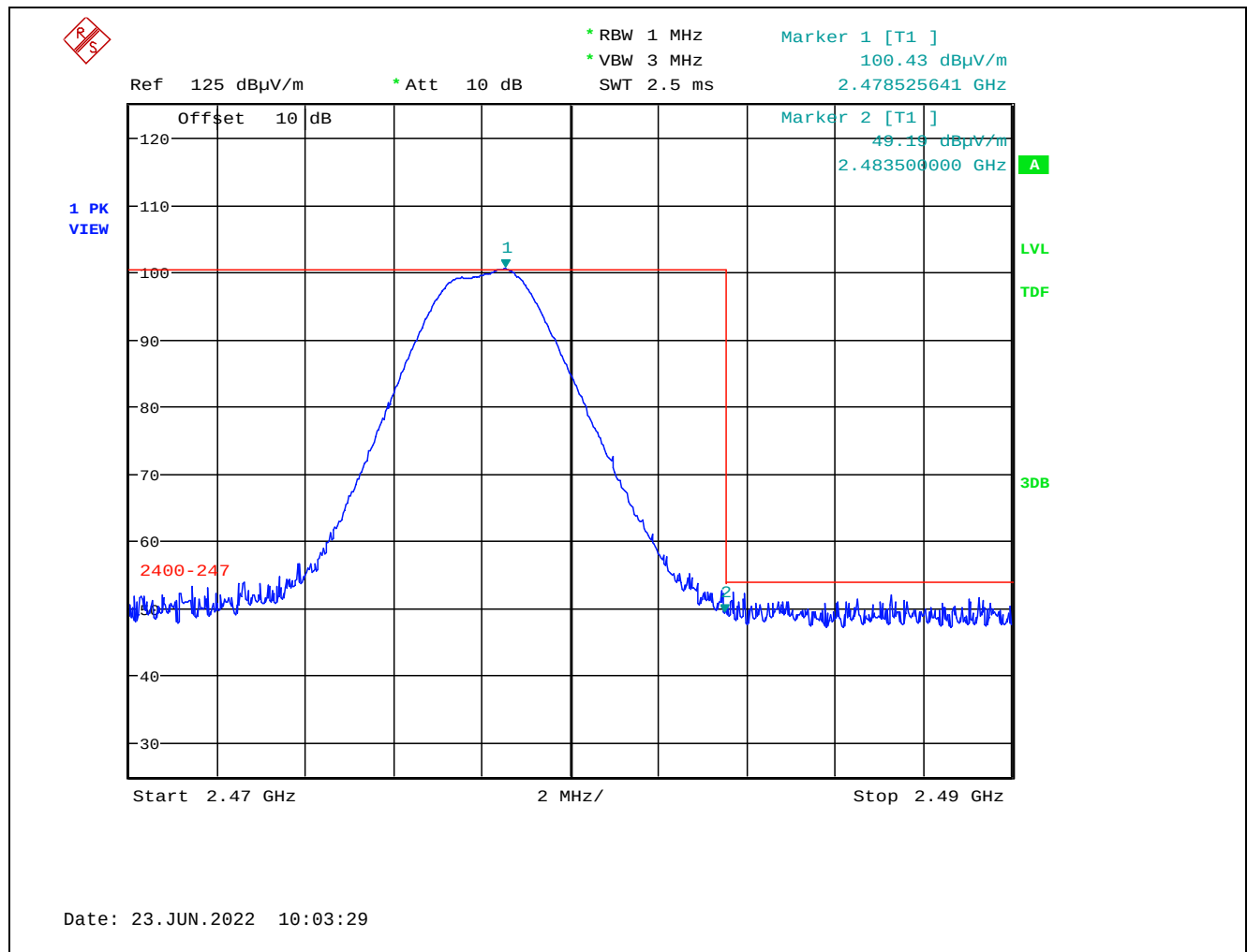
Plot 5.2.3.2.2.5. Band-Edge RF Radiated Emissions at 3 m, Vertical Polarization, Peak High End of Frequency Band, 2478 MHz, 8 dBm Power Setting, 2 Mbps
