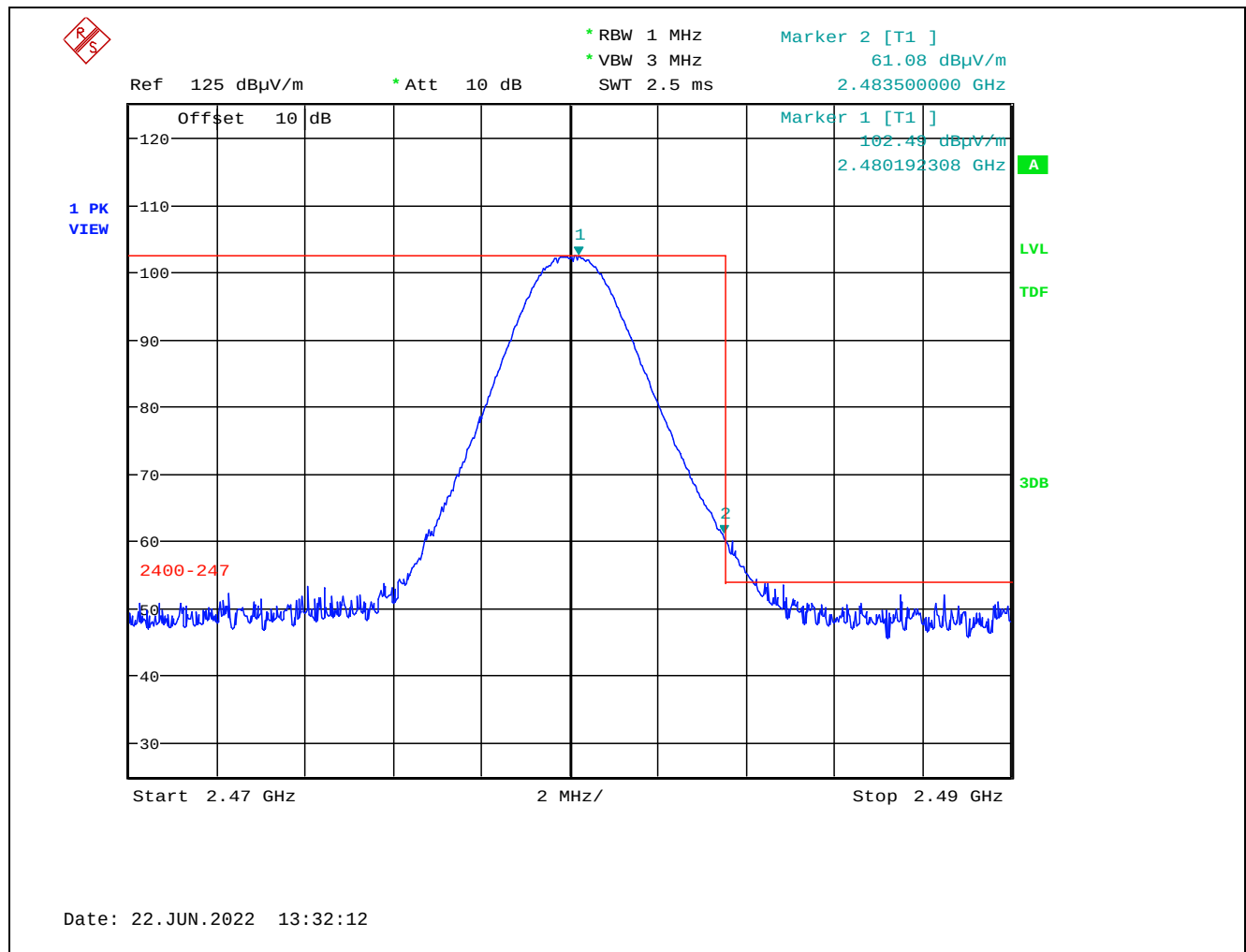
Plot 5.2.3.1.2.5. Band-Edge RF Radiated Emissions at 3 m, Vertical Polarization, Peak High End of Frequency Band, 2480 MHz, 8 dBm Power Setting, 1 Mbps
