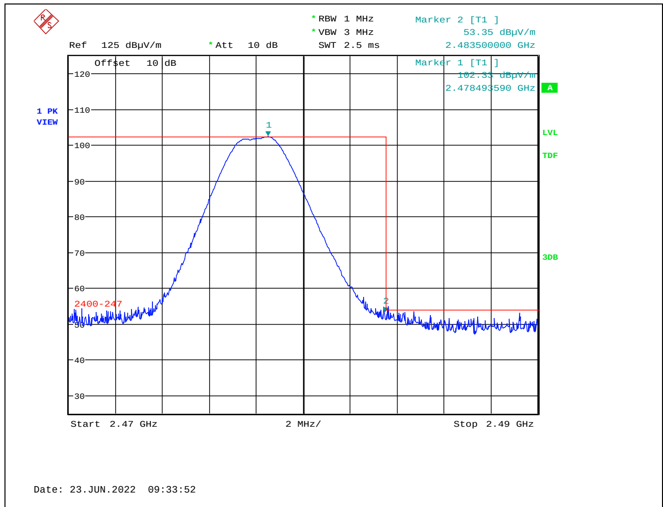
Plot 5.2.3.2.7. Band-Edge RF Radiated Emissions at 3 m, Horizontal Polarization, Peak High End of Frequency Band, 2478 MHz, 8 dBm Power Setting, 2 Mbps
