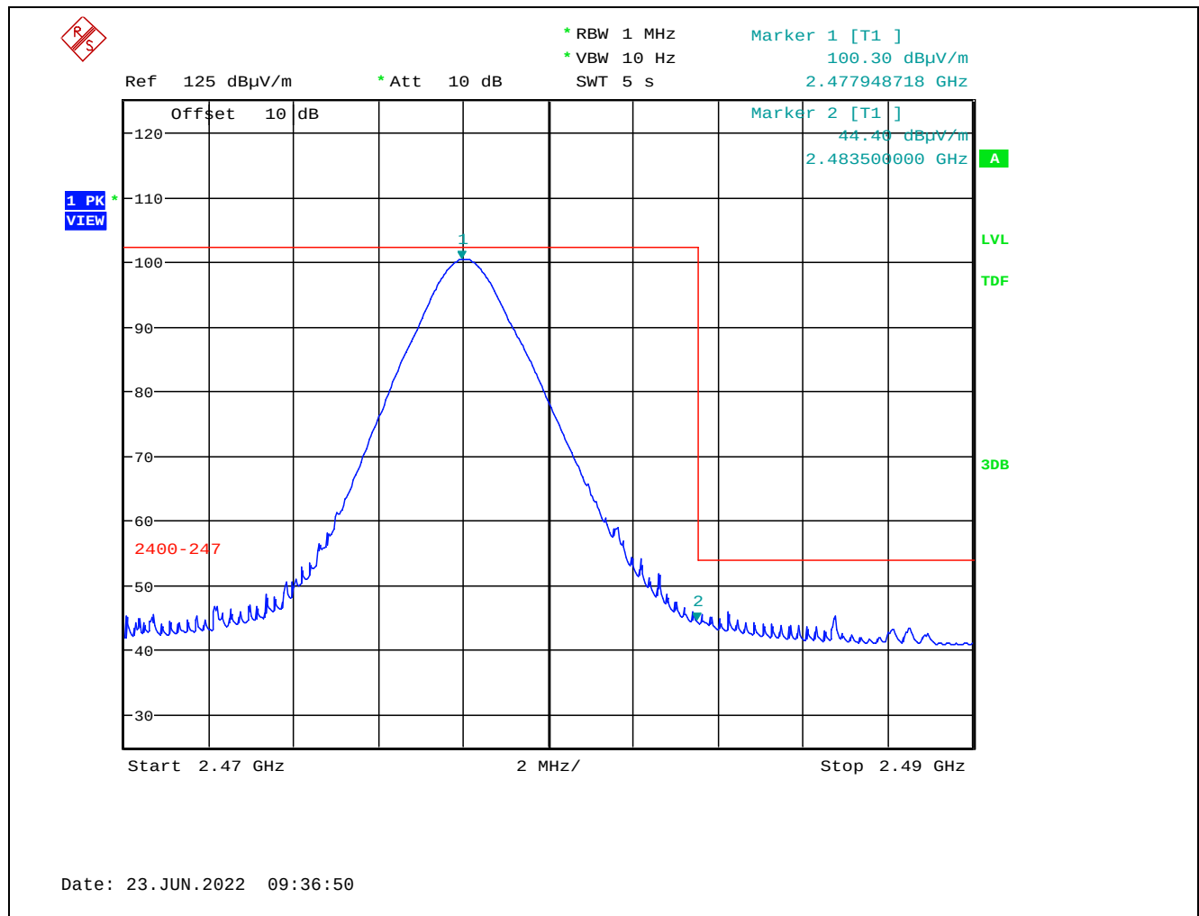
Plot 5.2.3.2.2.8. Band-Edge RF Radiated Emissions at 3 m, Horizontal Polarization, Average High End of Frequency Band, 2478 MHz, 8 dBm Power Setting, 2 Mbps
