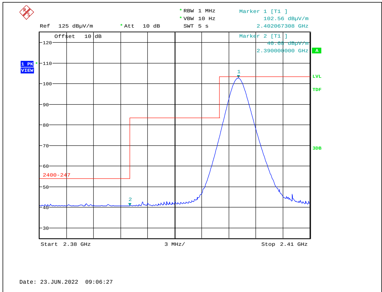
Plot 5.2.3.1.2.4. Band-Edge RF Radiated Emissions at 3 m, Horizontal Polarization, Average Low End of Frequency Band, 2402 MHz, 8 dBm Power Setting, 1 Mbps
