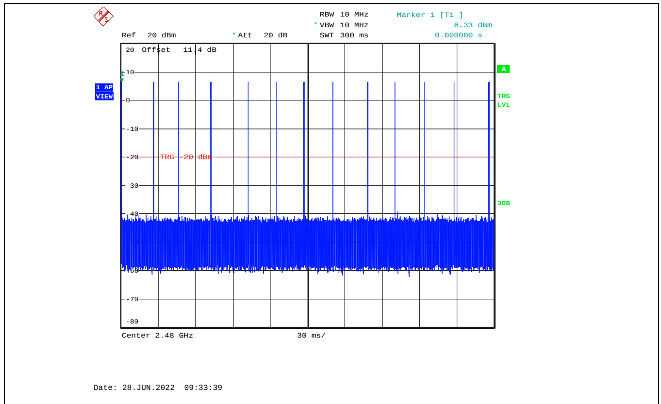
Plot 5.3.3.1.1. Duty Cycle (Pulse Train)
