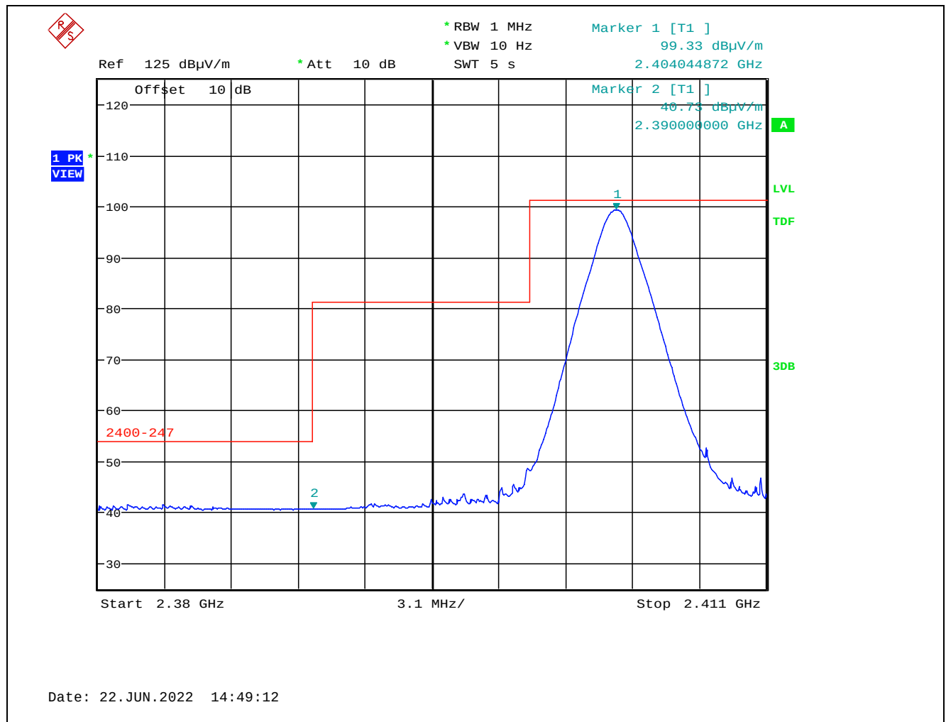
Plot 5.2.3.2.2.2. Band-Edge RF Radiated Emissions at 3 m, Vertical Polarization, Average Low End of Frequency Band, 2404 MHz, 8 dBm Power Setting, 2 Mbps
