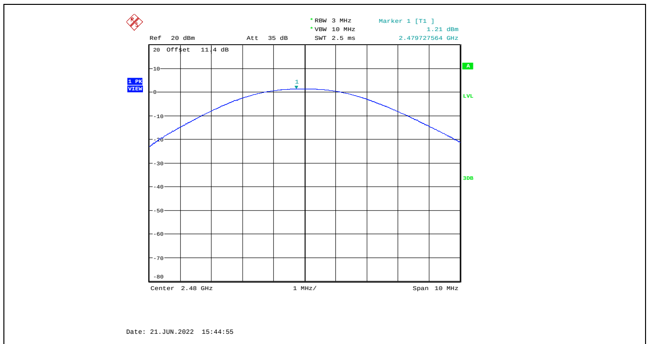
Plot 5.1.3.6. Maximum Peak Conducted Output Power, GFSK Modulation, 1 Mbps, -2 dBm Power Setting, 2480 MHz
