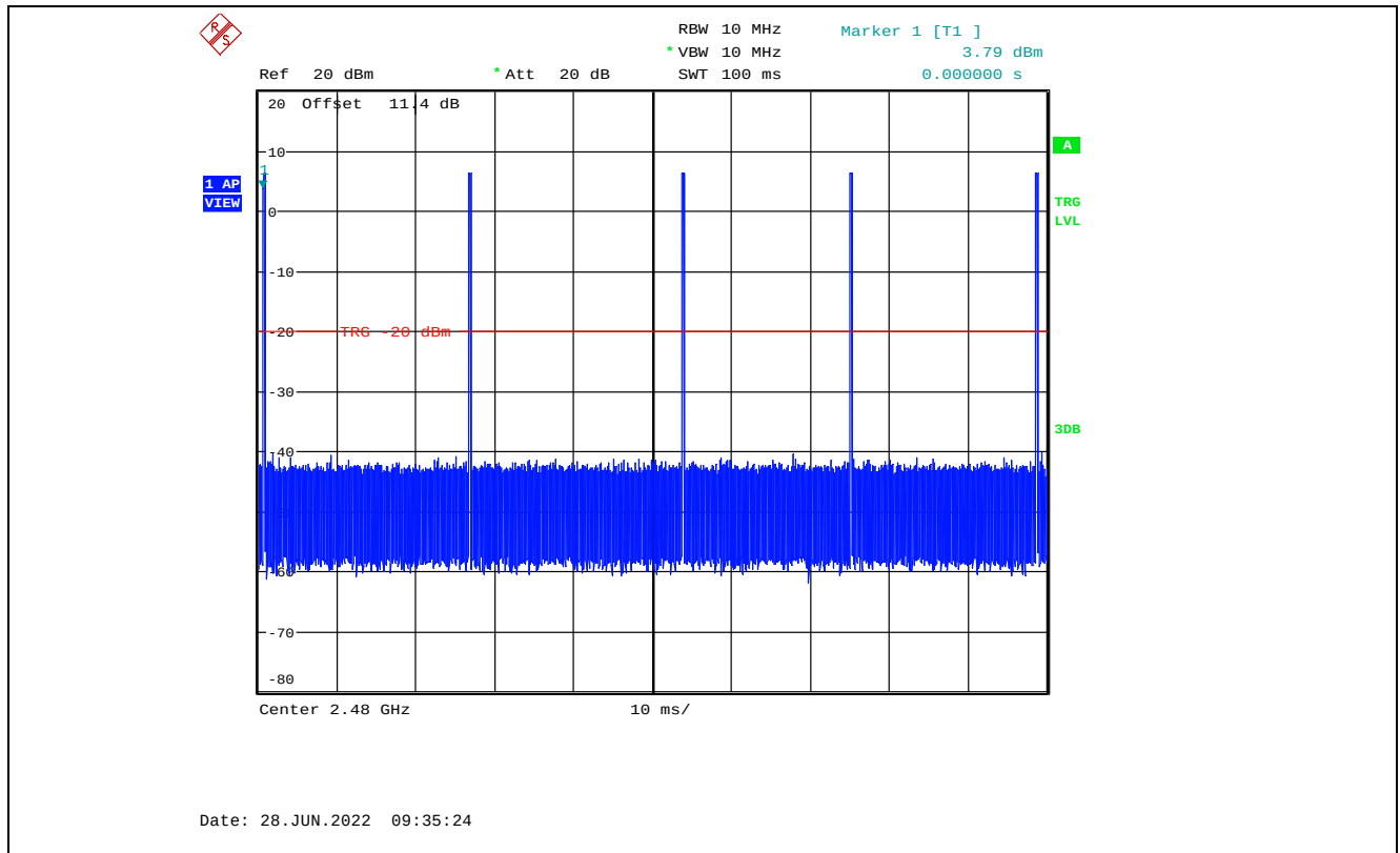
Plot 5.3.3.1.2. Duty Cycle (5 Pulses in 100 ms)
