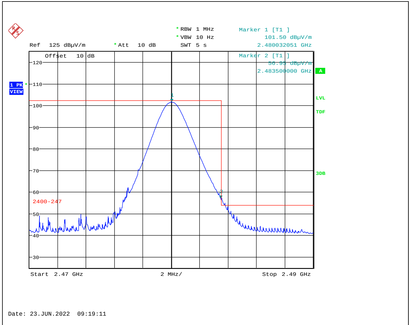
Plot 5.2.3.1.2.8. Band-Edge RF Radiated Emissions at 3 m, Horizontal Polarization, Average High End of Frequency Band, 2480 MHz, 8 dBm Power Setting, 1 Mbps Marker 2: 56.95 dBμV/m – 35.94 dB Duty Cycle Factor = 21.01 dBμV/m (Limit 54 dBμV/m)
