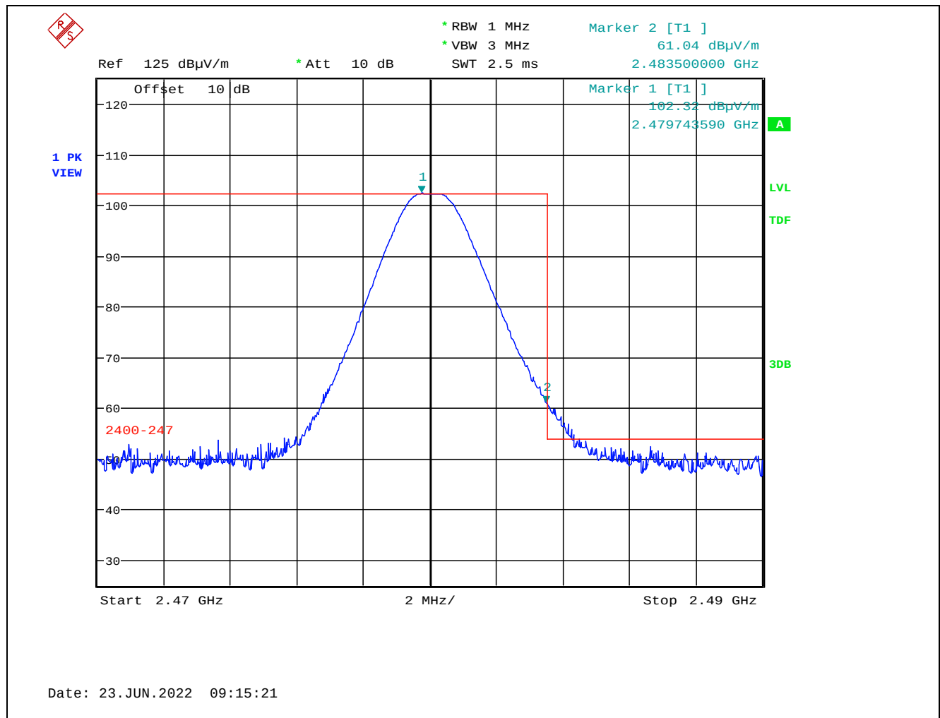
Plot 5.2.3.1.2.7. Band-Edge RF Radiated Emissions at 3 m, Horizontal Polarization, Peak High End of Frequency Band, 2480 MHz, 8 dBm Power Setting, 1 Mbps
