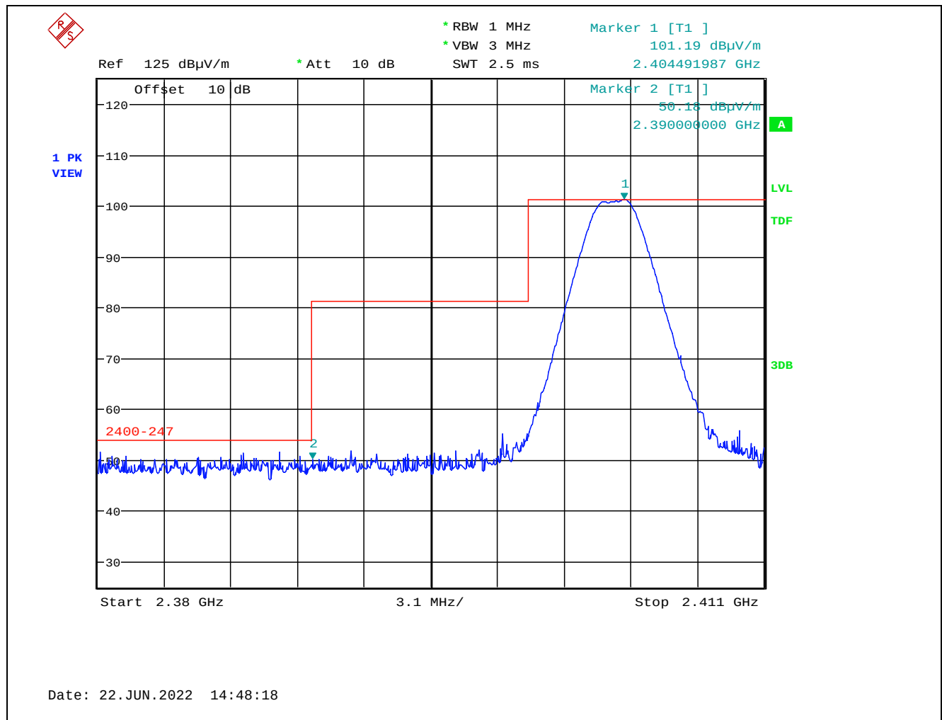
Plot 5.2.3.2.2.1. Band-Edge RF Radiated Emissions at 3 m, Vertical Polarization, Peak Low End of Frequency Band, 2404 MHz, 8 dBm Power Setting, 2 Mbps
