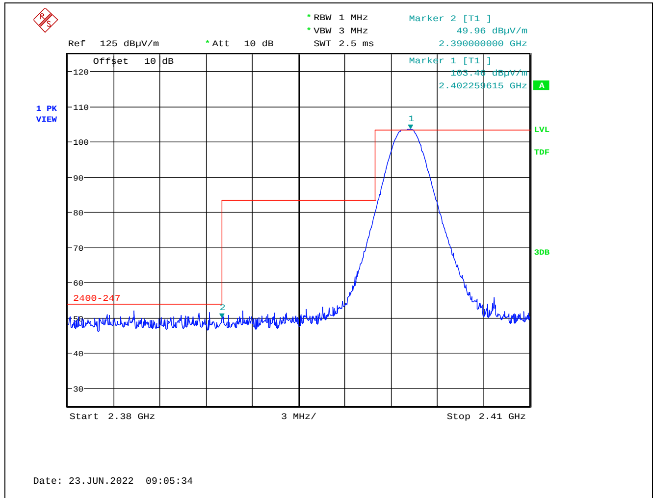
Plot 5.2.3.1.2.3. Band-Edge RF Radiated Emissions at 3 m, Horizontal Polarization, Peak Low End of Frequency Band, 2402 MHz, 8 dBm Power Setting, 1 Mbps
