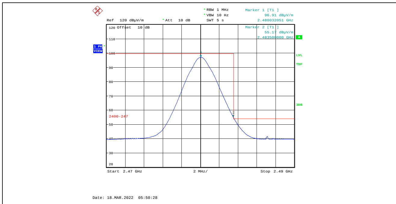
Plot 5.4.4.1.2.12. Band-Edge RF Radiated Emissions at 3 m, Horizontal Polarization, Average High End of Frequency Band, 2480 MHz, 3 dBm Power Setting Marker 2: 55.17 dBμV/m – 3.61 dB Duty Cycle Factor = 51.56 dBμV/m (Limit 54 dBμV/m)
