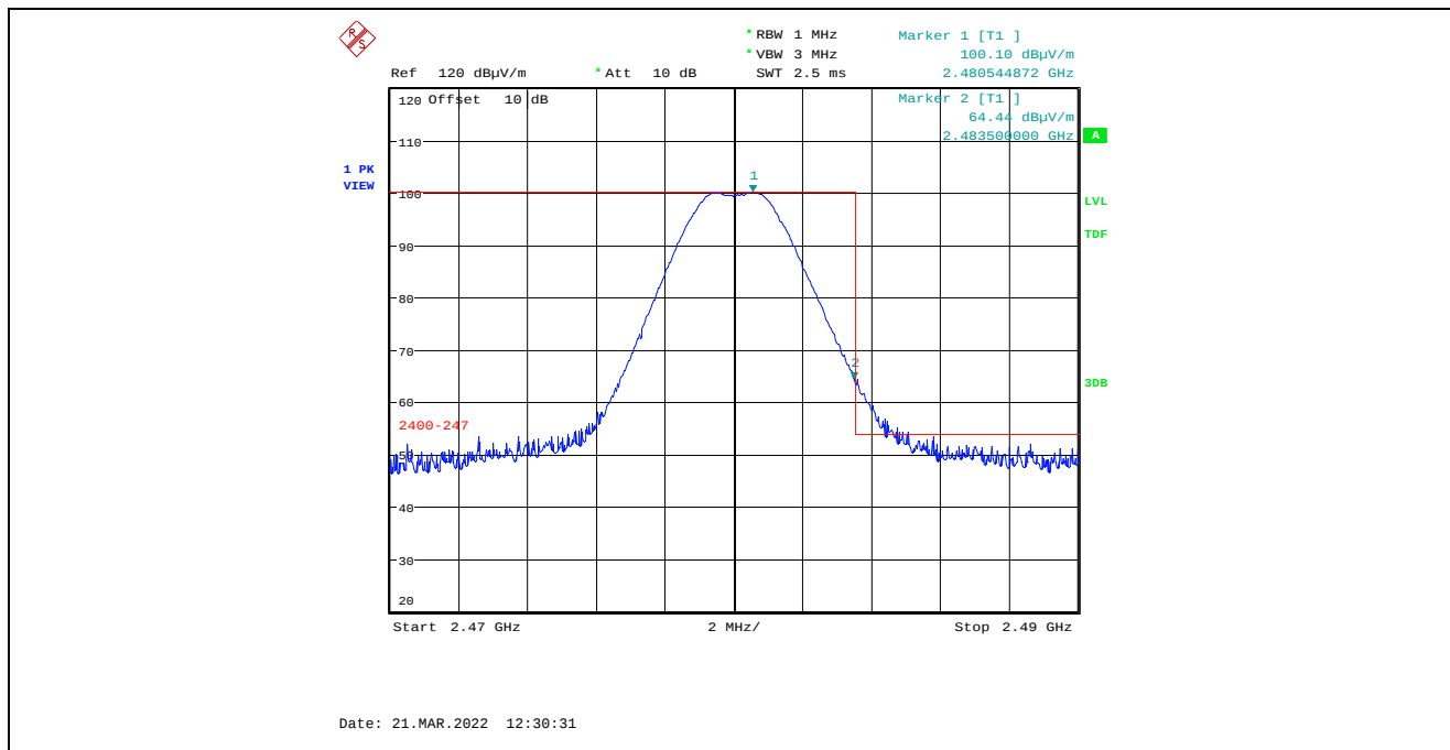
Plot 5.4.4.4.2.11. Band-Edge RF Radiated Emissions at 3 m, Horizontal Polarization, Peak High End of Frequency Band, 2480 MHz, 3 dBm Power Setting
