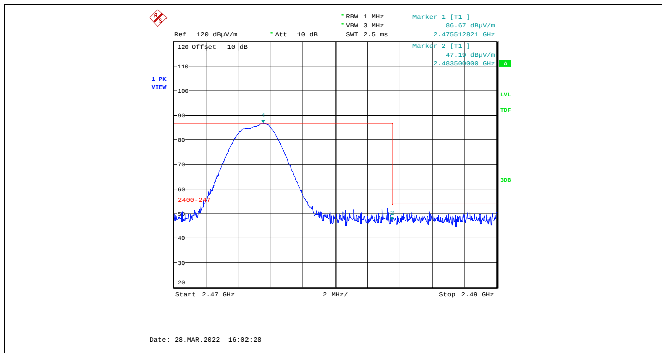
Plot 5.4.4.3.2.7. Band-Edge RF Radiated Emissions at 3 m, Horizontal Polarization, Peak High End of Frequency Band, 2475 MHz, 7 dBm Power Setting
