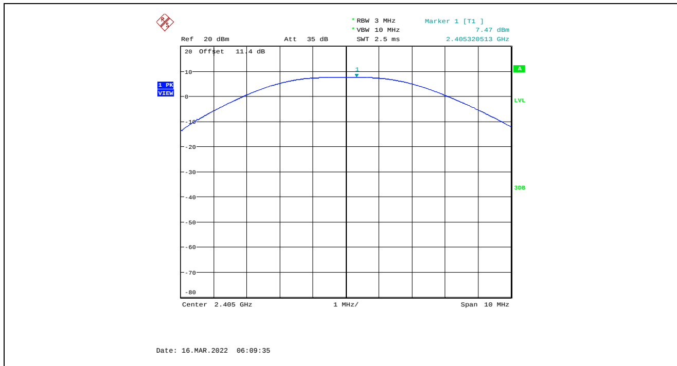
Plot 5.3.4.1. Maximum Peak Conducted Output Power, QPSK Modulation, 7 dBm Power Setting, 2405 MHz
