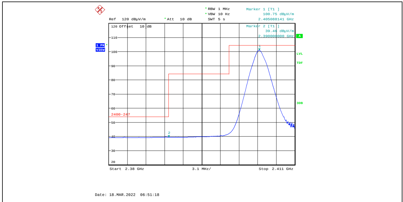
Plot 5.4.4.1.2.2. Band-Edge RF Radiated Emissions at 3 m, Vertical Polarization, Average Low End of Frequency Band, 2405 MHz, 7 dBm Power Setting
