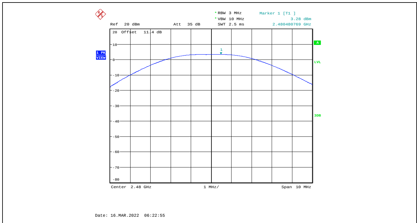
Plot 5.3.4.4. Maximum Peak Conducted Output Power, QPSK Modulation, 3 dBm Power Setting, 2480 MHz
