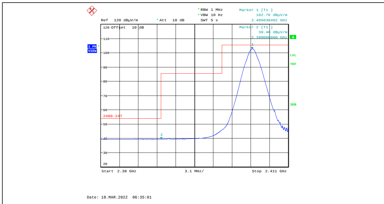
Plot 5.4.4.1.2.4. Band-Edge RF Radiated Emissions at 3 m, Horizontal Polarization, Average Low End of Frequency Band, 2405 MHz, 7 dBm Power Setting
