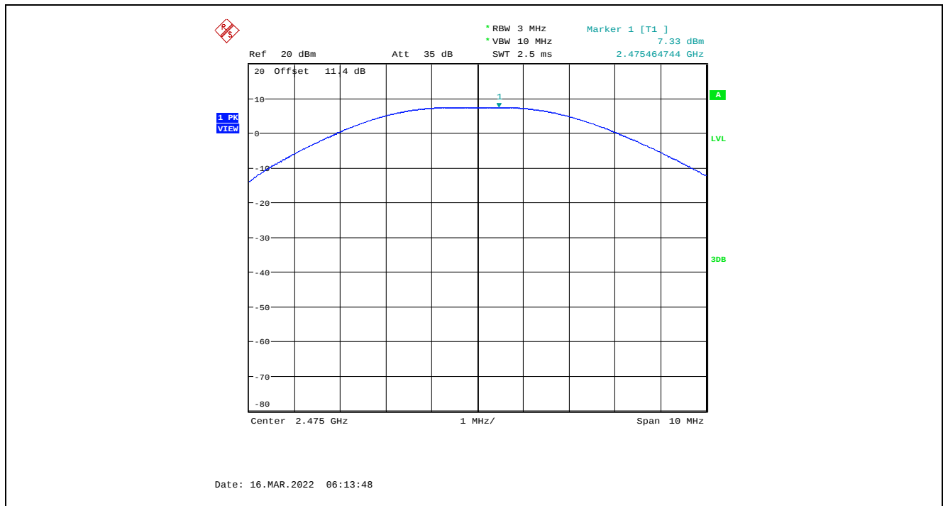
Plot 5.3.4.3. Maximum Peak Conducted Output Power, QPSK Modulation, 7 dBm Power Setting, 2475 MHz
