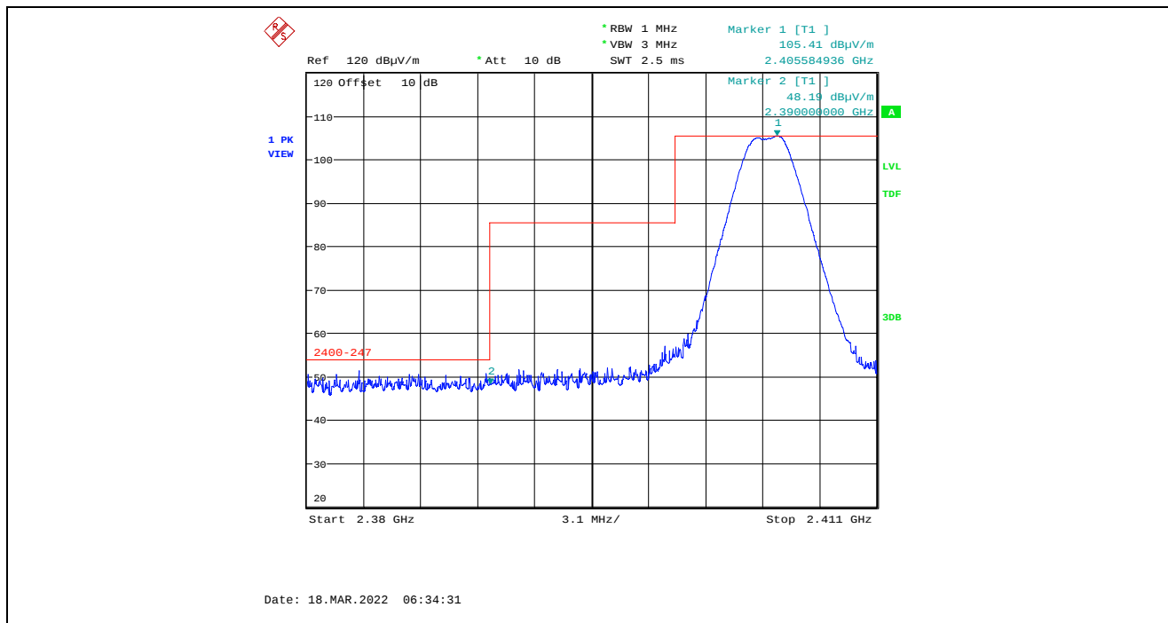
Plot 5.4.4.1.2.3. Band-Edge RF Radiated Emissions at 3 m, Horizontal Polarization, Peak Low End of Frequency Band, 2405 MHz, 7 dBm Power Setting
