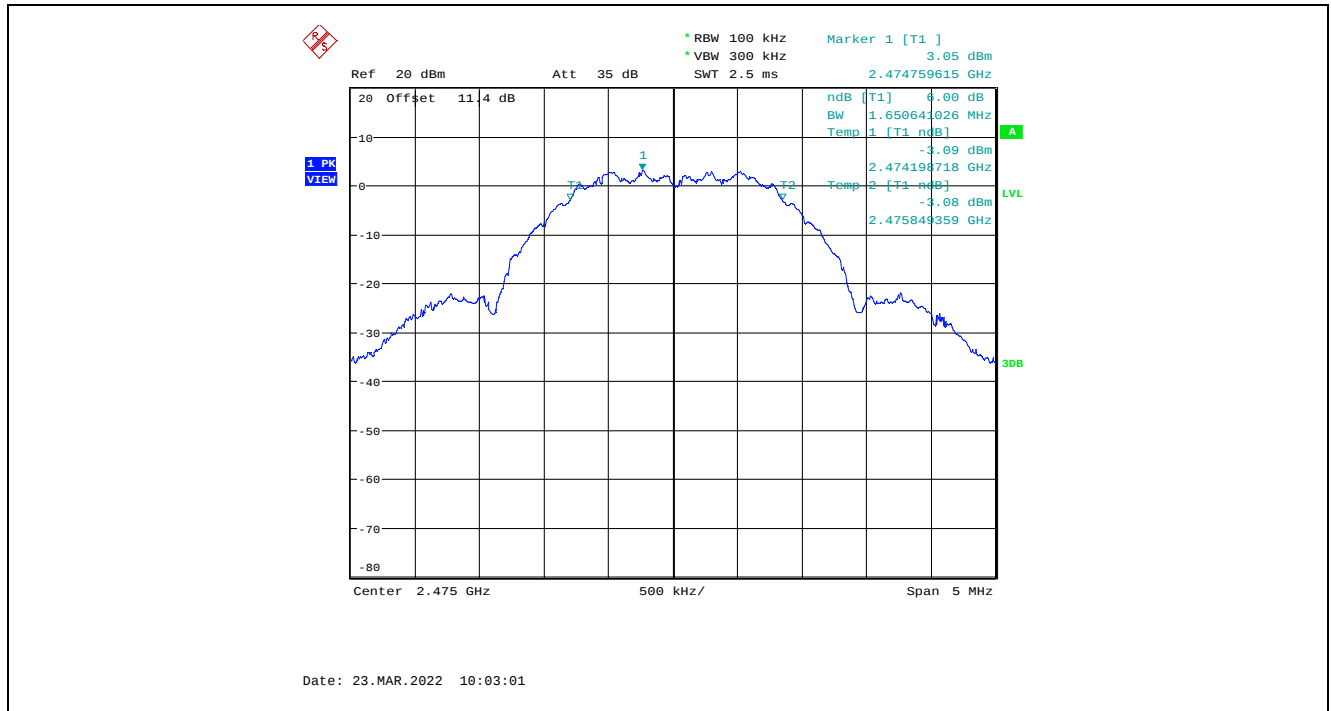
Plot 5.2.4.3. 6 dB Bandwidth, QPSK Modulation, 7 dBm Power Setting, 2475 MHz
