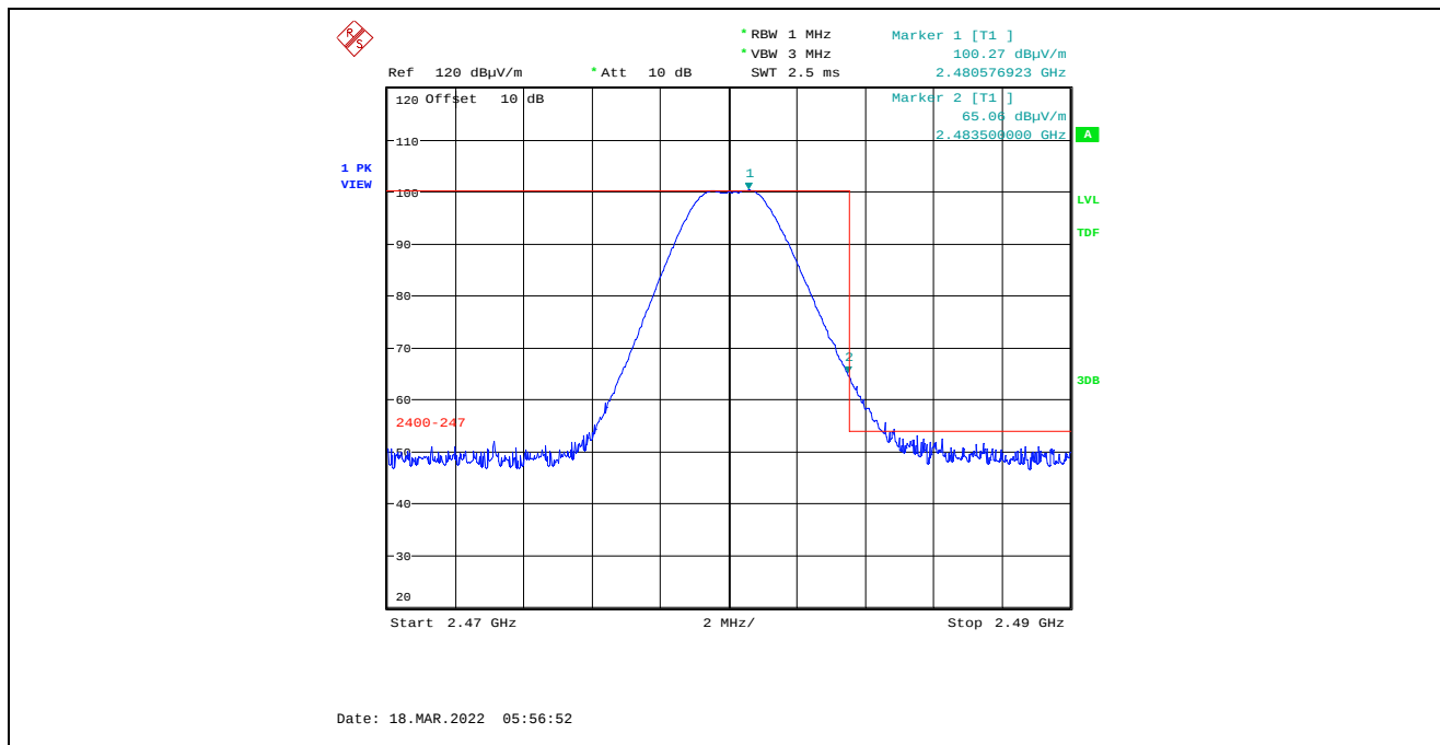
Plot 5.4.4.1.2.9. Band-Edge RF Radiated Emissions at 3 m, Vertical Polarization, Peak High End of Frequency Band, 2480 MHz, 3 dBm Power Setting
