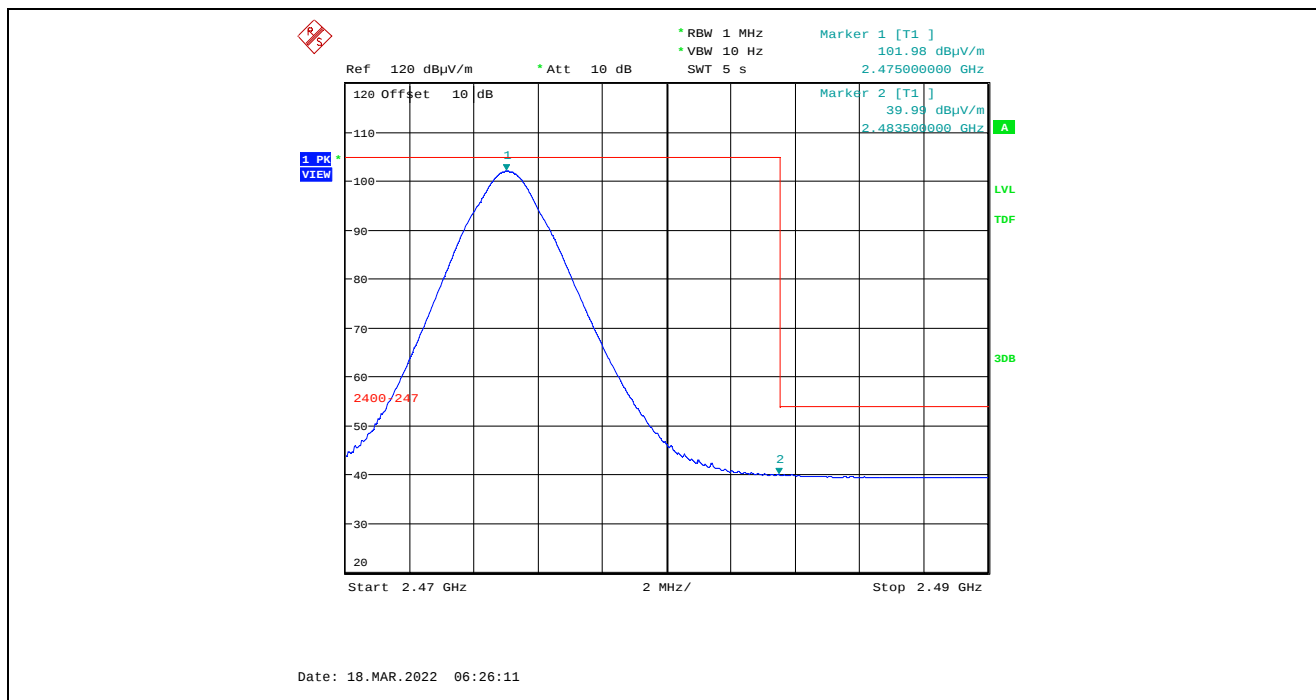
Plot 5.4.4.1.2.8. Band-Edge RF Radiated Emissions at 3 m, Horizontal Polarization, Average High End of Frequency Band, 2475 MHz, 7 dBm Power Setting
