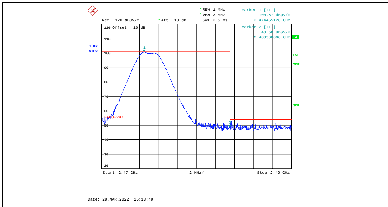
Plot 5.4.4.3.2.5. Band-Edge RF Radiated Emissions at 3 m, Vertical Polarization, Peak High End of Frequency Band, 2475 MHz, 7 dBm Power Setting
