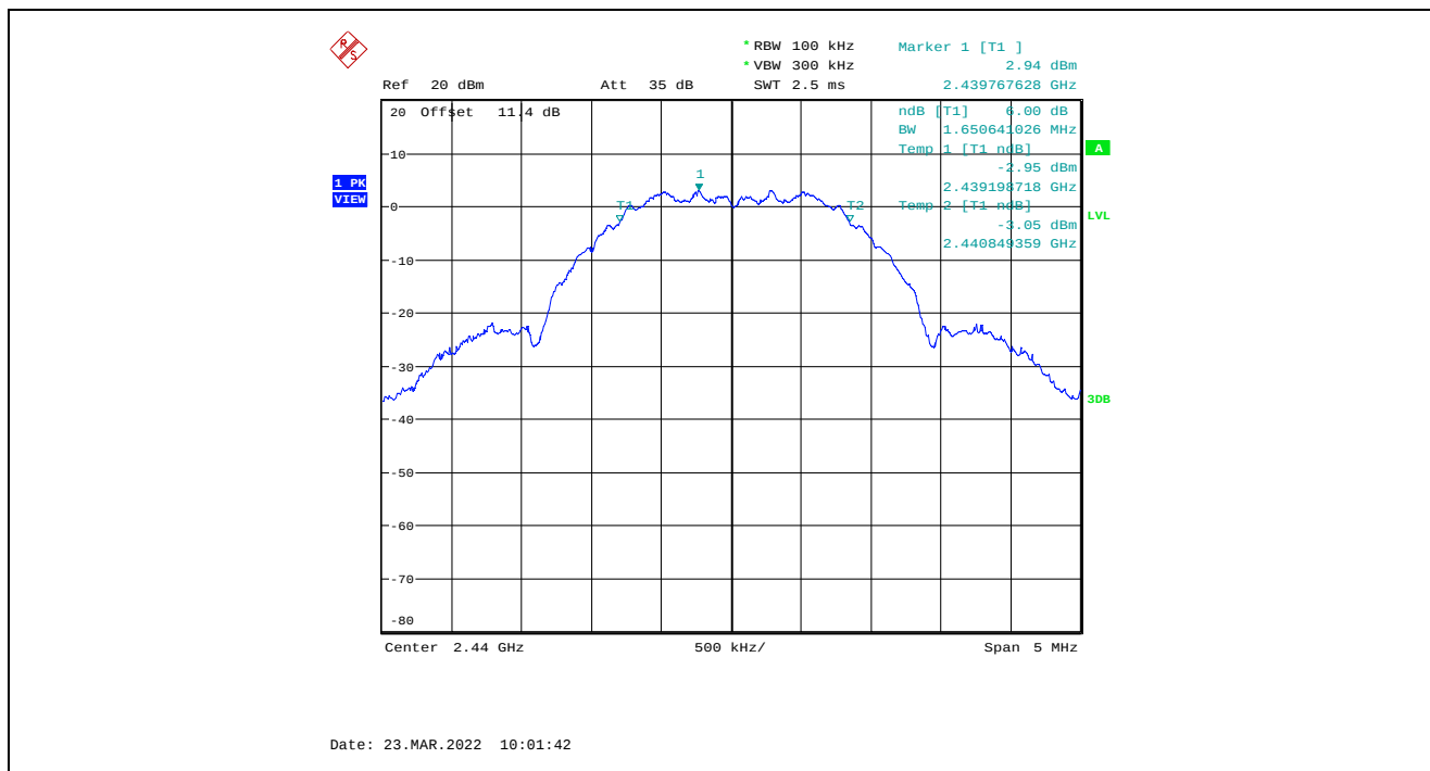
Plot 5.2.4.2. 6 dB Bandwidth, QPSK Modulation, 7 dBm Power Setting, 2440 MHz
