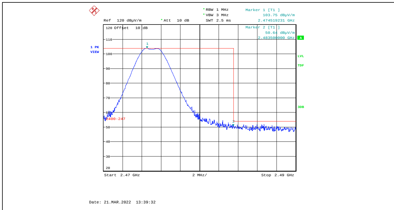
Plot 5.4.4.2.2.7. Band-Edge RF Radiated Emissions at 3 m, Horizontal Polarization, Peak High End of Frequency Band, 2475 MHz, 7 dBm Power Setting
