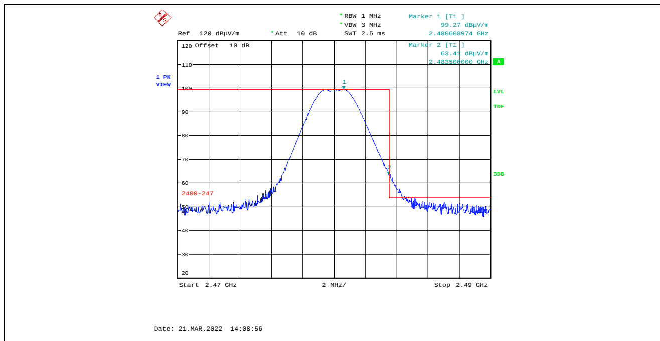
Plot 5.4.4.2.2.9. Band-Edge RF Radiated Emissions at 3 m, Vertical Polarization, Peak High End of Frequency Band, 2480 MHz, 3 dBm Power Setting
