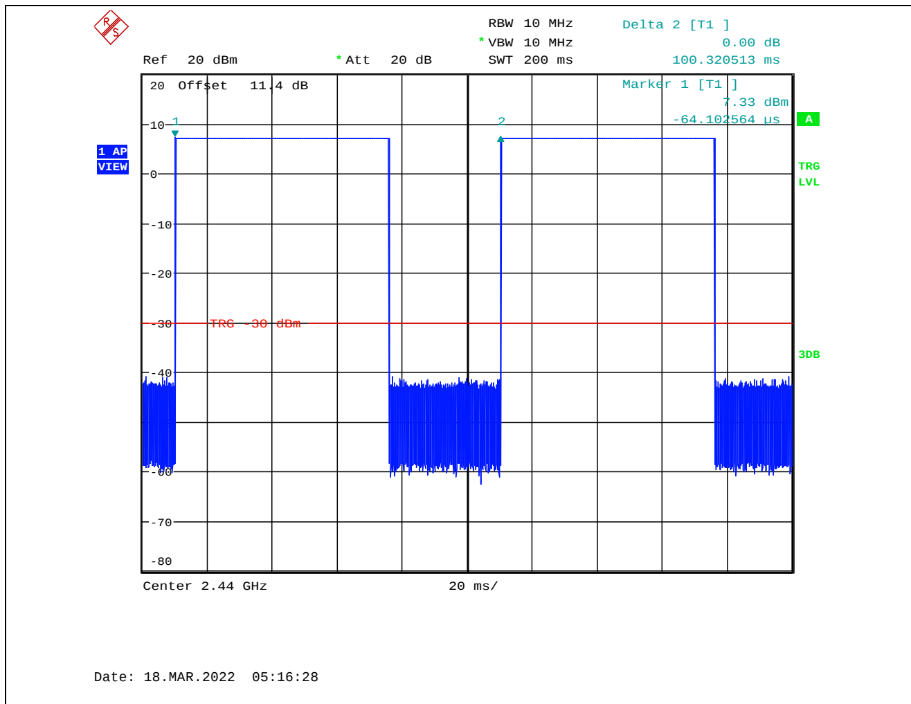
Plot 5.7.4.1.2. Duty Cycle (period of the pulse train)
