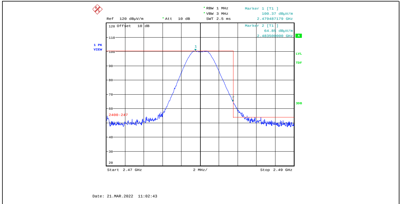
Plot 5.4.4.4.2.9. Band-Edge RF Radiated Emissions at 3 m, Vertical Polarization, Peak High End of Frequency Band, 2480 MHz, 3 dBm Power Setting
