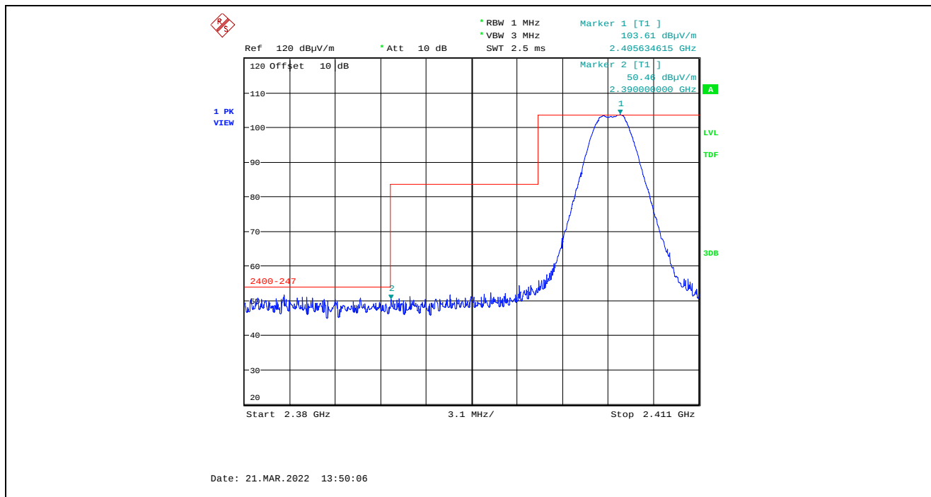
Plot 5.4.4.2.2.3. Band-Edge RF Radiated Emissions at 3 m, Horizontal Polarization, Peak Low End of Frequency Band, 2405 MHz, 7 dBm Power Setting
