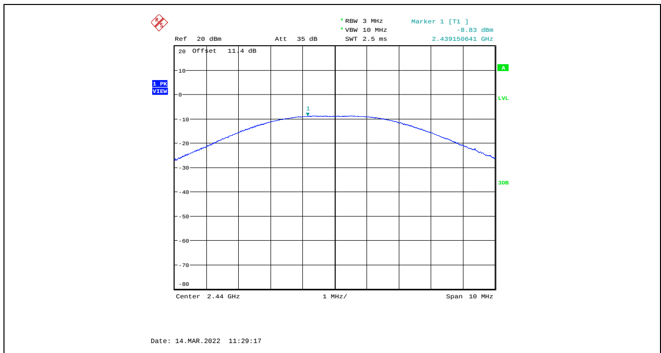
Plot 5.3.4.6. Maximum Peak Conducted Output Power, QPSK Modulation, -10 dBm Power Setting, 2440 MHz
