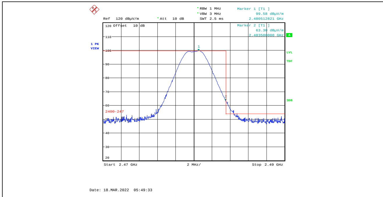
Plot 5.4.4.1.2.11. Band-Edge RF Radiated Emissions at 3 m, Horizontal Polarization, Peak High End of Frequency Band, 2480 MHz, 3 dBm Power Setting
