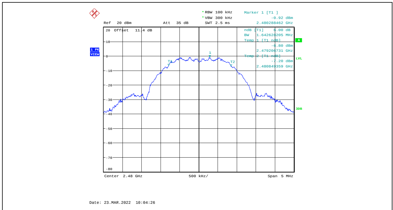
Plot 5.2.4.4. 6 dB Bandwidth, QPSK Modulation, 3 dBm Power Setting, 2480 MHz
