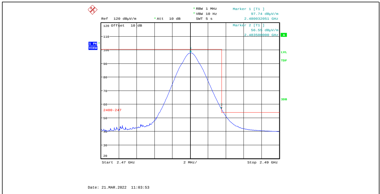
Plot 5.4.4.4.2.10. Band-Edge RF Radiated Emissions at 3 m, Vertical Polarization, Average High End of Frequency Band, 2480 MHz, 3 dBm Power Setting Marker 2: 56.55 dBμV/m – 3.61 dB = 52.94 dBμV/m (Limit 54 dBμV/m)
