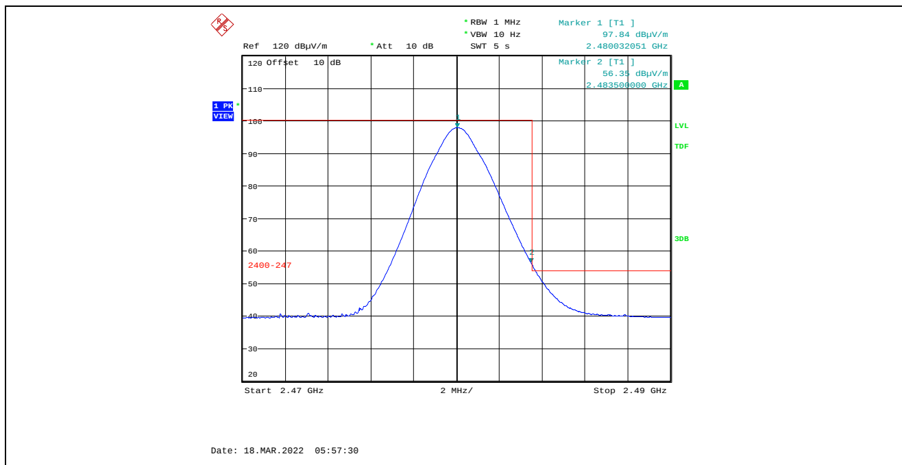
Plot 5.4.4.1.2.10. Band-Edge RF Radiated Emissions at 3 m, Vertical Polarization, Average High End of Frequency Band, 2480 MHz, 3 dBm Power Setting Marker 2: 56.35 dBμV/m – 3.61 dB Duty Cycle Factor = 52.74 dBμV/m (Limit 54 dBμV/m)
