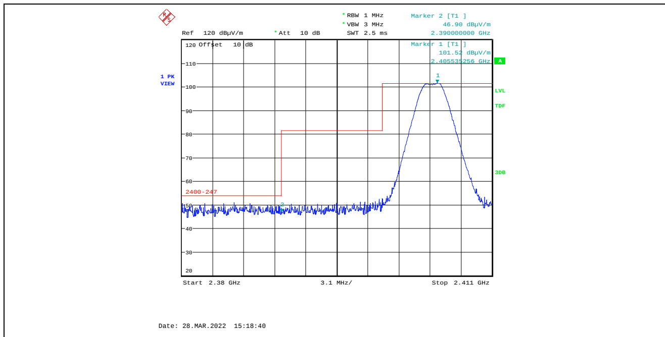
Plot 5.4.4.3.2.1. Band-Edge RF Radiated Emissions at 3 m, Vertical Polarization, Peak Low End of Frequency Band, 2405 MHz, 7 dBm Power Setting
