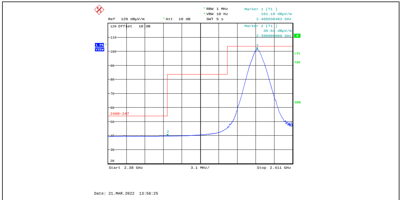
Plot 5.4.4.2.2.2. Band-Edge RF Radiated Emissions at 3 m, Vertical Polarization, Average Low End of Frequency Band, 2405 MHz, 7 dBm Power Setting
