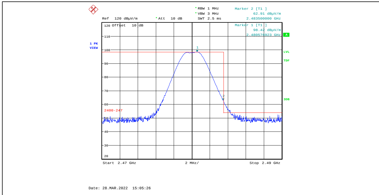
Plot 5.4.4.3.2.9. Band-Edge RF Radiated Emissions at 3 m, Vertical Polarization, Peak High End of Frequency Band, 2480 MHz, 3 dBm Power Setting
