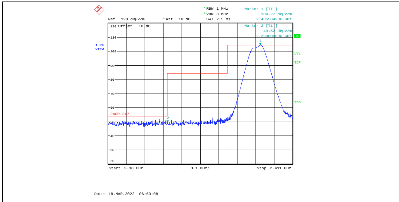
Plot 5.4.4.1.2.1. Band-Edge RF Radiated Emissions at 3 m, Vertical Polarization, Peak Low End of Frequency Band, 2405 MHz, 7 dBm Power Setting
