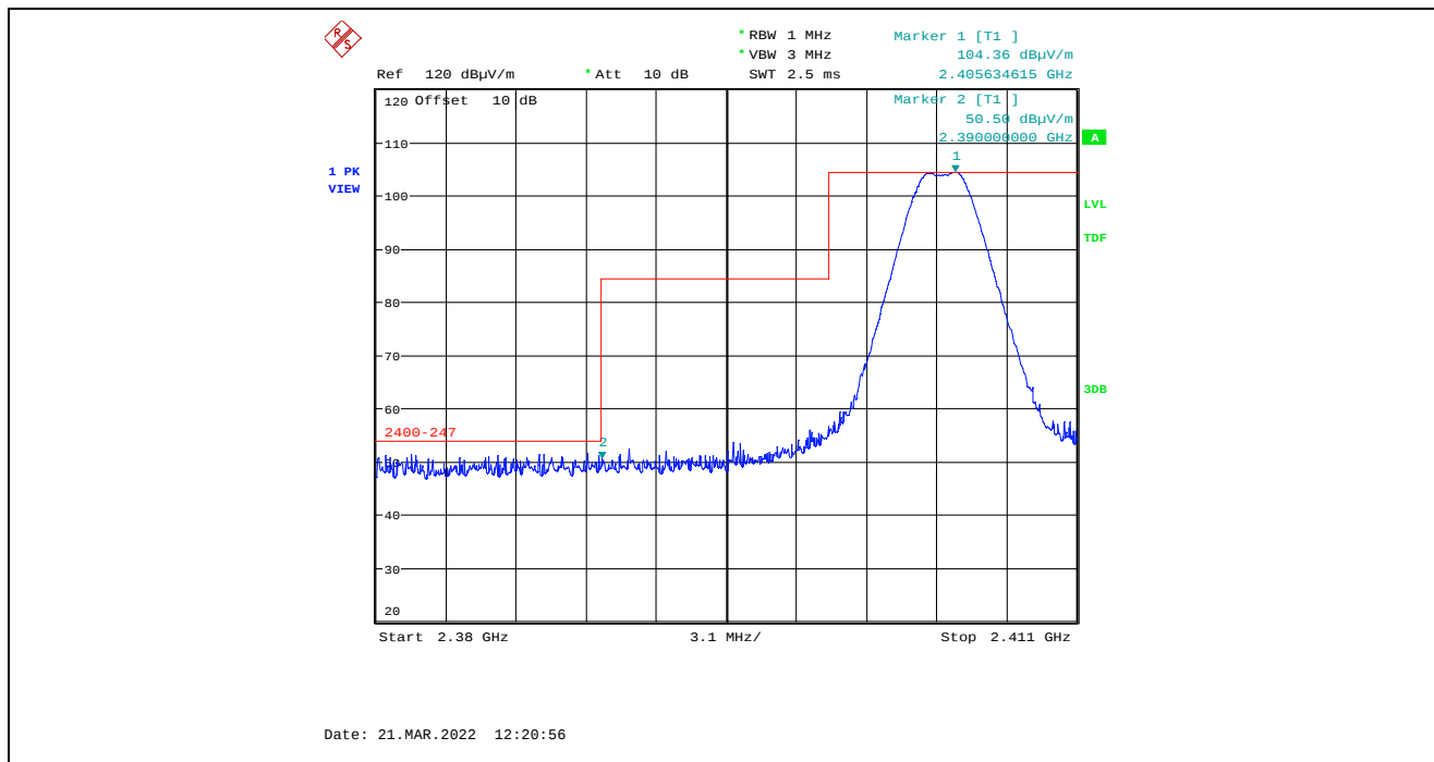
Plot 5.4.4.4.2.3. Band-Edge RF Radiated Emissions at 3 m, Horizontal Polarization, Peak Low End of Frequency Band, 2405 MHz, 7 dBm Power Setting
