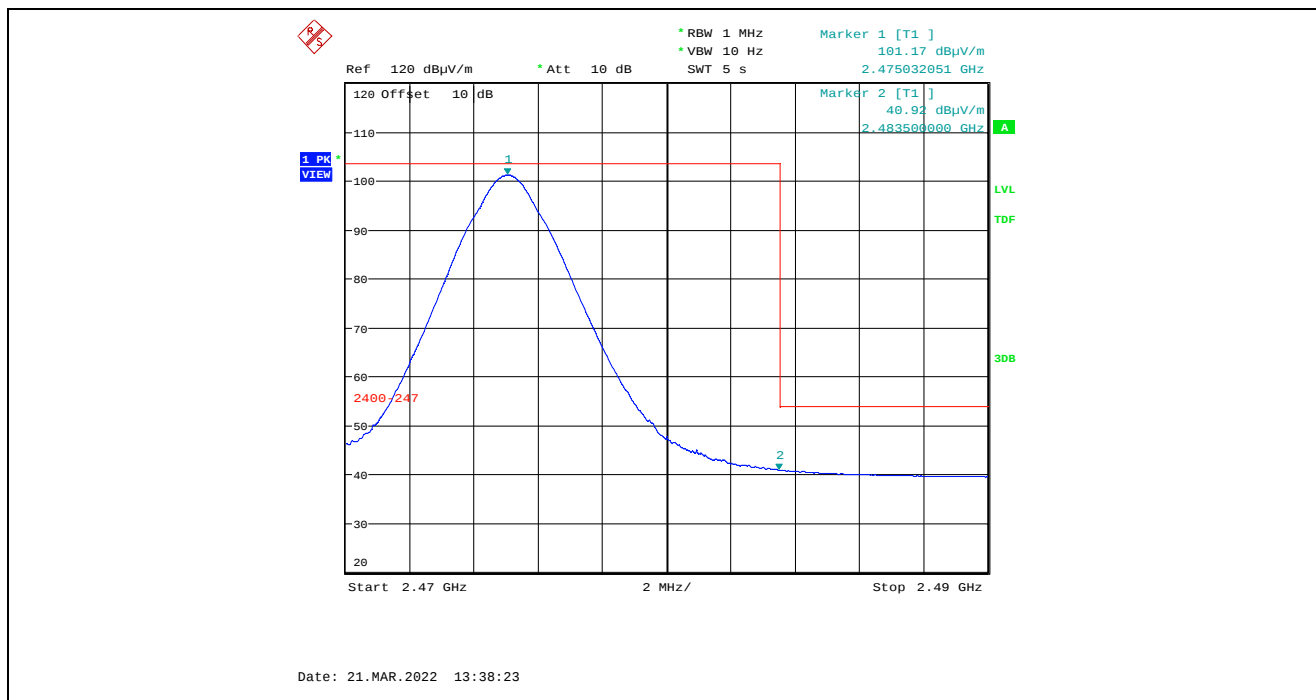
Plot 5.4.4.2.2.8. Band-Edge RF Radiated Emissions at 3 m, Horizontal Polarization, Average High End of Frequency Band, 2475 MHz, 7 dBm Power Setting
