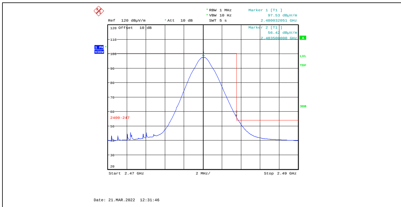
Plot 5.4.4.4.2.12. Band-Edge RF Radiated Emissions at 3 m, Horizontal Polarization, Average High End of Frequency Band, 2480 MHz, 3 dBm Power Setting Marker 2: 56.42 dBμV/m - 3.61 dB Duty Cycle Factor = 52.81 dBμV/m (Limit 54 dBμV/m)
