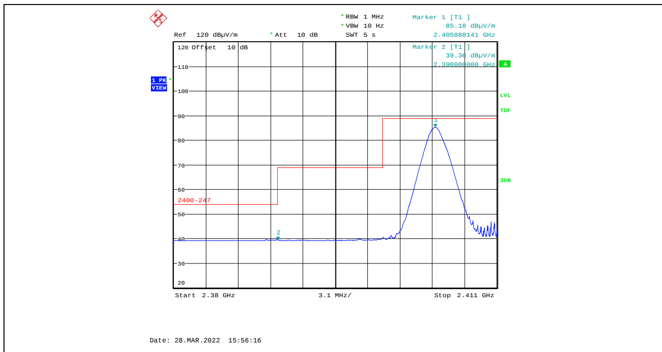
Plot 5.4.4.3.2.4. Band-Edge RF Radiated Emissions at 3 m, Horizontal Polarization, Average Low End of Frequency Band, 2405 MHz, 7 dBm Power Setting
