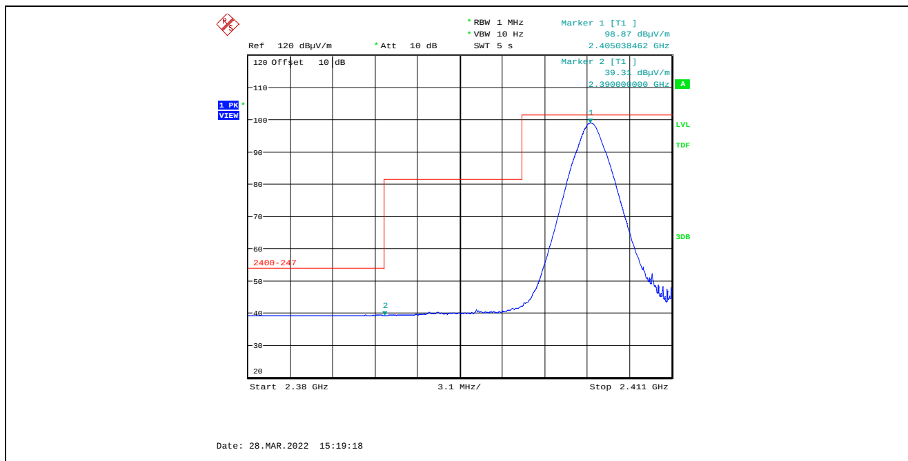
Plot 5.4.4.3.2.2. Band-Edge RF Radiated Emissions at 3 m, Vertical Polarization, Average Low End of Frequency Band, 2405 MHz, 7 dBm Power Setting
