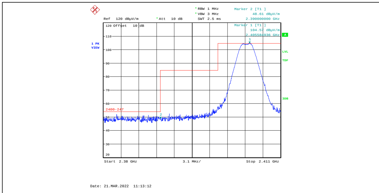
Plot 5.4.4.4.2.1. Band-Edge RF Radiated Emissions at 3 m, Vertical Polarization, Peak Low End of Frequency Band, 2405 MHz, 7 dBm Power Setting
