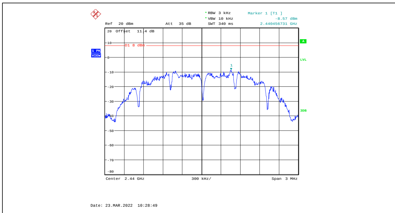
Plot 5.5.4.2. Power Spectral Density, QPSK Modulation, 7 dBm Power Setting, 2440 MHz
