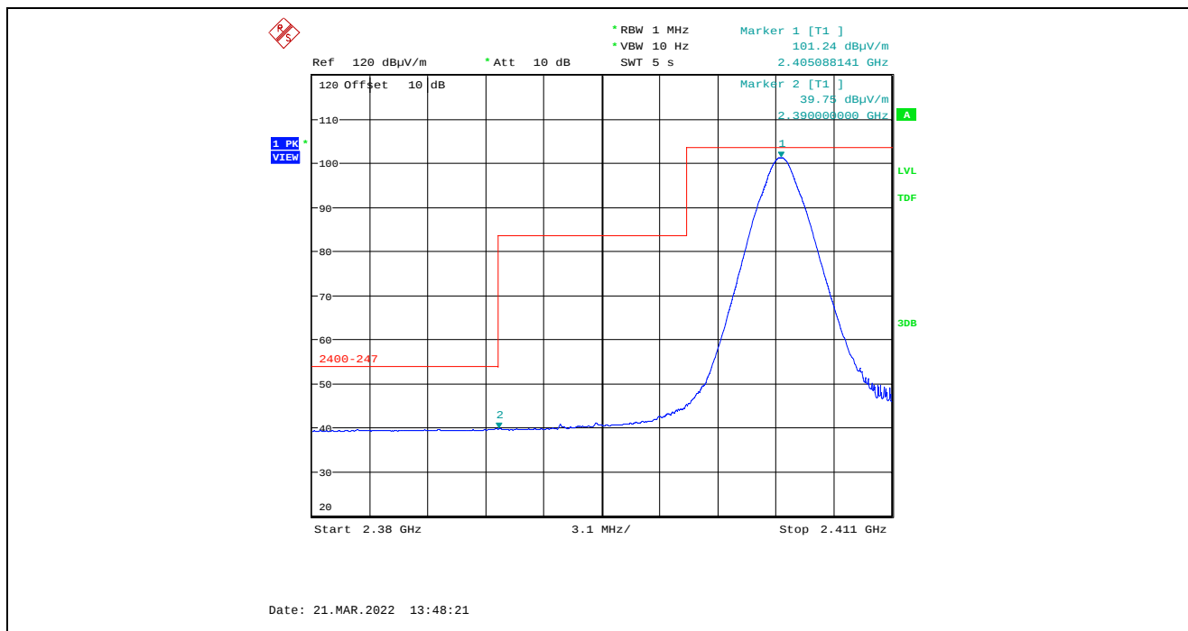
Plot 5.4.4.2.2.4. Band-Edge RF Radiated Emissions at 3 m, Horizontal Polarization, Average Low End of Frequency Band, 2405 MHz, 7 dBm Power Setting
