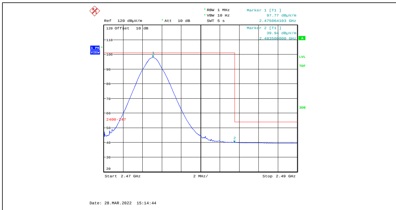
Plot 5.4.4.3.2.6. Band-Edge RF Radiated Emissions at 3 m, Vertical Polarization, Average High End of Frequency Band, 2475 MHz, 7 dBm Power Setting
