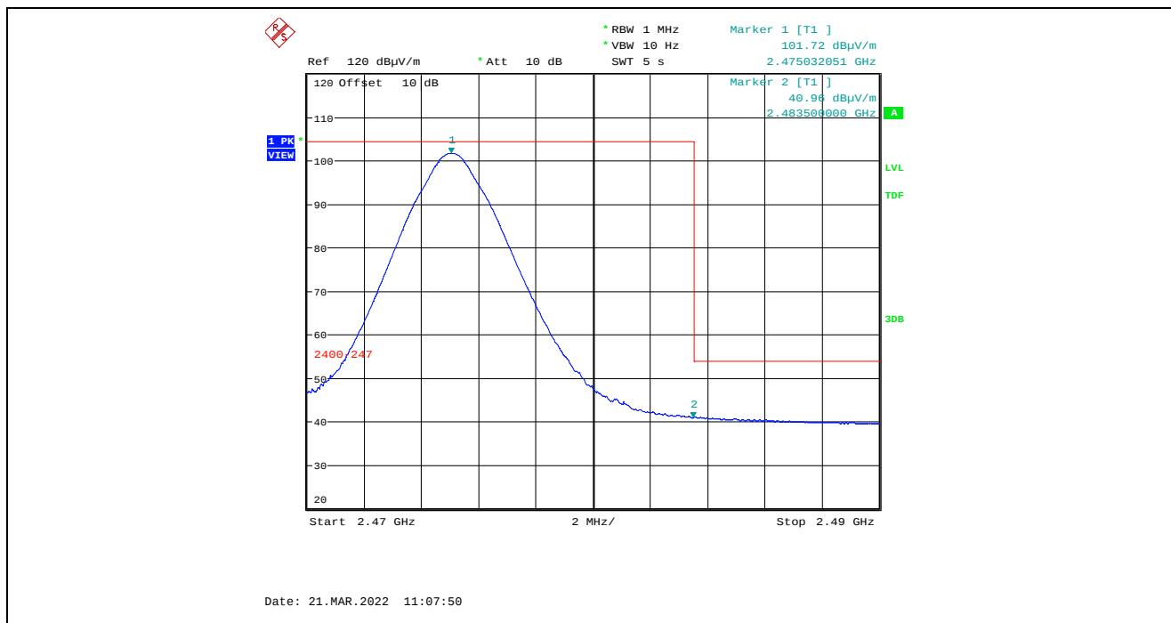
Plot 5.4.4.4.2.6. Band-Edge RF Radiated Emissions at 3 m, Vertical Polarization, Average High End of Frequency Band, 2475 MHz, 7 dBm Power Setting
