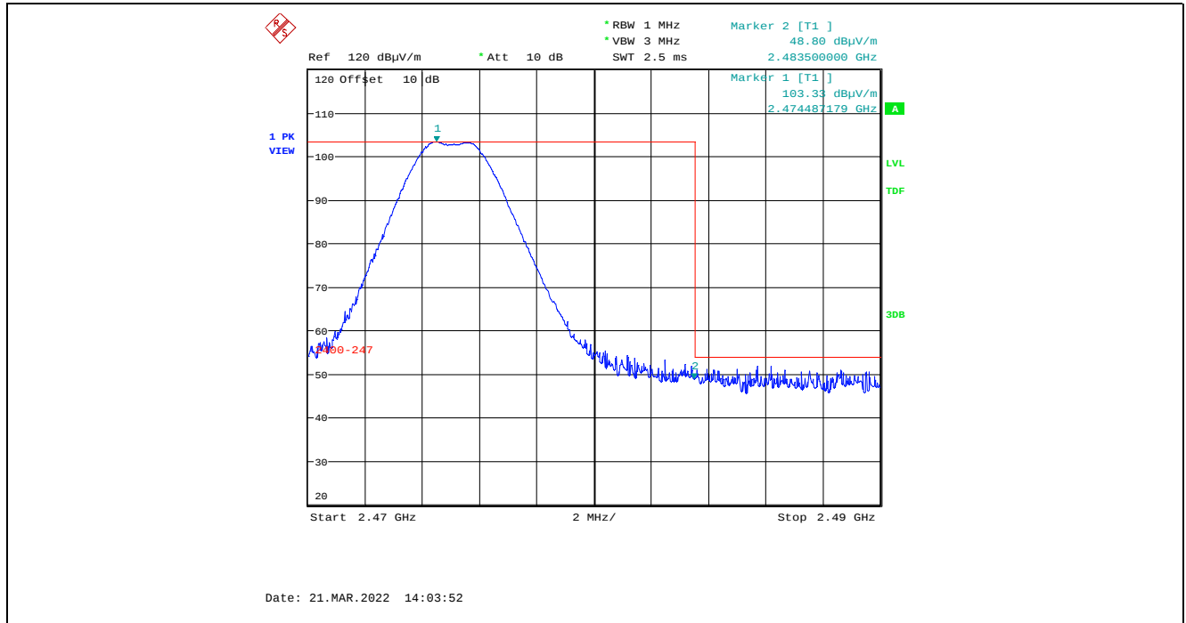
Plot 5.4.4.2.2.5. Band-Edge RF Radiated Emissions at 3 m, Vertical Polarization, Peak High End of Frequency Band, 2475 MHz, 7 dBm Power Setting
