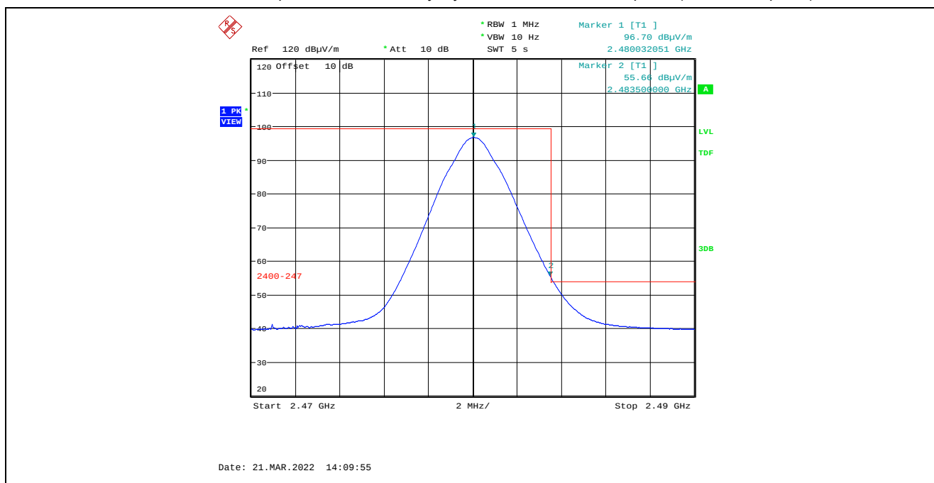
Plot 5.4.4.2.2.10. Band-Edge RF Radiated Emissions at 3 m, Vertical Polarization, Average High End of Frequency Band, 2480 MHz, 3 dBm Power Setting Marker 2: 55.66 dBμV/m – 3.61 dB Duty Cycle Factor = 52.05 dBμV/m (Limit 54 dBμV/m)
