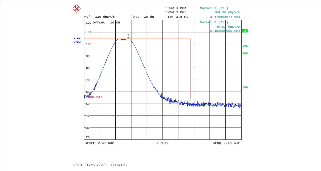
Plot 5.4.4.4.2.5. Band-Edge RF Radiated Emissions at 3 m, Vertical Polarization, Peak High End of Frequency Band, 2475 MHz, 7 dBm Power Setting
