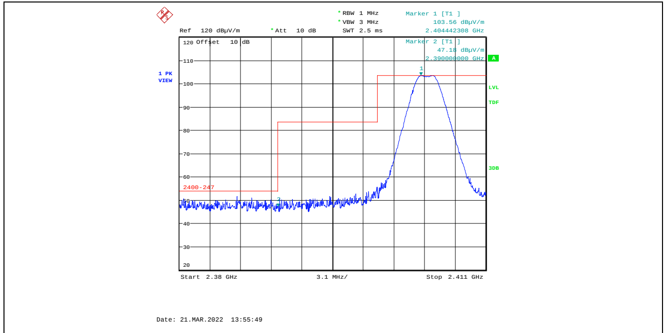
Plot 5.4.4.2.2.1. Band-Edge RF Radiated Emissions at 3 m, Vertical Polarization, Peak Low End of Frequency Band, 2405 MHz, 7 dBm Power Setting
