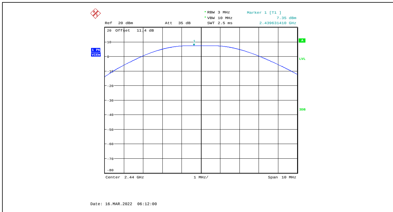
Plot 5.3.4.2. Maximum Peak Conducted Output Power, QPSK Modulation, 7 dBm Power Setting, 2440 MHz
