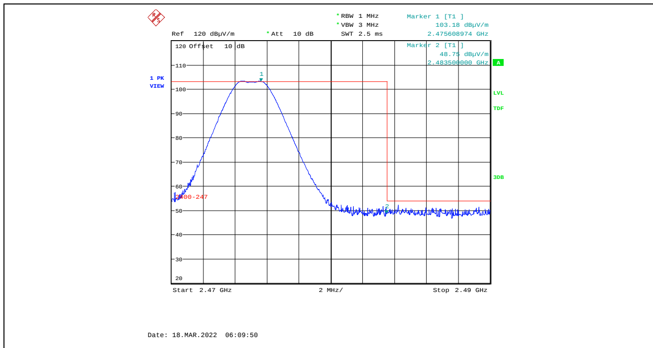
Plot 5.4.4.1.2.5. Band-Edge RF Radiated Emissions at 3 m, Vertical Polarization, Peak High End of Frequency Band, 2475 MHz, 7 dBm Power Setting
