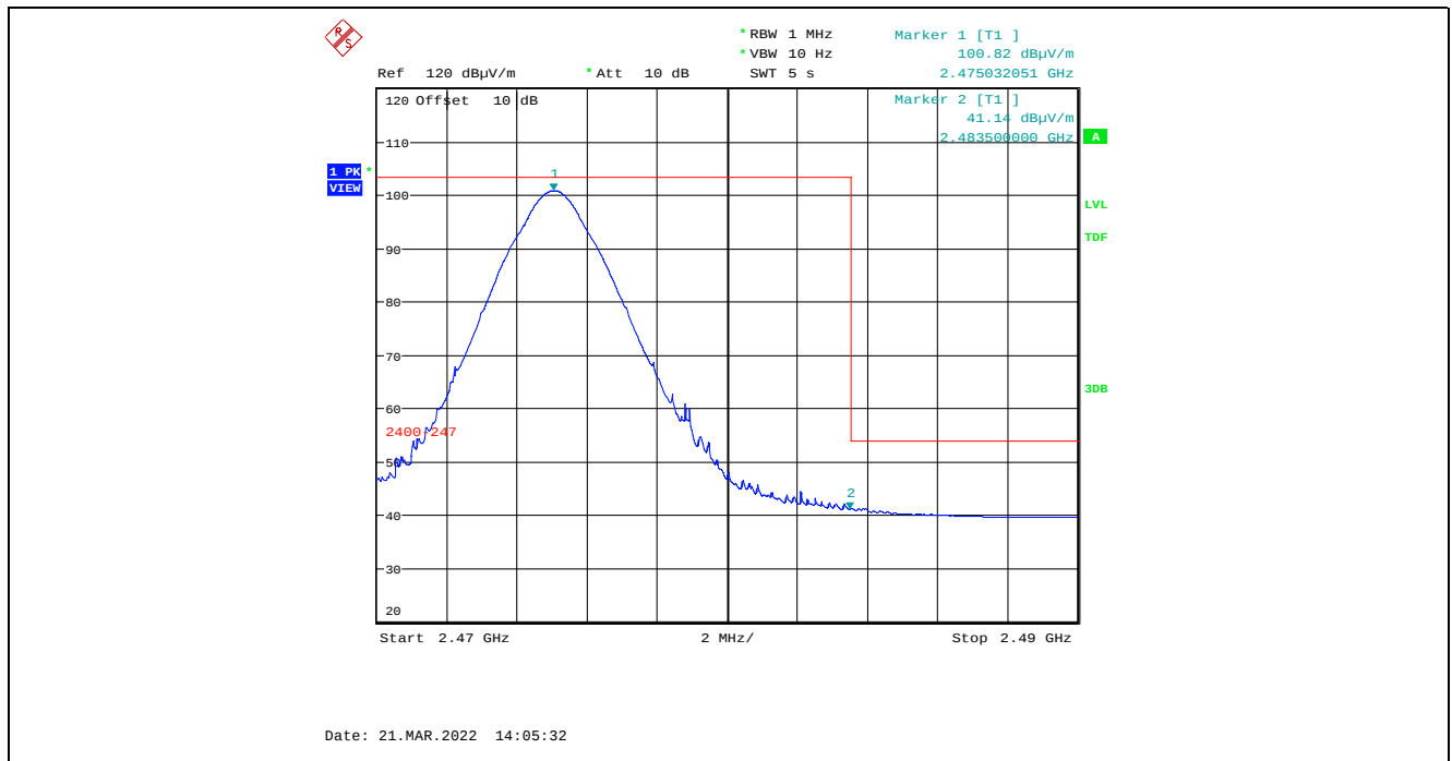
Plot 5.4.4.2.2.6. Band-Edge RF Radiated Emissions at 3 m, Vertical Polarization, Average High End of Frequency Band, 2475 MHz, 7 dBm Power Setting
