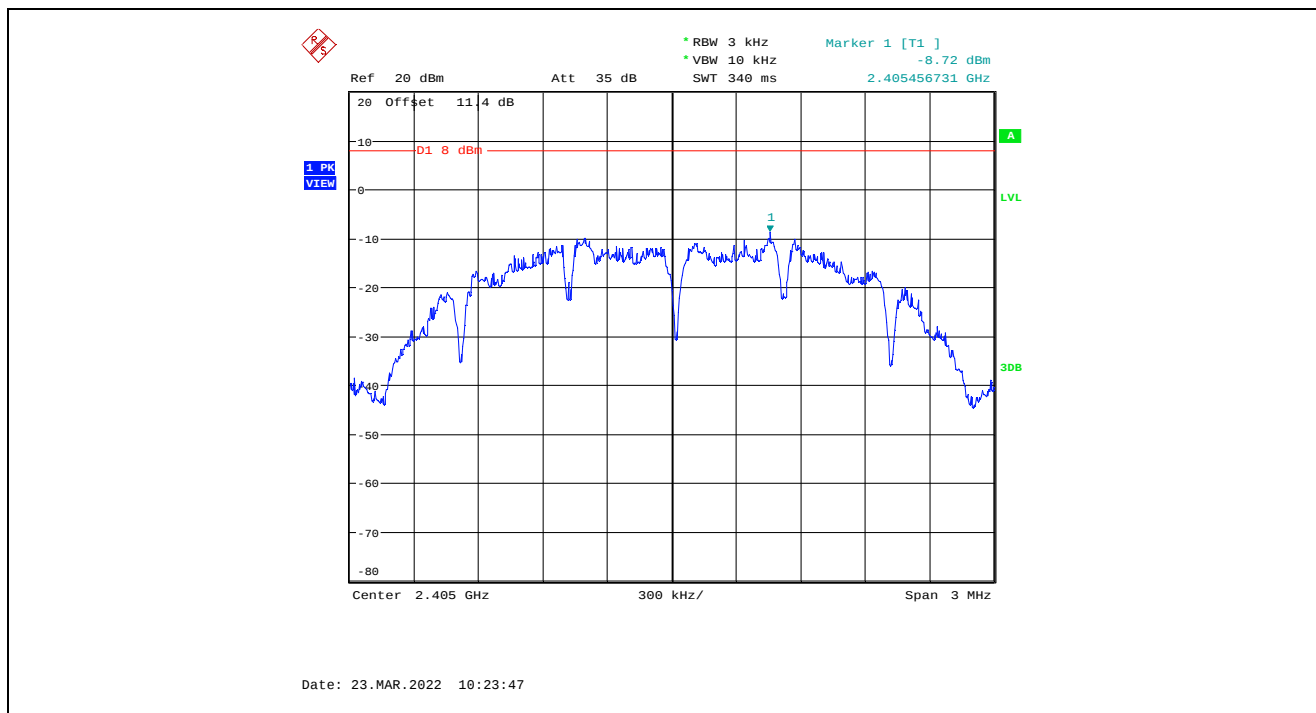
Plot 5.5.4.1. Power Spectral Density, QPSK Modulation, 7 dBm Power Setting, 2405 MHz
