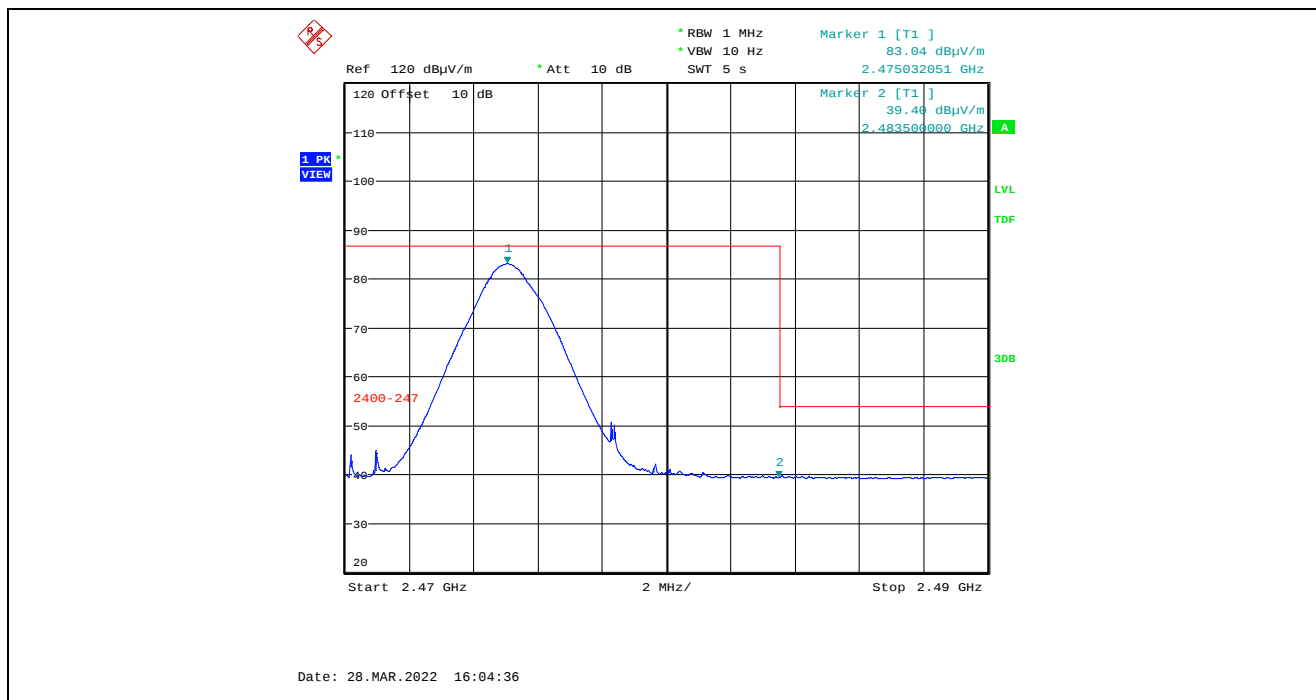
Plot 5.4.4.3.2.8. Band-Edge RF Radiated Emissions at 3 m, Horizontal Polarization, Average High End of Frequency Band, 2475 MHz, 7 dBm Power Setting
