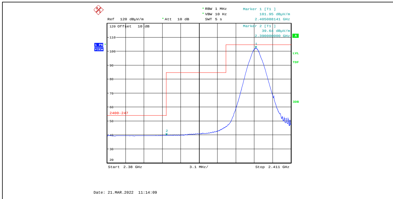
Plot 5.4.4.4.2.2. Band-Edge RF Radiated Emissions at 3 m, Vertical Polarization, Average Low End of Frequency Band, 2405 MHz, 7 dBm Power Setting
