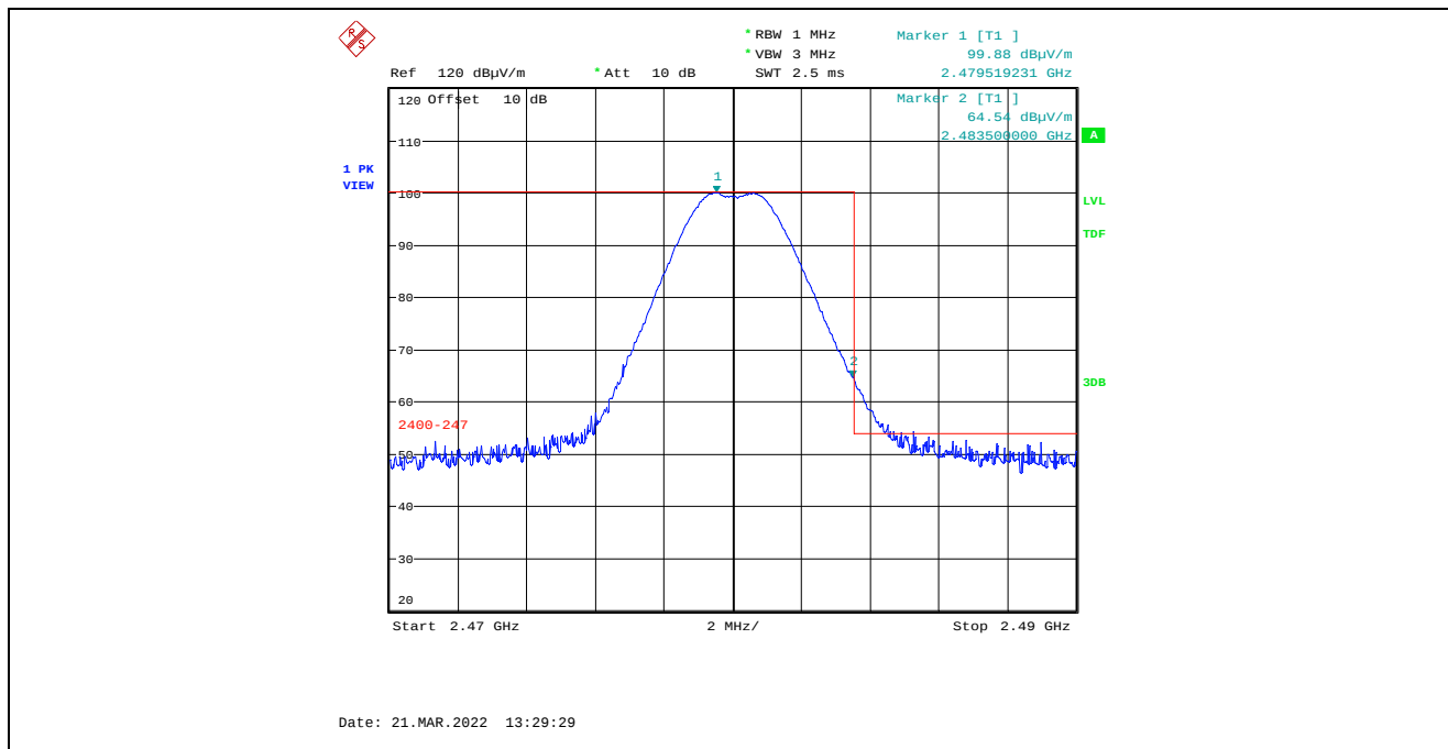
Plot 5.4.4.2.2.11. Band-Edge RF Radiated Emissions at 3 m, Horizontal Polarization, Peak High End of Frequency Band, 2480 MHz, 3 dBm Power Setting
