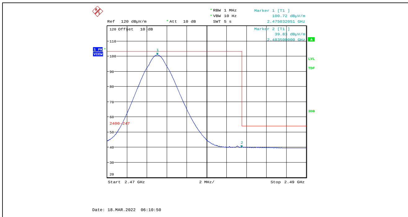
Plot 5.4.4.1.2.6. Band-Edge RF Radiated Emissions at 3 m, Vertical Polarization, Average High End of Frequency Band, 2475 MHz, 7 dBm Power Setting
