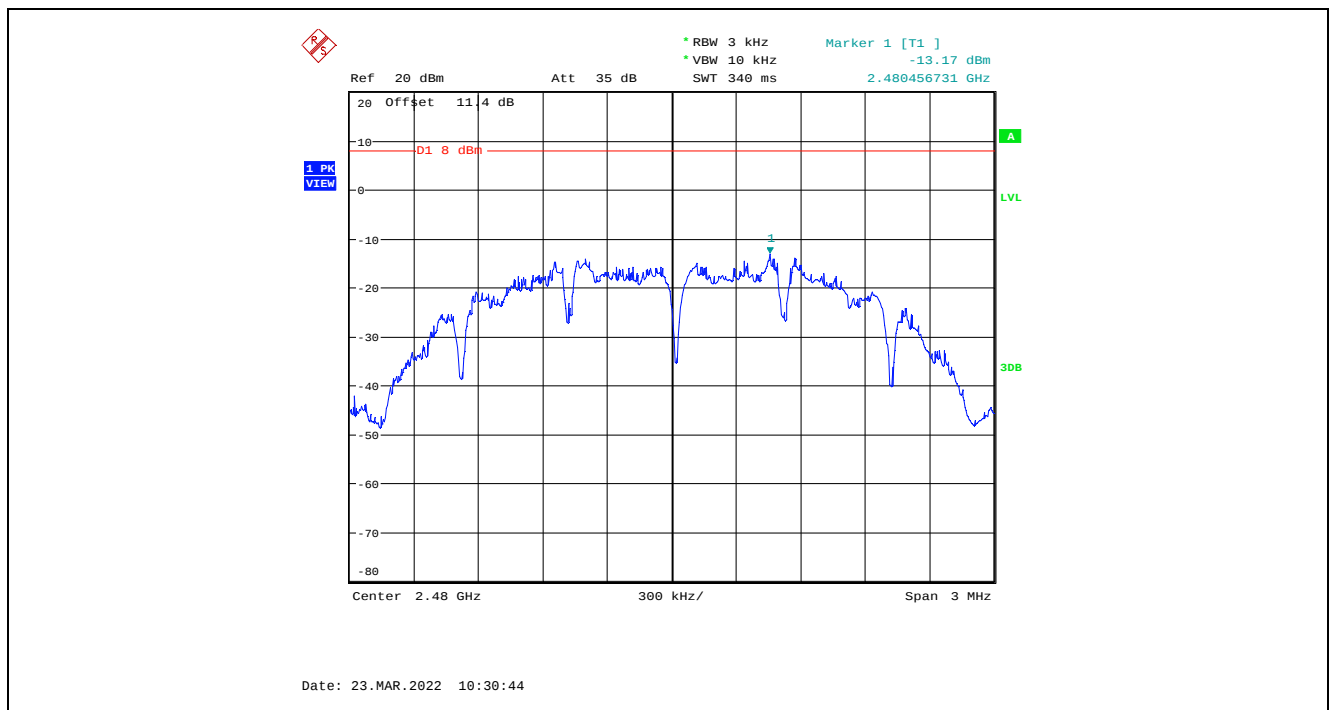
Plot 5.5.4.4. Power Spectral Density, QPSK Modulation, 3 dBm Power Setting, 2480 MHz
