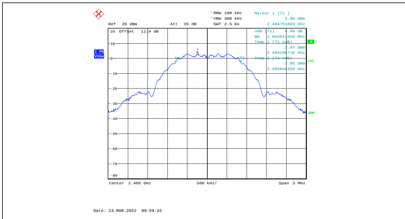
Plot 5.2.4.1. 6 dB Bandwidth, QPSK Modulation, 7 dBm Power Setting, 2405 MHz
