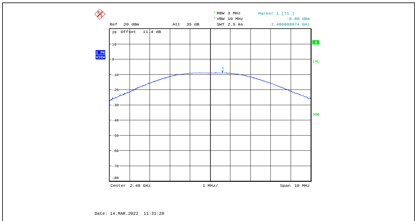
Plot 5.3.4.8. Maximum Peak Conducted Output Power, QPSK Modulation, -10 dBm Power Setting, 2480 MHz
