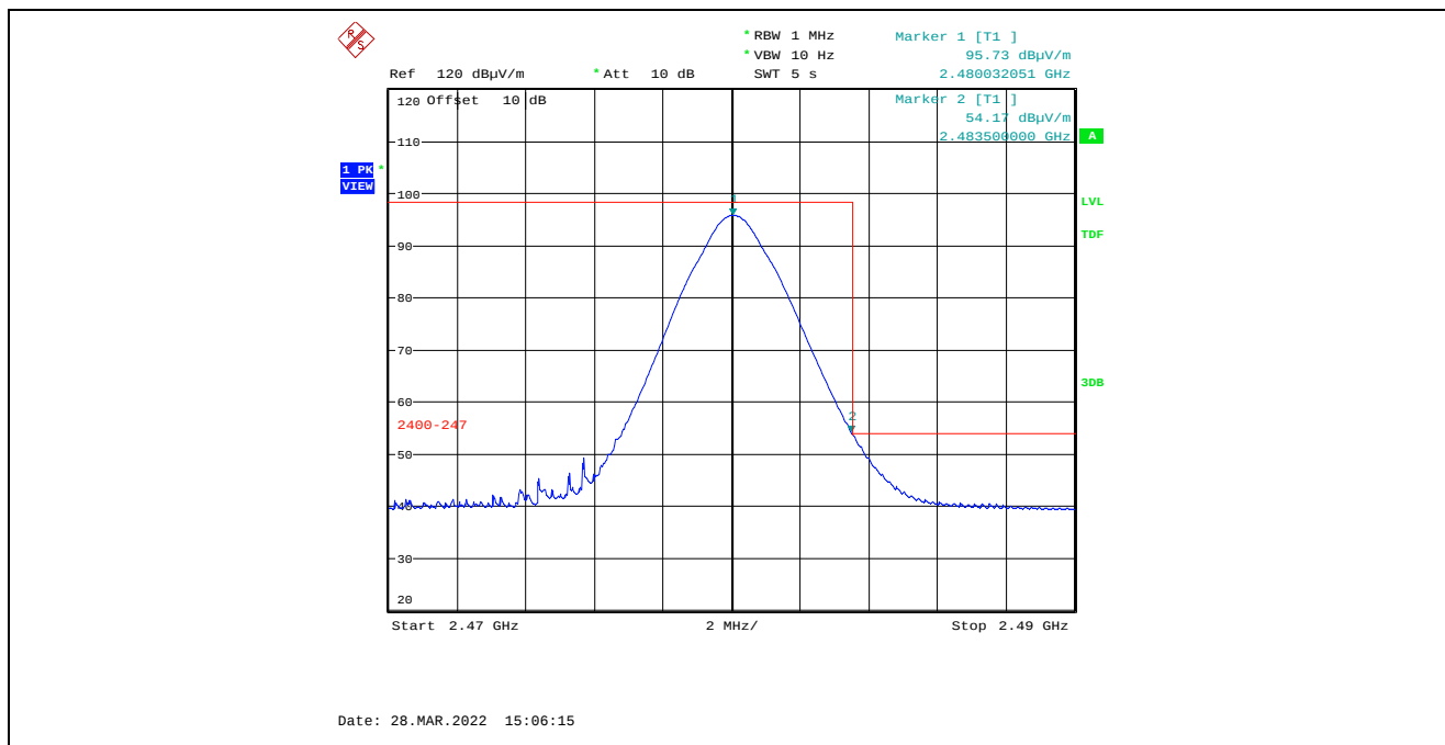
Plot 5.4.4.3.2.10. Band-Edge RF Radiated Emissions at 3 m, Vertical Polarization, Average High End of Frequency Band, 2480 MHz, 3 dBm Power Setting Marker 2: 54.17 dBμV/m – 3.61 dB Duty Cycle Factor = 50.56 dBμV/m (Limit 54 dBμV/m)
