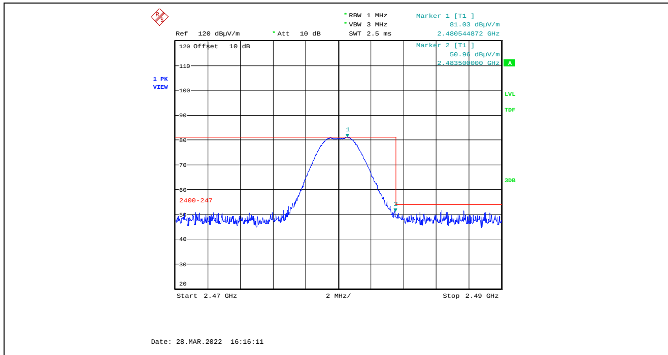
Plot 5.4.4.3.2.11. Band-Edge RF Radiated Emissions at 3 m, Horizontal Polarization, Peak High End of Frequency Band, 2480 MHz, 3 dBm Power Setting
