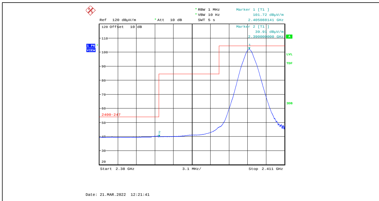
Plot 5.4.4.4.2.4. Band-Edge RF Radiated Emissions at 3 m, Horizontal Polarization, Average Low End of Frequency Band, 2405 MHz, 7 dBm Power Setting
