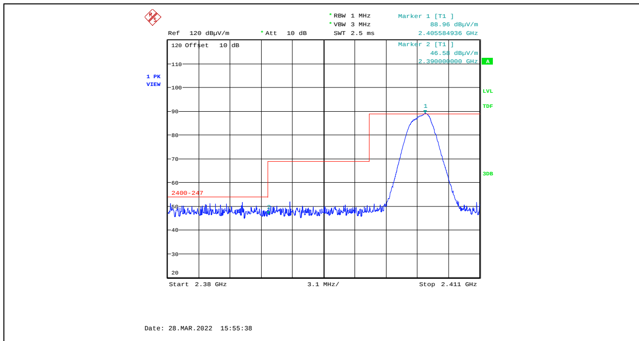
Plot 5.4.4.3.2.3. Band-Edge RF Radiated Emissions at 3 m, Horizontal Polarization, Peak Low End of Frequency Band, 2405 MHz, 7 dBm Power Setting
