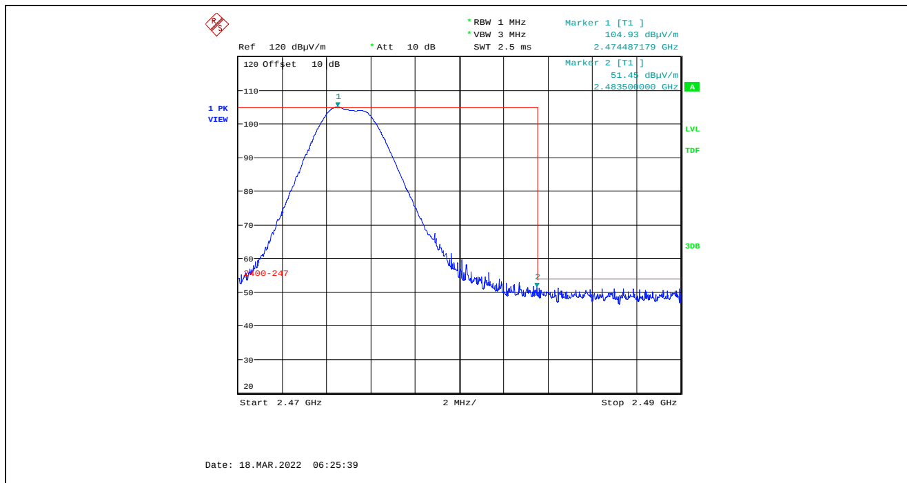
Plot 5.4.4.1.2.7. Band-Edge RF Radiated Emissions at 3 m, Horizontal Polarization, Peak High End of Frequency Band, 2475 MHz, 7 dBm Power Setting
