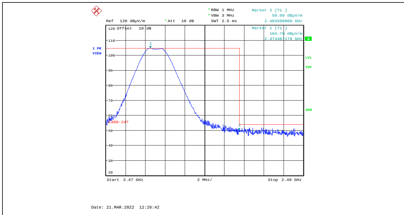
Plot 5.4.4.4.2.7. Band-Edge RF Radiated Emissions at 3 m, Horizontal Polarization, Peak High End of Frequency Band, 2475 MHz, 7 dBm Power Setting
