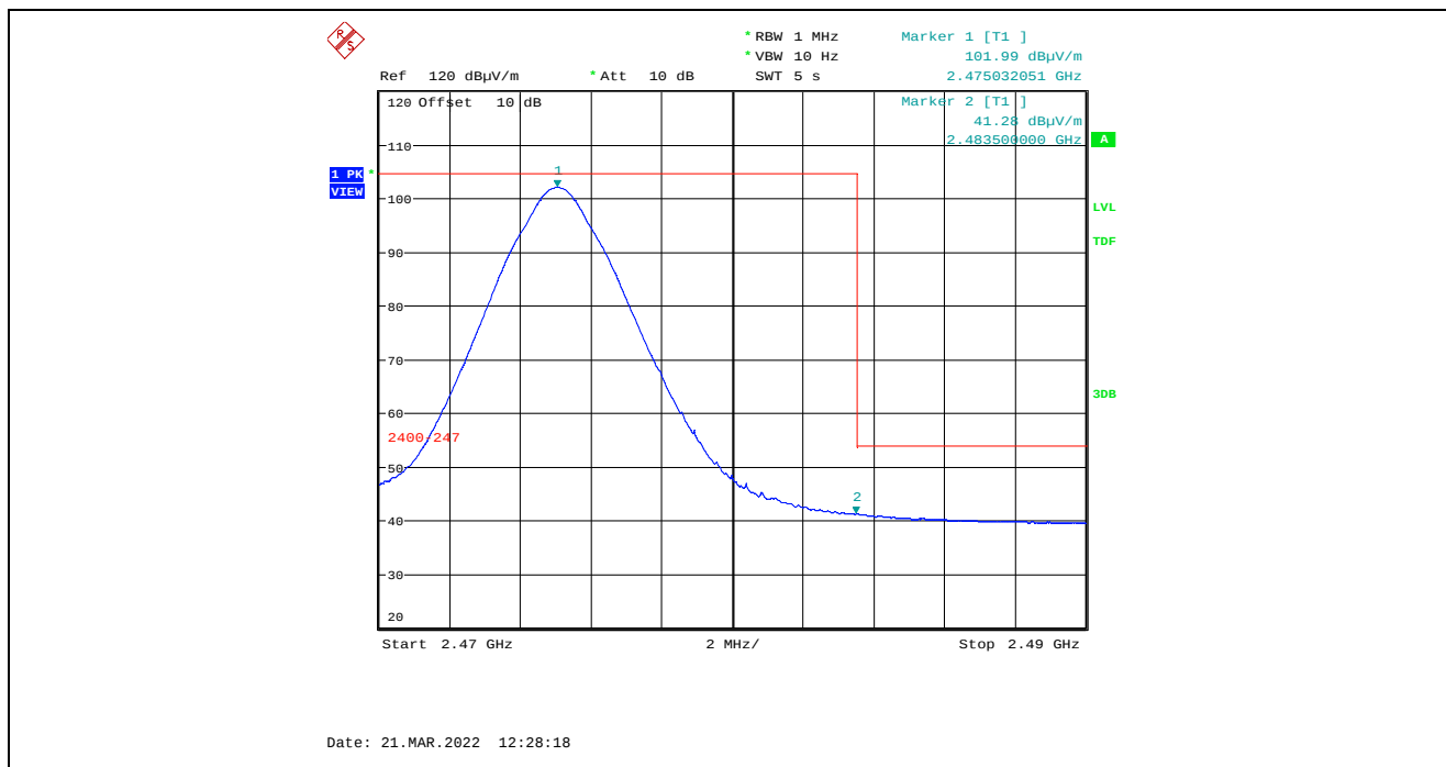
Plot 5.4.4.4.2.8. Band-Edge RF Radiated Emissions at 3 m, Horizontal Polarization, Average High End of Frequency Band, 2475 MHz, 7 dBm Power Setting
