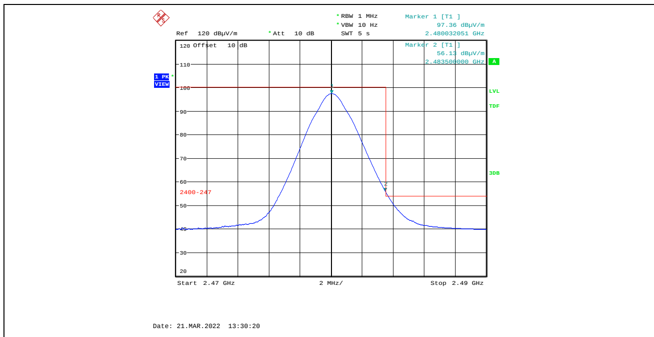
Plot 5.4.4.2.2.12. Band-Edge RF Radiated Emissions at 3 m, Horizontal Polarization, Average High End of Frequency Band, 2480 MHz, 3 dBm Power Setting Marker 2: 56.13 dBμV/m – 3.61 dB Duty Cycle Factor = 52.52 dBμV/m (Limit 54 dBμV/m)
