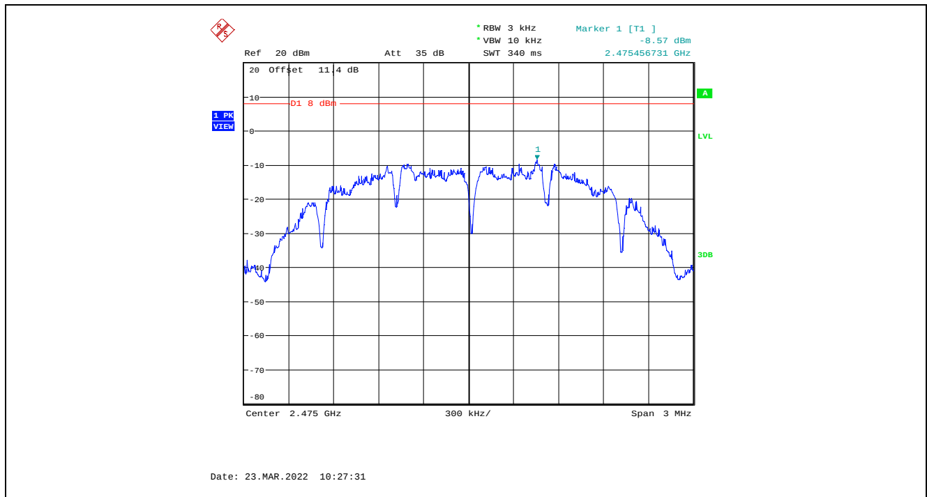
Plot 5.5.4.3. Power Spectral Density, QPSK Modulation, 7 dBm Power Setting, 2475 MHz
