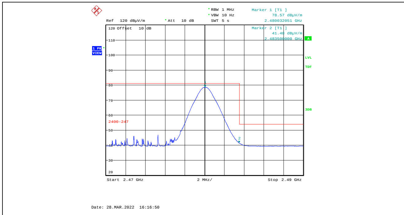
Plot 5.4.4.3.2.12. Band-Edge RF Radiated Emissions at 3 m, Horizontal Polarization, Average High End of Frequency Band, 2480 MHz, 3 dBm Power Setting
