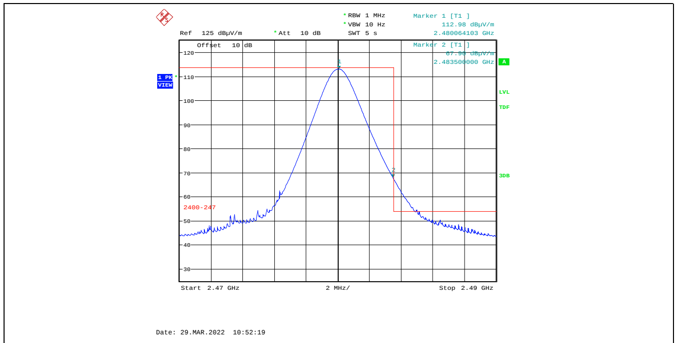
Plot 5.4.4.4.2.6. Band-Edge RF Radiated Emissions at 3 m, Vertical Polarization, Average High End of Frequency Band, 2480 MHz, 8 dBm Power Setting, 1 Mbps Marker 2: 67.90 dBμV/m – 33.51 dB Duty Cycle Factor = 34.39 dBμV/m (Limit 54 dBμV/m)
