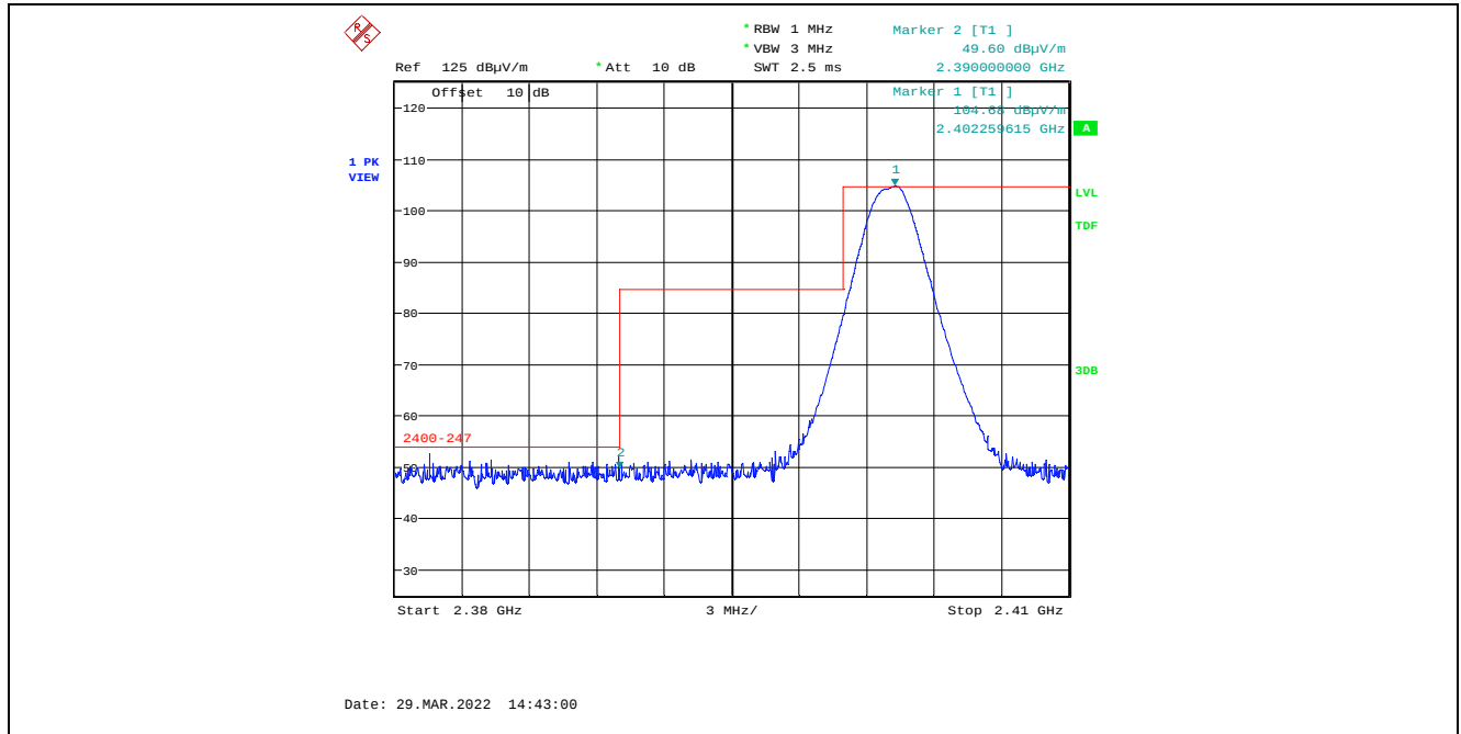
Plot 5.4.4.1.2.1. Band-Edge RF Radiated Emissions at 3 m, Vertical Polarization, Peak Low End of Frequency Band, 2402 MHz, 8 dBm Power Setting, 1 Mbps
