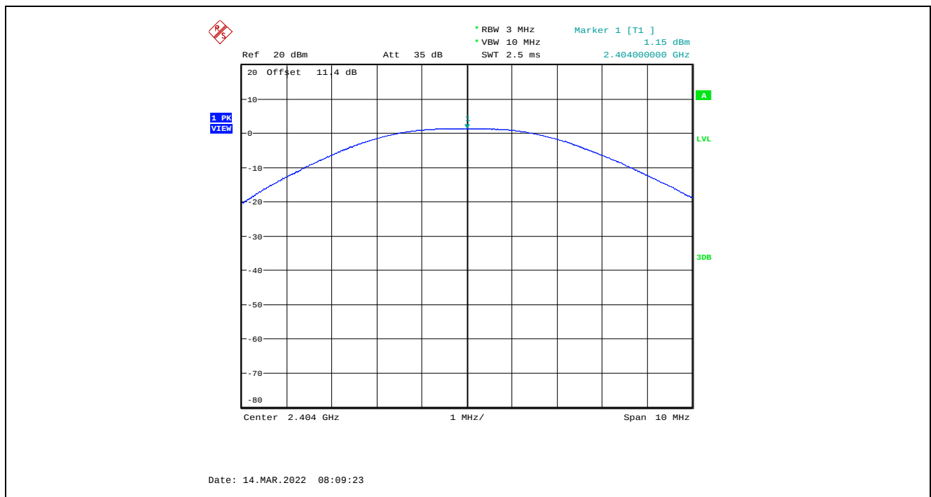
Plot 5.3.4.10. Maximum Peak Conducted Output Power, GFSK Modulation, 2 Mbps, -2 dBm Power Setting, 2404 MHz
