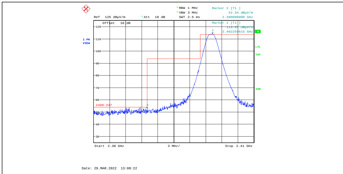
Plot 5.4.4.2.2.1. Band-Edge RF Radiated Emissions at 3 m, Vertical Polarization, Peak Low End of Frequency Band, 2402 MHz, 8 dBm Power Setting, 1 Mbps
