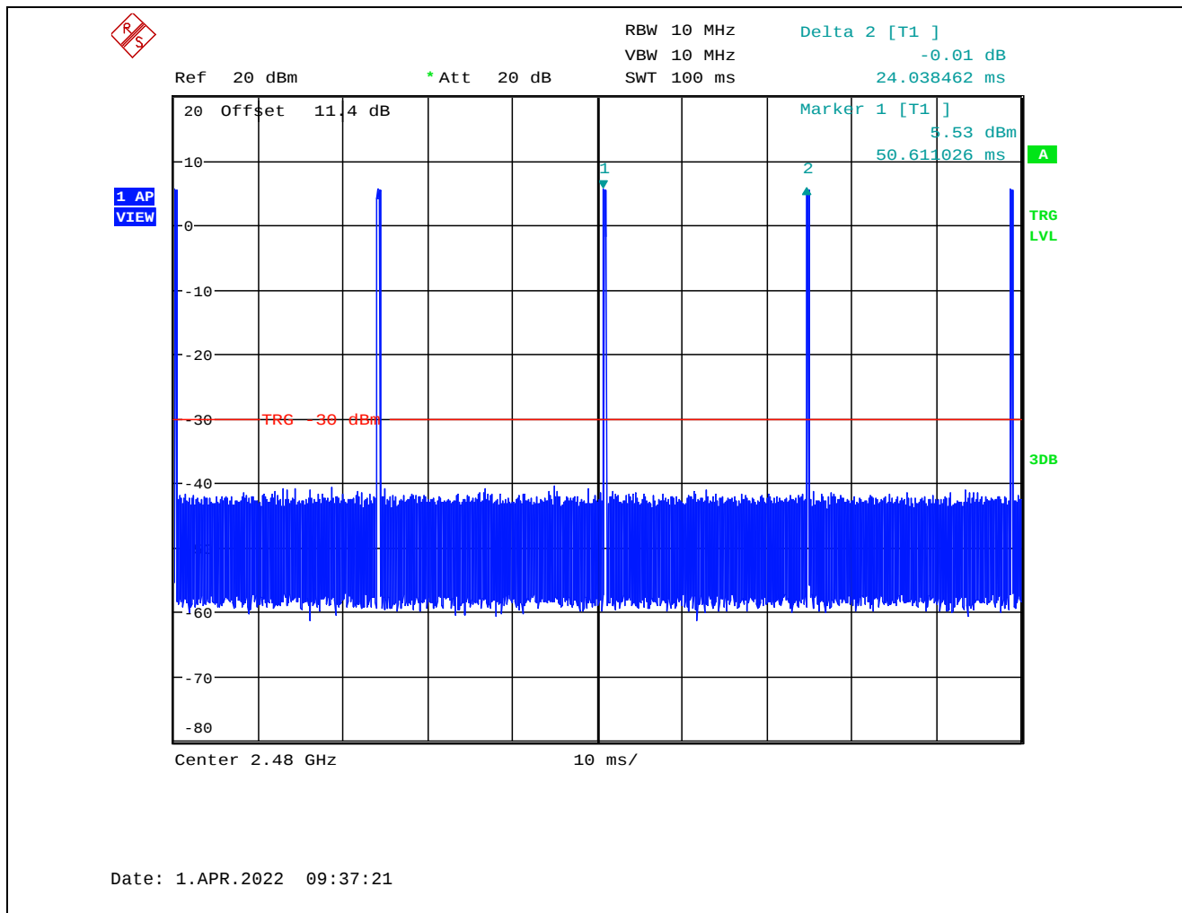
Plot 5.7.4.1.2. Duty Cycle (5 Pulses in 100 ms)
