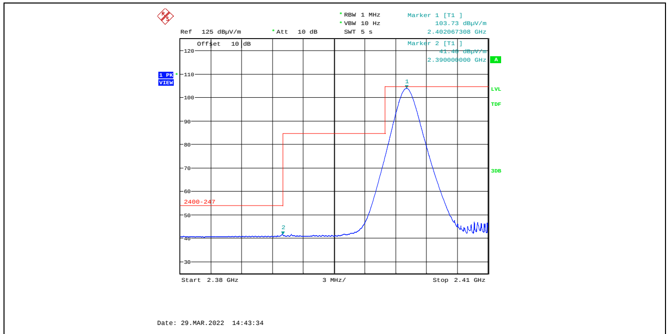
Plot 5.4.4.1.2.2. Band-Edge RF Radiated Emissions at 3 m, Vertical Polarization, Average Low End of Frequency Band, 2402 MHz, 8 dBm Power Setting, 1 Mbps
