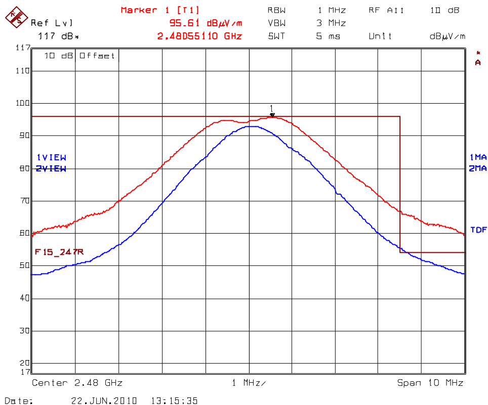
Plot 5.9.4.4.5. Band-Edge RF Radiated Emissions @ 3 m High End of Frequency Band, 2480 MHz Rx Antenna Orientation: Horizontal
