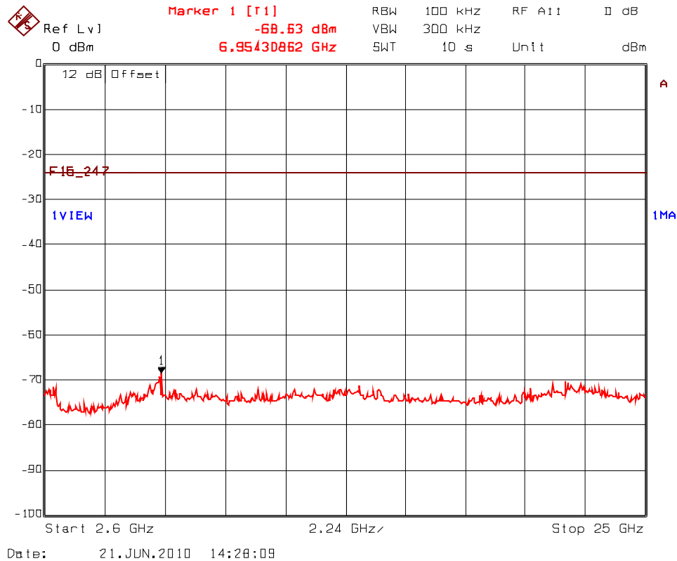
Plot 5.8.4.2.14. Spurious RF Conducted Emissions Transmitter Frequency: 2475 MHz, Low Power
