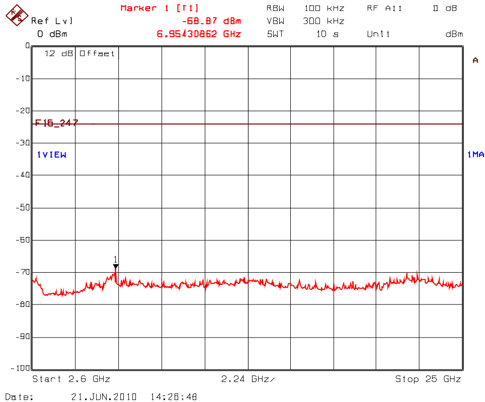
Plot 5.8.4.2.12. Spurious RF Conducted Emissions Transmitter Frequency: 2440 MHz, Low Power
