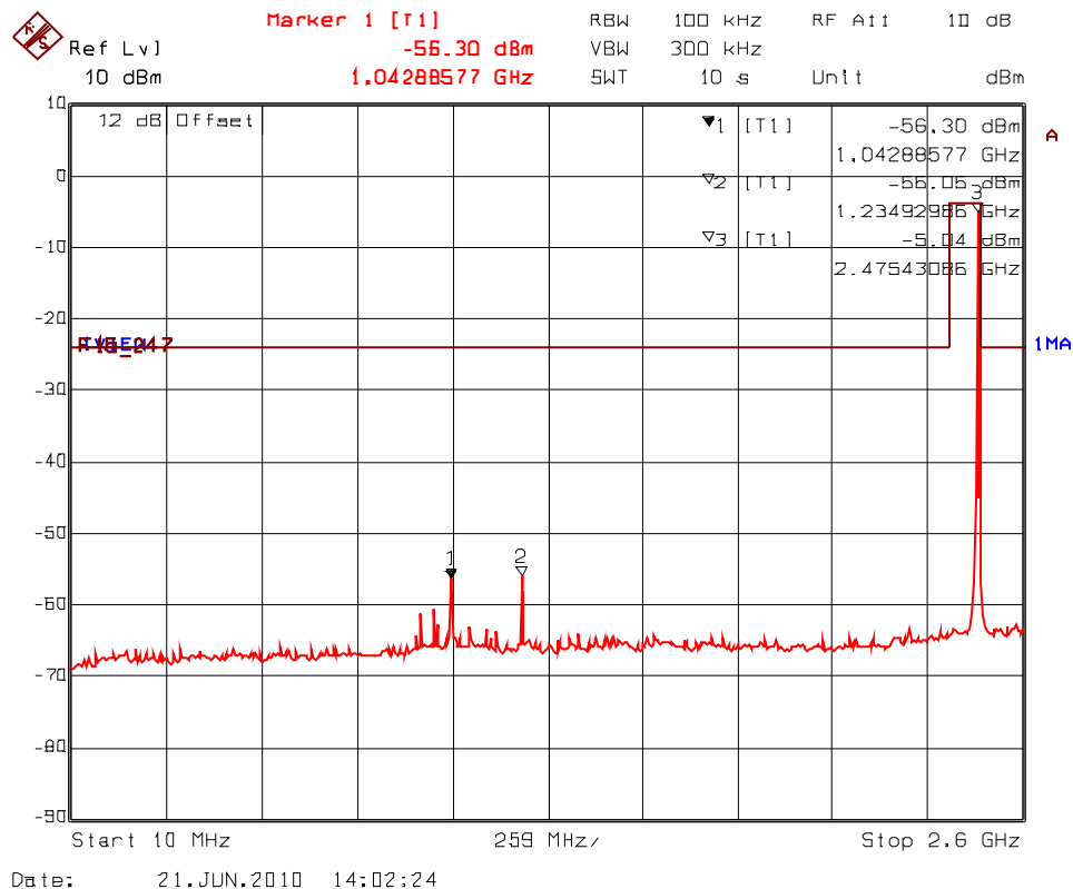
Plot 5.8.4.2.13. Spurious RF Conducted Emissions Transmitter Frequency: 2475 MHz, Low Power
