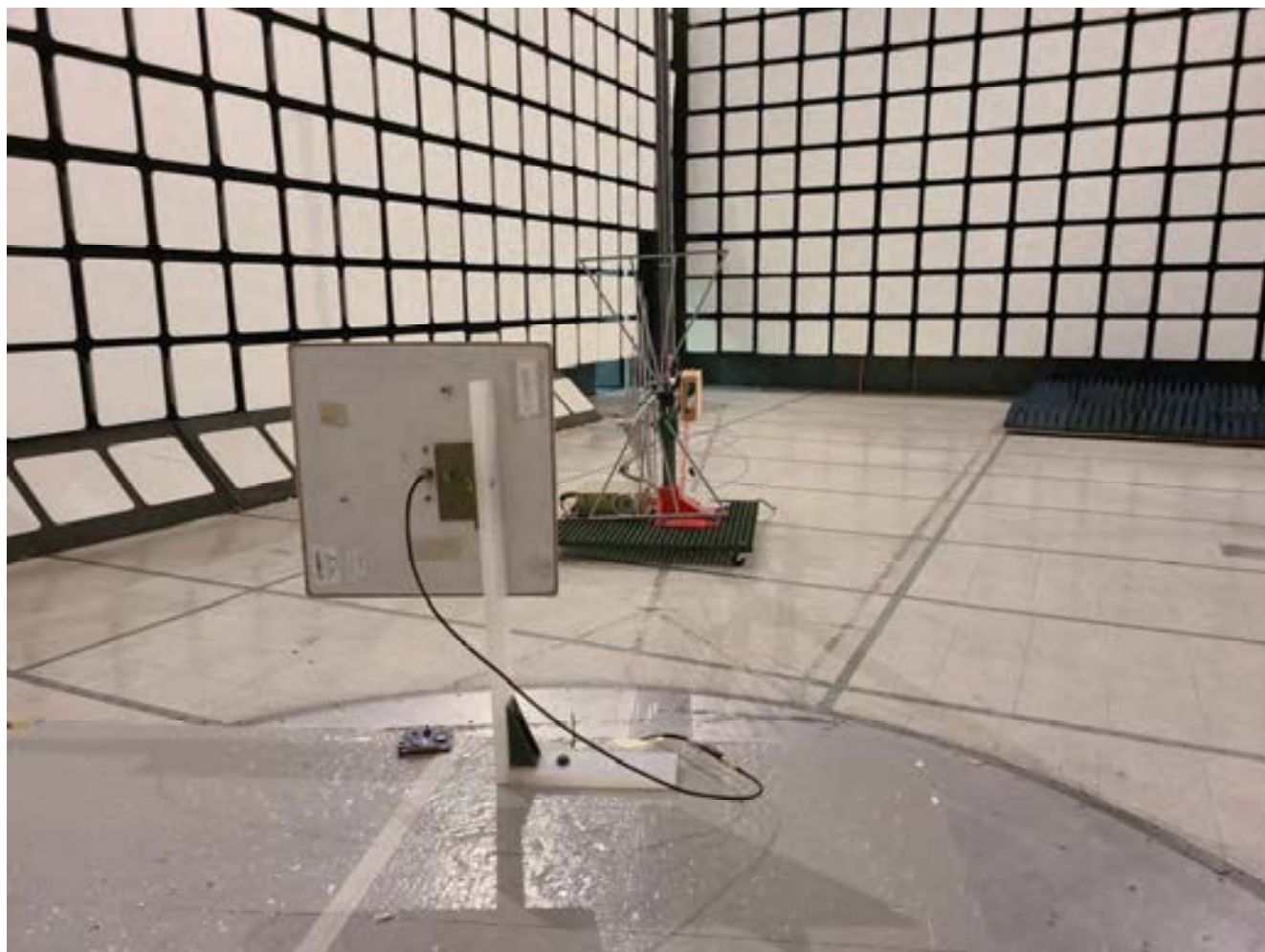
Radiated Emissions @ 3 m EUT with 19 dBi Panel Antenna, Orthogonal Position 1
