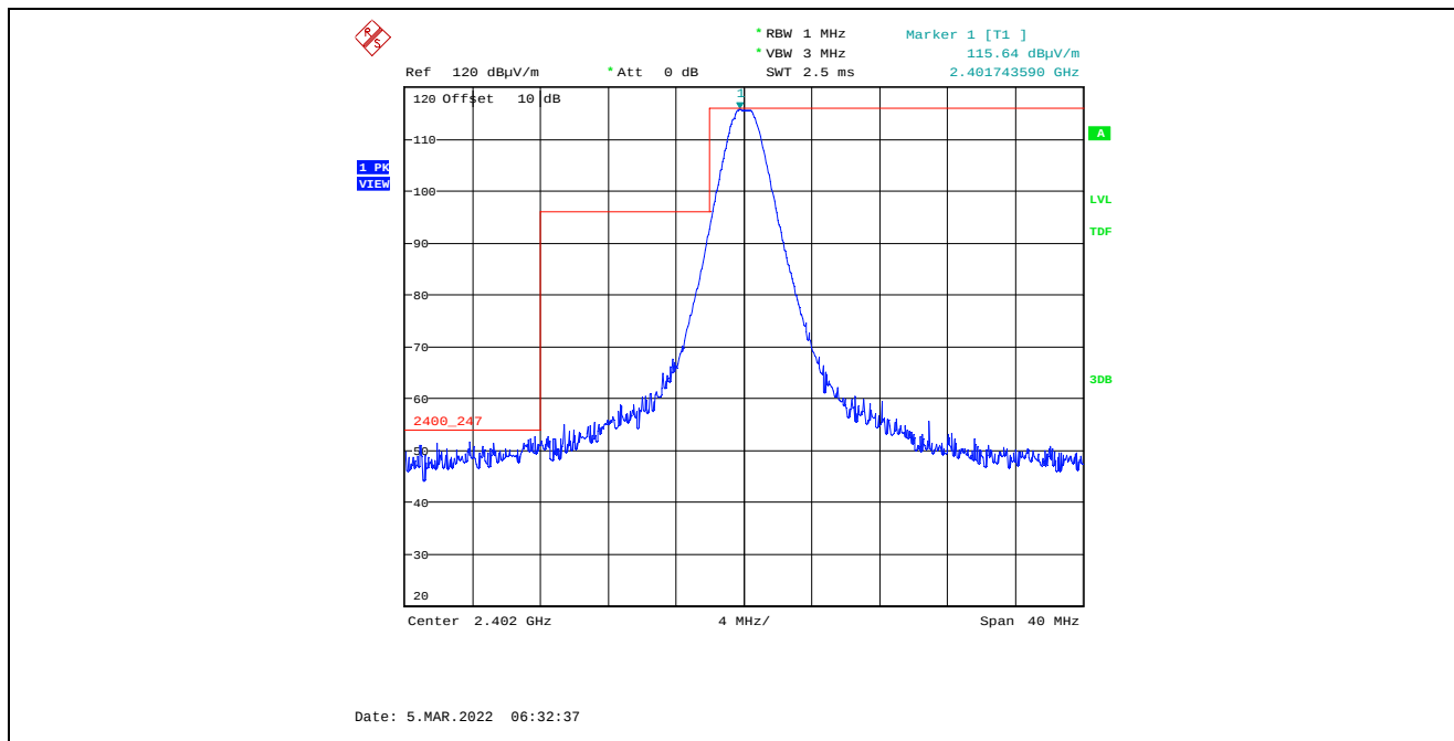
Plot 5.4.4.4.2.1. Band-Edge RF Radiated Emissions at 3 m, Horizontal Polarization, Peak Low End of Frequency Band, 2402 MHz, 8 dBm Power Setting, 1 Mbps
