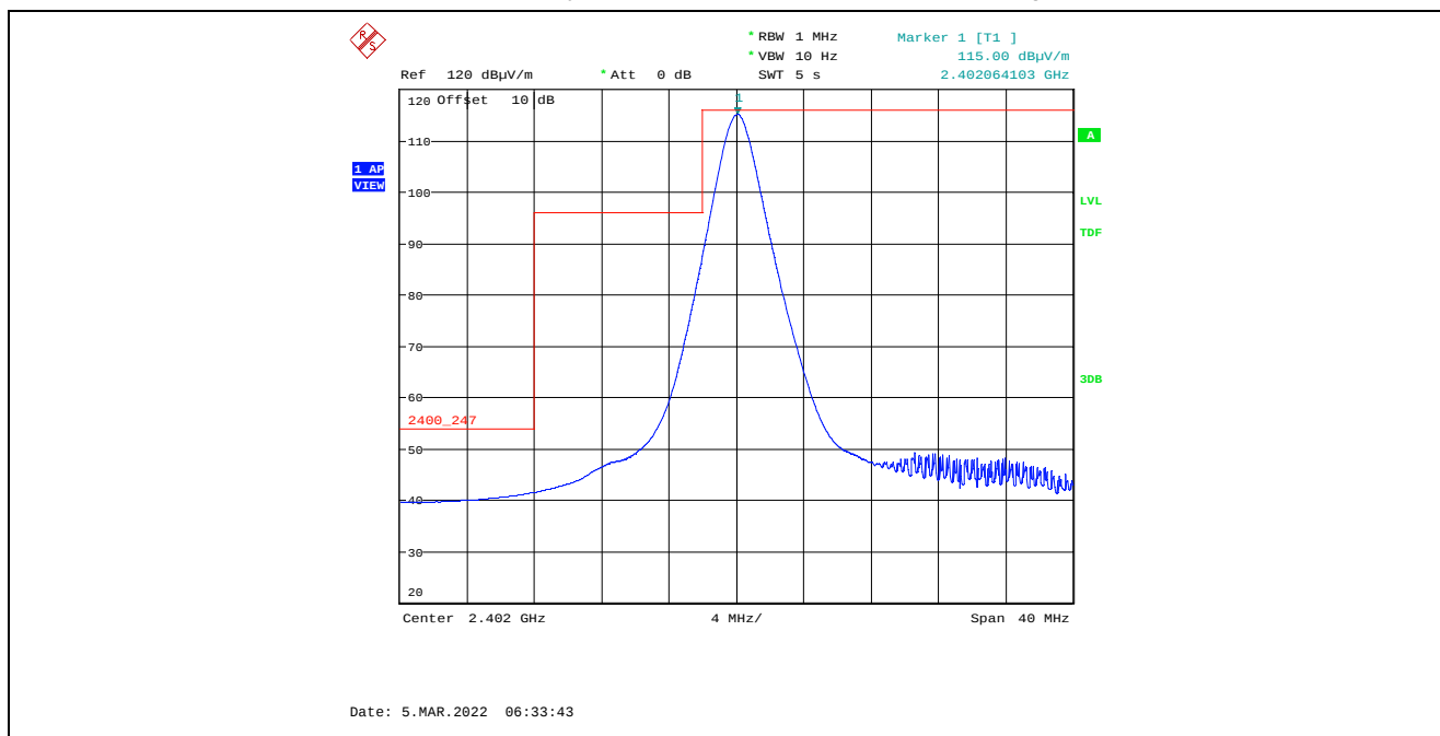
Plot 5.4.4.4.2.2. Band-Edge RF Radiated Emissions at 3 m, Horizontal Polarization, Average Low End of Frequency Band, 2402 MHz, 8 dBm Power Setting, 1 Mbps
