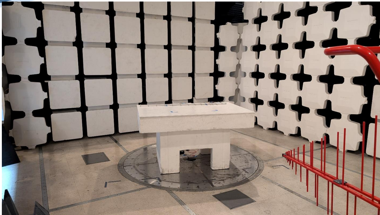
Spurious Emissions Below 1GHz
