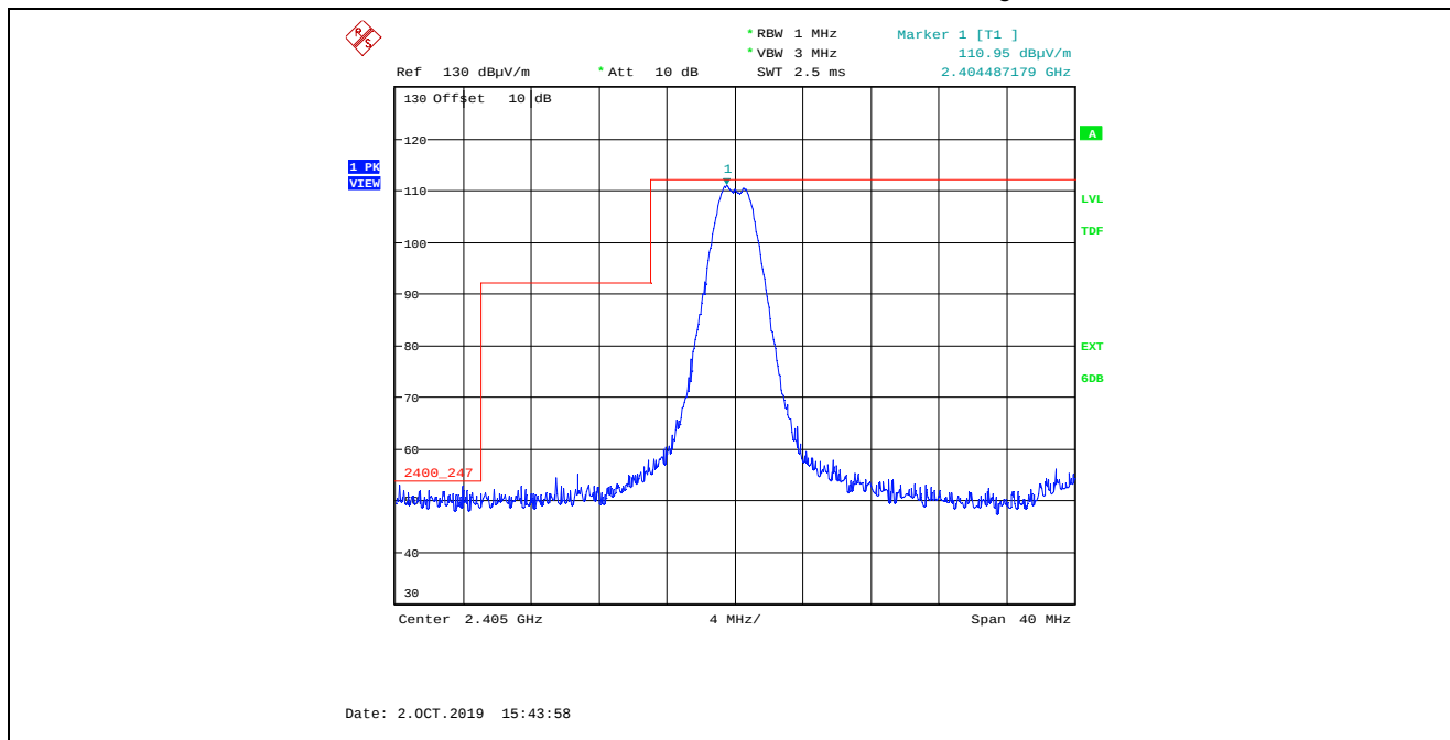
Plot 5.2.4.2.1. Band-Edge Radiated Emissions, Lower Band-edge, Peak Detector Rx Antenna in Vertical Polarization, QPSK Modulation, Power Setting 20, Ch 11, 2405 MHz
