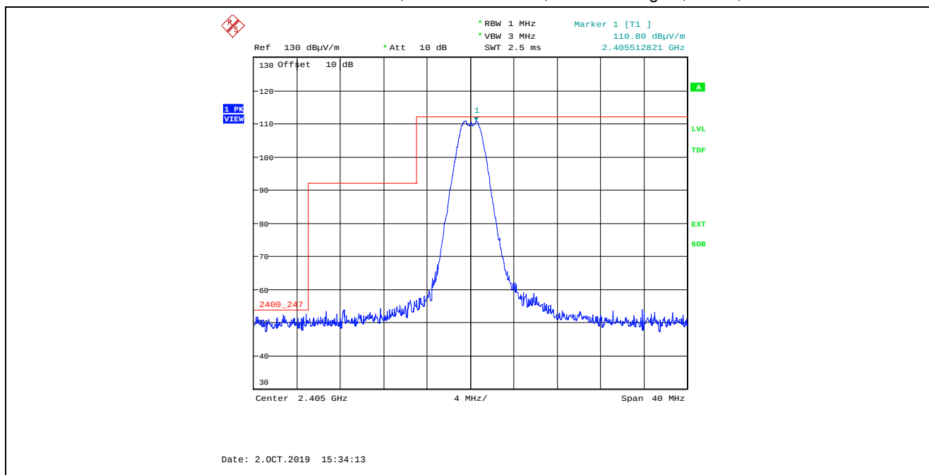
Plot 5.2.4.2.2. Band-Edge Radiated Emissions, Lower Band-edge, Peak Detector Rx Antenna in Horizontal Polarization, QPSK Modulation, Power Setting 20, Ch 20, 2405 MHz
