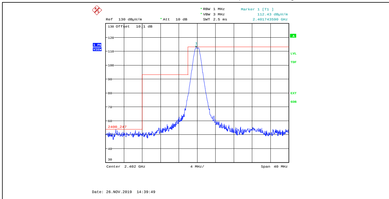
Plot 5.2.4.2.1. Band-Edge Radiated Emissions, Lower Band- edge, Peak Detector Rx Antenna in Vertical Polarization, GFSK Modulation, 1 Mbps, Power Setting 200, 2402 MHz
