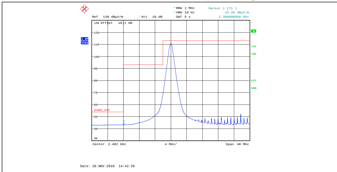
Plot 5.2.4.2.2. Band-Edge Radiated Emissions, Lower Band- edge, Average Detector Rx Antenna in Vertical Polarization, GFSK Modulation, 1 Mbps, Power Setting 200, 2402 MHz
