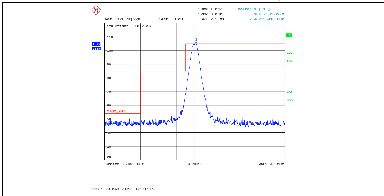
Plot 5.2.4.2.1. Band-Edge Radiated Emissions, Lower Band- edge, Peak Detector Rx Antenna in Vertical Polarization, GFSK Modulation, 1 Mbps, Power Setting 90, Ch 00, 2402 MHz
