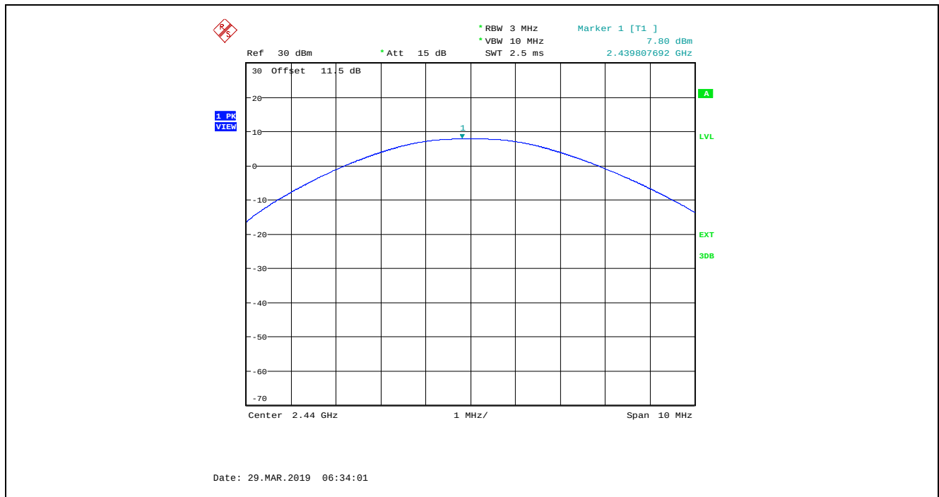
Plot 5.1.4.5. Maximum Peak Conducted Output Power, GFSK Modulation, Power Setting 90, 2 Mbps, Ch 19, 2440 MHz
