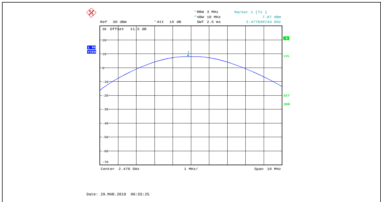
Plot 5.1.4.6. Maximum Peak Conducted Output Power, GFSK Modulation, Power Setting 90, 2 Mbps, Ch 38, 2478 MHz
