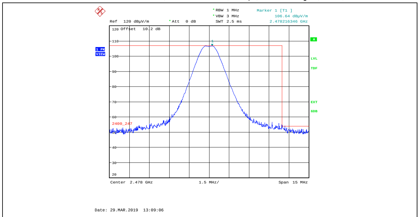
Plot 5.2.4.2.10. Band-Edge Radiated Emissions, Higher Band-edge, Peak Detector Rx Antenna in Horizontal Polarization, GFSK Modulation, 2 Mbps, Power Setting 90, Ch 38, 2478 MHz
