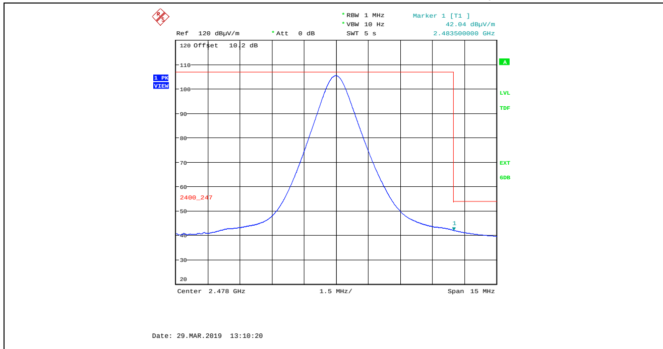
Plot 5.2.4.2.11. Band-Edge Radiated Emissions, Higher Band- edge, Average Detector Rx Antenna in Horizontal Polarization, GFSK Modulation, 2 Mbps, Power Setting 90, Ch 38, 2478 MHz
