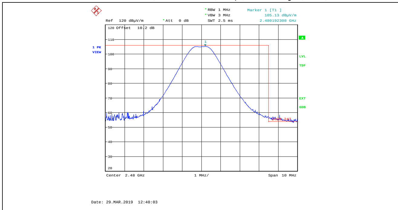
Plot 5.2.4.2.3. Band-Edge Radiated Emissions, Higher Band-edge, Peak Detector Rx Antenna in Vertical Polarization, GFSK Modulation, 1 Mbps, Power Setting 90, Ch 39, 2480 MHz
