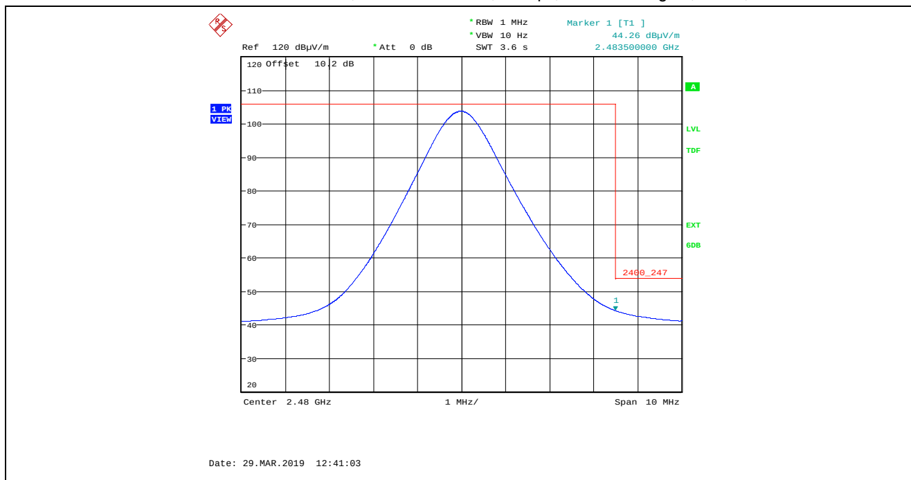
Plot 5.2.4.2.4. Band-Edge Radiated Emissions, Higher Band-edge, Average Detector Rx Antenna in Vertical Polarization, GFSK Modulation, 1 Mbps, Power Setting 90, Ch 39, 2480 MHz
