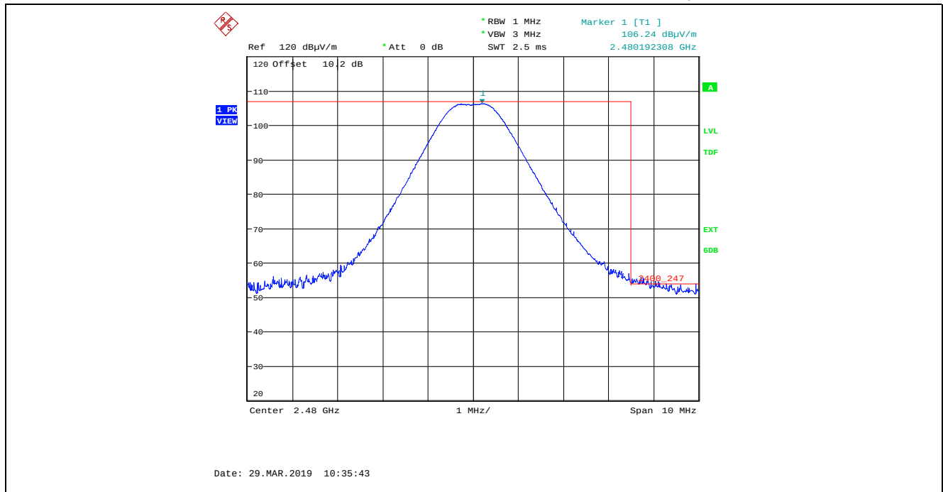
Plot 5.2.4.2.5. Band-Edge Radiated Emissions, Higher Band-edge, Peak Detector Rx Antenna in Horizontal Polarization, GFSK Modulation, 1 Mbps, Power Setting 90, Ch 39, 2480 MHz
