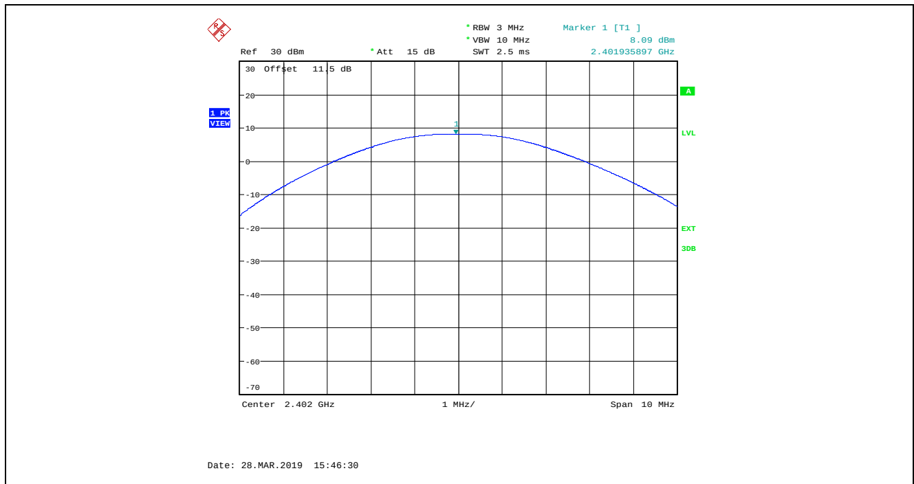
Plot 5.1.4.1. Maximum Peak Conducted Output Power, GFSK Modulation, Power Setting 90, 1 Mbps, Ch 00, 2402 MHz
