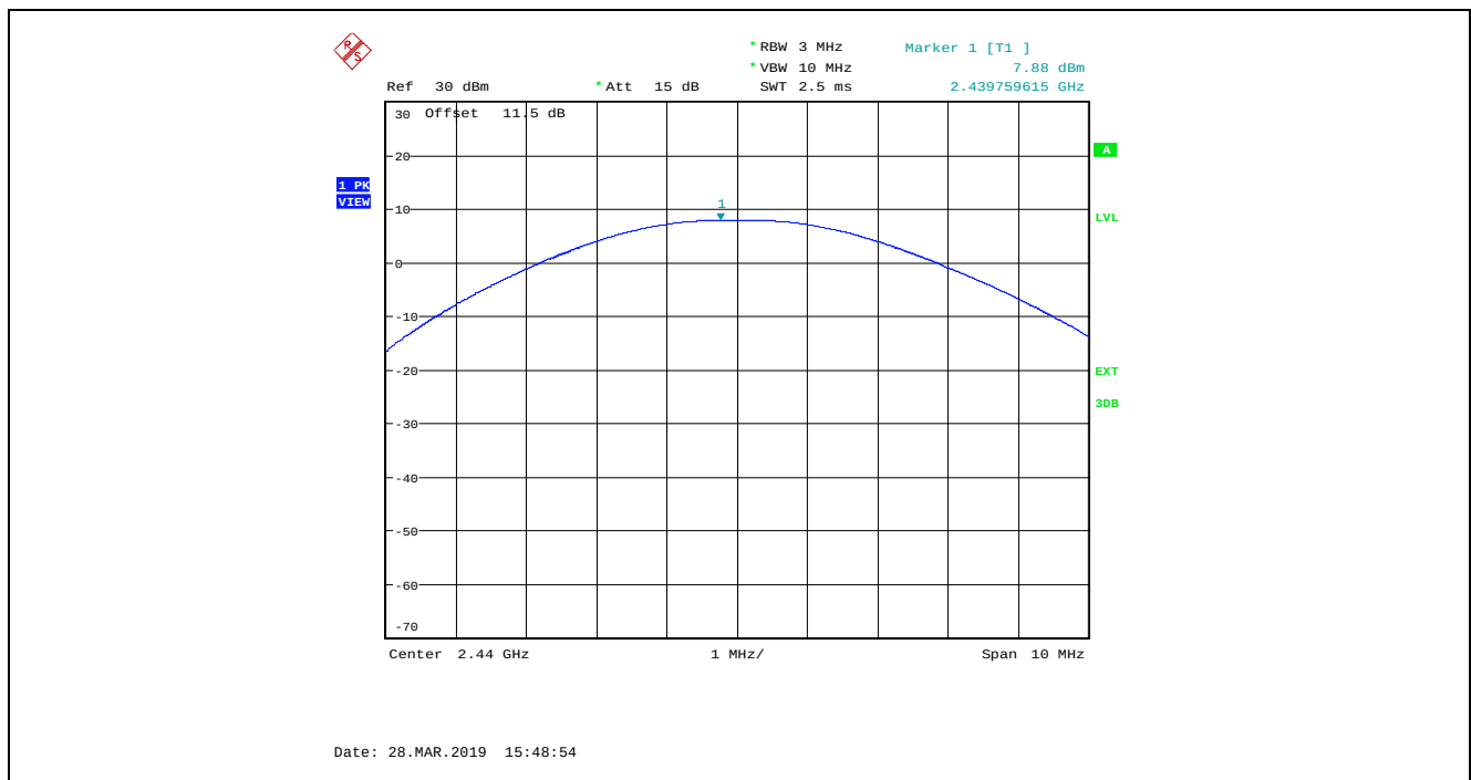
Plot 5.1.4.2. Maximum Peak Conducted Output Power, GFSK Modulation, Power Setting 90, 1 Mbps, Ch 19, 2440 MHz
