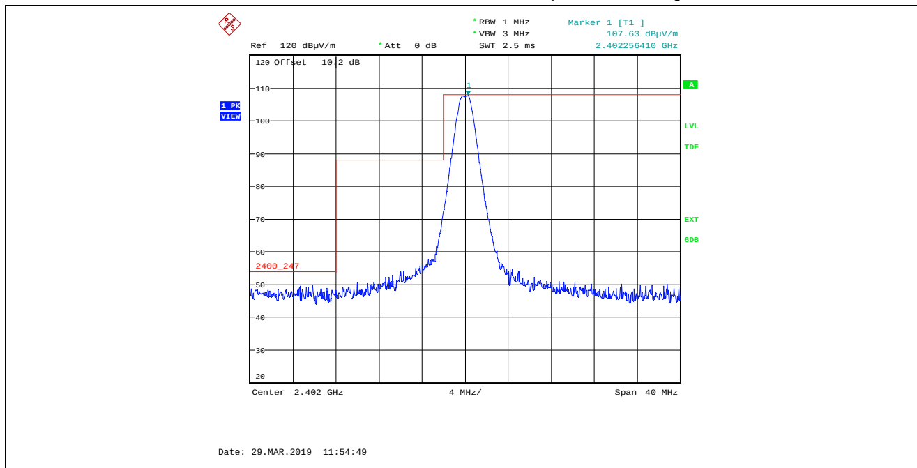
Plot 5.2.4.2.2. Band-Edge Radiated Emissions, Lower Band-edge, Peak Detector Rx Antenna in Horizontal Polarization, GFSK Modulation, 1 Mbps, Power Setting 90, Ch 00, 2402 MHz
