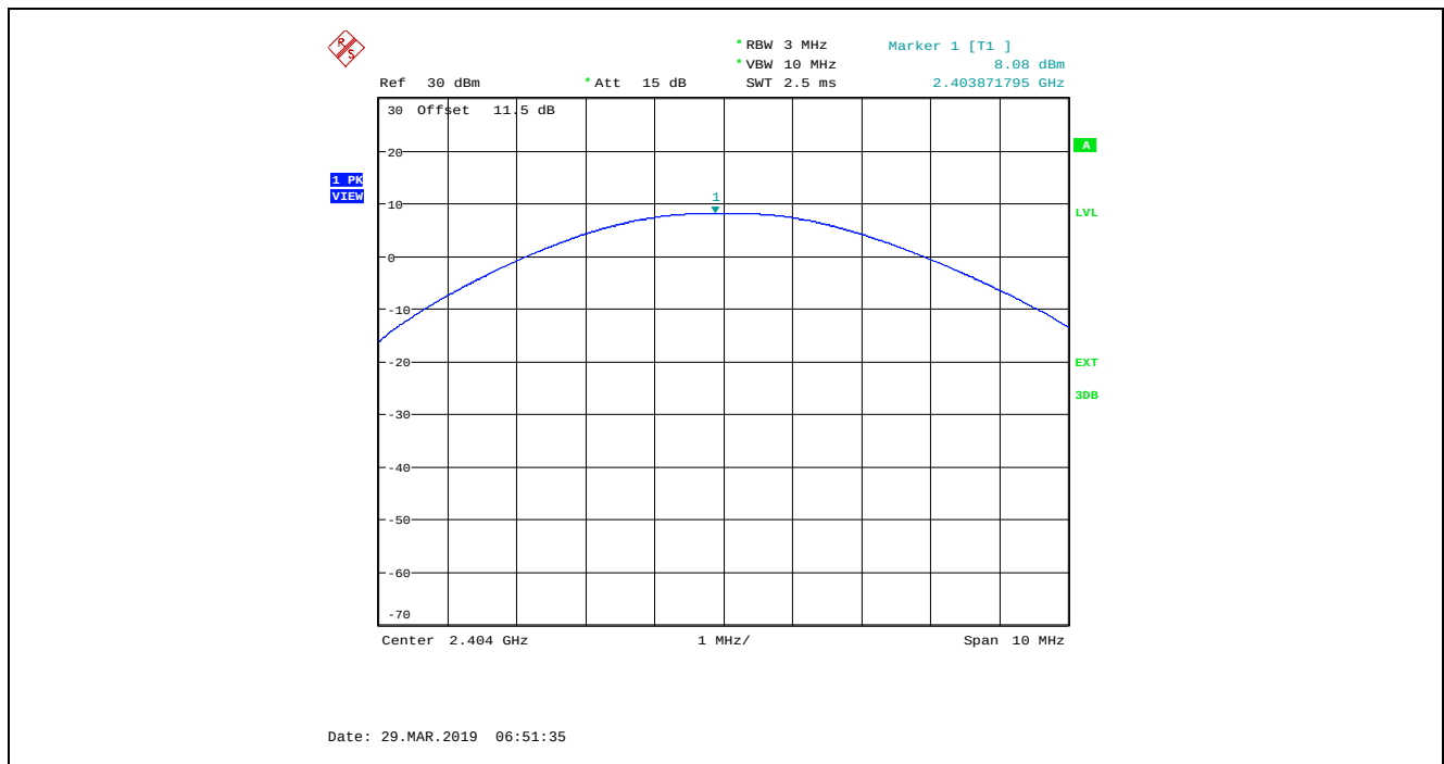
Plot 5.1.4.4. Maximum Peak Conducted Output Power, GFSK Modulation, Power Setting 90, 2 Mbps, Ch 01, 2404 MHz
