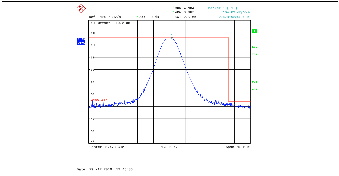
Plot 5.2.4.2.9. Band-Edge Radiated Emissions, Higher Band-edge, Peak Detector Rx Antenna in Vertical Polarization, GFSK Modulation, 2 Mbps, Power Setting 90, Ch 38, 2478 MHz
