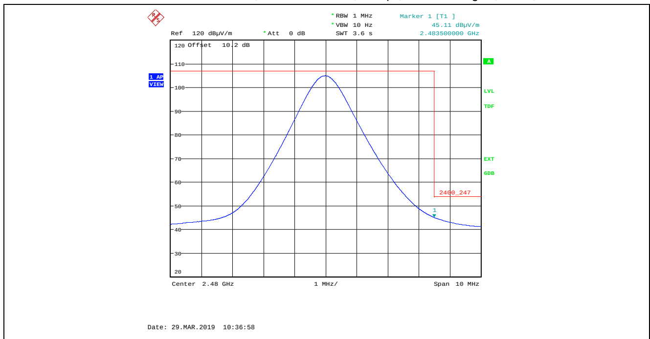
Plot 5.2.4.2.6. Band-Edge Radiated Emissions, Higher Band-edge, Average Detector Rx Antenna in Horizontal Polarization, GFSK Modulation, 1 Mbps, Power Setting 90, Ch 39, 2480 MHz
