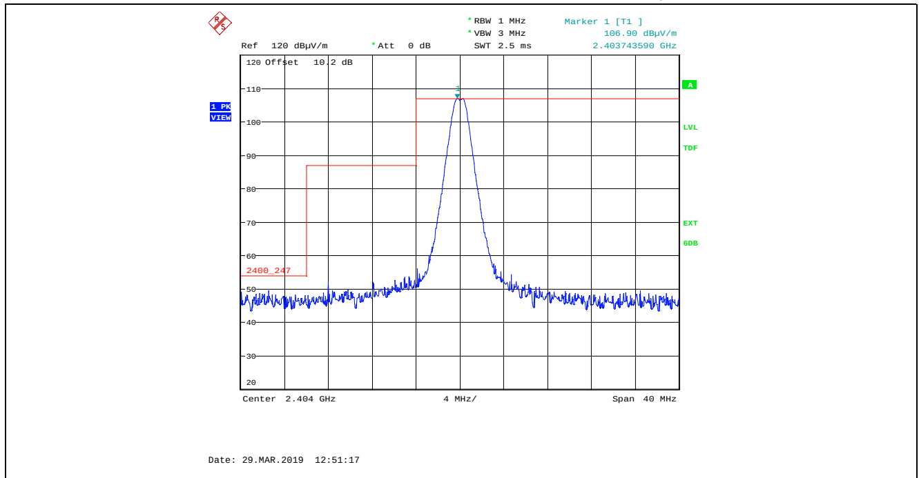
Plot 5.2.4.2.7. Band-Edge Radiated Emissions, Lower Band-edge, Peak Detector Rx Antenna in Vertical Polarization, GFSK Modulation, 2 Mbps, Power Setting 90, Ch 01, 2404 MHz
