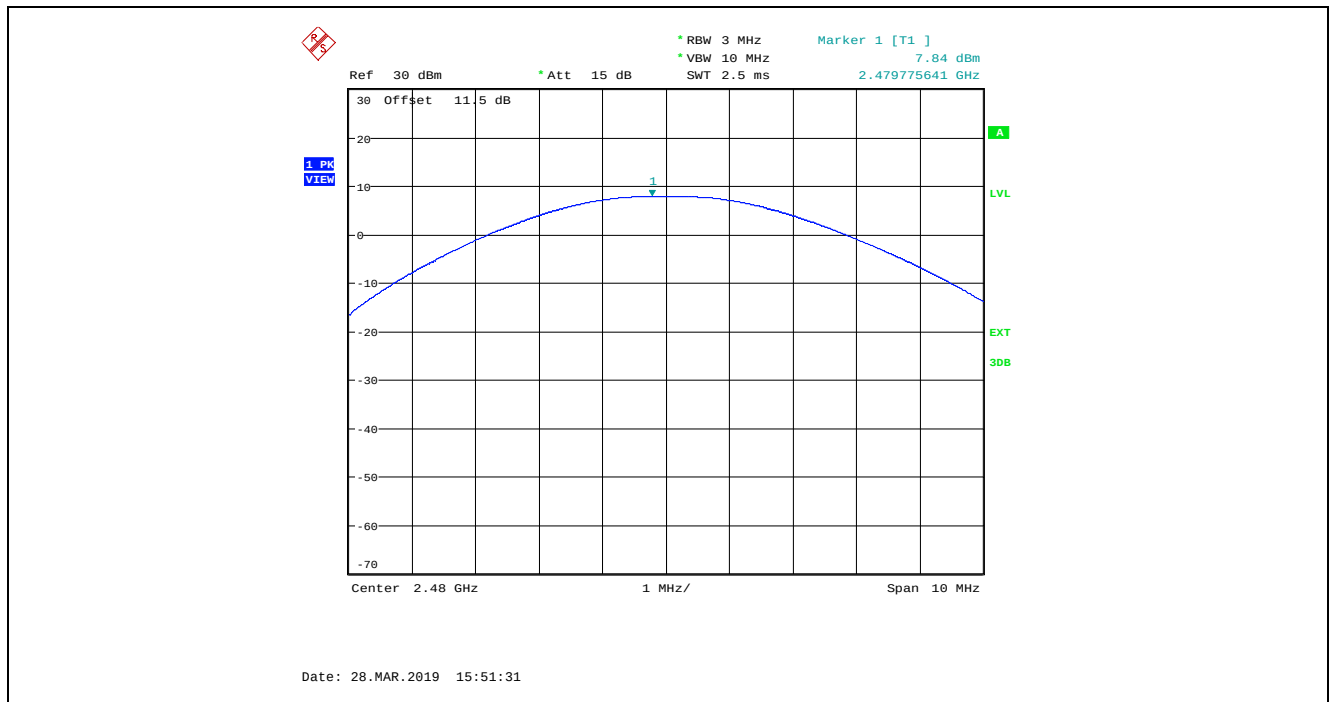
Plot 5.1.4.3. Maximum Peak Conducted Output Power, GFSK Modulation, Power Setting 90, 1 Mbps, Ch 39, 2480 MHz
