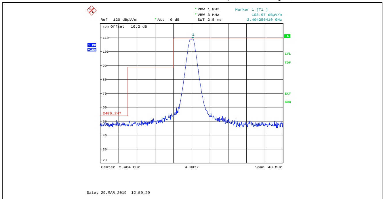
Plot 5.2.4.2.8. Band-Edge Radiated Emissions, Lower Band- edge, Peak Detector Rx Antenna in Horizontal Polarization, GFSK Modulation, 2 Mbps, Power Setting 90, Ch 01, 2404 MHz
