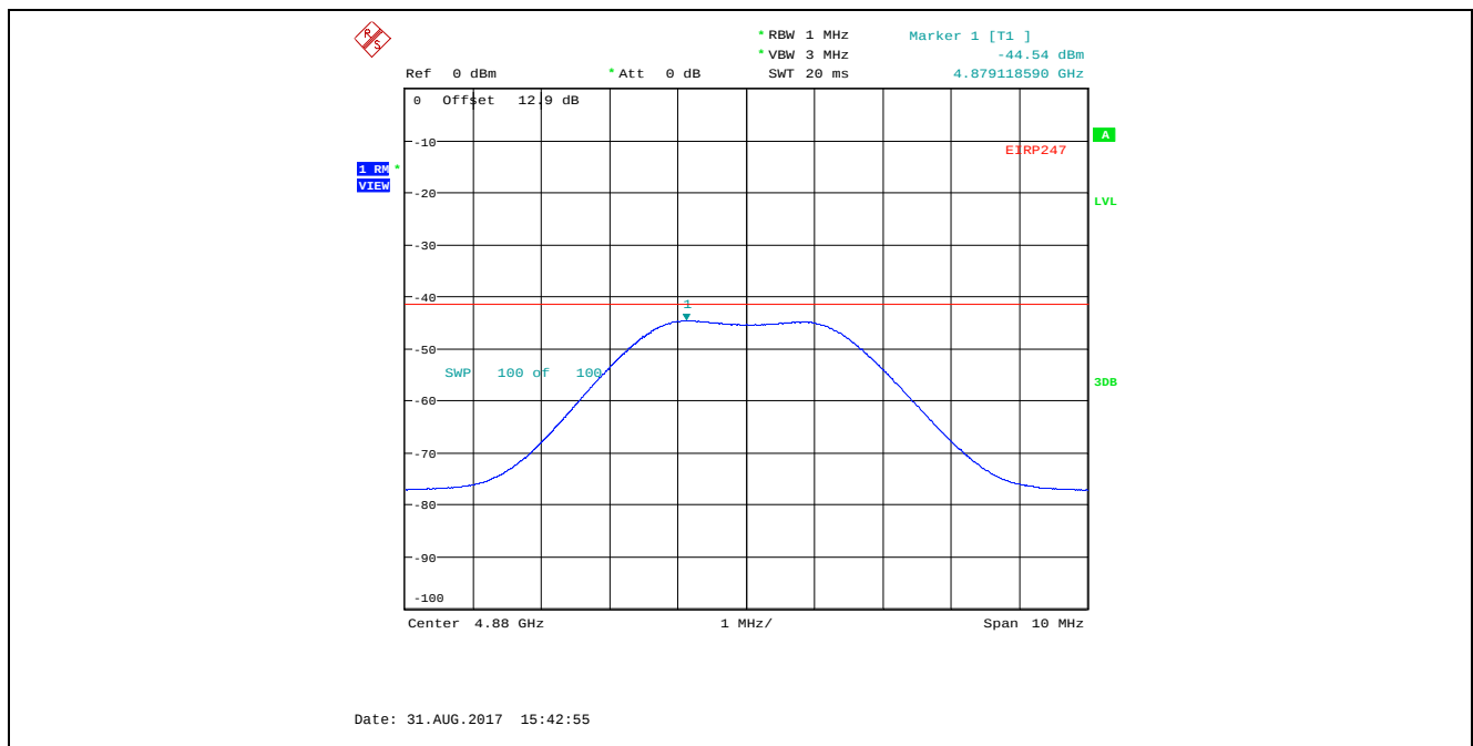
Plot 5.4.4.3.30. Conducted Spurious Emissions in Restricted Frequency Bands, High Power 2440 MHz, GFSK Modulation, 2 Mbps, Marker 1, Trace Averaging RMS Detector
