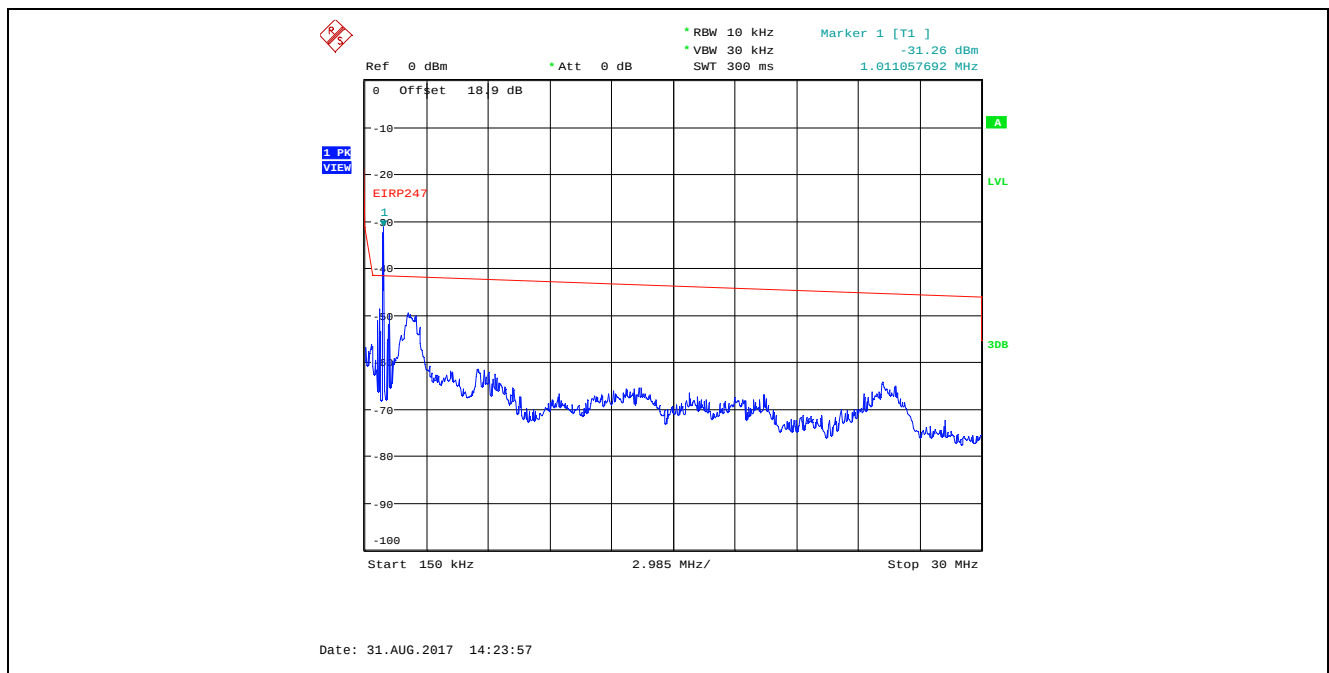
Plot 5.4.4.3.14. Conducted Spurious Emissions in Restricted Frequency Bands, High Power 2480 MHz, GFSK Modulation, 1 Mbps, 150 kHz - 30 MHz, Peak Detector Marker 1 is Outside of the Restricted Bands
