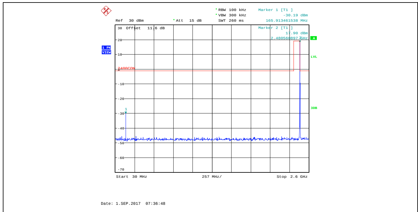
Plot 5.4.4.2.5. Conducted Spurious Emissions in Non-Restricted Frequency Bands, High Power 2480 MHz, GFSK Modulation, 1 Mbps, 30 MHz – 2.6 GHz, Peak Detector
