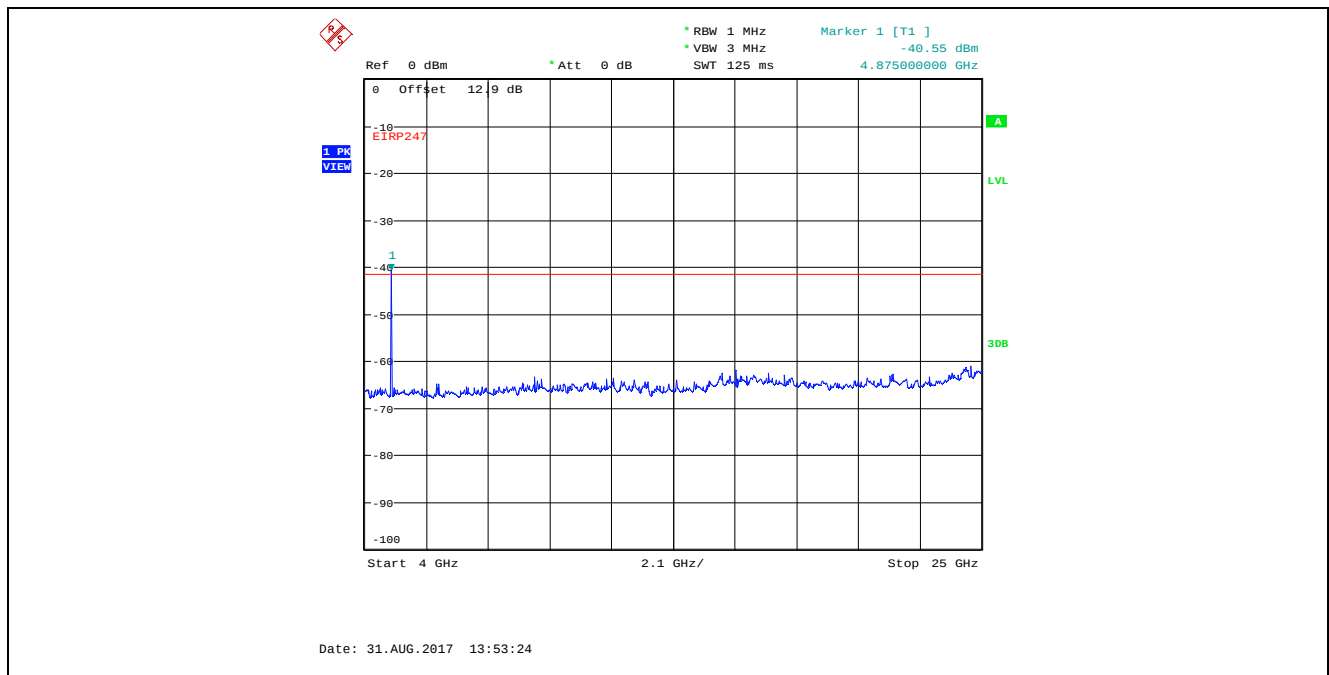
Plot 5.4.4.3.11. Conducted Spurious Emissions in Restricted Frequency Bands, High Power 2440 MHz, GFSK Modulation, 1 Mbps, 4 GHz - 25 GHz, Peak Detector
