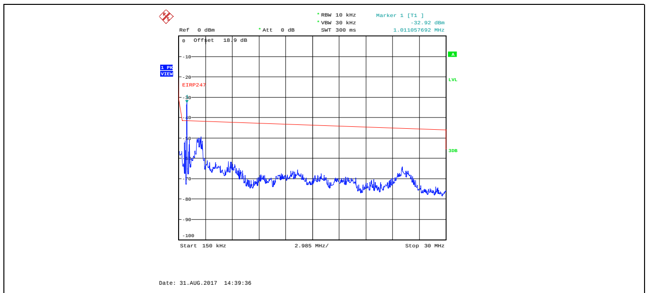
Plot 5.4.4.3.2. Conducted Spurious Emissions in Restricted Frequency Bands, High Power 2402 MHz, GFSK Modulation, 1 Mbps, 150 kHz - 30 MHz, Peak Detector Marker 1 is Outside of the Restricted Bands
