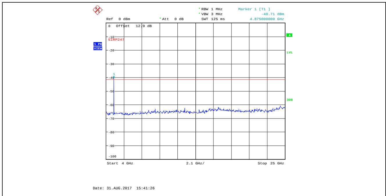
Plot 5.4.4.3.29. Conducted Spurious Emissions in Restricted Frequency Bands, High Power 2440 MHz, GFSK Modulation, 2 Mbps, 4 GHz - 25 GHz, Peak Detector
