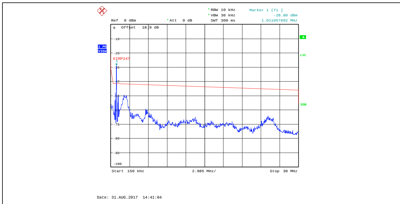
Plot 5.4.4.3.8. Conducted Spurious Emissions in Restricted Frequency Bands, High Power 2440 MHz, GFSK Modulation, 1 Mbps, 150 kHz - 30 MHz, Peak Detector Marker 1 is Outside of the Restricted Bands
