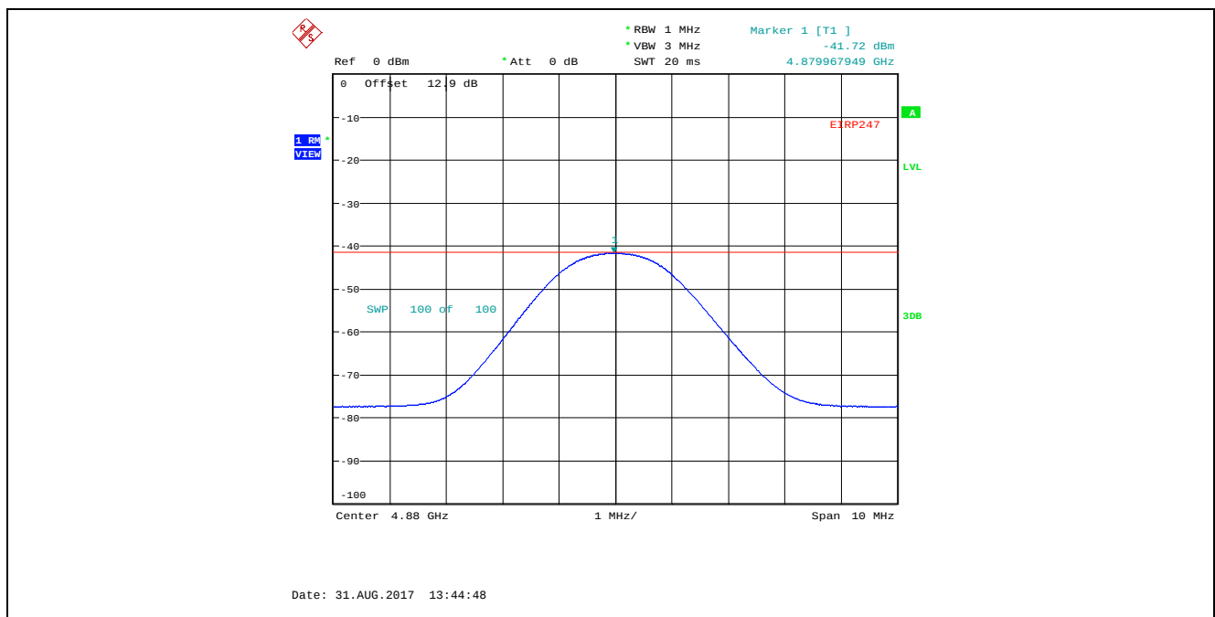
Plot 5.4.4.3.12. Conducted Spurious Emissions in Restricted Frequency Bands, High Power 2440 MHz, GFSK Modulation, 1 Mbps, Marker 1 (-41.72 dBm < -41.26 dBm Limit), Trace Averaging RMS Detector
