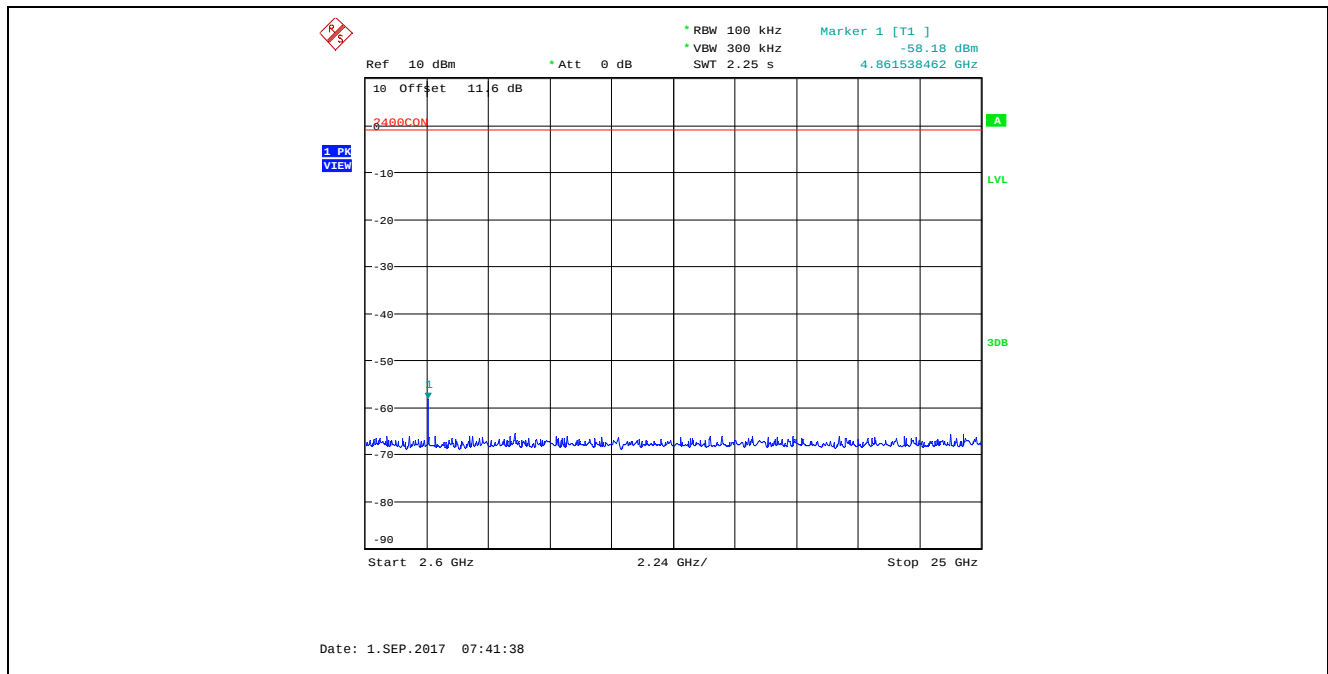
Plot 5.4.4.2.4. Conducted Spurious Emissions in Non-Restricted Frequency Bands, High Power 2440 MHz, GFSK Modulation, 1 Mbps, 2.6 GHz – 25 GHz, Peak Detector
