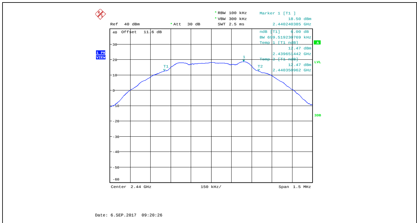
Plot 5.2.4.2. 6 dB Bandwidth, GFSK Modulation, Power Setting at 200, Channel 19, 2440 MHz, 1 Mbps
