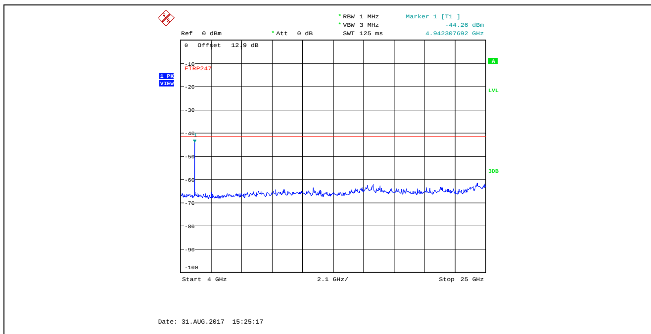
Plot 5.4.4.3.35. Conducted Spurious Emissions in Restricted Frequency Bands, High Power 2480 MHz, GFSK Modulation, 2 Mbps, 4 GHz - 25 GHz, Peak Detector
