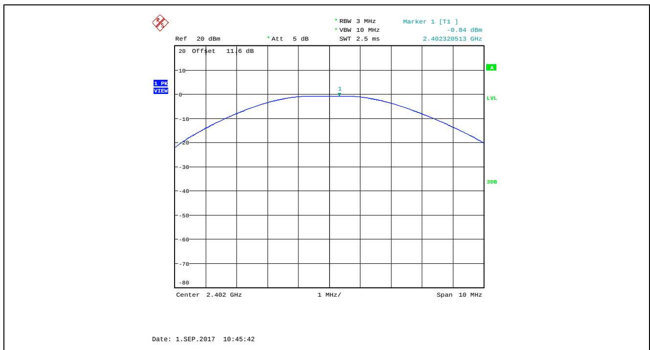
Plot 5.3.4.10. Maximum Peak Conducted Output Power, GFSK Modulation, Low Power, 2 Mbps, Ch 00, 2402 MHz
