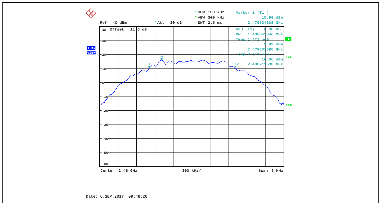
Plot 5.2.4.6. 6 dB Bandwidth, GFSK Modulation, Power Setting at 200, Channel 39, 2480 MHz, 2 Mbps
