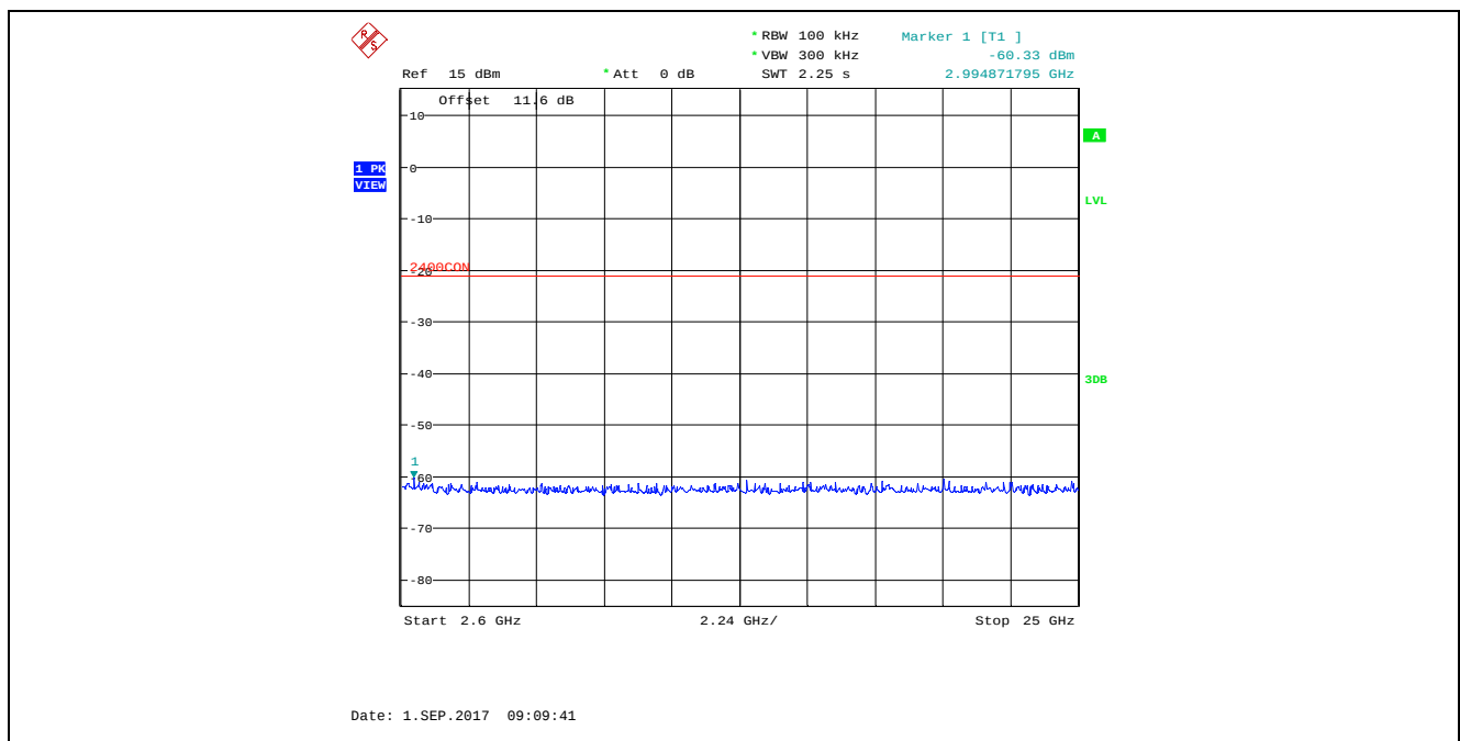
Plot 5.4.4.2.16. Conducted Spurious Emissions in Non-Restricted Frequency Bands, Low Power 2440 MHz, GFSK Modulation, 1 Mbps, 2.6 GHz – 25 GHz, Peak Detector
