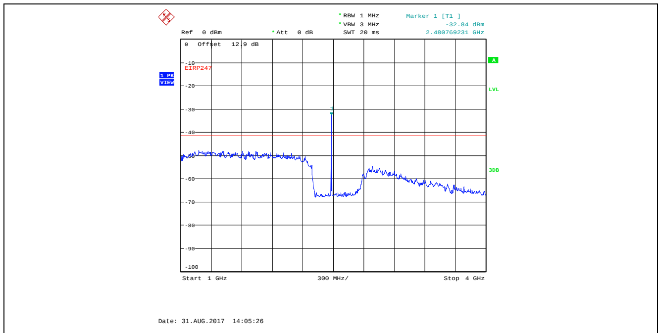
Plot 5.4.4.3.16. Conducted Spurious Emissions in Restricted Frequency Bands, High Power 2480 MHz, GFSK Modulation, 1 Mbps, 1 GHz - 4 GHz, Peak Detector Marker 1 is the Fundamental Frequency
