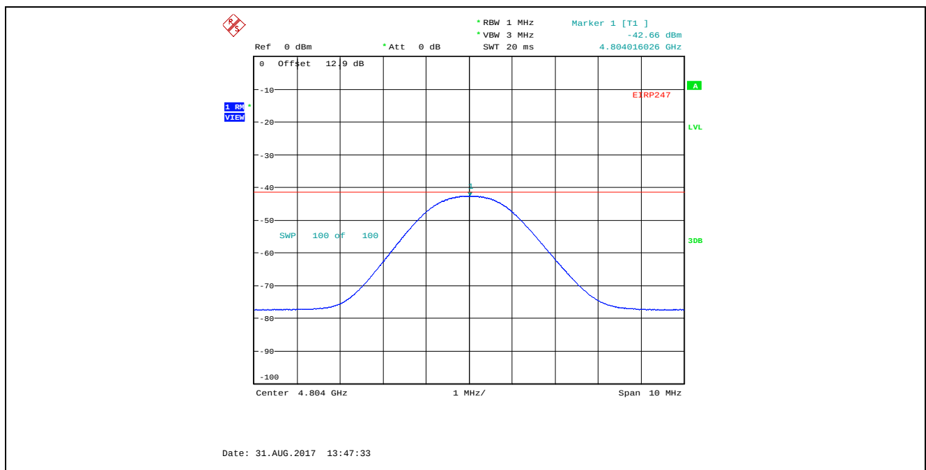
Plot 5.4.4.3.6. Conducted Spurious Emissions in Restricted Frequency Bands, High Power 2402 MHz, GFSK Modulation, 1 Mbps, Marker 1, Trace Averaging RMS Detector
