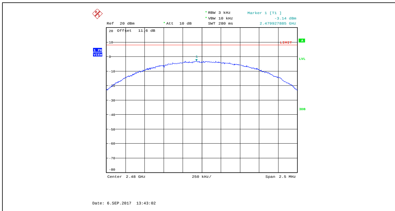
Plot 5.6.4.6. Power Spectral Density, GFSK Modulation, High Power, Channel 39, 2480 MHz, 2 Mbps
