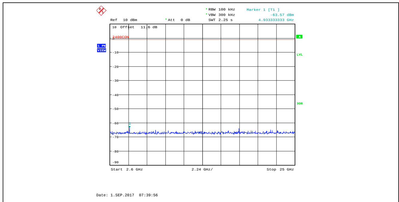
Plot 5.4.4.2.6. Conducted Spurious Emissions in Non-Restricted Frequency Bands, High Power 2480 MHz, GFSK Modulation, 1 Mbps, 2.6 GHz – 25 GHz, Peak Detector
