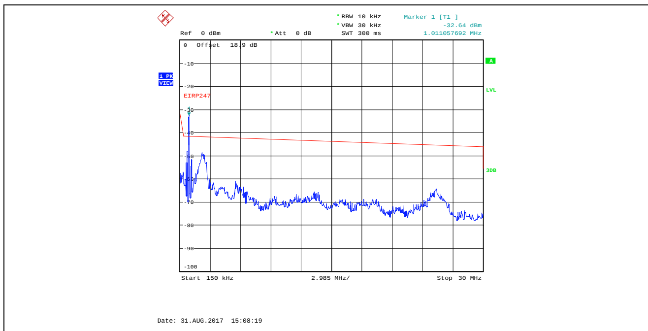
Plot 5.4.4.3.32. Conducted Spurious Emissions in Restricted Frequency Bands, High Power 2480 MHz, GFSK Modulation, 2 Mbps, 150 kHz - 30 MHz, Peak Detector Marker 1 is Outside of the Restricted Bands
