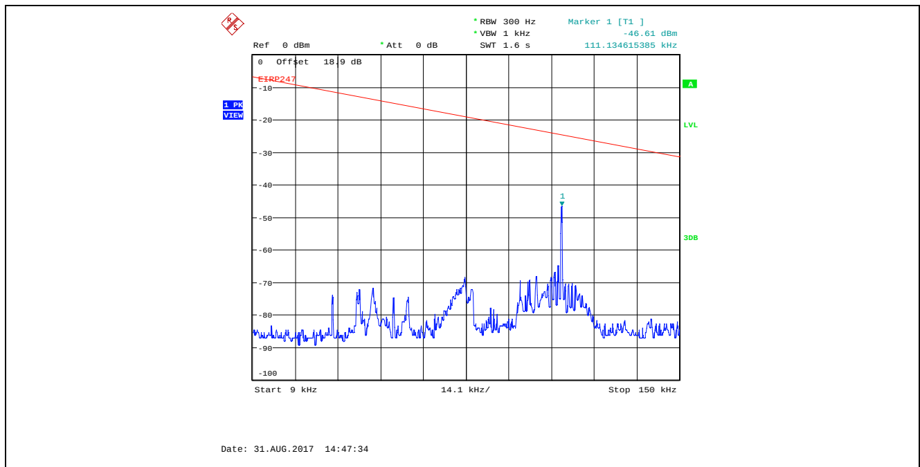
Plot 5.4.4.3.13. Conducted Spurious Emissions in Restricted Frequency Bands, High Power 2480 MHz, GFSK Modulation, 1 Mbps, 9 kHz - 150 kHz, Peak Detector
