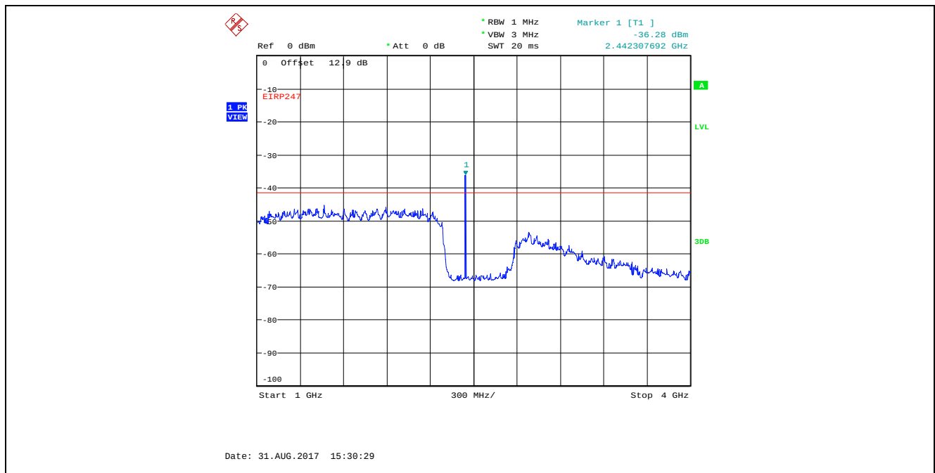
Plot 5.4.4.3.28. Conducted Spurious Emissions in Restricted Frequency Bands, High Power 2440 MHz, GFSK Modulation, 2 Mbps, 1 GHz - 4 GHz, Peak Detector Marker 1 is the Fundamental Frequency
