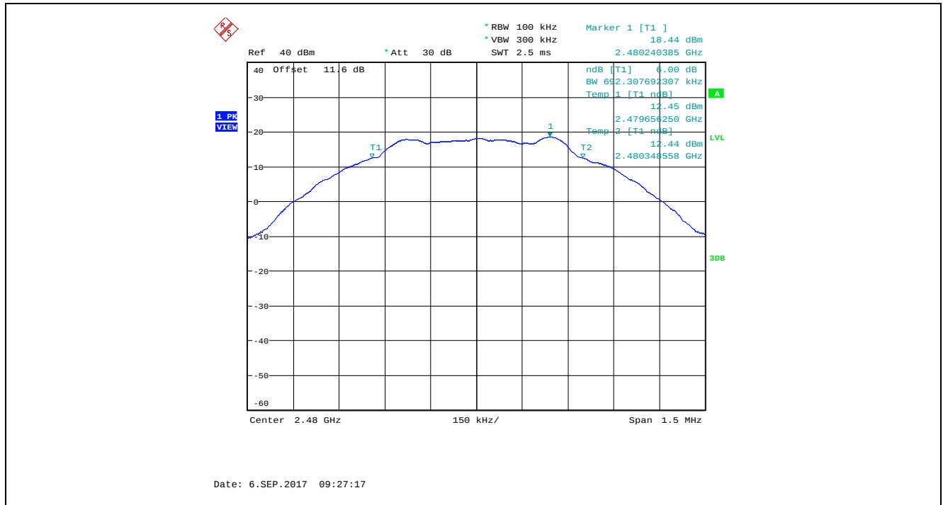
Plot 5.2.4.3. 6 dB Bandwidth, GFSK Modulation, Power Setting at 200, Channel 39, 2480 MHz, 1 Mbps
