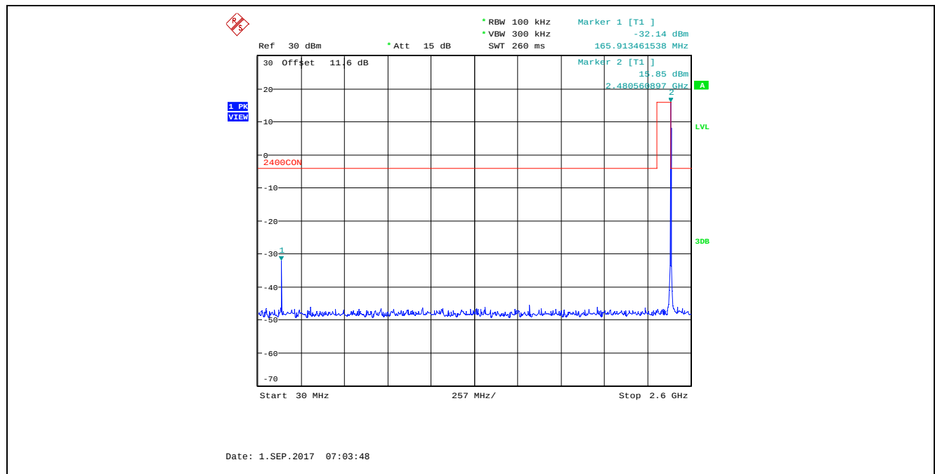
Plot 5.4.4.2.11. Conducted Spurious Emissions in Non-Restricted Frequency Bands, High Power 2480 MHz, GFSK Modulation, 2 Mbps, 30 MHz – 2.6 GHz, Peak Detector
