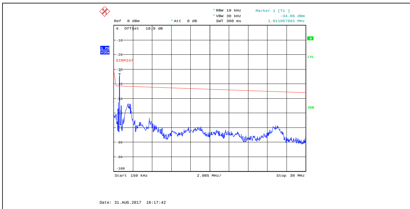
Plot 5.4.4.3.26. Conducted Spurious Emissions in Restricted Frequency Bands, High Power 2440 MHz, GFSK Modulation, 2 Mbps, 150 kHz - 30 MHz, Peak Detector Marker 1 is Outside of the Restricted Bands
