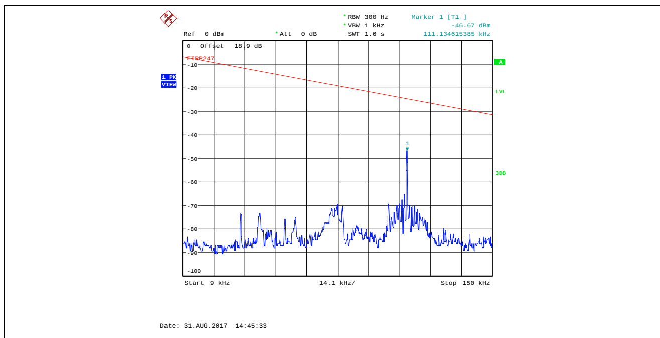
Plot 5.4.4.3.7. Conducted Spurious Emissions in Restricted Frequency Bands, High Power 2440 MHz, GFSK Modulation, 1 Mbps, 9 kHz - 150 kHz, Peak Detector
