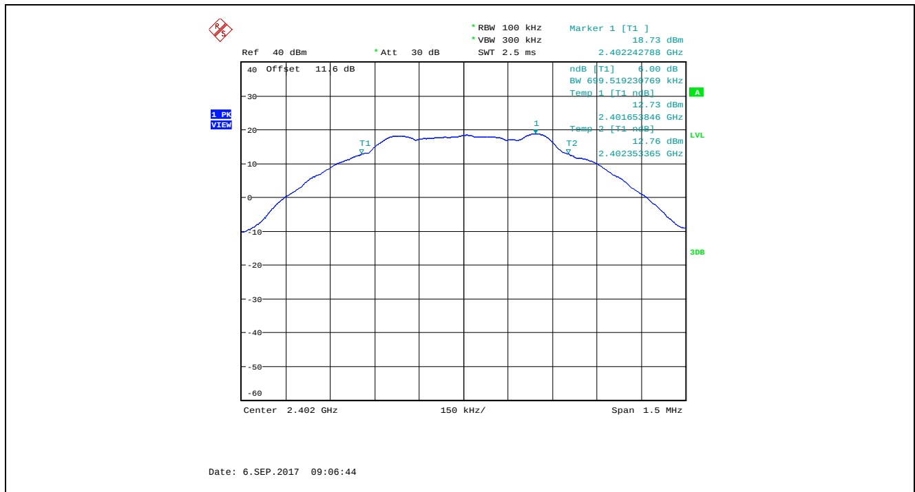
Plot 5.2.4.1. 6 dB Bandwidth, GFSK Modulation, Power Setting at 200, Channel 00, 2402 MHz, 1 Mbps
