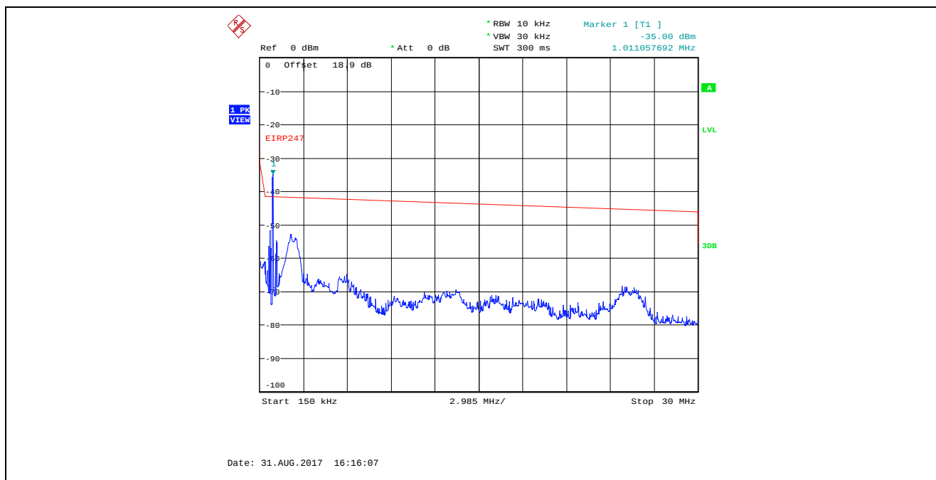
Plot 5.4.4.3.20. Conducted Spurious Emissions in Restricted Frequency Bands, High Power 2402 MHz, GFSK Modulation, 2 Mbps, 150 kHz - 30 MHz, Peak Detector Marker 1 is Outside of the Restricted Bands
