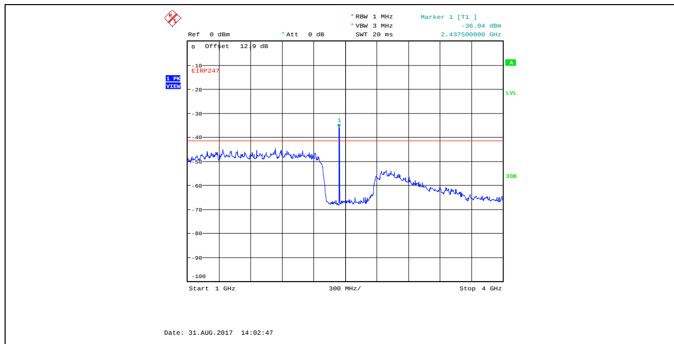
Plot 5.4.4.3.10. Conducted Spurious Emissions in Restricted Frequency Bands, High Power 2440 MHz, GFSK Modulation, 1 Mbps, 1 GHz - 4 GHz, Peak Detector Marker 1 is the Fundamental Frequency
