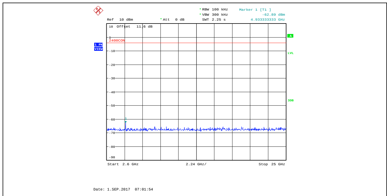
Plot 5.4.4.2.12. Conducted Spurious Emissions in Non-Restricted Frequency Bands, High Power 2480 MHz, GFSK Modulation, 2 Mbps, 2.6 GHz – 25 GHz, Peak Detector
