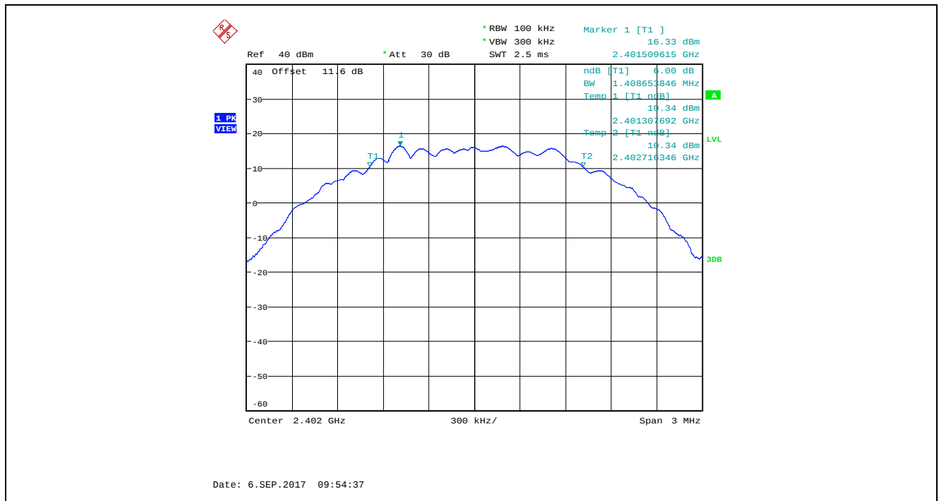
Plot 5.2.4.4. 6 dB Bandwidth, GFSK Modulation, Power Setting at 200, Channel 00, 2402 MHz, 2 Mbps
