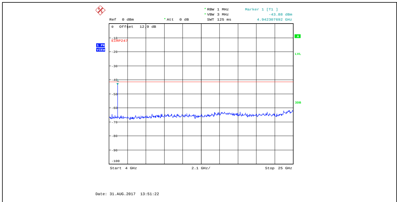
Plot 5.4.4.3.17. Conducted Spurious Emissions in Restricted Frequency Bands, High Power 2480 MHz, GFSK Modulation, 1 Mbps, 4 GHz - 25 GHz, Peak Detector
