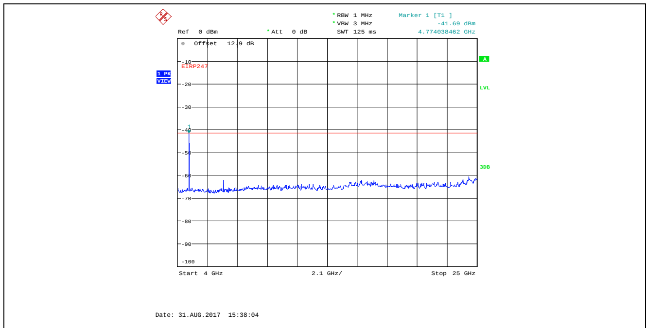
Plot 5.4.4.3.23. Conducted Spurious Emissions in Restricted Frequency Bands, High Power 2402 MHz, GFSK Modulation, 2 Mbps, 4 GHz - 25 GHz, Peak Detector
