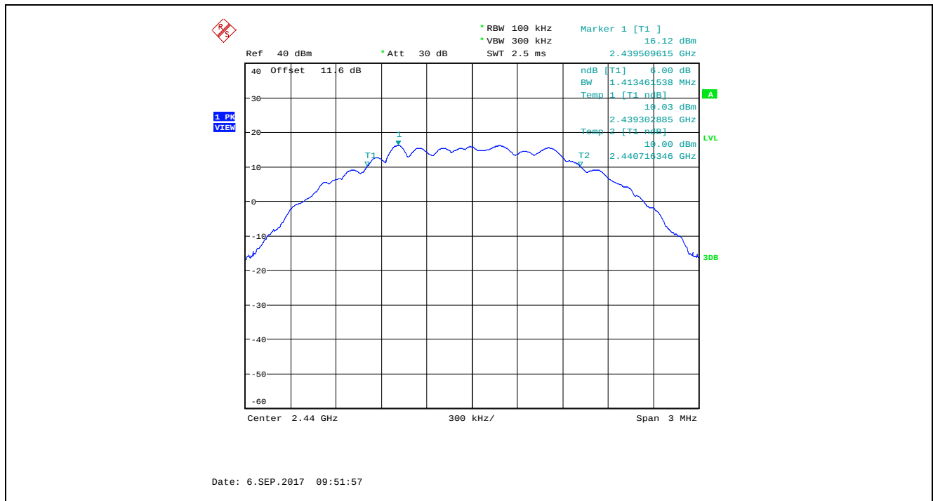
Plot 5.2.4.5. 6 dB Bandwidth, GFSK Modulation, Power Setting at 200, Channel 19, 2440 MHz, 2 Mbps
