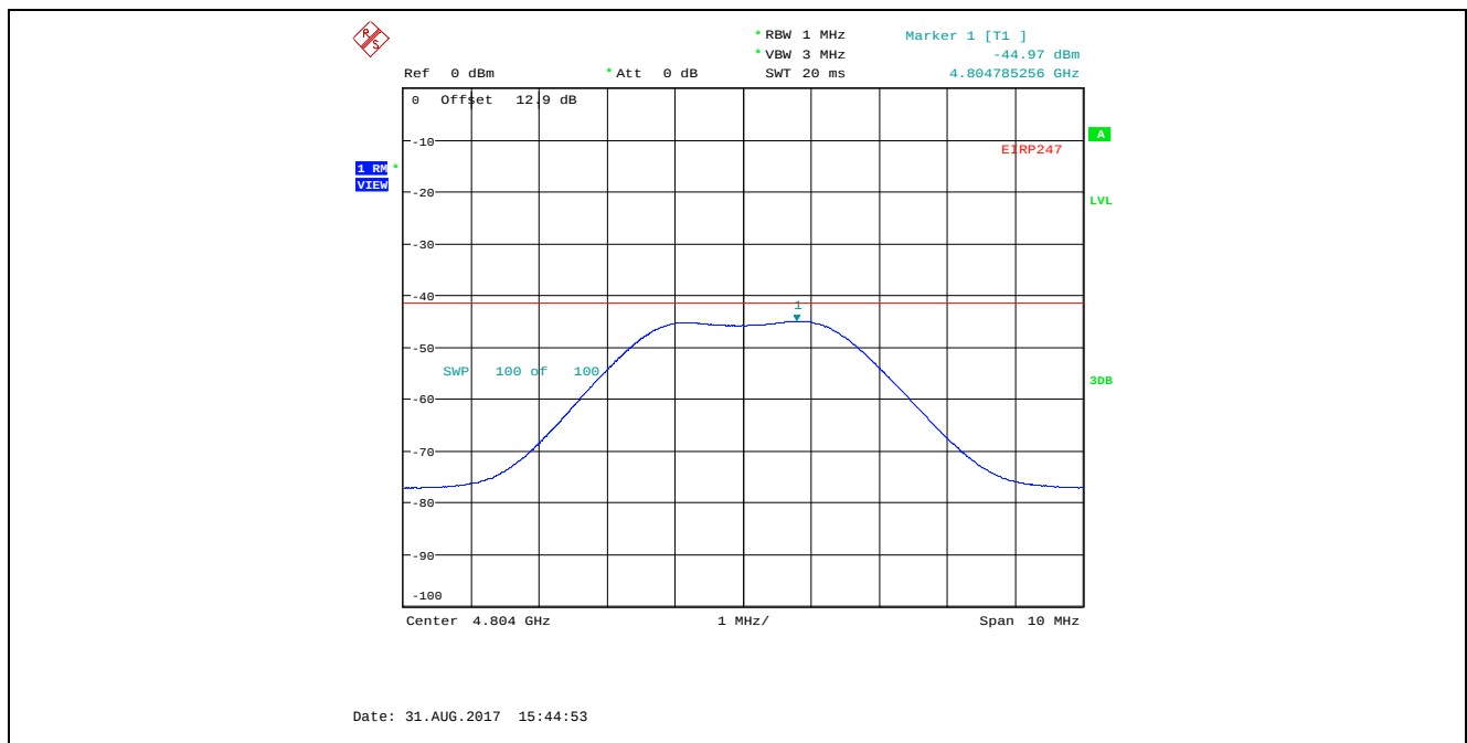
Plot 5.4.4.3.24. Conducted Spurious Emissions in Restricted Frequency Bands, High Power 2402 MHz, GFSK Modulation, 2 Mbps, Marker 1, Trace Averaging RMS Detector
