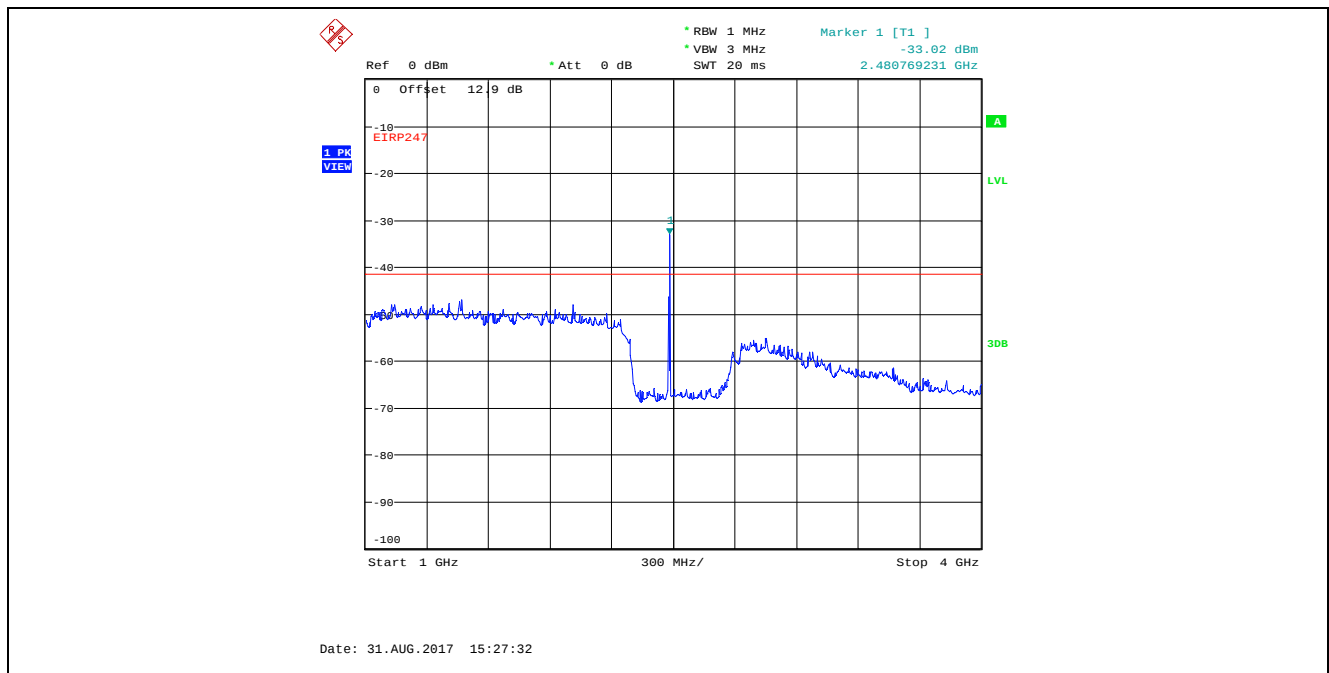
Plot 5.4.4.3.34. Conducted Spurious Emissions in Restricted Frequency Bands, High Power 2480 MHz, GFSK Modulation, 2 Mbps, 1 GHz - 4 GHz, Peak Detector Marker 1 is the Fundamental Frequency
