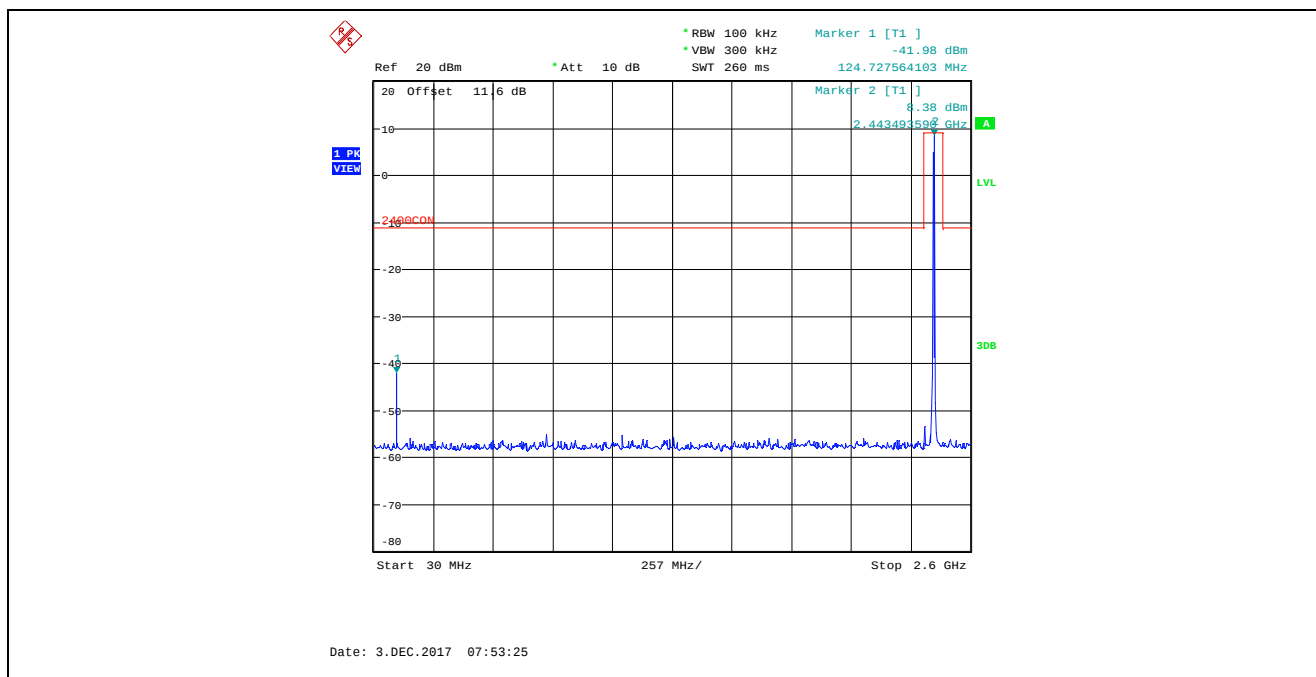
Plot 5.4.4.2.9. Conducted Spurious Emissions in Non-Restricted Frequency Bands, High Power 2440 MHz, GFSK Modulation, 2 Mbps, 30 MHz – 2.6 GHz, Peak Detector
