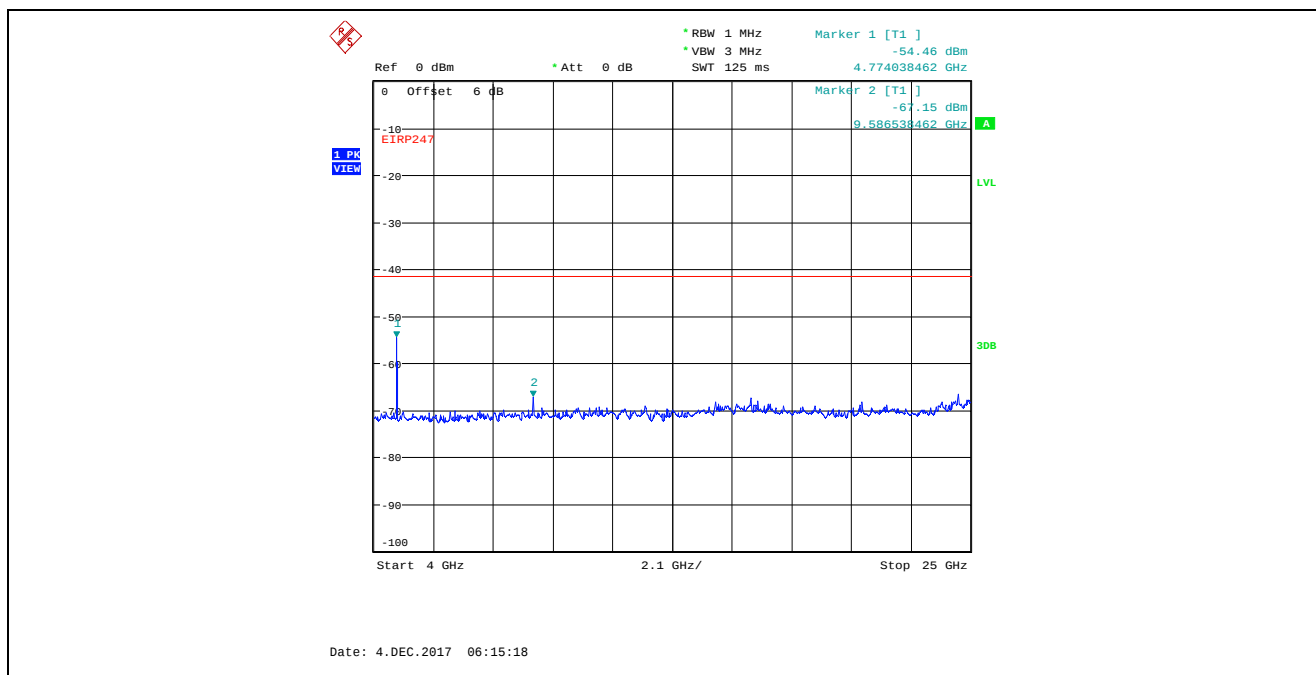
Plot 5.4.4.3.20. Conducted Spurious Emissions in Restricted Frequency Bands, High Power 2402 MHz, GFSK Modulation, 2 Mbps, 4 GHz - 25 GHz, Peak Detector
