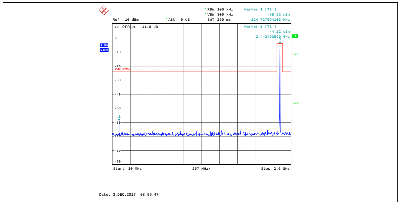
Plot 5.4.4.2.21. Conducted Spurious Emissions in Non-Restricted Frequency Bands, Low Power 2440 MHz, GFSK Modulation, 2 Mbps, 30 MHz – 2.6 GHz, Peak Detector
