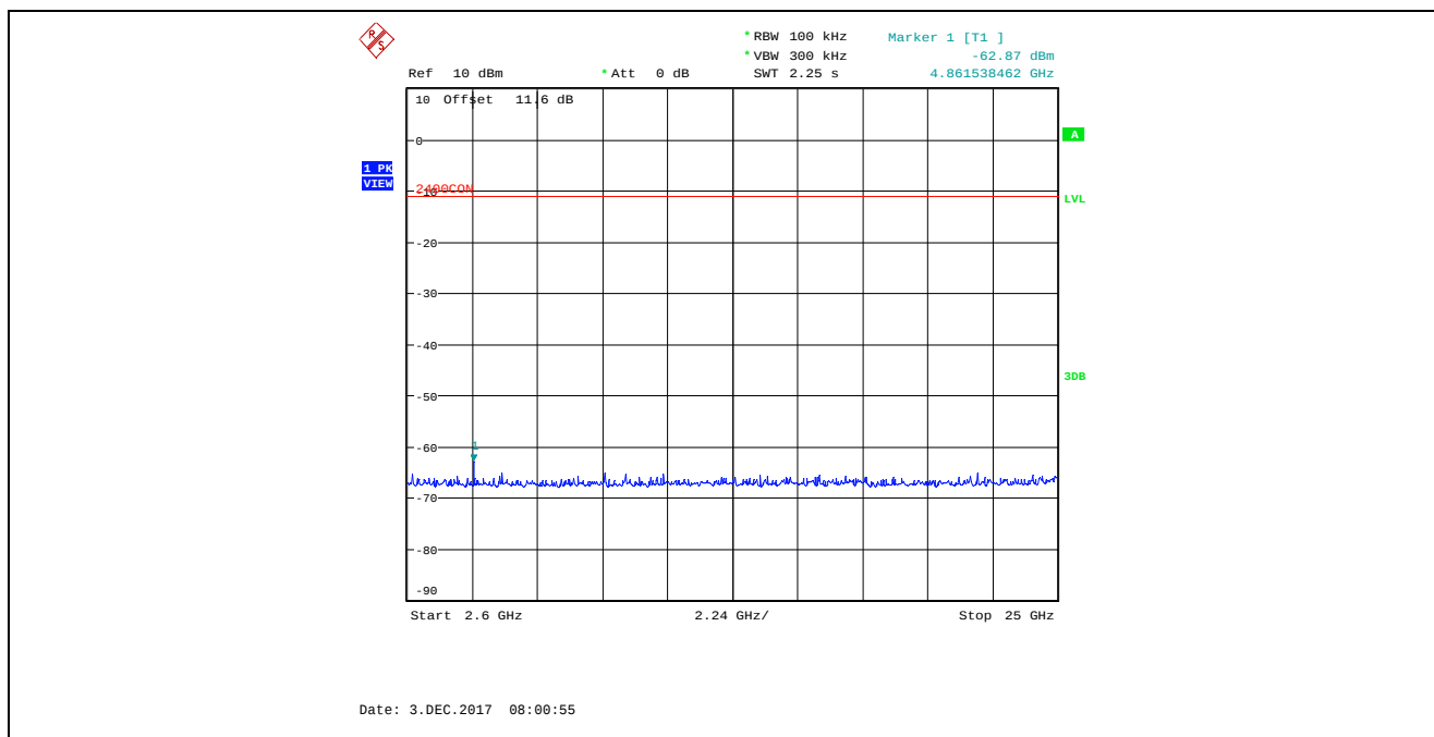
Plot 5.4.4.2.10. Conducted Spurious Emissions in Non-Restricted Frequency Bands, High Power 2440 MHz, GFSK Modulation, 2 Mbps, 2.6 GHz – 25 GHz, Peak Detector
