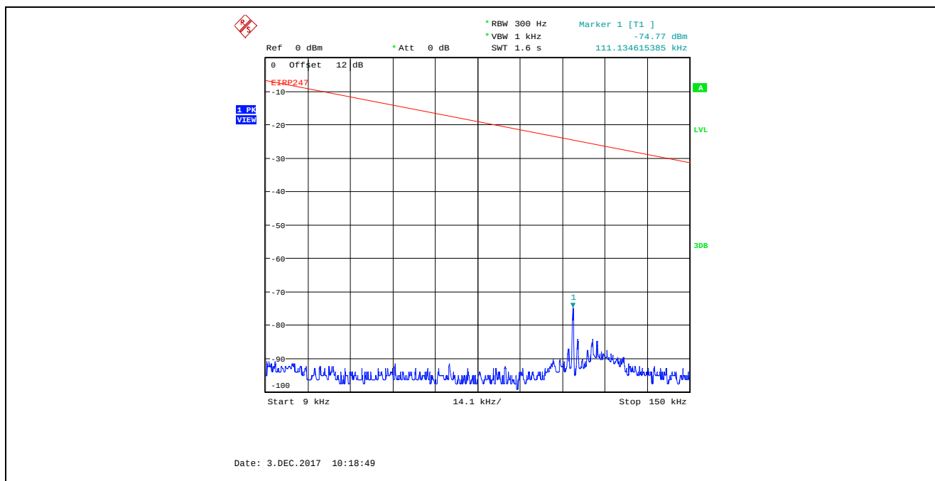
Plot 5.4.4.3.16. Conducted Spurious Emissions in Restricted Frequency Bands, High Power 2402 MHz, GFSK Modulation, 2 Mbps, 9 kHz - 150 kHz, Peak Detector
