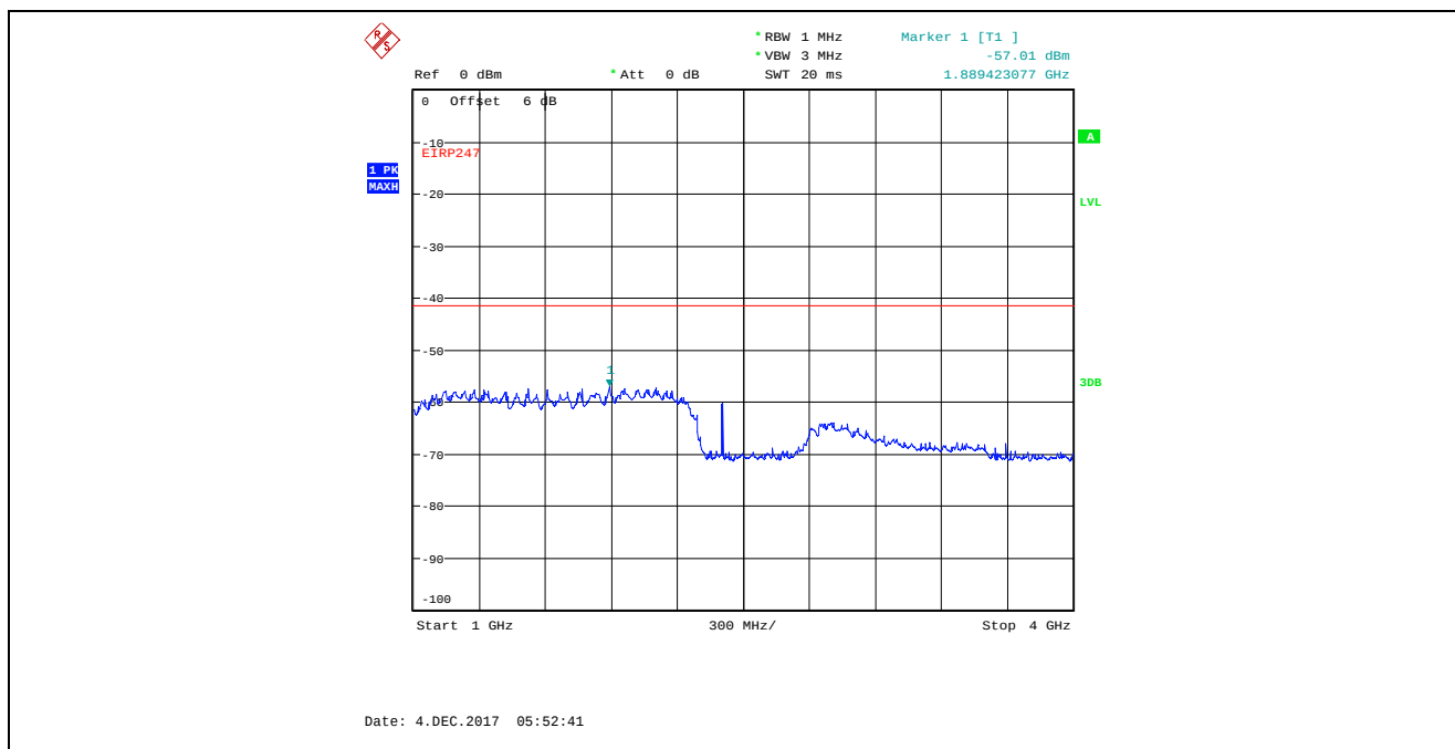
Plot 5.4.4.3.19. Conducted Spurious Emissions in Restricted Frequency Bands, High Power 2402 MHz, GFSK Modulation, 2 Mbps, 1 GHz - 4 GHz, Peak Detector
