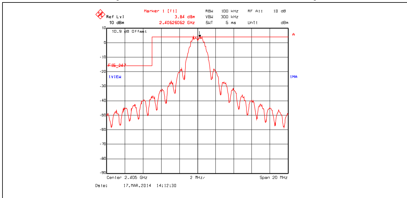
Plot 5.4.4.1.1. Band-Edge RF Conducted Emissions Lower Band-edge, Channel 11, 2405 MHz, QPSK Modulation, Power Setting 8 Mode 1
