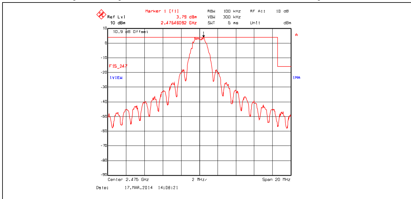
Plot 5.4.4.1.2. Band-Edge RF Conducted Emissions Higher Band-edge, Channel 25, 2475 MHz, QPSK Modulation, Power Setting 8 Mode 1
