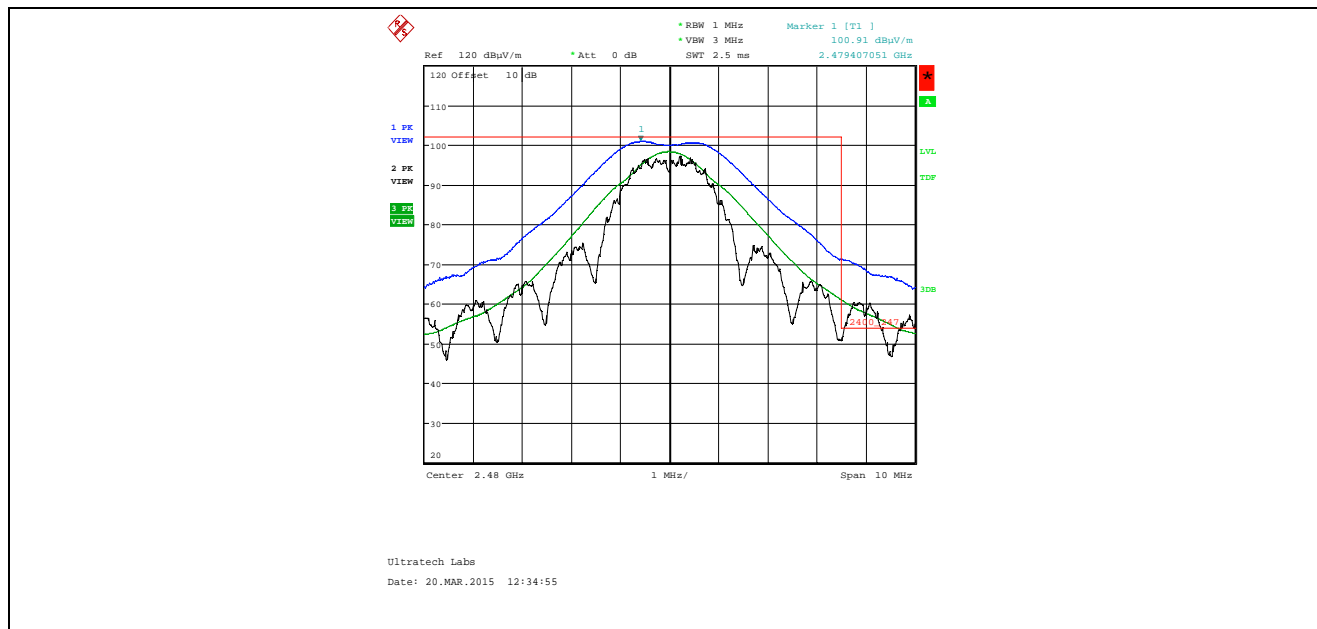
Plot 5.4.4.4.2.1. Band-Edge RF Radiated Emissions at 3 m, Horizontal Polarization High End of Frequency Band, QPSK Modulation, Power -26 Mode 3
