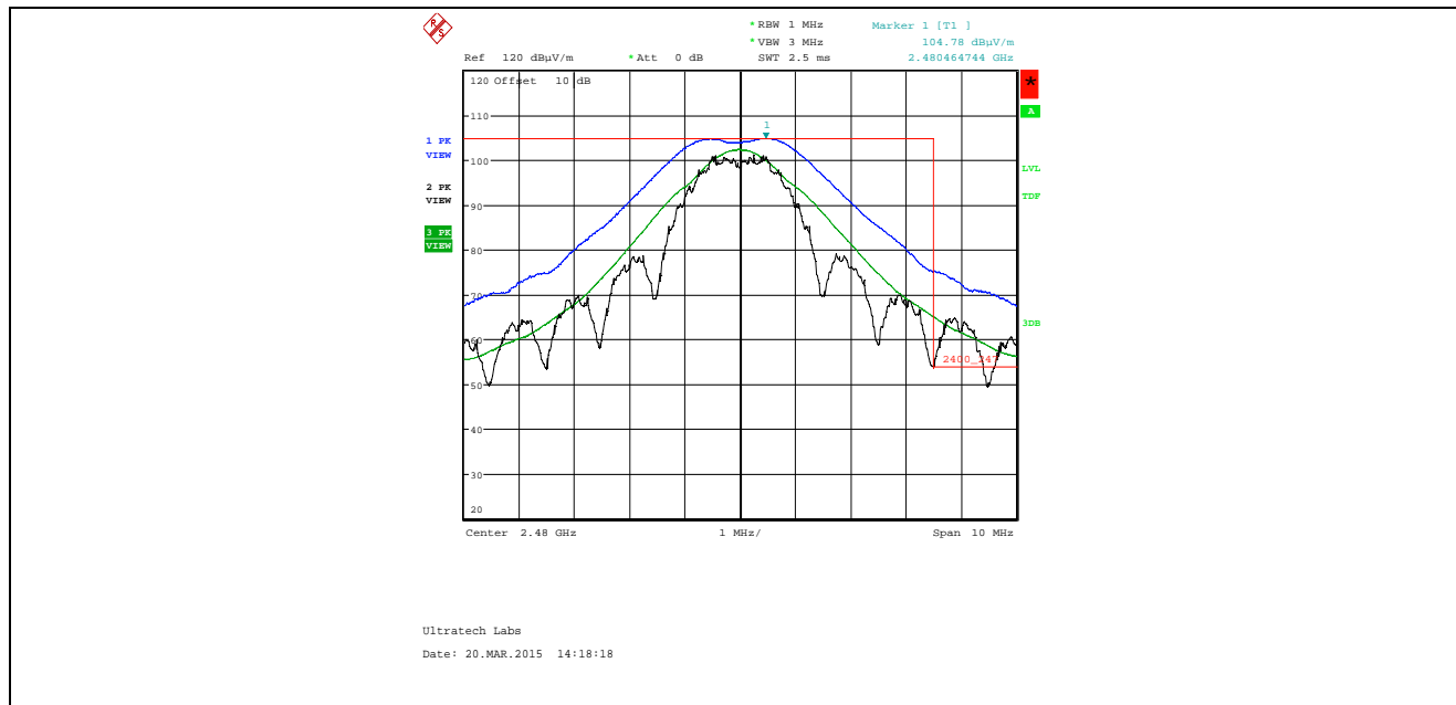
Plot 5.4.4.1.1.3. Band-Edge RF Radiated Emissions at 3 m, Vertical Polarization High End of Frequency Band, QPSK Modulation, Power -26 Mode 3
