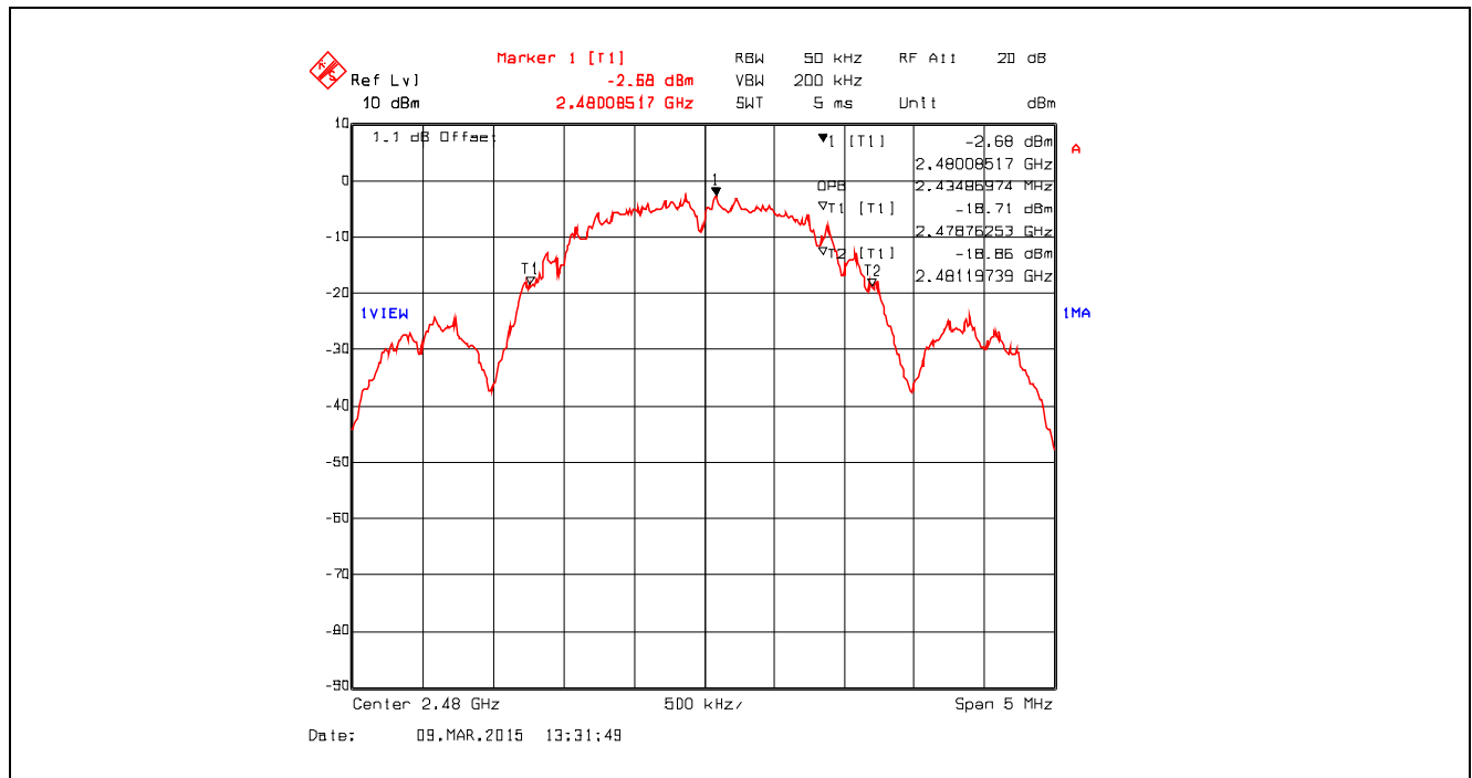
Plot 5.1.4.2. 99% Occupied Bandwidth, Channel 26, 2480 MHz, QPSK Modulation, Power Setting -26 Mode 3
