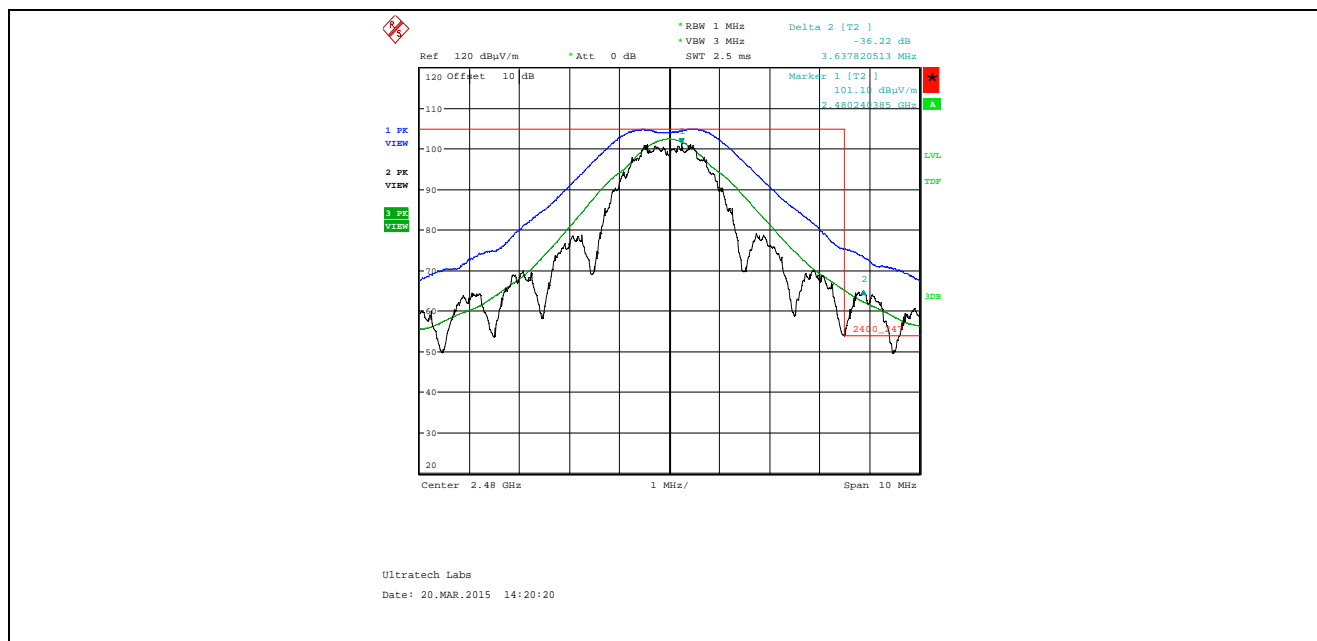
Plot 5.4.4.1.1.4. Band-Edge RF Radiated Emissions at 3 m, Vertical Polarization High End of Frequency Band, QPSK Modulation, Power -26 Mode 3
