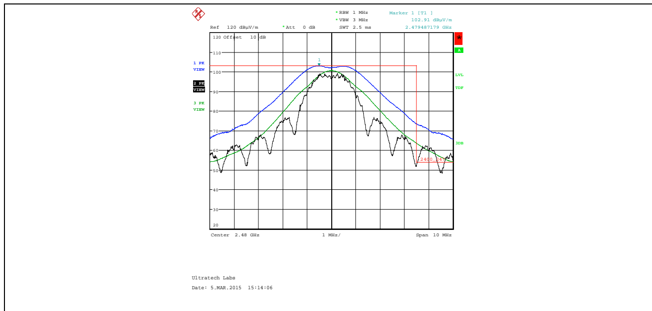
Plot 5.4.4.5.2.1. Band-Edge RF Radiated Emissions at 3 m, Horizontal Polarization High End of Frequency Band, QPSK Modulation, Power -26 Mode 3
