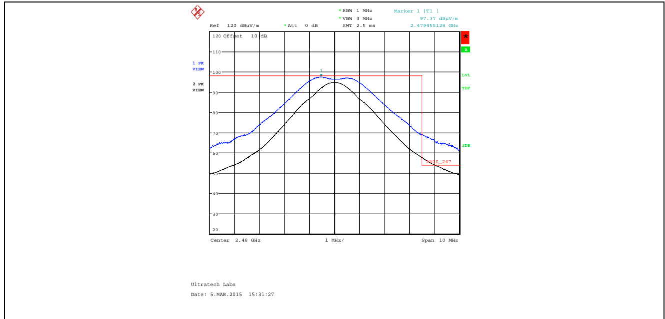
Plot 5.4.4.5.2.3. Band-Edge RF Radiated Emissions at 3 m, Vertical Polarization High End of Frequency Band, QPSK Modulation, Power -26 Mode 3
