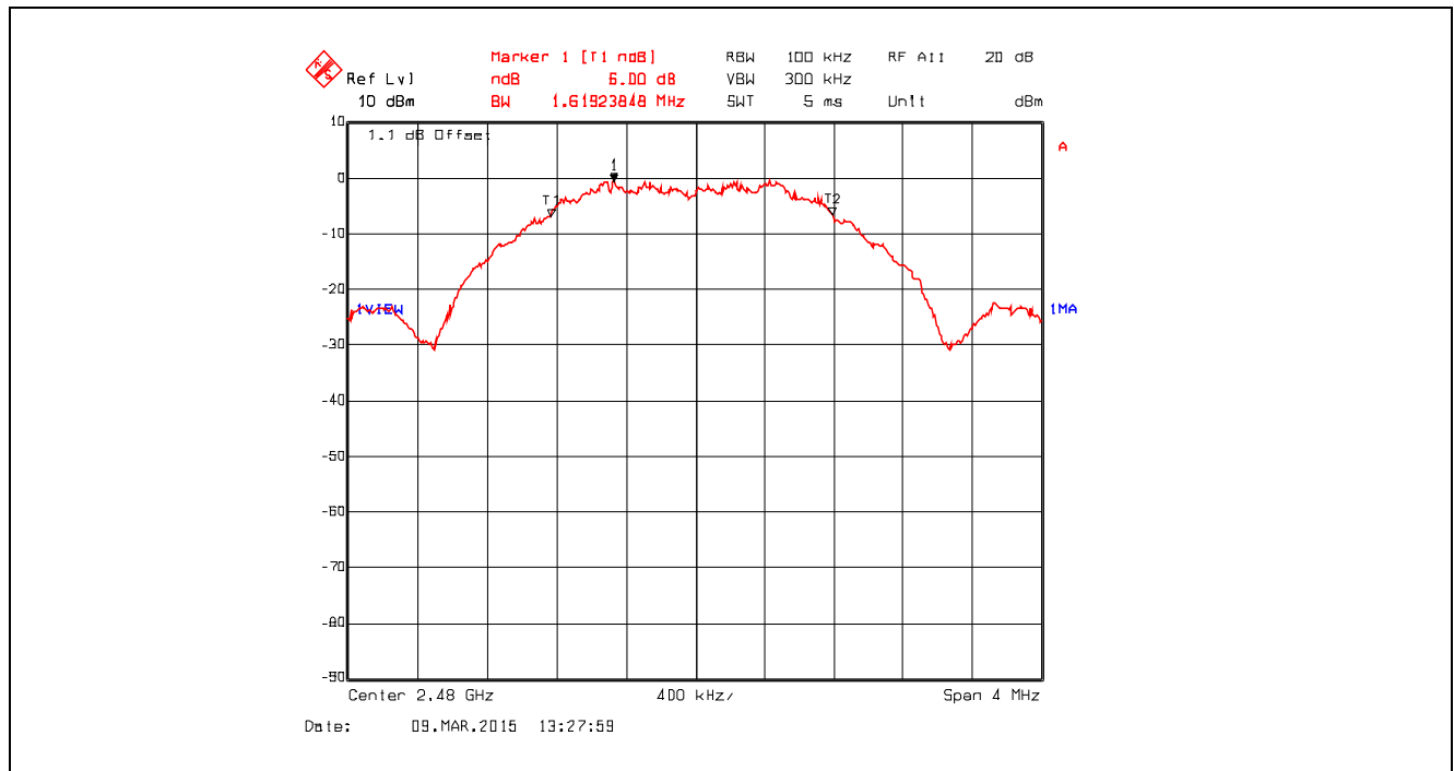
Plot 5.1.4.1. 6 dB Bandwidth, Channel 26, 2480 MHz, QPSK Modulation, Power Setting -26 Mode 3
