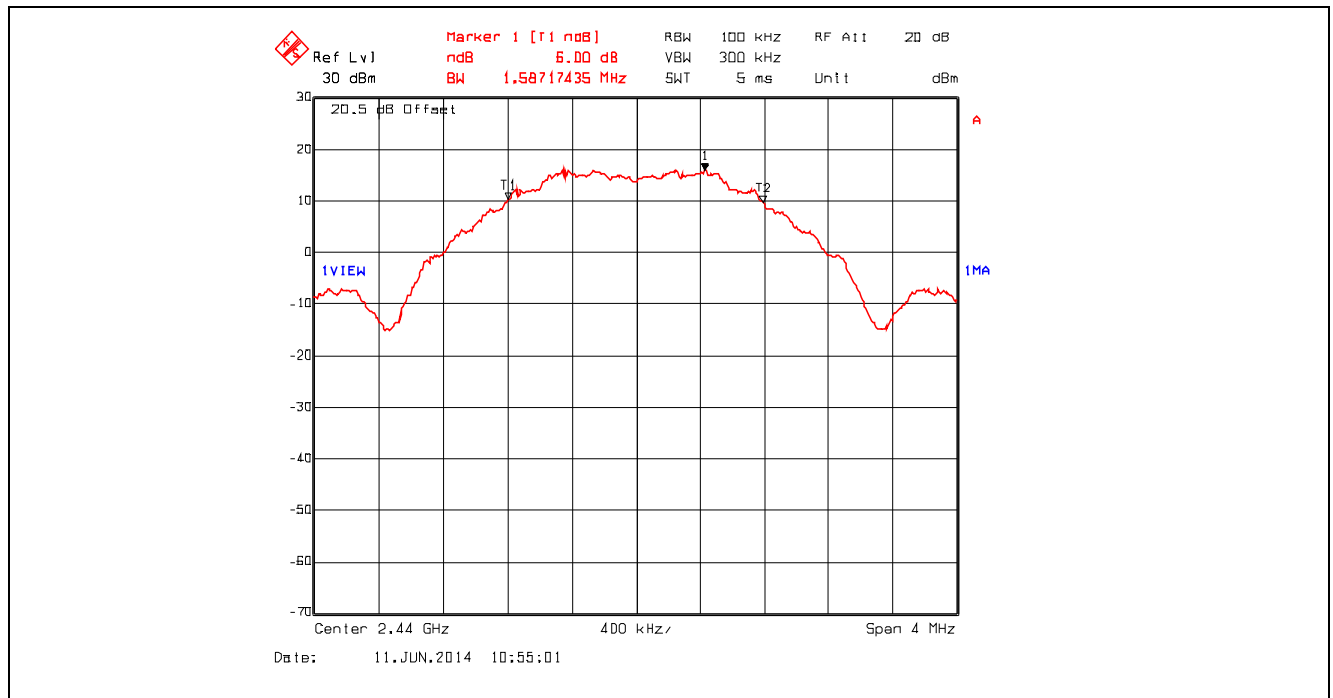
Plot 5.2.4.2. 6 dB Bandwidth, Channel 18, 2440 MHz, QPSK Modulation, Power Setting -8 Mode 3
