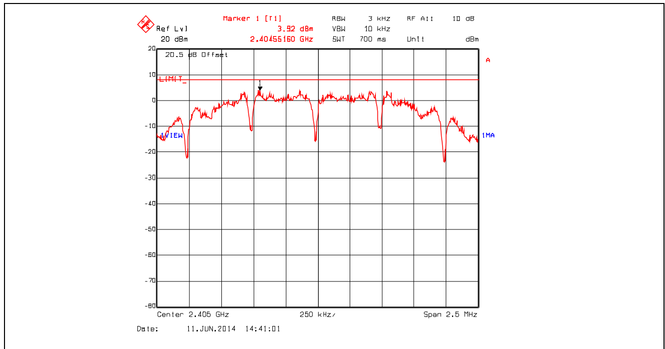
Plot 5.6.4.1. Power Spectral Density, Channel 11, 2405 MHz, QPSK Modulation, Power Setting -8 Mode 3
