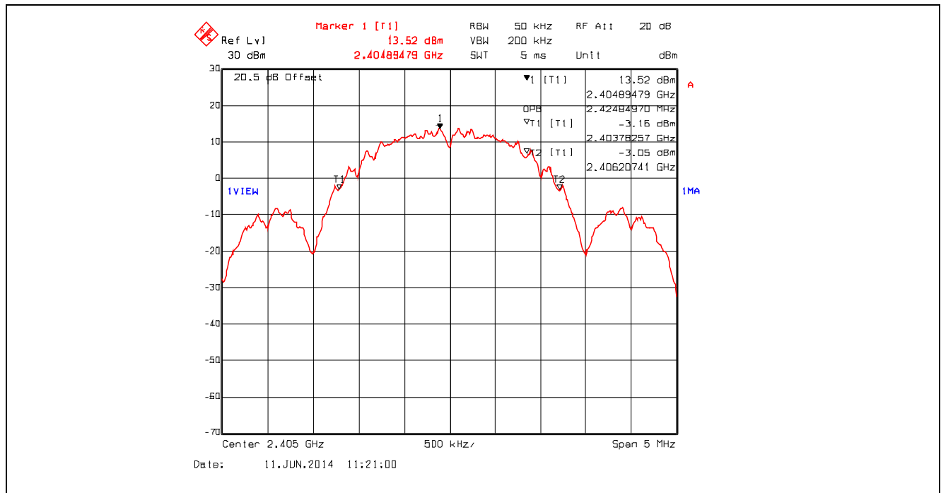
Plot 5.2.4.4. 99% Occupied Bandwidth, Channel 11, 2405 MHz, QPSK Modulation, Power Setting -8 Mode 3
