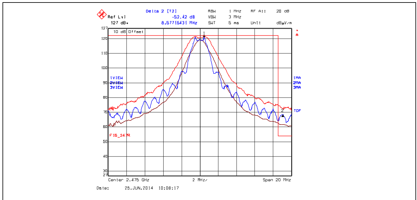
Plot 5.5.4.4.2.3. Band-Edge RF Radiated Emissions at 3 m, Horizontal Polarization High End of Frequency Band, QPSK Modulation, Power -8 Mode 3
