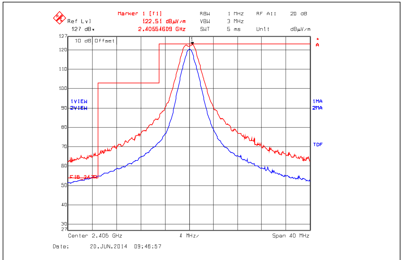
Plot 5.5.4.3.2.4. Band-Edge RF Radiated Emissions at 3 m, Vertical Polarization Low End of Frequency Band, QPSK Modulation, Power -8 Mode 3
