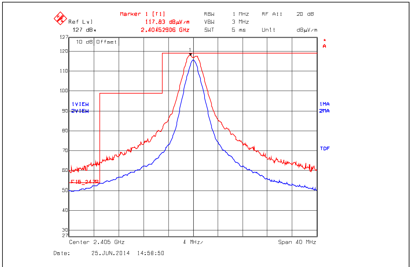
Plot 5.5.4.5.2.4. Band-Edge RF Radiated Emissions at 3 m, Vertical Polarization Low End of Frequency Band, QPSK Modulation, Power -8 Mode 3
