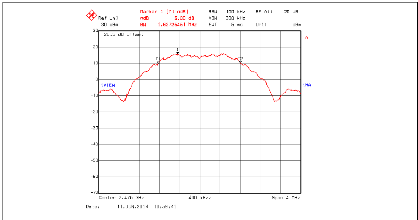
Plot 5.2.4.3. 6 dB Bandwidth, Channel 25, 2475 MHz, QPSK Modulation, Power Setting -8 Mode 3
