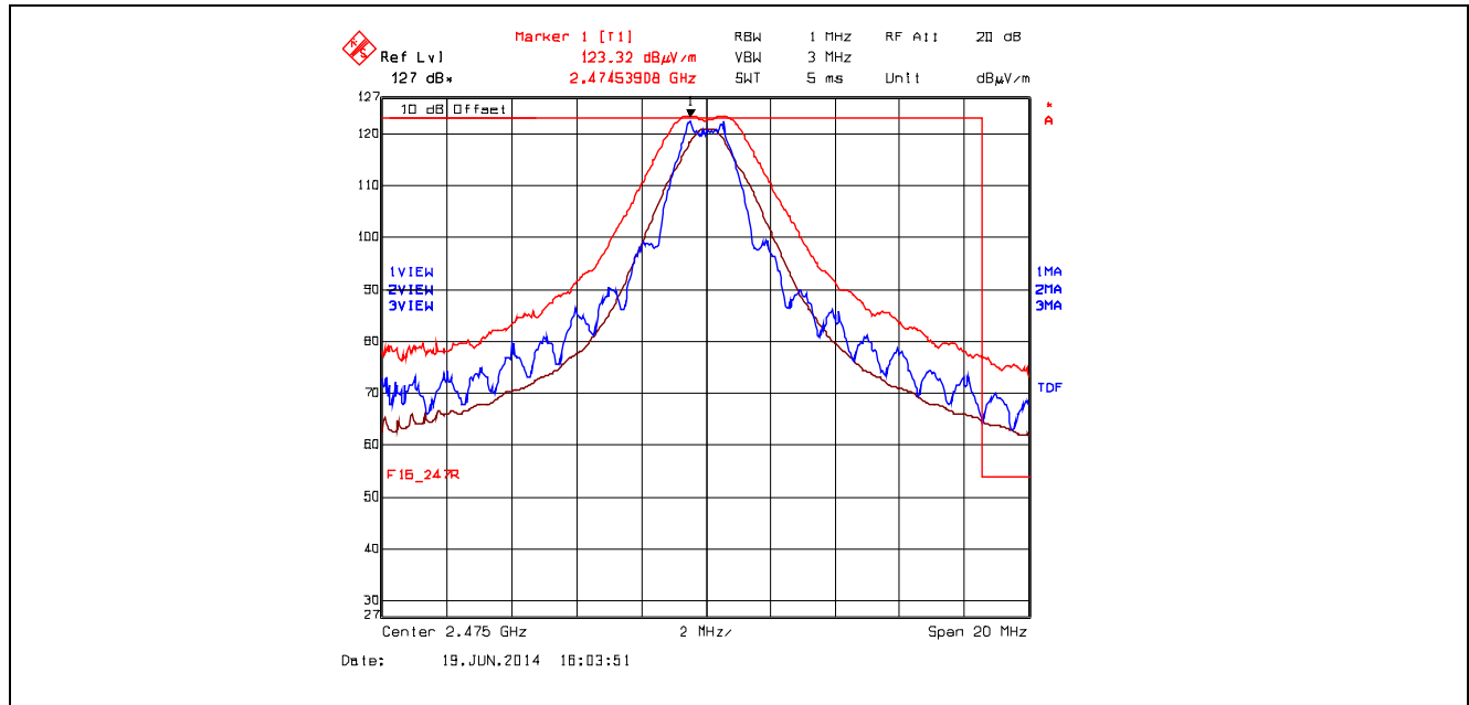
Plot 5.5.4.3.2.5. Band-Edge RF Radiated Emissions at 3 m, Vertical Polarization High End of Frequency Band, QPSK Modulation, Power -8 Mode 3
