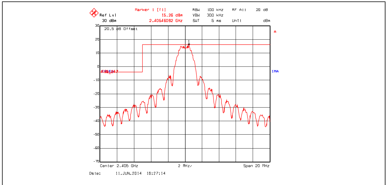
Plot 5.4.4.1.1. Band-Edge RF Conducted Emissions Lower Band-edge, Channel 11, 2405 MHz, QPSK Modulation, Power Setting -8 Mode 3
