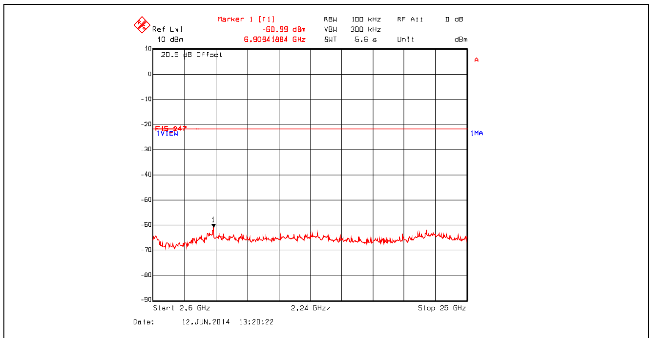
Plot 5.4.4.2.10. Conducted Spurious Emissions Channel 18, 2440 MHz, QPSK Modulation, Power Setting -26 Mode 3, 2.6 GHz – 25 GHz
