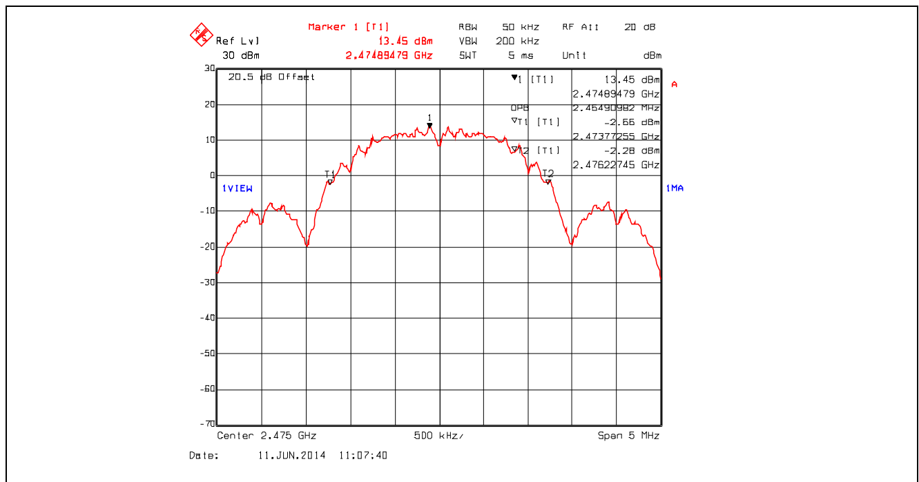
Plot 5.2.4.6. 99% Occupied Bandwidth, Channel 25, 2475 MHz, QPSK Modulation, Power Setting -8 Mode 3
