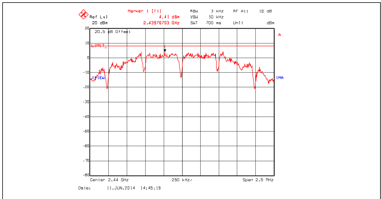
Plot 5.6.4.2. Power Spectral Density, Channel 18, 2440 MHz, QPSK Modulation, Power Setting -8 Mode 3
