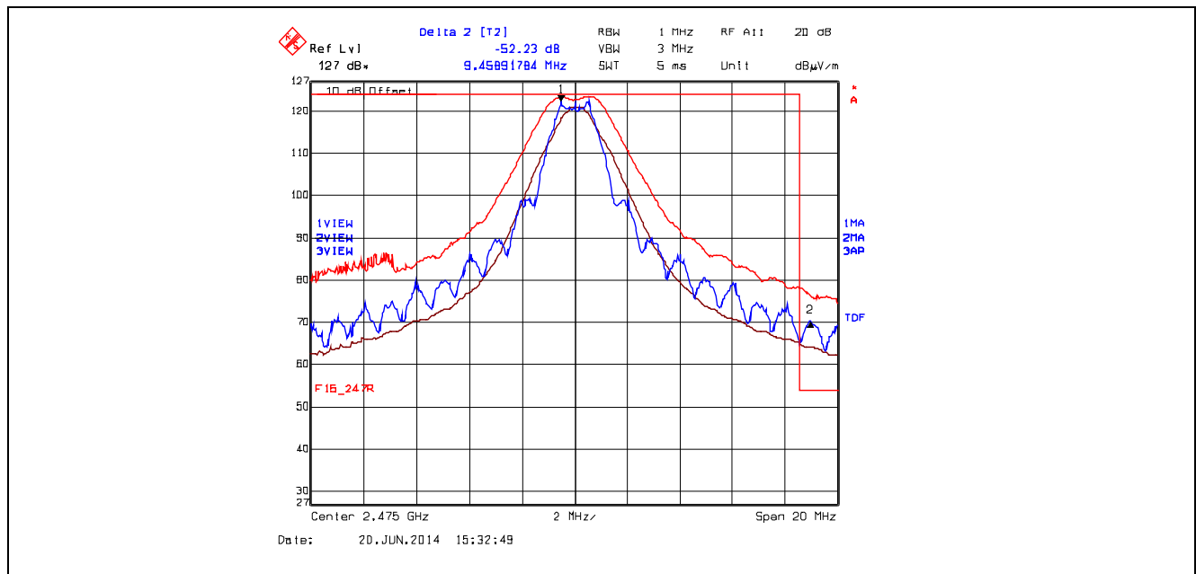
Plot 5.5.4.2.3. Band-Edge RF Radiated Emissions at 3 m, Horizontal Polarization High End of Frequency Band, QPSK Modulation, Power -8 Mode 3
