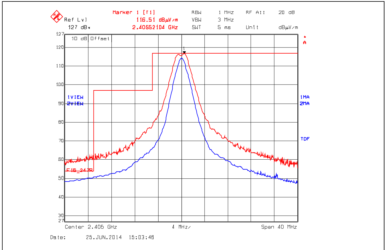
Plot 5.5.4.5.2.1. Band-Edge RF Radiated Emissions at 3 m, Horizontal Polarization Low End of Frequency Band, QPSK Modulation, Power -8 Mode 3
