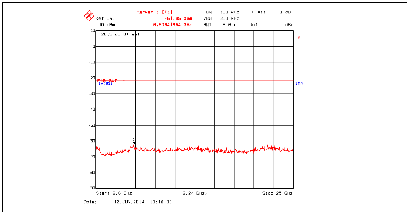
Plot 5.4.4.2.12. Conducted Spurious Emissions Channel 25, 2475 MHz, QPSK Modulation, Power Setting -26 Mode 3, 2.6 GHz – 25 GHz
