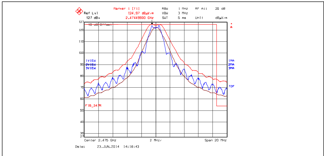
Plot 5.5.4.1.2.5. Band-Edge RF Radiated Emissions at 3 m, Vertical Polarization High End of Frequency Band, QPSK Modulation, Power -8 Mode 3
