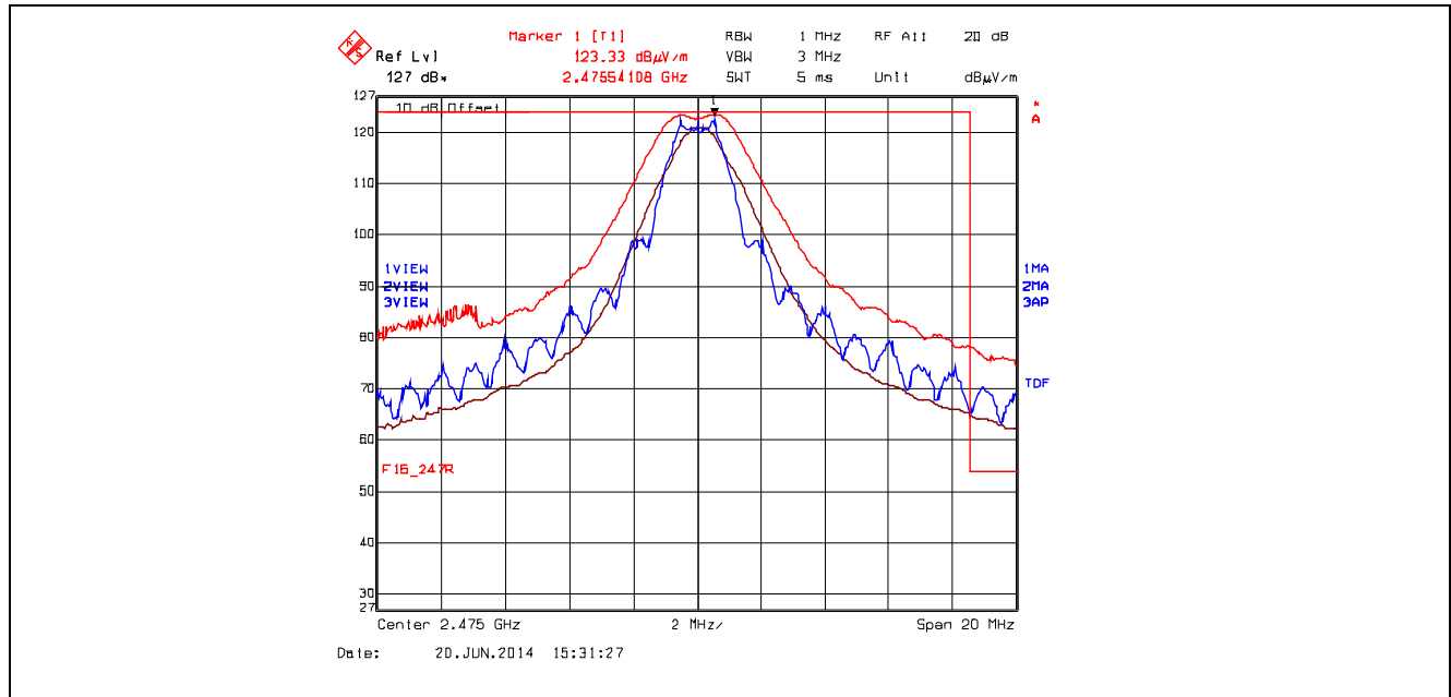
Plot 5.5.4.2.2. Band-Edge RF Radiated Emissions at 3 m, Horizontal Polarization High End of Frequency Band, QPSK Modulation, Power -8 Mode 3
