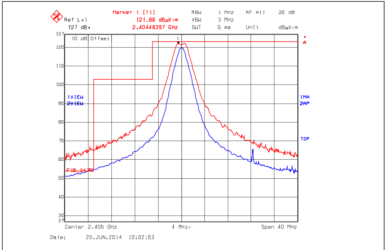
Plot 5.5.4.3.2.1. Band-Edge RF Radiated Emissions at 3 m, Horizontal Polarization Low End of Frequency Band, QPSK Modulation, Power -8 Mode 3
