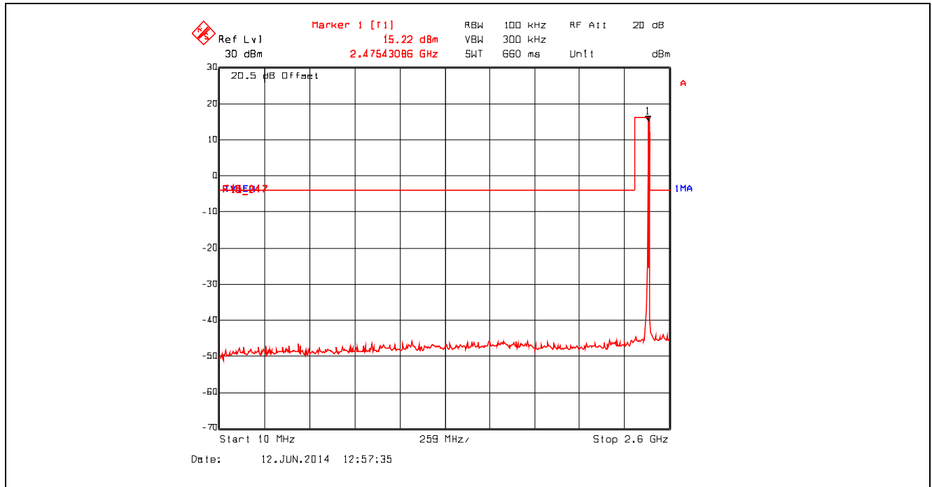
Plot 5.4.4.2.5. Conducted Spurious Emissions Channel 25, 2475 MHz, QPSK Modulation, Power Setting -8 Mode 3, 10 MHz – 2.6 GHz
