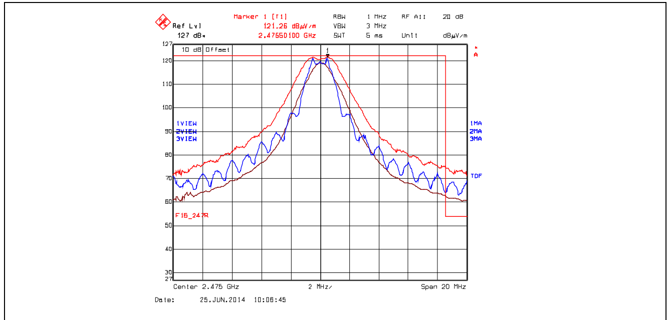
Plot 5.5.4.4.2.2. Band-Edge RF Radiated Emissions at 3 m, Horizontal Polarization High End of Frequency Band, QPSK Modulation, Power -8 Mode 3
