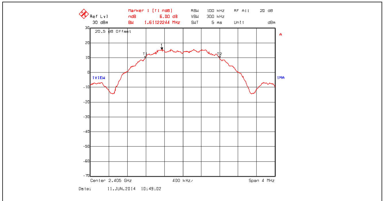
Plot 5.2.4.1. 6 dB Bandwidth, Channel 11, 2405 MHz, QPSK Modulation, Power Setting -8 Mode 3
