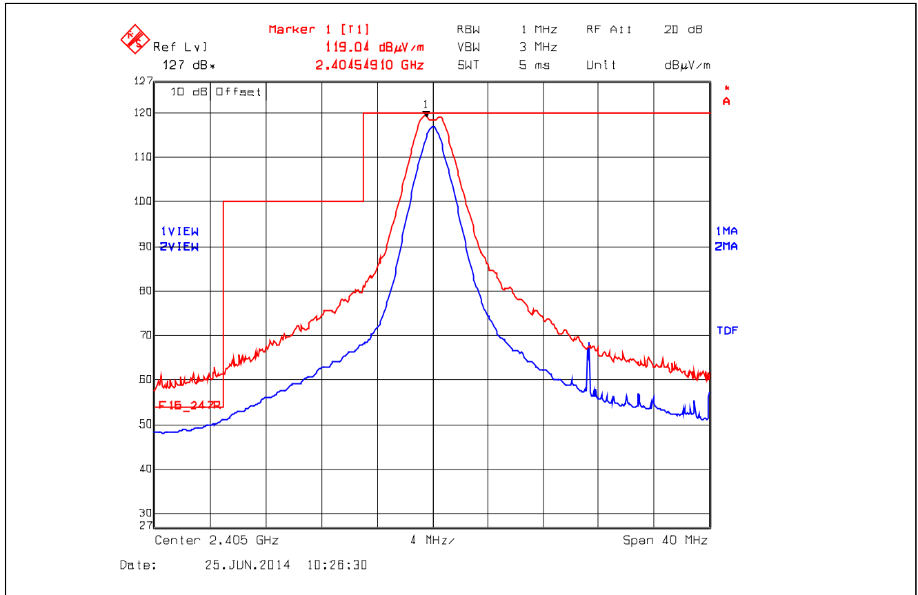
Plot 5.5.4.4.2.1. Band-Edge RF Radiated Emissions at 3 m, Horizontal Polarization Low End of Frequency Band, QPSK Modulation, Power -8 Mode 3
