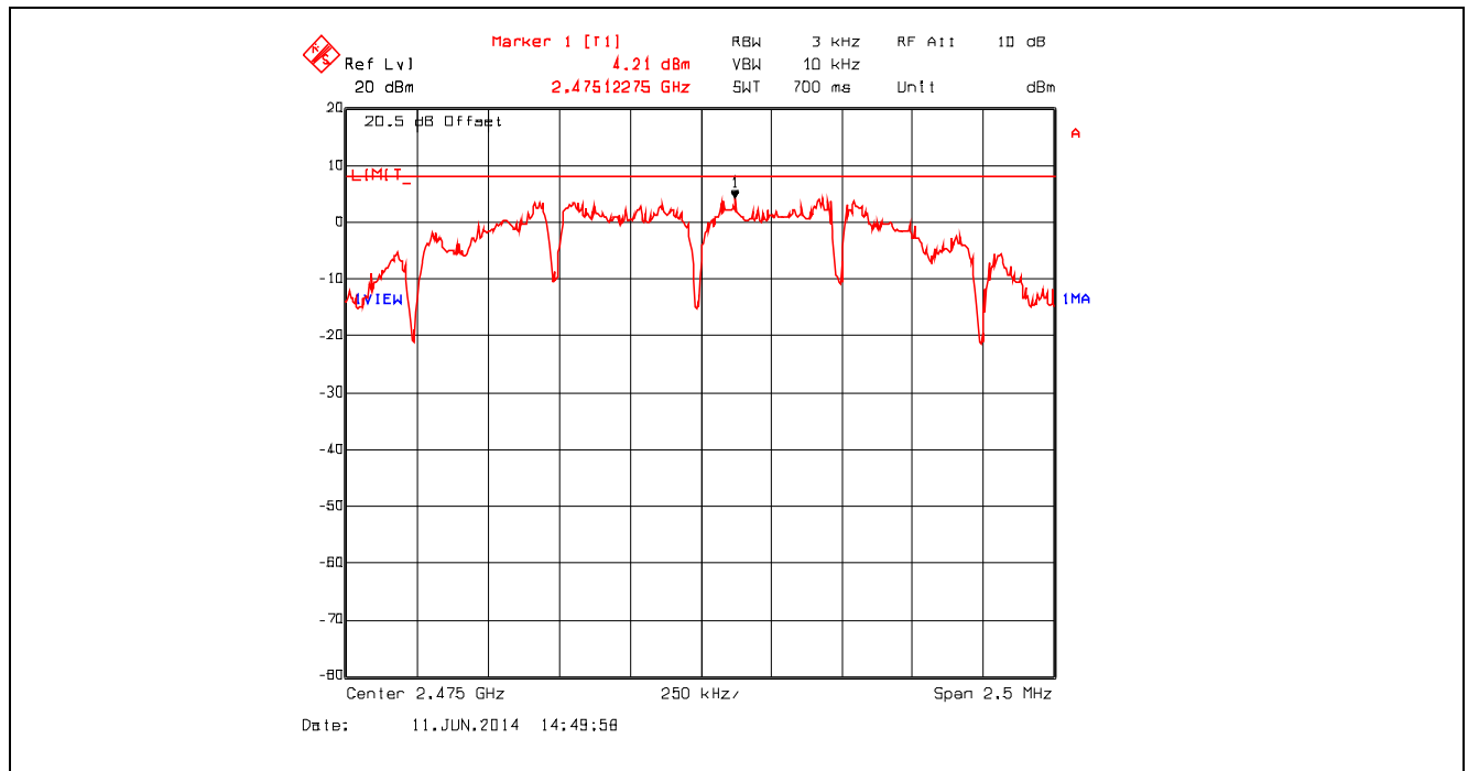
Plot 5.6.4.3. Power Spectral Density, Channel 25, 2475 MHz, QPSK Modulation, Power Setting -8 Mode 3
