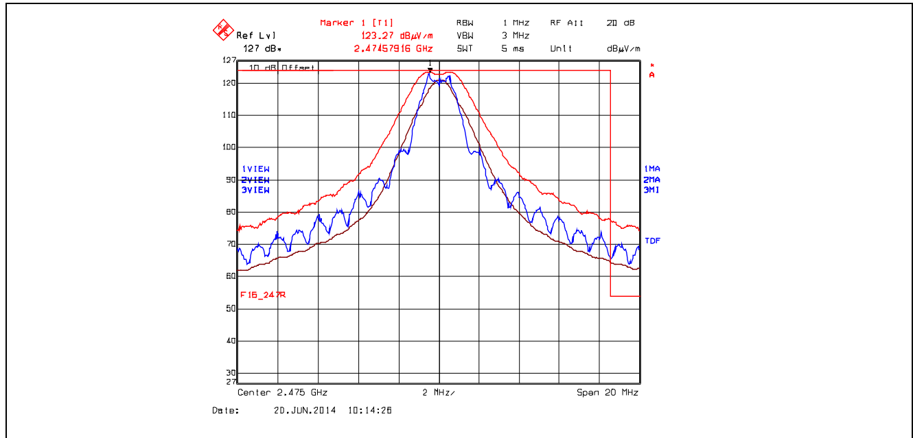
Plot 5.5.4.3.2.2. Band-Edge RF Radiated Emissions at 3 m, Horizontal Polarization High End of Frequency Band, QPSK Modulation, Power -8 Mode 3
