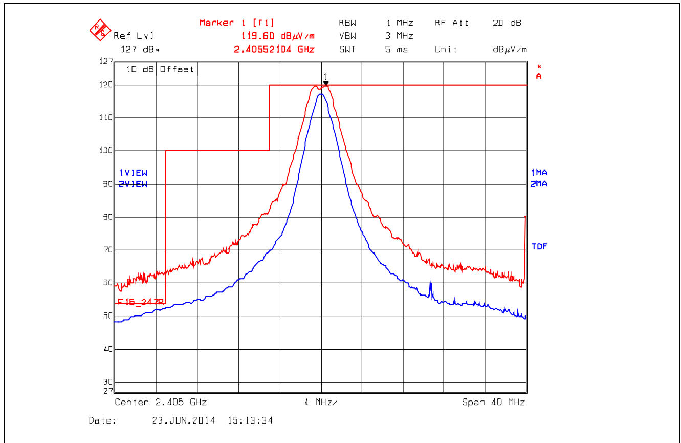
Plot 5.5.4.1.2.1. Band-Edge RF Radiated Emissions at 3 m, Horizontal Polarization Low End of Frequency Band, QPSK Modulation, Power -8 Mode 3
