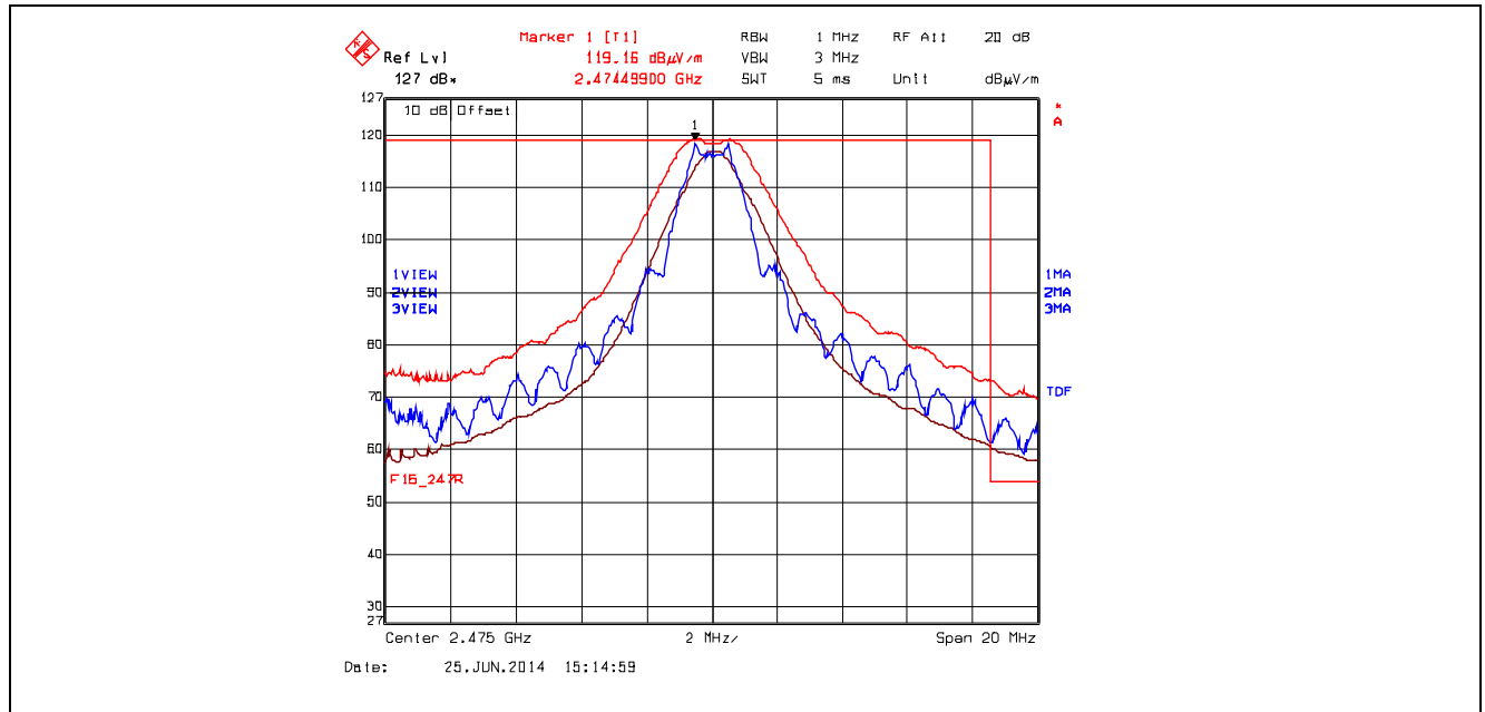
Plot 5.5.4.5.2.5. Band-Edge RF Radiated Emissions at 3 m, Vertical Polarization High End of Frequency Band, QPSK Modulation, Power -8 Mode 3
