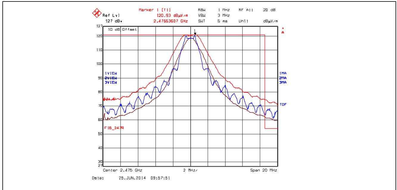
Plot 5.5.4.4.2.5. Band-Edge RF Radiated Emissions at 3 m, Vertical Polarization High End of Frequency Band, QPSK Modulation, Power -8 Mode 3
