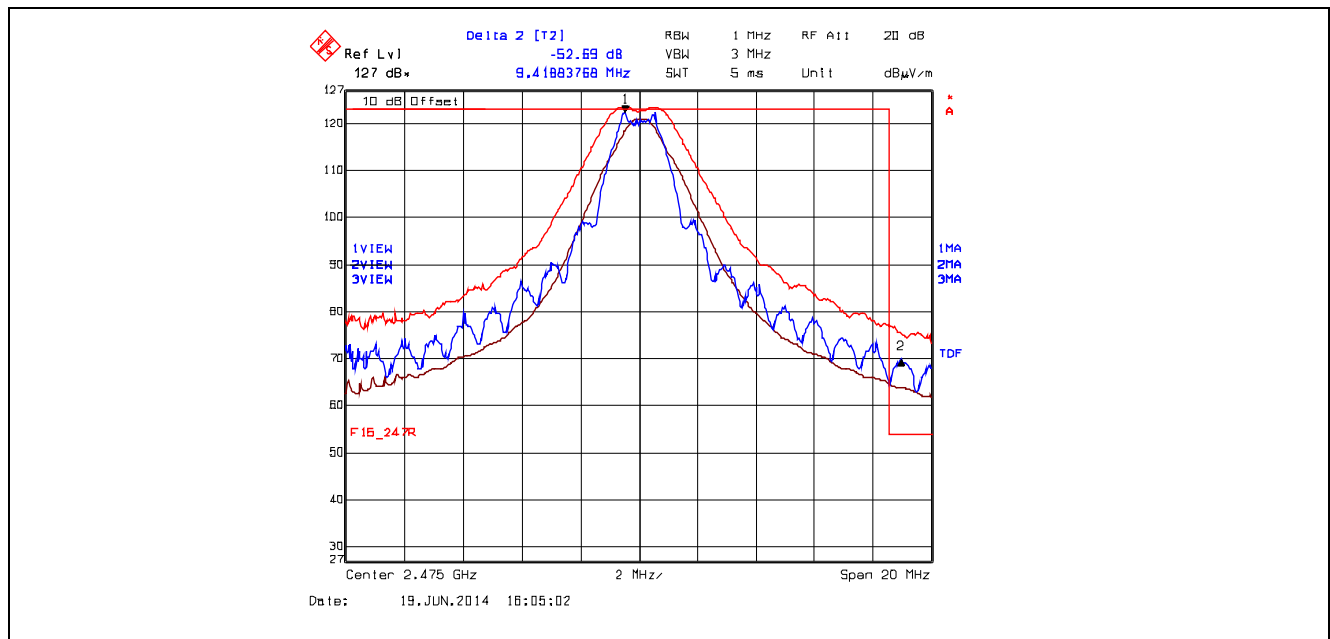
Plot 5.5.4.3.2.6. Band-Edge RF Radiated Emissions at 3 m, Vertical Polarization High End of Frequency Band, QPSK Modulation, Power -8 Mode 3
