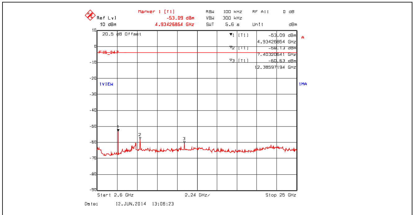
Plot 5.4.4.2.6. Conducted Spurious Emissions Channel 25, 2475 MHz, QPSK Modulation, Power Setting -8 Mode 3, 2.6 GHz – 25 GHz
