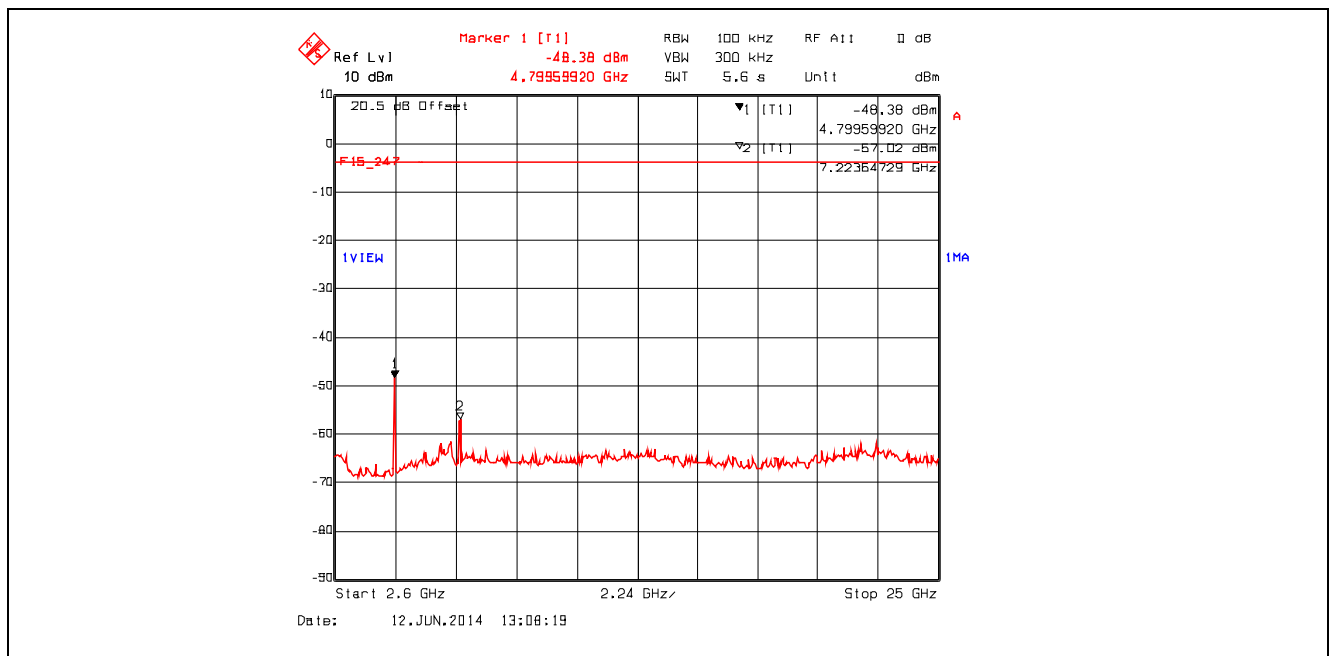
Plot 5.4.4.2.2. Conducted Spurious Emissions Channel 11, 2405 MHz, QPSK Modulation, Power Setting -8 Mode 3, 2.6 GHz – 25 GHz
