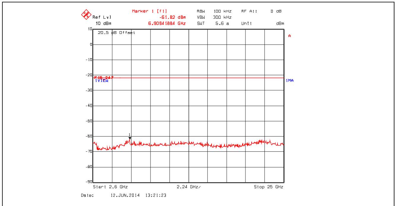
Plot 5.4.4.2.8. Conducted Spurious Emissions Channel 11, 2405 MHz, QPSK Modulation, Power Setting -26 Mode 3, 2.6 GHz – 25 GHz
