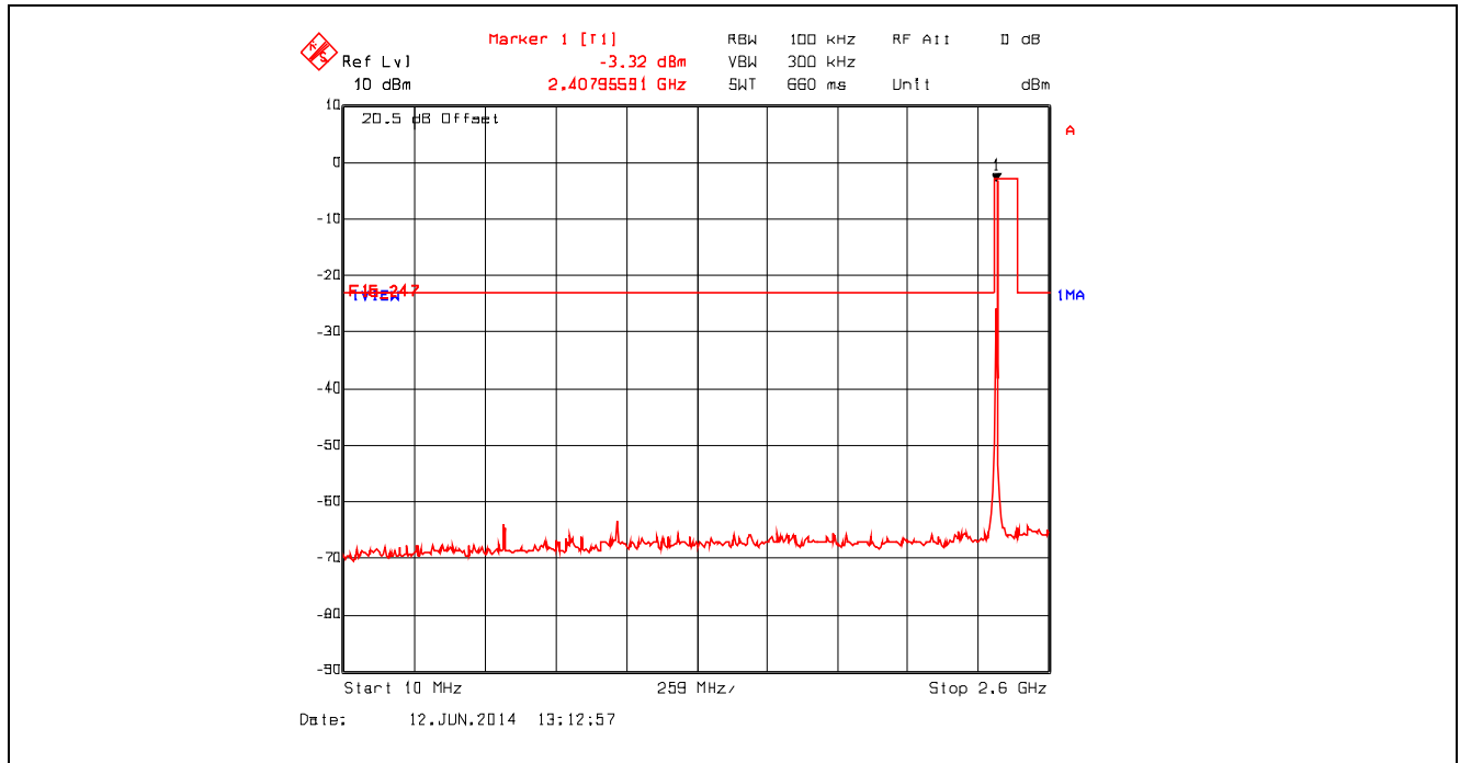
Plot 5.4.4.2.7. Conducted Spurious Emissions Channel 11, 2405 MHz, QPSK Modulation, Power Setting -26 Mode 3, 10 MHz – 2.6 GHz
