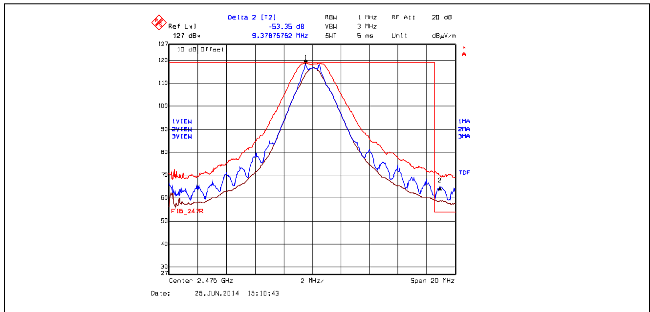
Plot 5.5.4.5.2.3. Band-Edge RF Radiated Emissions at 3 m, Horizontal Polarization High End of Frequency Band, QPSK Modulation, Power -8 Mode 3
