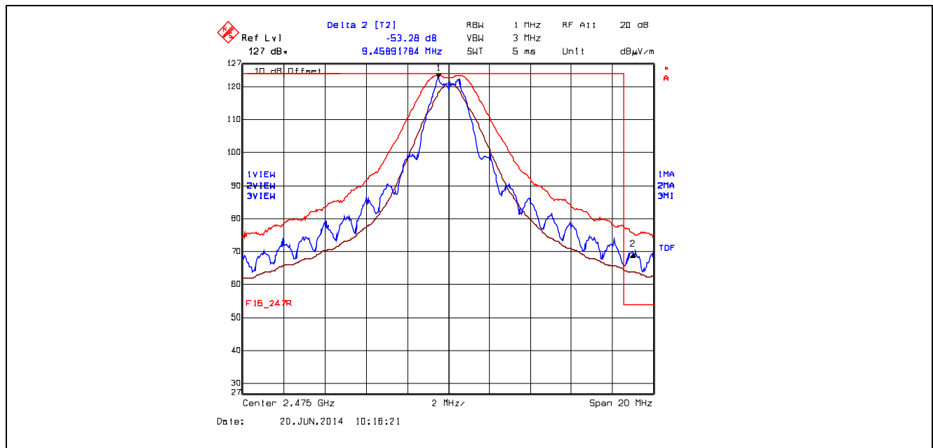
Plot 5.5.4.3.2.3. Band-Edge RF Radiated Emissions at 3 m, Horizontal Polarization High End of Frequency Band, QPSK Modulation, Power -8 Mode 3
