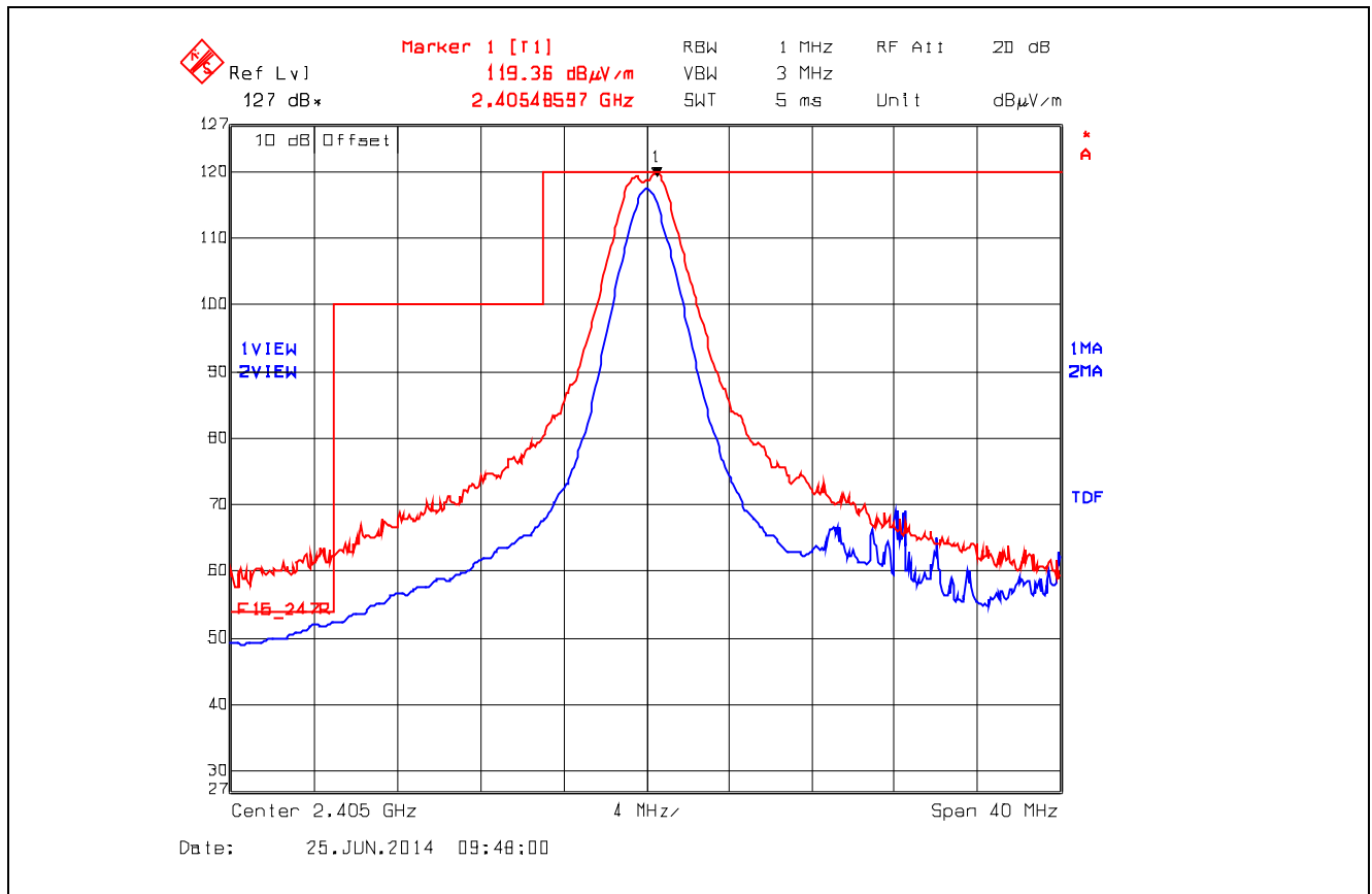
Plot 5.5.4.4.2.4. Band-Edge RF Radiated Emissions at 3 m, Vertical Polarization Low End of Frequency Band, QPSK Modulation, Power -8 Mode 3
