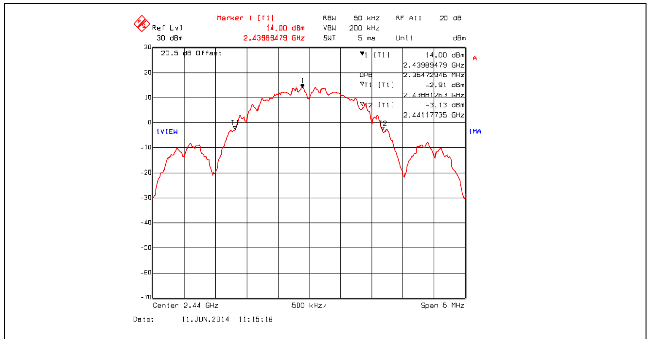
Plot 5.2.4.5. 99% Occupied Bandwidth, Channel 18, 2440 MHz, QPSK Modulation, Power Setting -8 Mode 3
