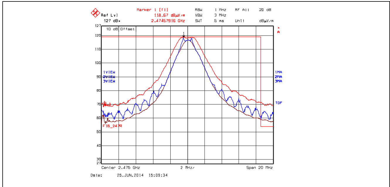
Plot 5.5.4.5.2.2. Band-Edge RF Radiated Emissions at 3 m, Horizontal Polarization High End of Frequency Band, QPSK Modulation, Power -8 Mode 3
