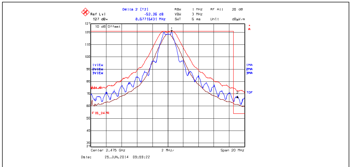
Plot 5.5.4.4.2.6. Band-Edge RF Radiated Emissions at 3 m, Vertical Polarization High End of Frequency Band, QPSK Modulation, Power -8 Mode 3
