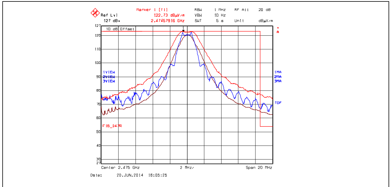
Plot 5.5.4.2.2.5. Band-Edge RF Radiated Emissions at 3 m, Vertical Polarization High End of Frequency Band, QPSK Modulation, Power -8 Mode 3
