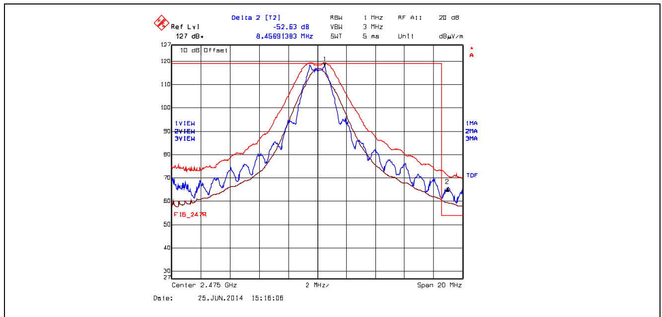
Plot 5.5.4.5.2.6. Band-Edge RF Radiated Emissions at 3 m, Vertical Polarization High End of Frequency Band, QPSK Modulation, Power -8 Mode 3
