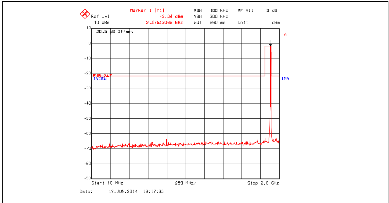
Plot 5.4.4.2.11. Conducted Spurious Emissions Channel 25, 2475 MHz, QPSK Modulation, Power Setting -26 Mode 3, 10 MHz – 2.6 GHz
