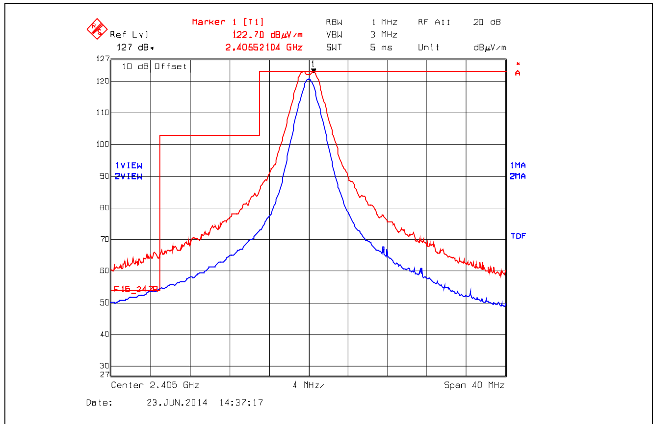
Plot 5.5.4.1.2.4. Band-Edge RF Radiated Emissions at 3 m, Vertical Polarization Low End of Frequency Band, QPSK Modulation, Power -8 Mode 3
