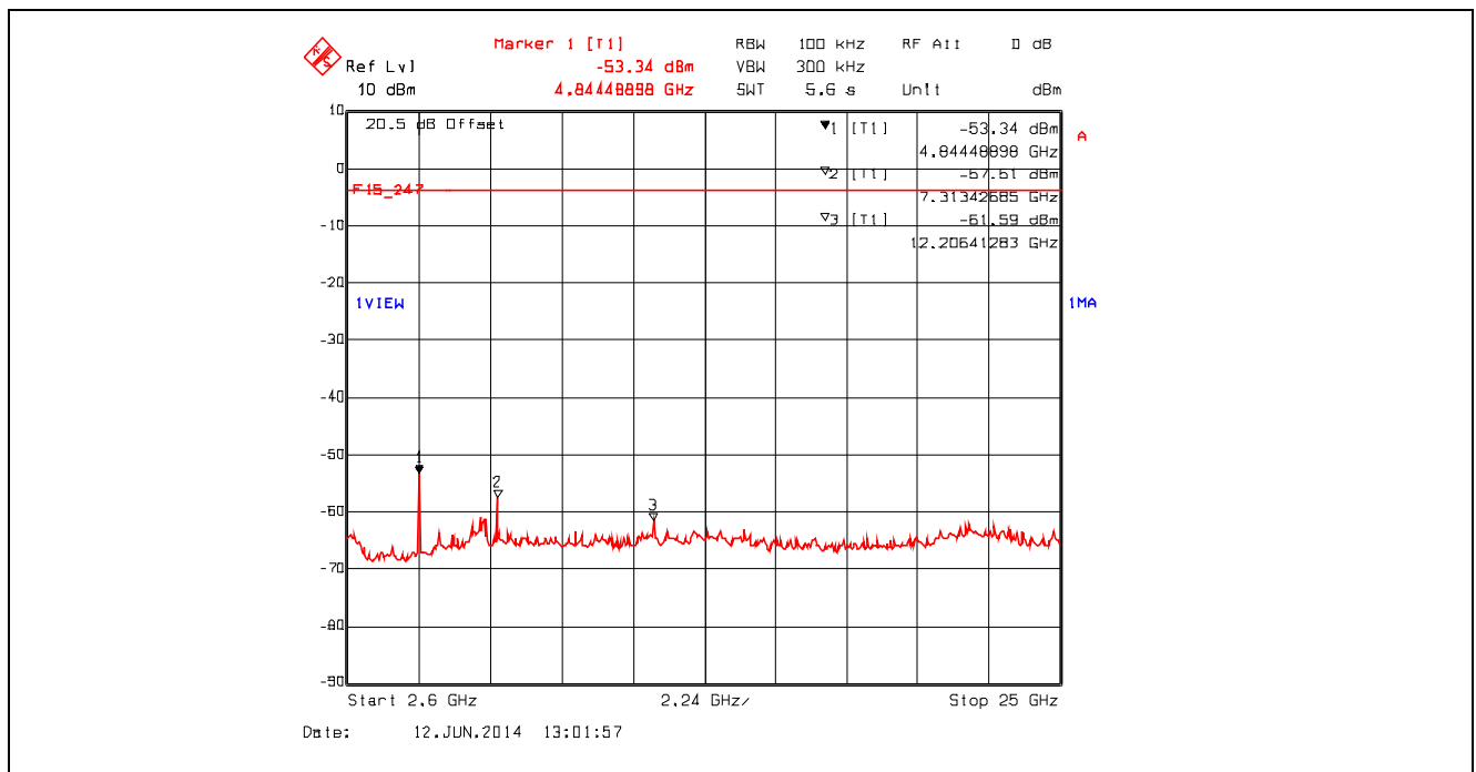
Plot 5.4.4.2.4. Conducted Spurious Emissions Channel 18, 2440 MHz, QPSK Modulation, Power Setting -8 Mode 3, 2.6 GHz – 25 GHz
