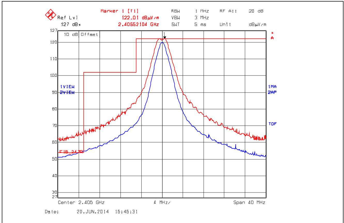
Plot 5.5.4.2.2.1. Band-Edge RF Radiated Emissions at 3 m, Horizontal Polarization Low End of Frequency Band, QPSK Modulation, Power -8 Mode 3
