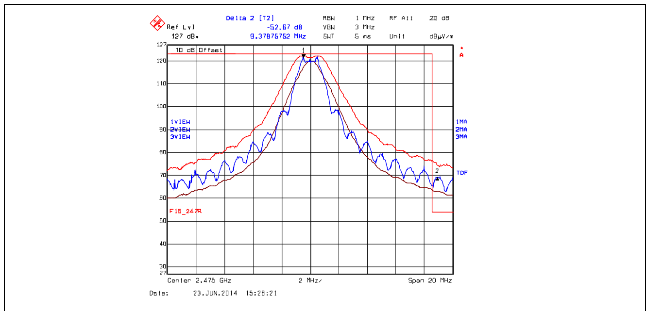
Plot 5.5.4.1.2.3. Band-Edge RF Radiated Emissions at 3 m, Horizontal Polarization High End of Frequency Band, QPSK Modulation, Power -8 Mode 3
