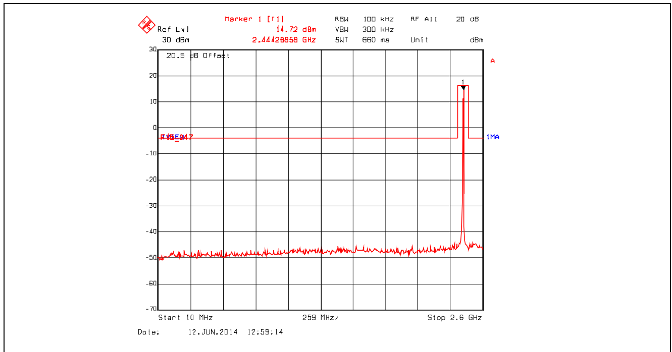
Plot 5.4.4.2.3. Conducted Spurious Emissions Channel 18, 2440 MHz, QPSK Modulation, Power Setting -8 Mode 3, 10 MHz – 2.6 GHz
