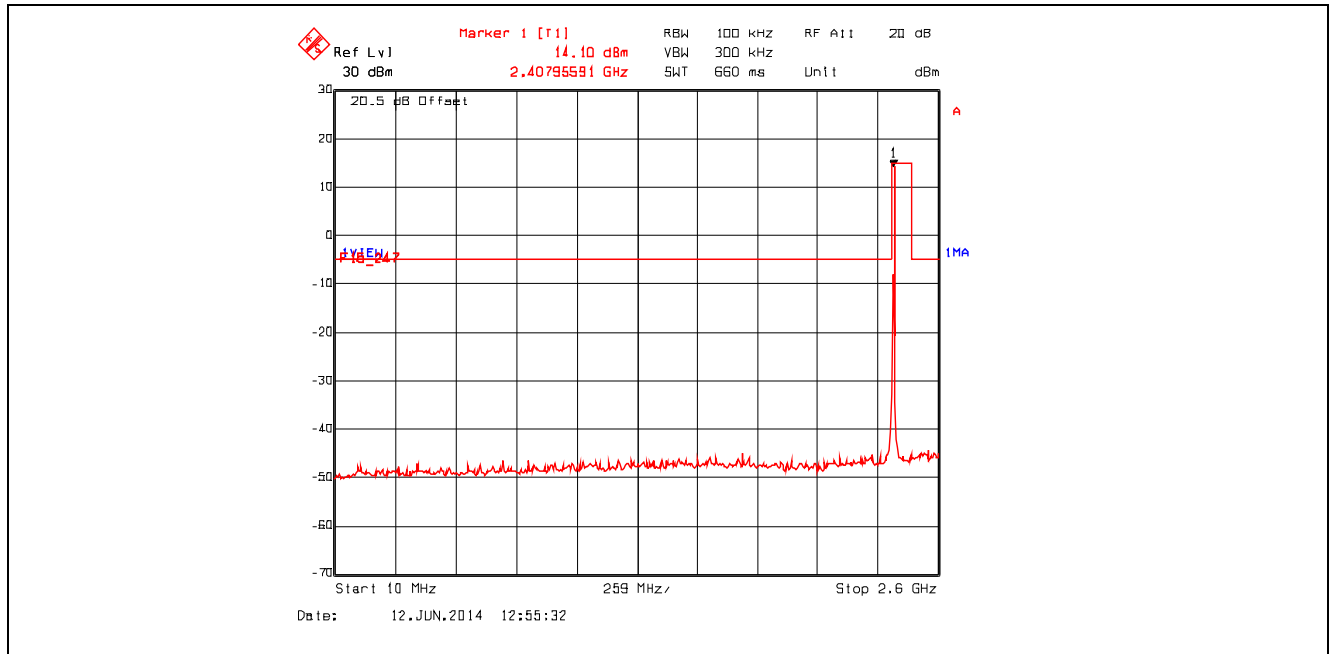
Plot 5.4.4.2.1. Conducted Spurious Emissions Channel 11, 2405 MHz, QPSK Modulation, Power Setting -8 Mode 3, 10 MHz – 2.6 GHz
