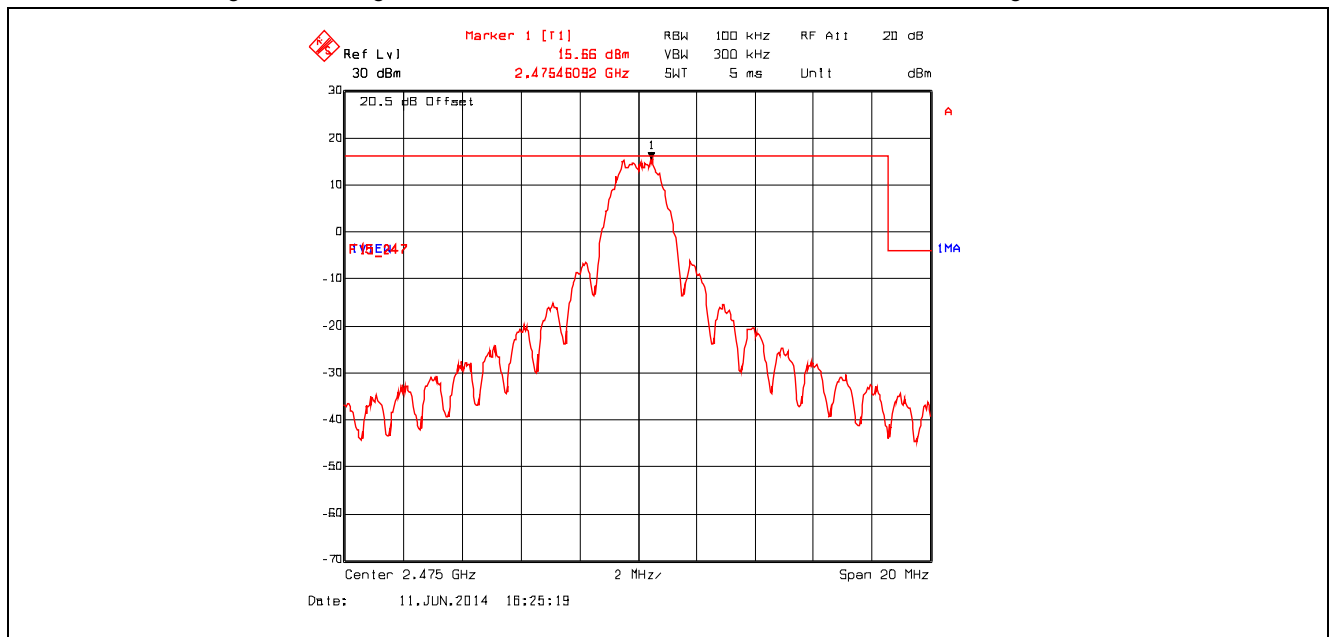
Plot 5.4.4.1.2. Band-Edge RF Conducted Emissions Higher Band-edge, Channel 25, 2475 MHz, QPSK Modulation, Power Setting -8 Mode 3
