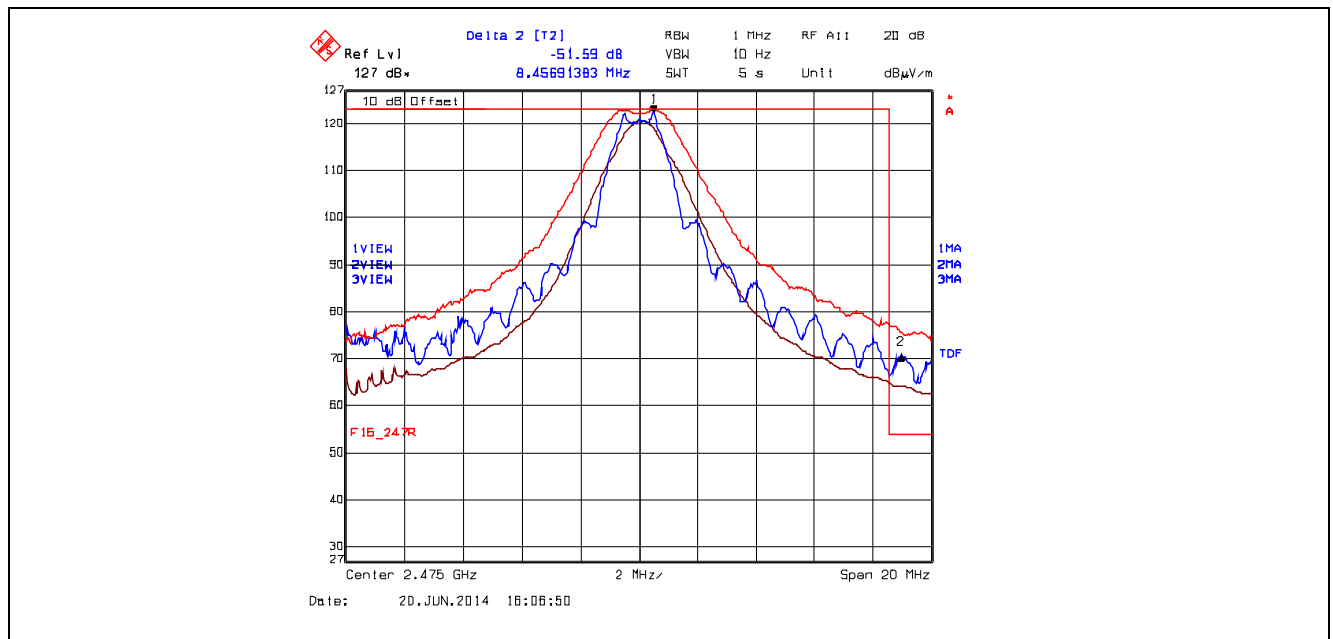
Plot 5.5.4.2.2.6. Band-Edge RF Radiated Emissions at 3 m, Vertical Polarization High End of Frequency Band, QPSK Modulation, Power -8 Mode 3
