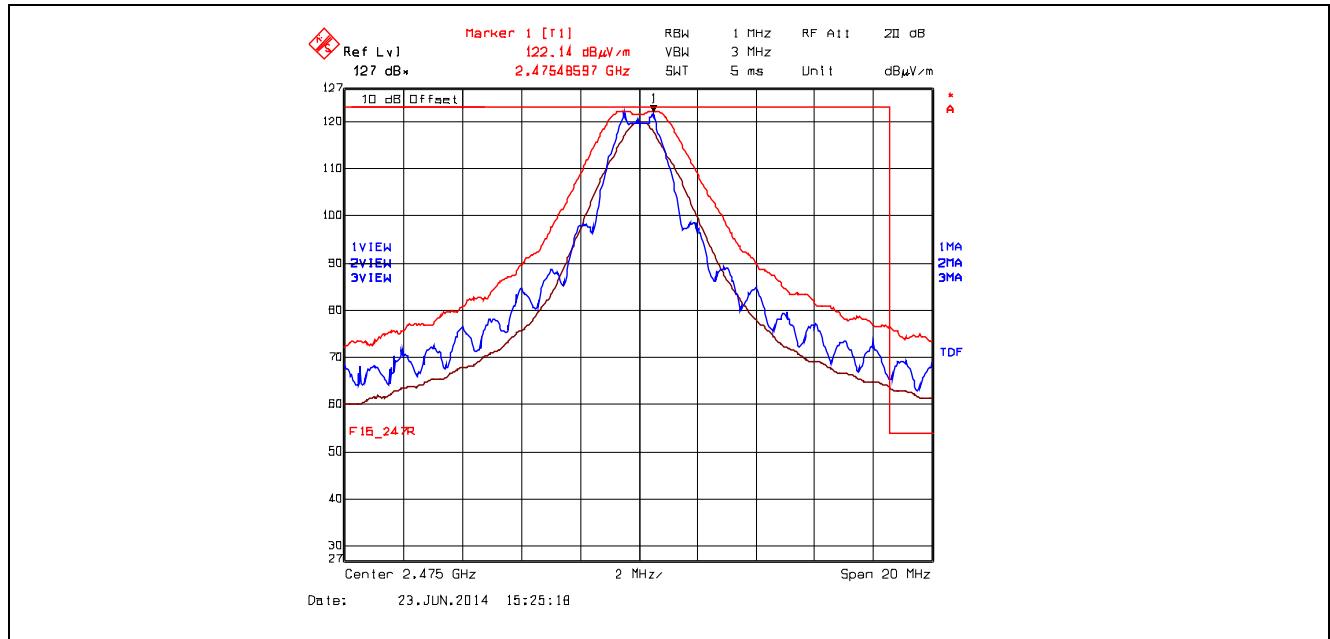
Plot 5.5.4.1.2.2. Band-Edge RF Radiated Emissions at 3 m, Horizontal Polarization High End of Frequency Band, QPSK Modulation, Power -8 Mode 3
