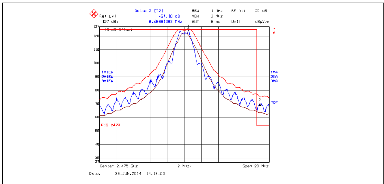
Plot 5.5.4.1.2.6. Band-Edge RF Radiated Emissions at 3 m, Vertical Polarization High End of Frequency Band, QPSK Modulation, Power -8 Mode 3
