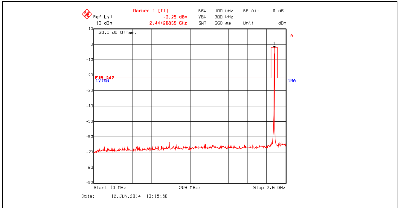
Plot 5.4.4.2.9. Conducted Spurious Emissions Channel 18, 2440 MHz, QPSK Modulation, Power Setting -26 Mode 3, 10 MHz – 2.6 GHz
