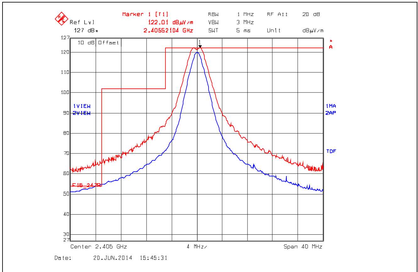
Plot 5.5.4.2.2.4. Band-Edge RF Radiated Emissions at 3 m, Vertical Polarization Low End of Frequency Band, QPSK Modulation, Power -8 Mode 3
