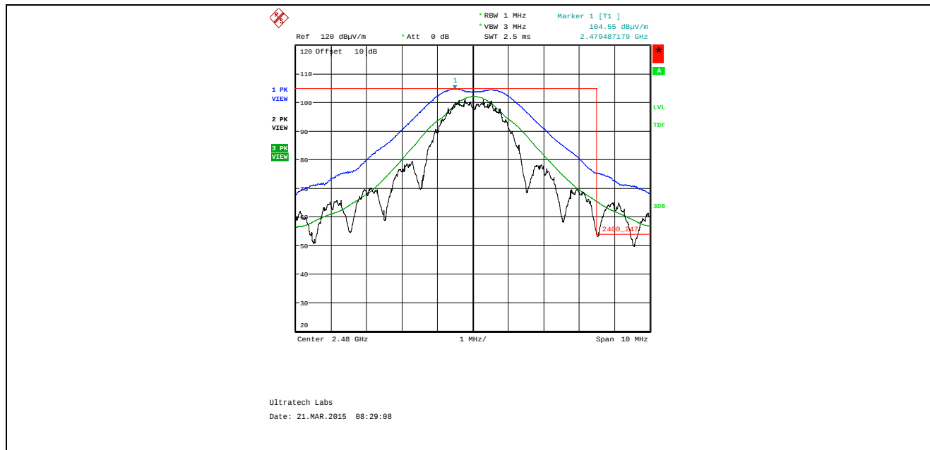
Plot 5.4.4.3.2.3. Band-Edge RF Radiated Emissions at 3 m, Vertical Polarization High End of Frequency Band, QPSK Modulation, Power -24 Mode 3
