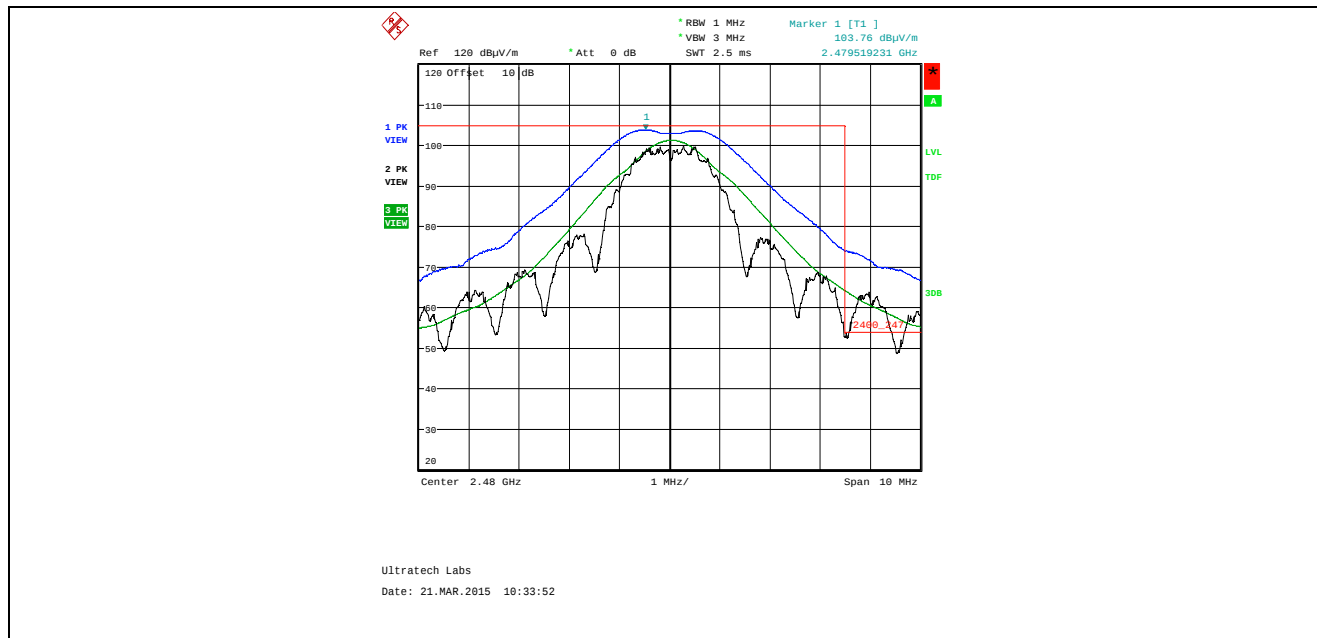
Plot 5.4.4.1.2.3. Band-Edge RF Radiated Emissions at 3 m, Vertical Polarization High End of Frequency Band, QPSK Modulation, Power -24 Mode 3
