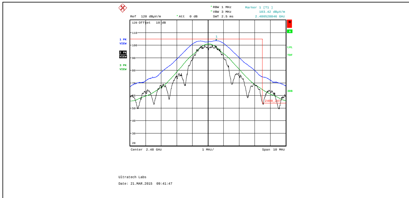
Plot 5.4.4.2.2.3. Band-Edge RF Radiated Emissions at 3 m, Vertical Polarization High End of Frequency Band, QPSK Modulation, Power -24 Mode 3
