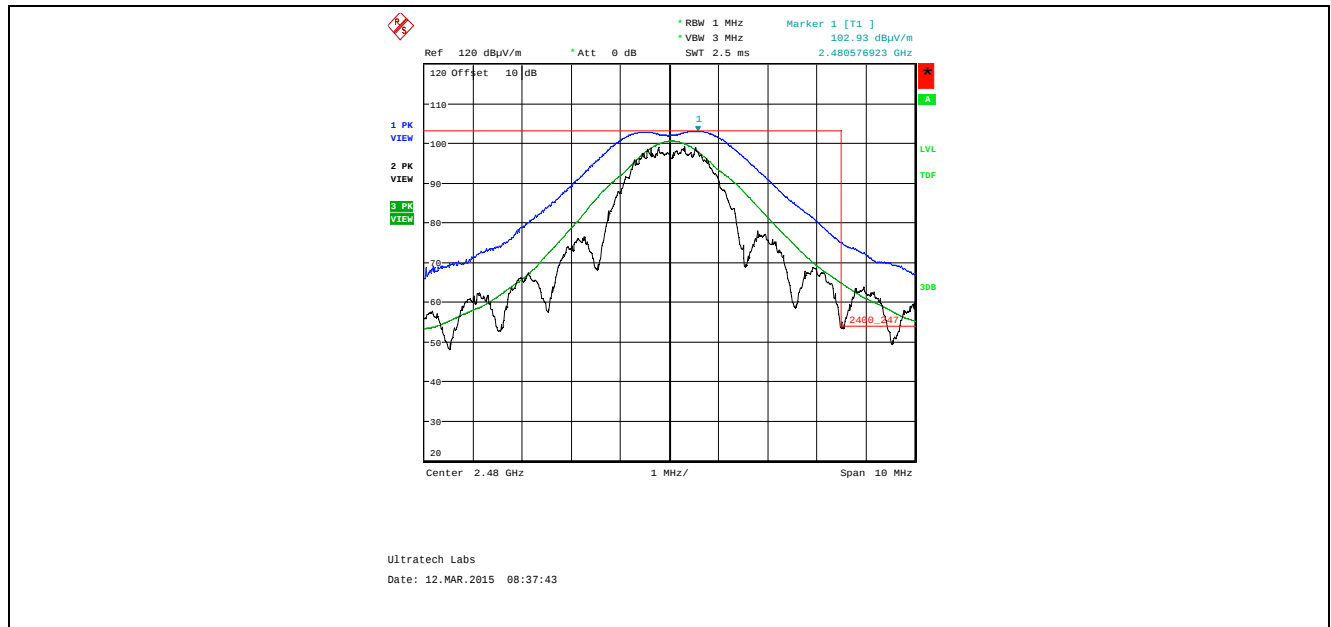
Plot 5.4.4.5.2.1. Band-Edge RF Radiated Emissions at 3 m, Horizontal Polarization High End of Frequency Band, QPSK Modulation, Power -24 Mode 3
