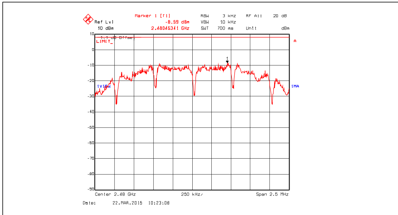
Plot 5.5.4.1. Power Spectral Density, Channel 26, 2480 MHz, QPSK Modulation, Power Setting -24 Mode 3
