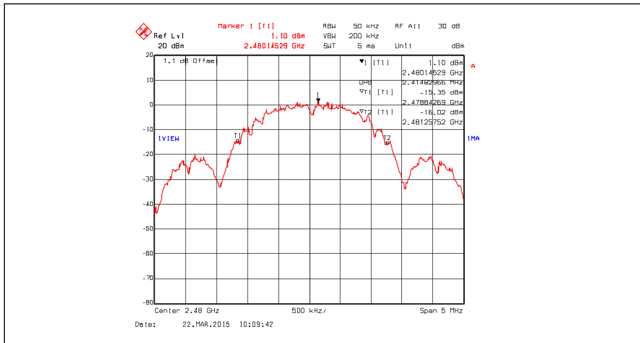
Plot 5.1.4.2. 99% Occupied Bandwidth, Channel 26, 2480 MHz, QPSK Modulation, Power Setting -24 Mode 3
