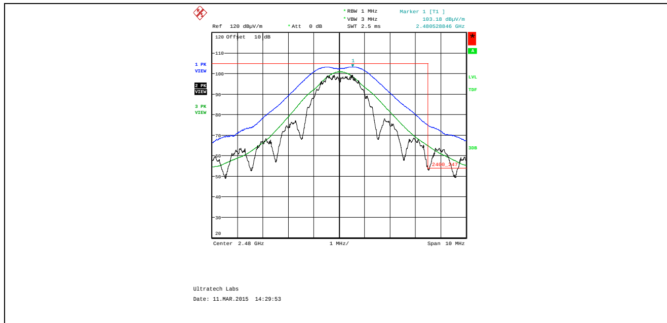
Plot 5.4.4.4.2.3. Band-Edge RF Radiated Emissions at 3 m, Vertical Polarization High End of Frequency Band, QPSK Modulation, Power -24 Mode 3
