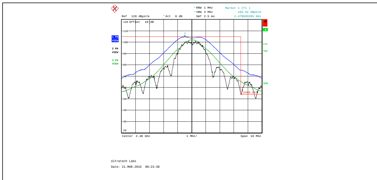
Plot 5.4.4.3.2.1. Band-Edge RF Radiated Emissions at 3 m, Horizontal Polarization High End of Frequency Band, QPSK Modulation, Power -24 Mode 3
