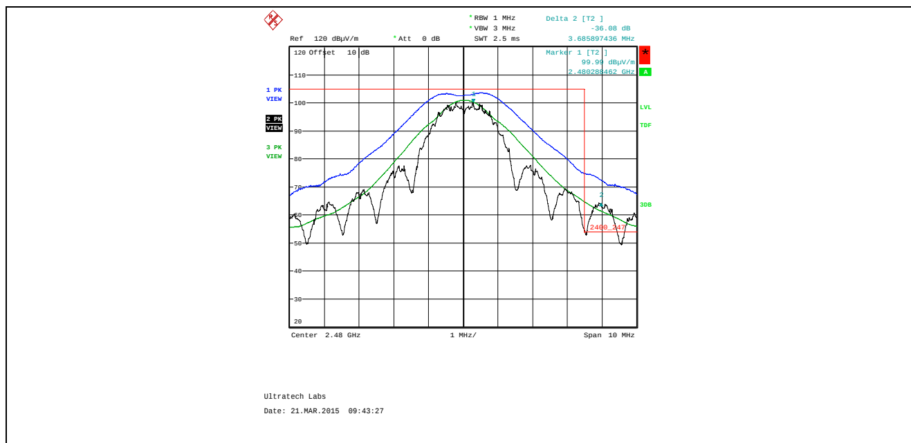
Plot 5.4.4.2.2.4. Band-Edge RF Radiated Emissions at 3 m, Vertical Polarization High End of Frequency Band, QPSK Modulation, Power -24 Mode 3
