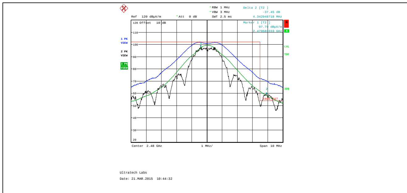
Plot 5.4.4.1.2.2. Band-Edge RF Radiated Emissions at 3 m, Horizontal Polarization High End of Frequency Band, QPSK Modulation, Power -24 Mode 3
