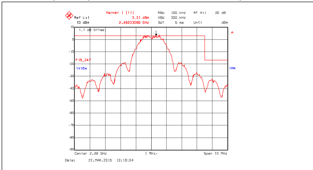
Plot 5.3.4.1.1. Band-Edge RF Conducted Emissions Higher Band-edge, Channel 26, 2480 MHz, QPSK Modulation, Power Setting -24 Mode 3
