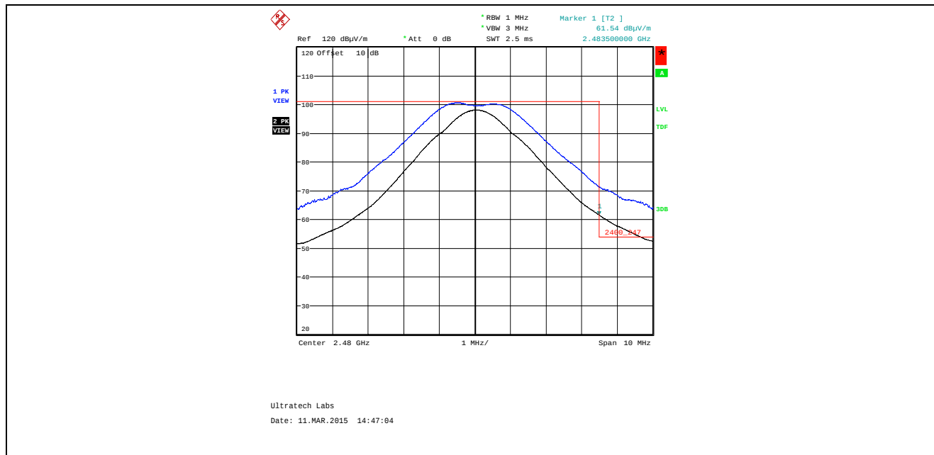
Plot 5.4.4.4.2.2. Band-Edge RF Radiated Emissions at 3 m, Horizontal Polarization High End of Frequency Band, QPSK Modulation, Power -24 Mode 3
