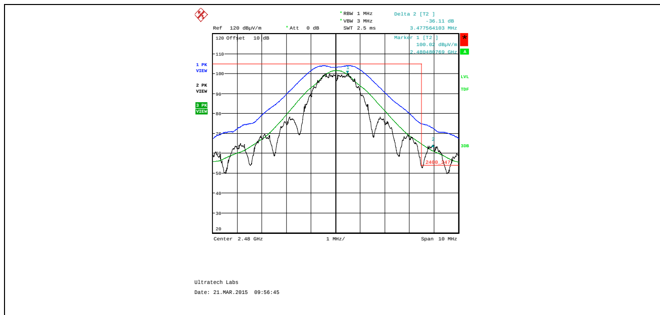
Plot 5.4.4.2.2.2. Band-Edge RF Radiated Emissions at 3 m, Horizontal Polarization High End of Frequency Band, QPSK Modulation, Power -24 Mode 3
