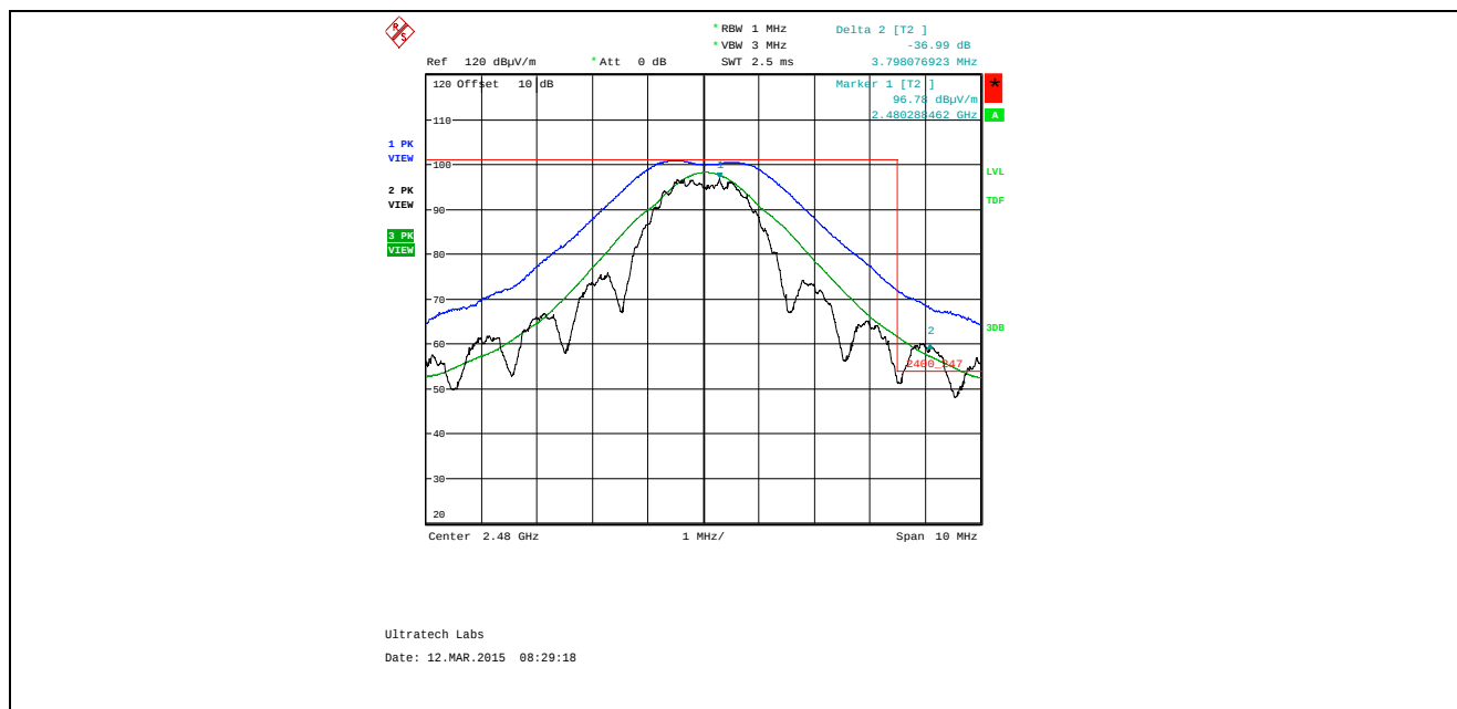
Plot 5.4.4.5.2.4. Band-Edge RF Radiated Emissions at 3 m, Vertical Polarization High End of Frequency Band, QPSK Modulation, Power -24 Mode 3
