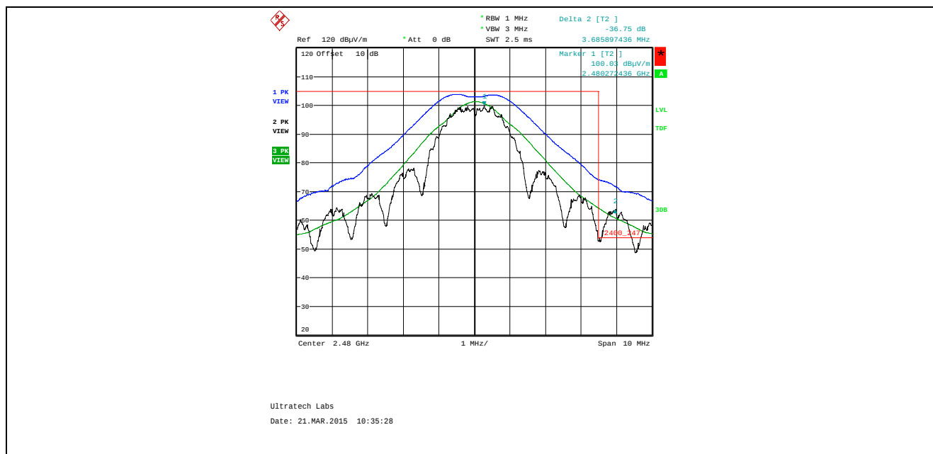
Plot 5.4.4.1.2.4. Band-Edge RF Radiated Emissions at 3 m, Vertical Polarization High End of Frequency Band, QPSK Modulation, Power -24 Mode 3
