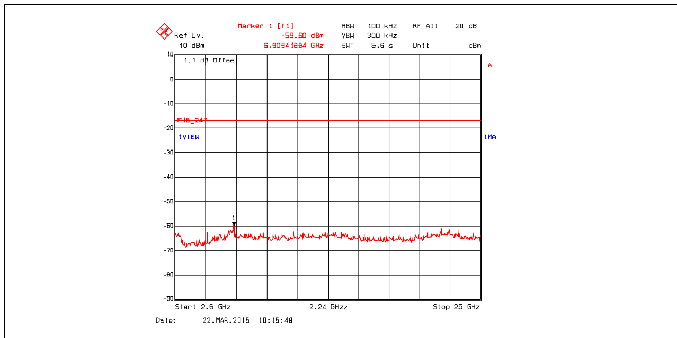
Plot 5.3.4.2.2. Conducted Spurious Emissions Channel 26, 2480 MHz, QPSK Modulation, Power Setting -24 Mode 3, 2.6 GHz – 25 GHz
