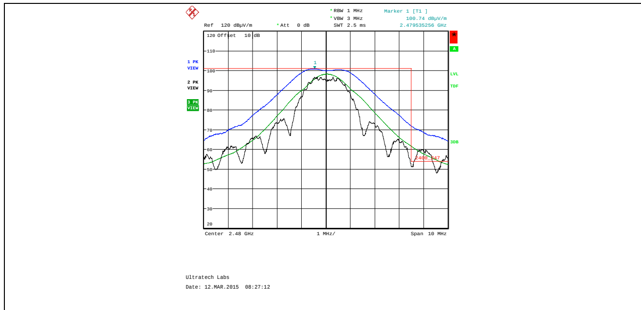
Plot 5.4.4.5.2.3. Band-Edge RF Radiated Emissions at 3 m, Vertical Polarization High End of Frequency Band, QPSK Modulation, Power -24 Mode 3
