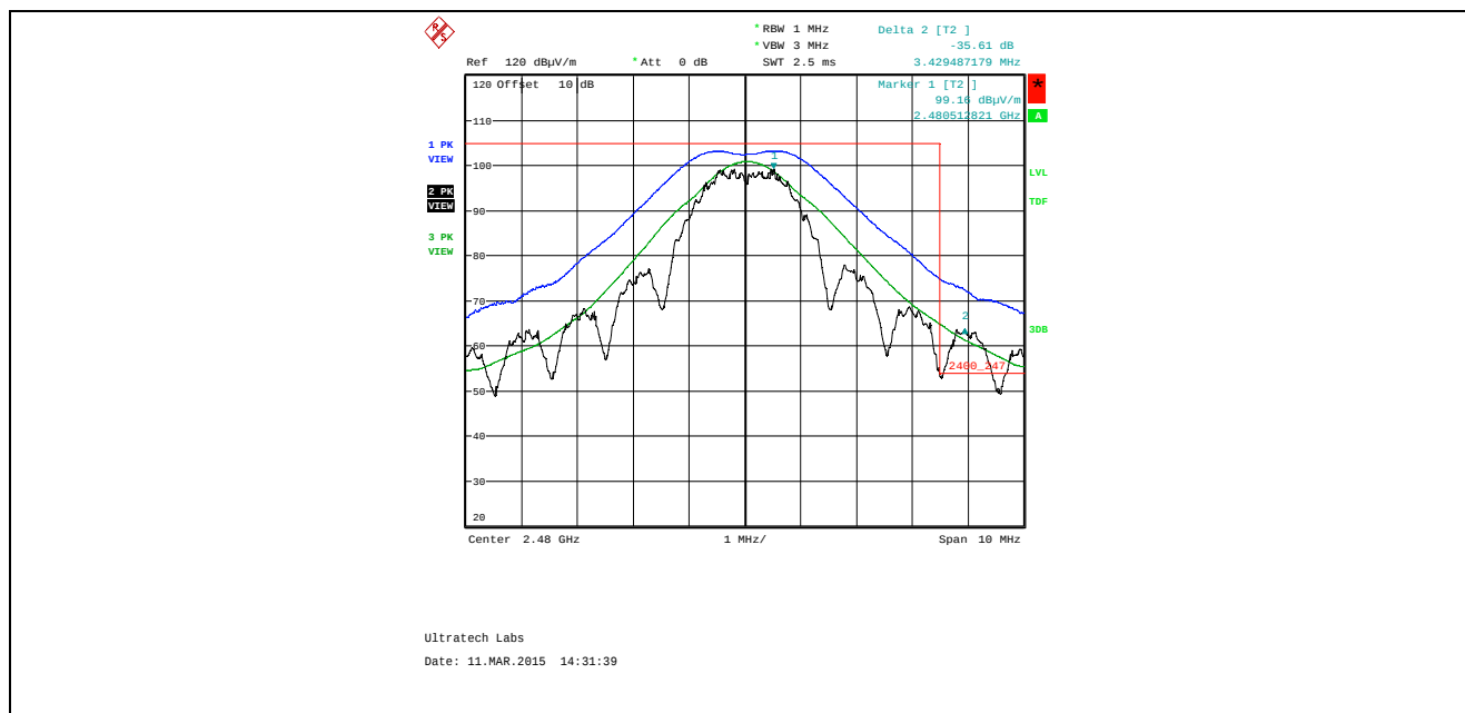
Plot 5.4.4.4.2.4. Band-Edge RF Radiated Emissions at 3 m, Vertical Polarization High End of Frequency Band, QPSK Modulation, Power -24 Mode 3
