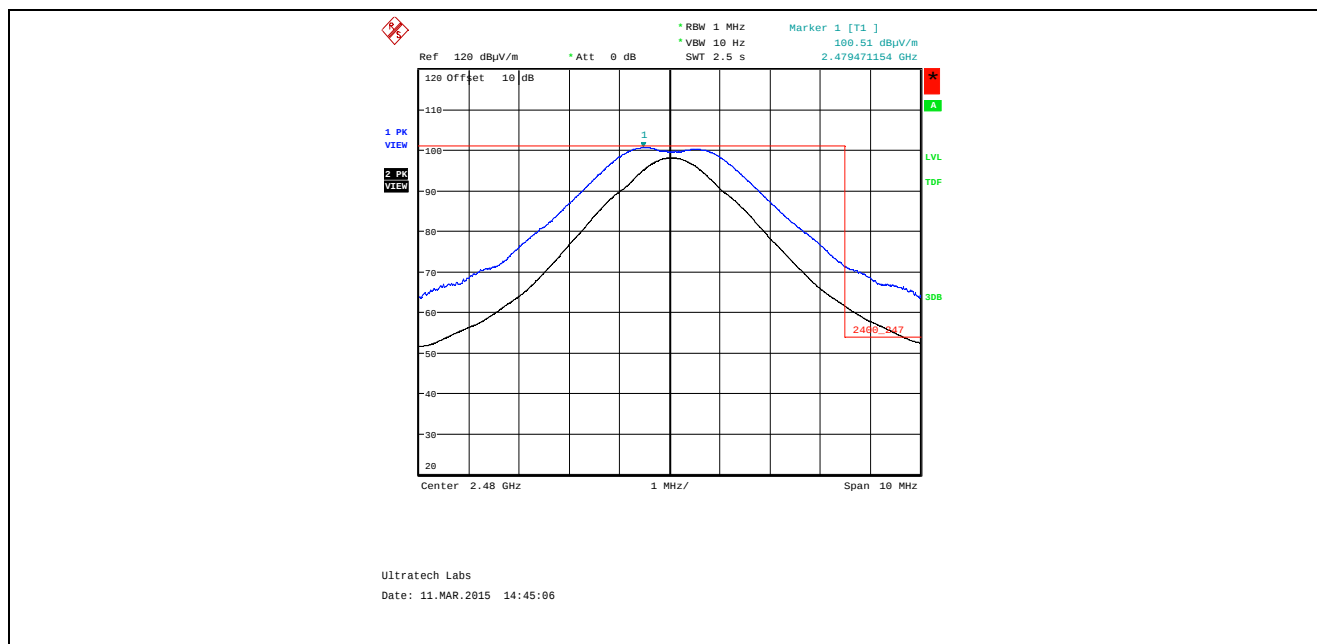
Plot 5.4.4.4.2.1. Band-Edge RF Radiated Emissions at 3 m, Horizontal Polarization High End of Frequency Band, QPSK Modulation, Power -24 Mode 3
