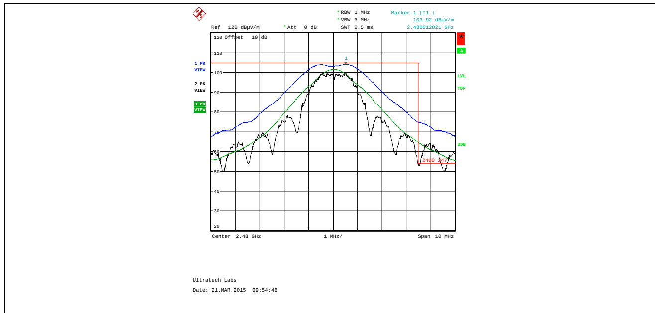
Plot 5.4.4.2.2.1. Band-Edge RF Radiated Emissions at 3 m, Horizontal Polarization High End of Frequency Band, QPSK Modulation, Power -24 Mode 3
