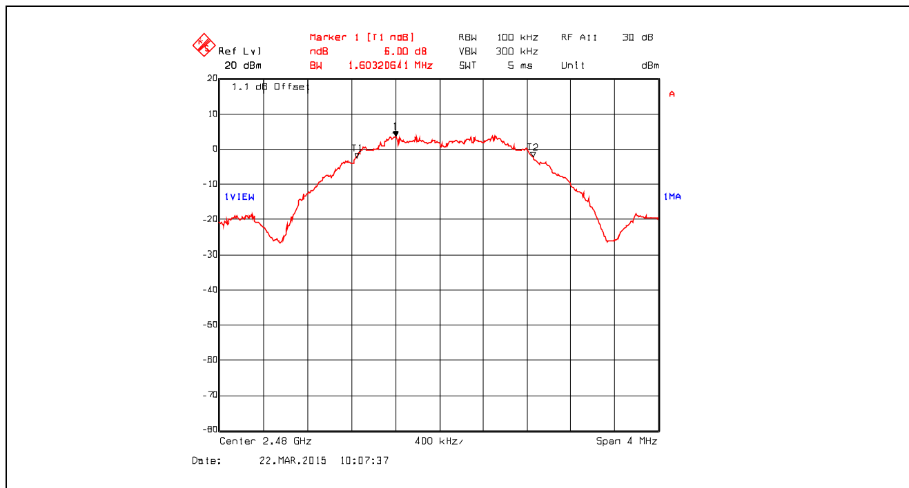
Plot 5.1.4.1. 6 dB Bandwidth, Channel 26, 2480 MHz, QPSK Modulation, Power Setting -24 Mode 3
