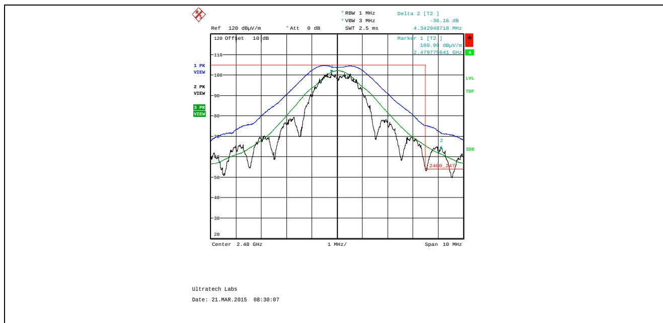
Plot 5.4.4.3.2.4. Band-Edge RF Radiated Emissions at 3 m, Vertical Polarization High End of Frequency Band, QPSK Modulation, Power -24 Mode 3
