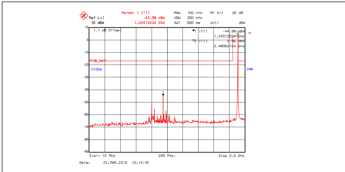
Plot 5.3.4.2.1. Conducted Spurious Emissions Channel 26, 2480 MHz, QPSK Modulation, Power Setting -24 Mode 3, 10 MHz – 2.6 GHz
