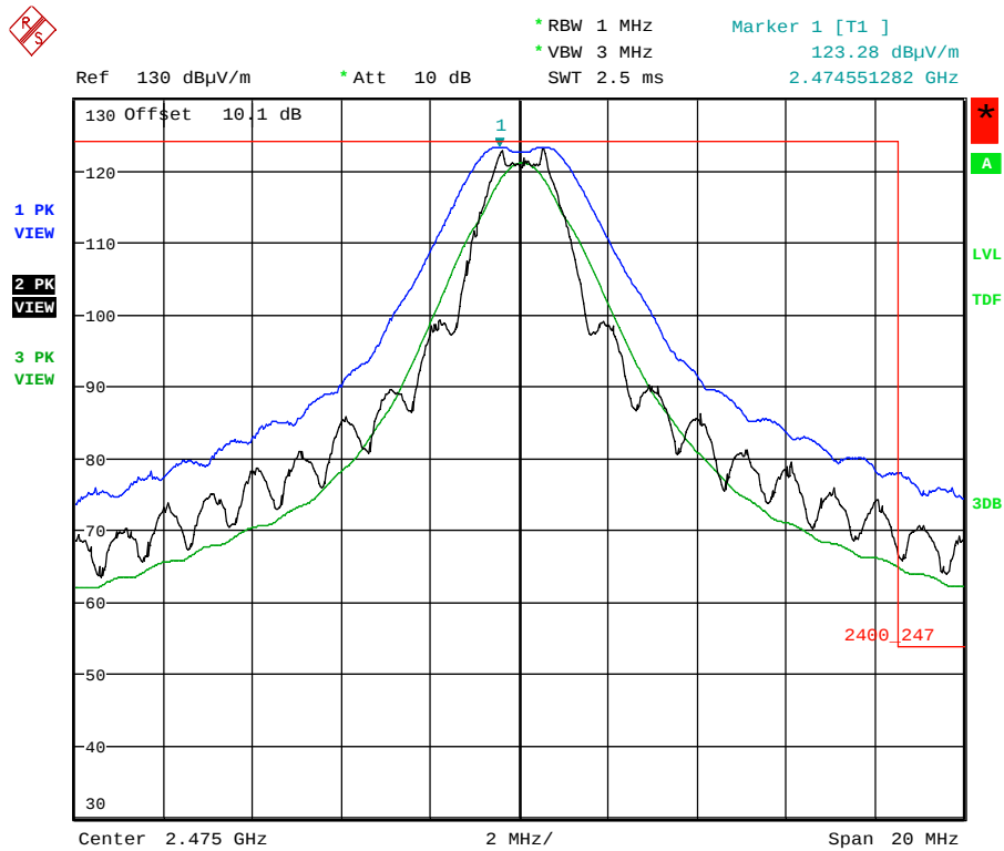
Plot 5.5.4.2.2.2. Band-Edge RF Radiated Emissions at 3 m, Horizontal Polarization High End of Frequency Band, QPSK Modulation, Power -7 Mode 3
