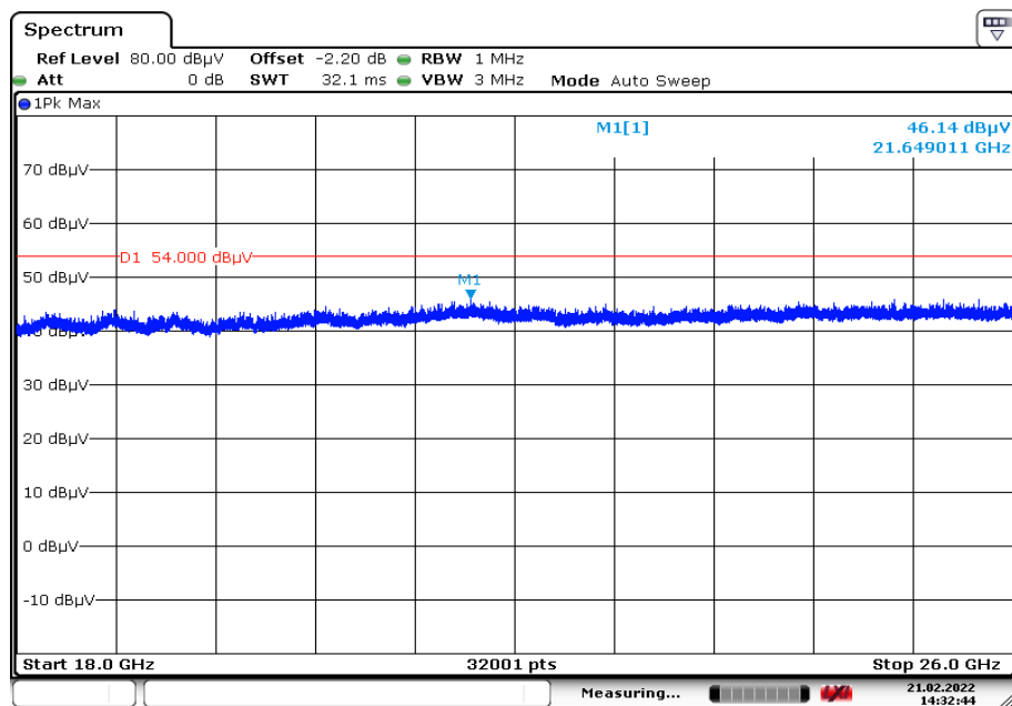
Plot 4: 18 GHz to 26 GHz, TX mode, valid for all channels, vertical & horizontal polarization
