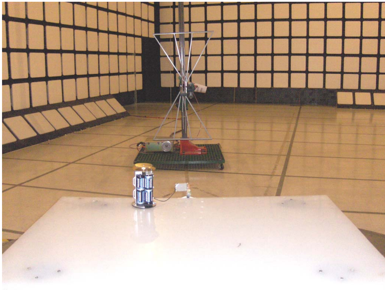
Radiated Emissions at 3 m EUT with 0 dBi Disc-Patch Antenna (Orthogonal Position 3)
