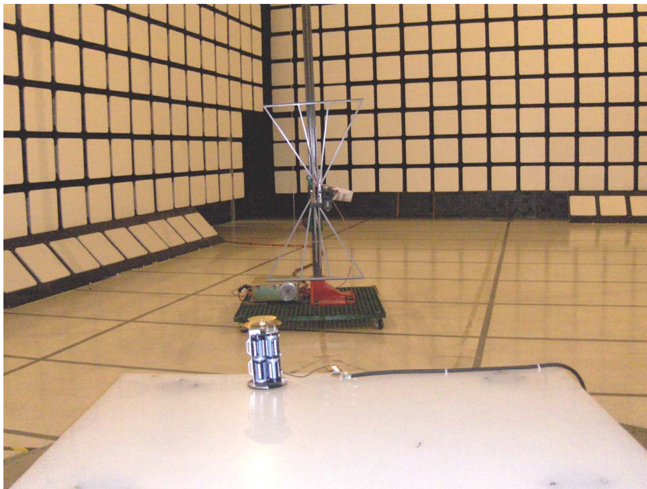
Radiated Emissions at 3 m EUT with 0 dBi Disc-Patch Antenna (Orthogonal Position 1)
