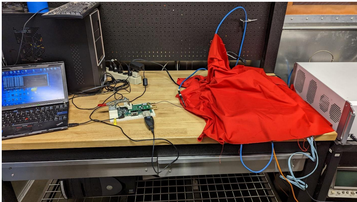
DIGI107 DFS Conducted Setup
