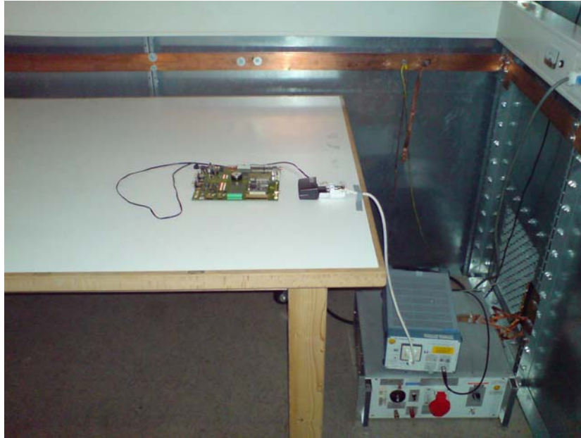
Picture 4: Conducted emissions to AC-mains test setup
