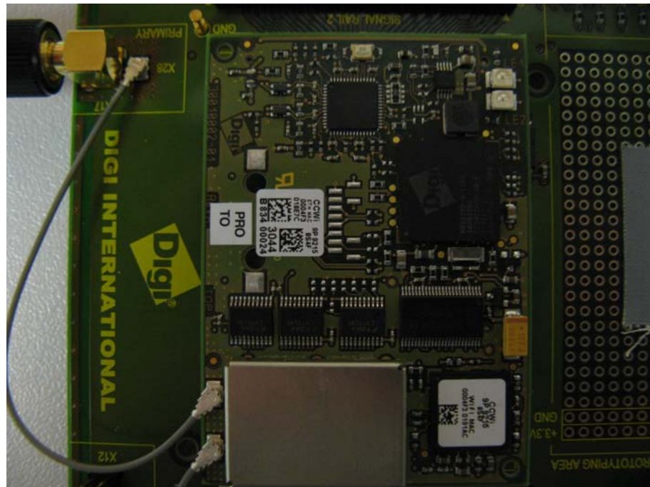
Picture 6: Photo of the EUT bottom
