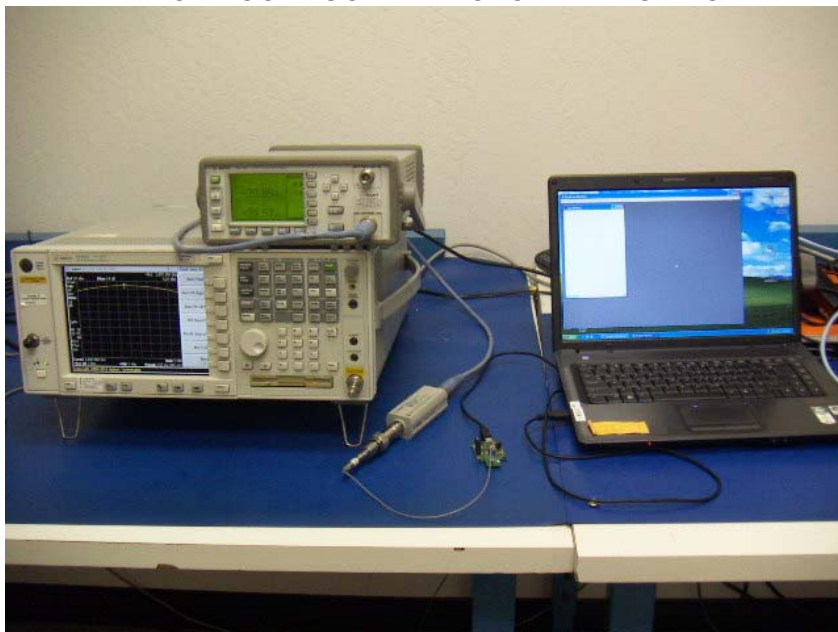
ANTENNA PORT CONDUCTED PHOTO AVERAGE POWER
