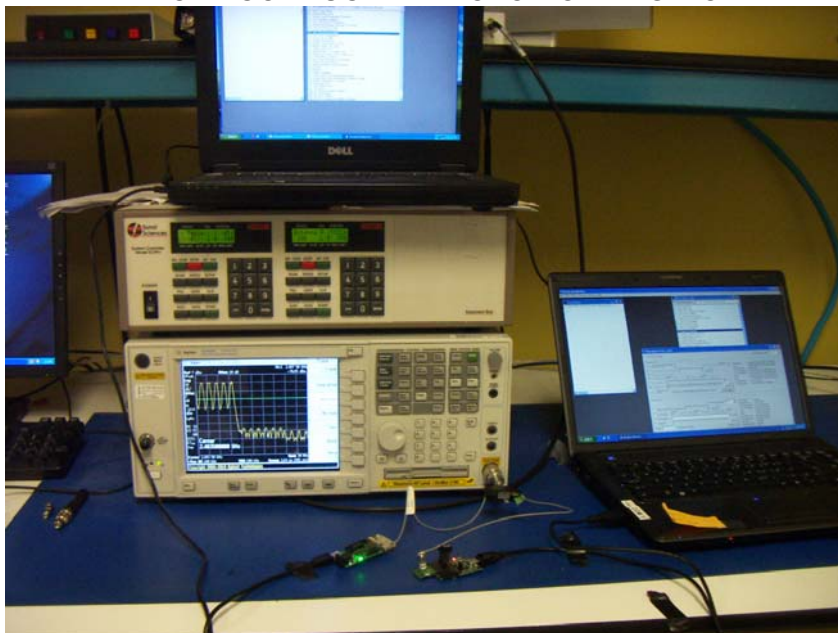
ANTENNA PORT CONDUCTED PHOTO HOPPING MODE
