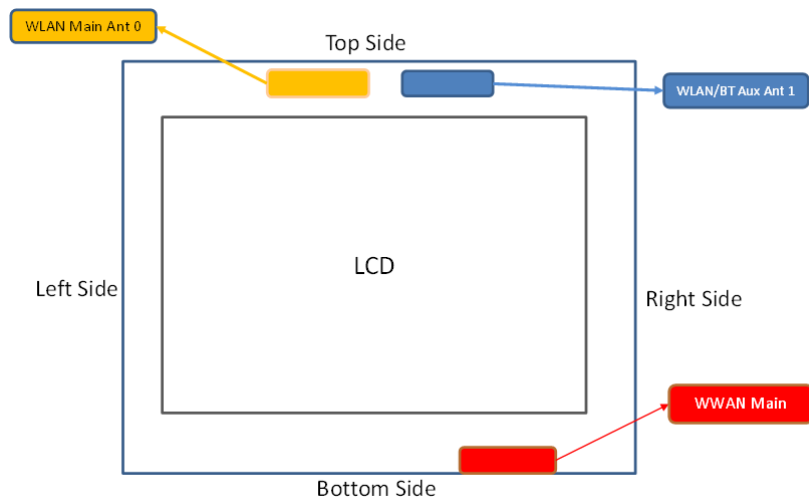
<EUT Front View>
