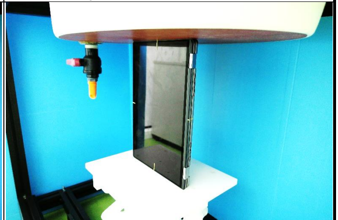
Body - Right Side of EUT at 0 mm
