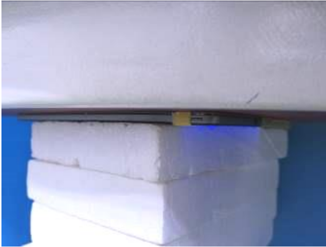
Fig-4.1 Rear Face of EUT with 0 mm Gap_Sample 1
