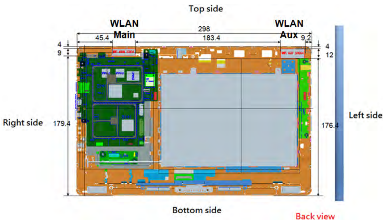
Fig.8 Antenna position of EUT (Back view)
