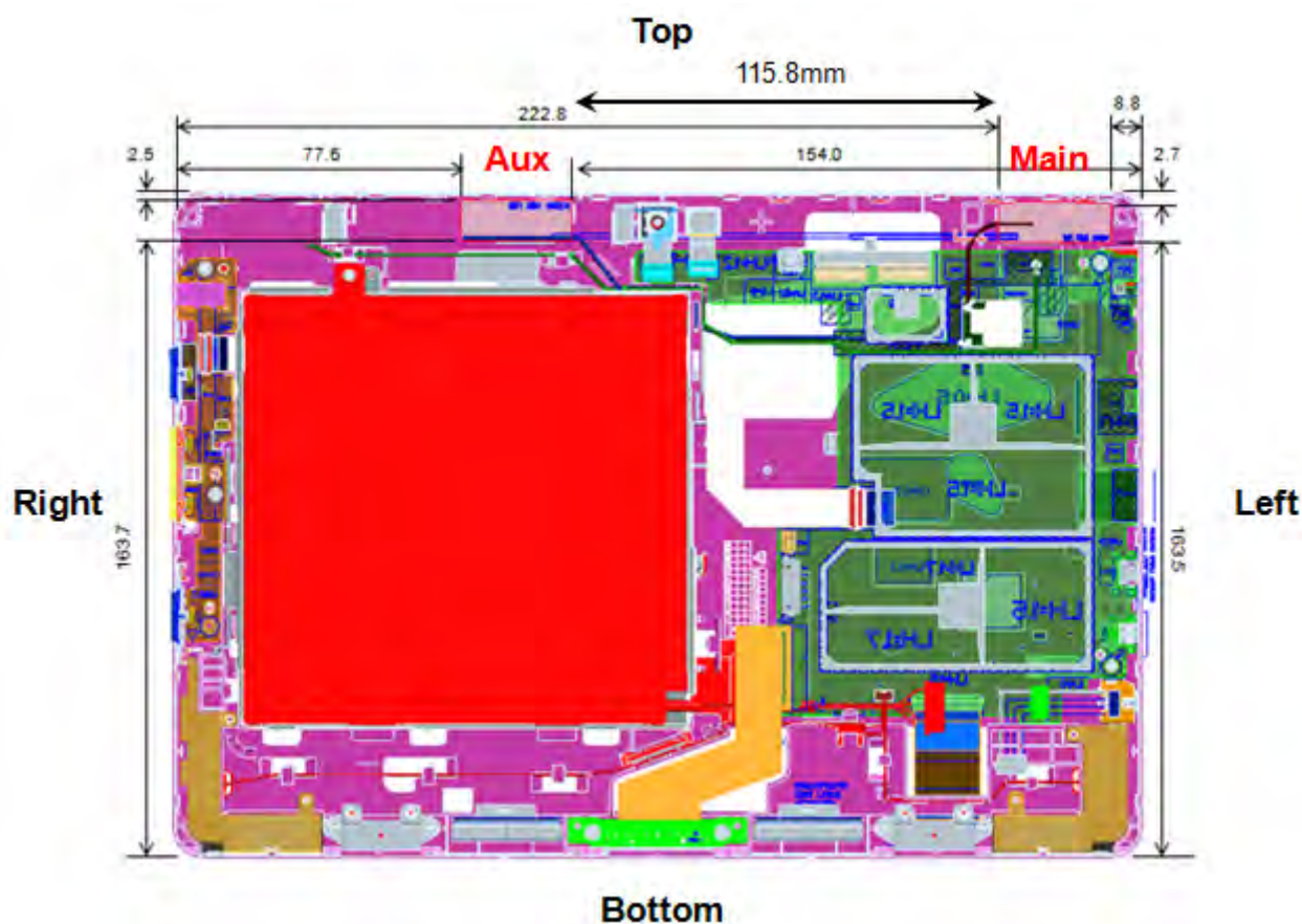
Fig.8 Antenna position of EUT (Back view)
