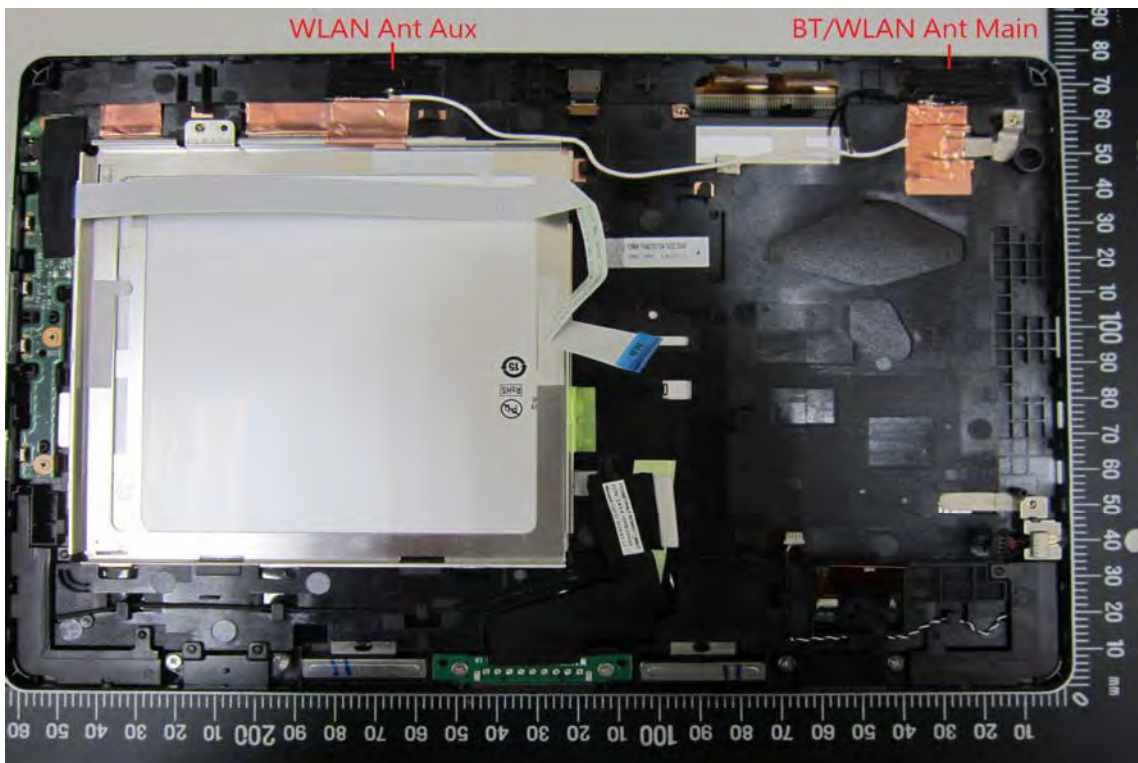
Antenna Location
