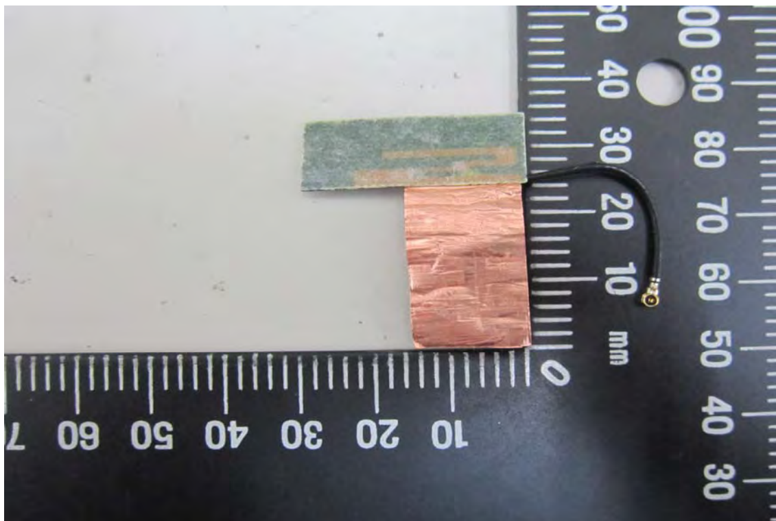
Antenna Aux - 1
