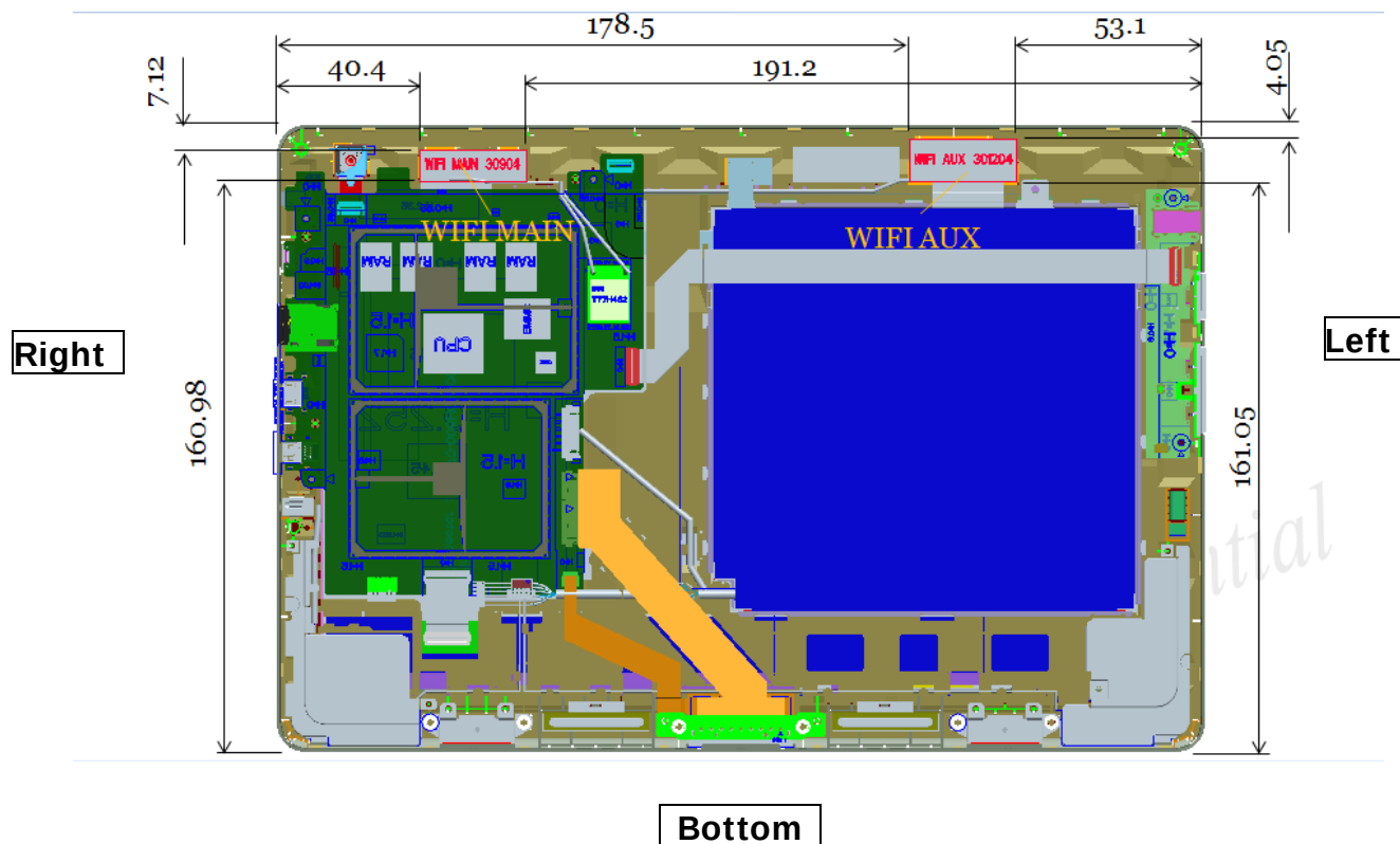
Fig.8 Antenna position of EUT (Back view)
