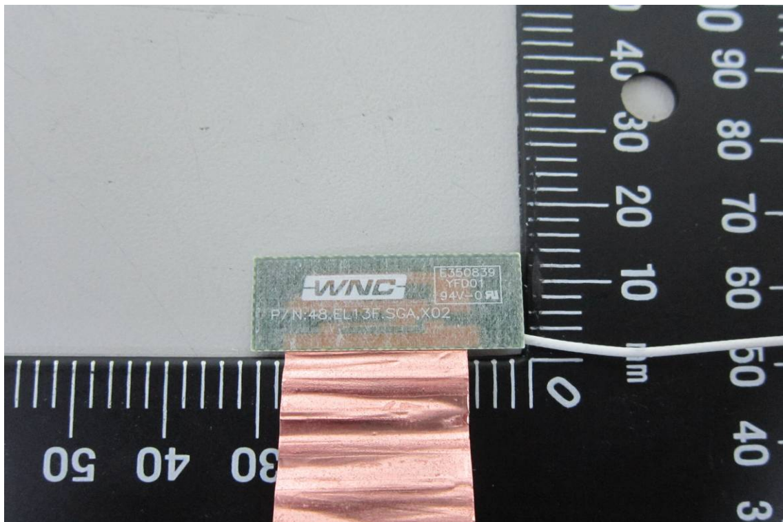
Antenna Aux - 1
