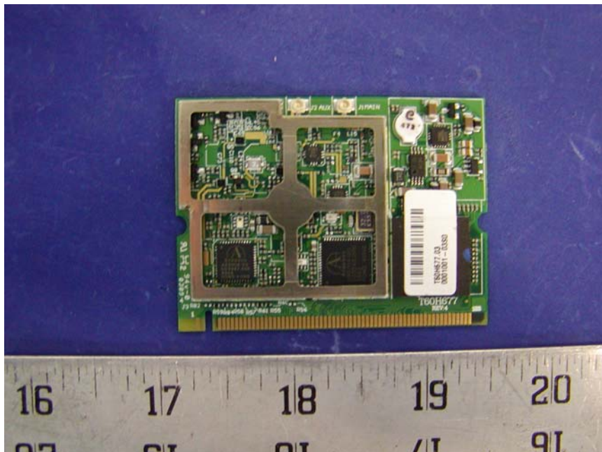
EUT – Cover Removed View
