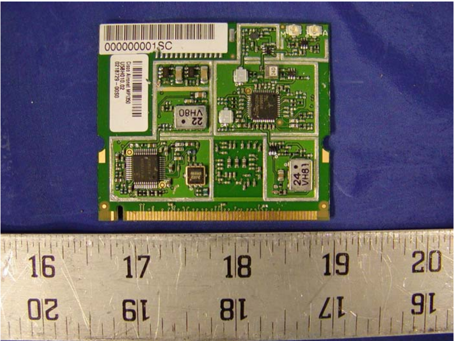
Shield Removed Top View
